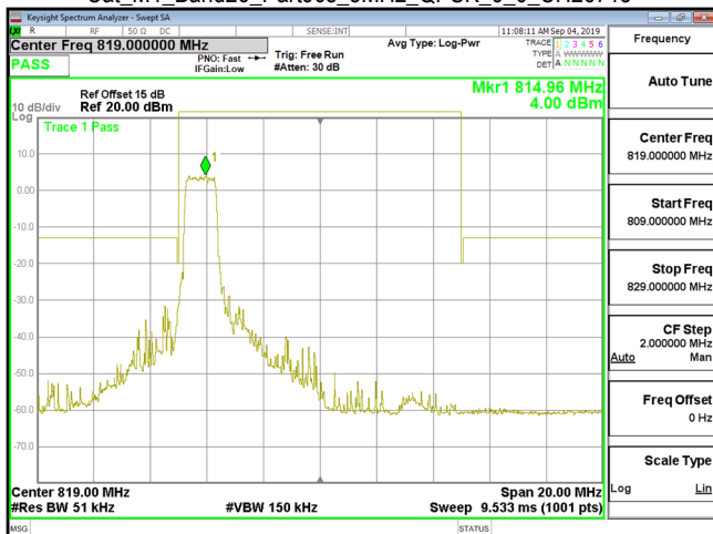
Cat_M1_Band26_Part90s_5MHz_QPSK_6_0_CH26715
