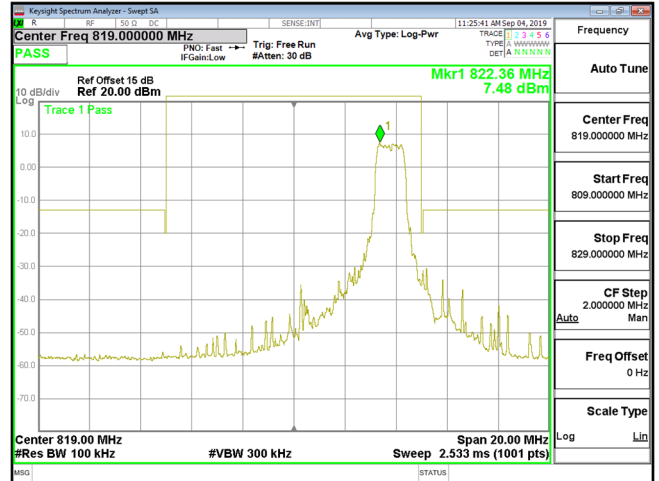
Cat_M1_Index 7_Band26_Part90s_10MHz_QPSK_50_0_CH26740
