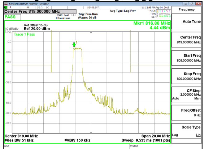
Cat_M1_Band26_Part90s_5MHz_QPSK_6_0_CH26740
