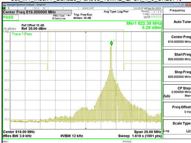
Cat_M1_Index 7_Band26_Part90s_10MHz_QPSK_1_0_CH26740
