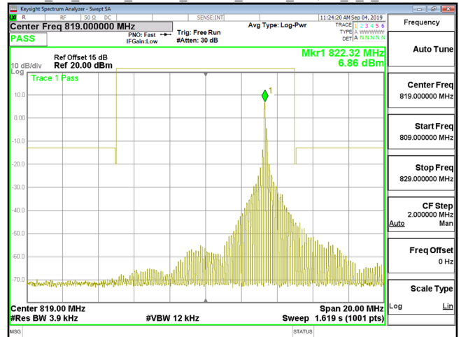
Cat_M1_Index 7_Band26_Part90s_10MHz_16QAM_1_0_CH26740
