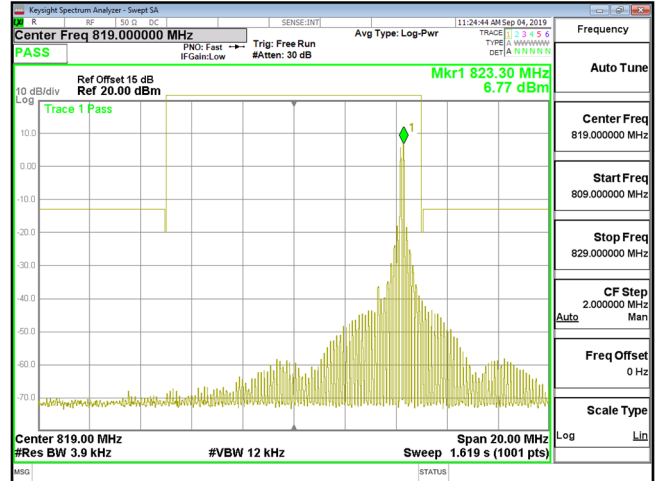
Cat_M1_Index 7_Band26_Part90s_10MHz_QPSK_1_49_CH26740
