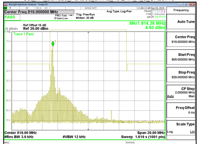
Cat_M1_Band26_Part90s_5MHz_16QAM_1_0_CH26715
