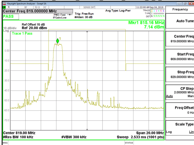
Cat_M1_Index 0_Band26_Part90s_10MHz_16QAM_6_0_CH26740
