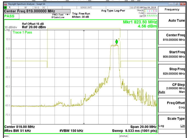
Cat_M1_Band26_Part90s_5MHz_QPSK_6_0_CH26765
