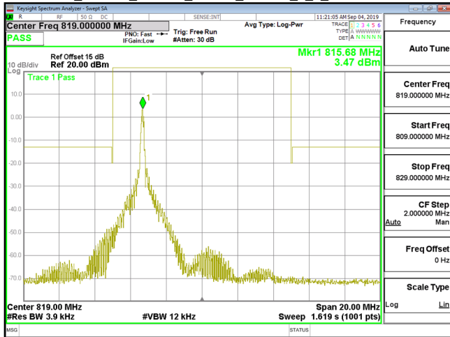
Cat_M1_Index 0_Band26_Part90s_10MHz_16QAM_6_0_CH26740
