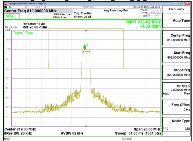
Cat_M1_Band26_Part90s_1.4MHz_QPSK_6_0_CH26740
