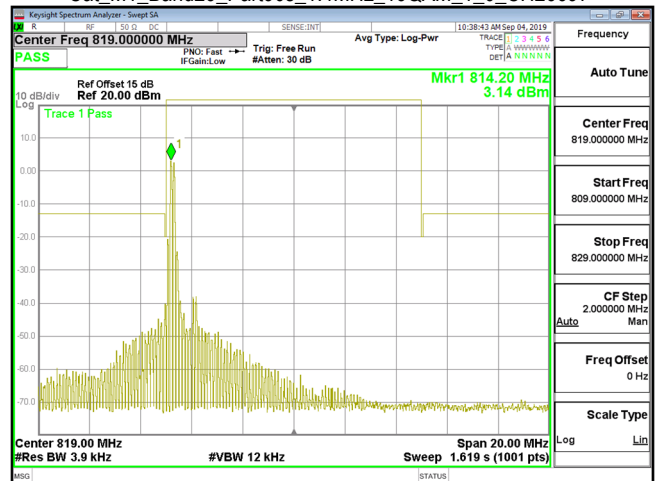
Cat_M1_Band26_Part90s_1.4MHz_16QAM_1_0_CH26697
