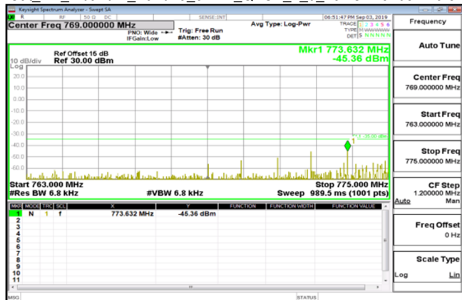
Cat_M1_Inband-1_Band13_5MHz_QPSK_1_0_LowCH23205-779.5
