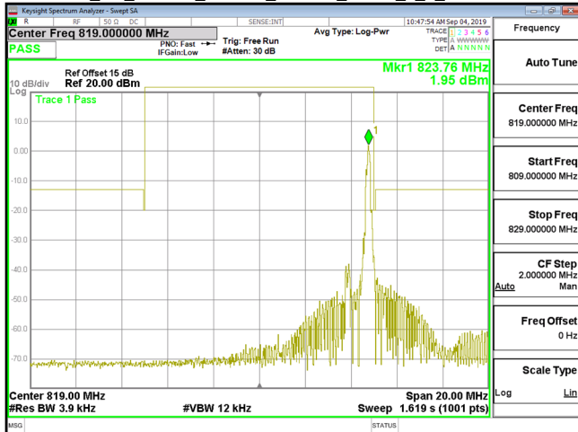
Cat_M1_Band26_Part90s_1.4MHz_QPSK_1_5_CH26783
