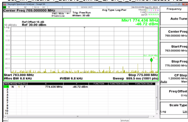
Cat_M1_Inband-1_Band13_5MHz_QPSK_1_0_MidCH23230-782
