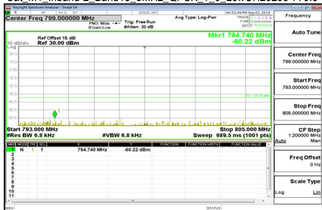
Cat_M1_Inband-2_Band13_5MHz_QPSK_1_0_LowCH23205-779.5
