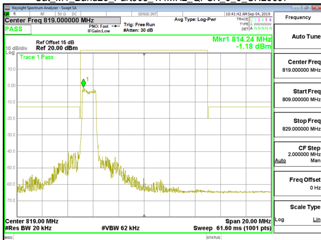
Cat_M1_Band26_Part90s_1.4MHz_QPSK_6_0_CH26697
