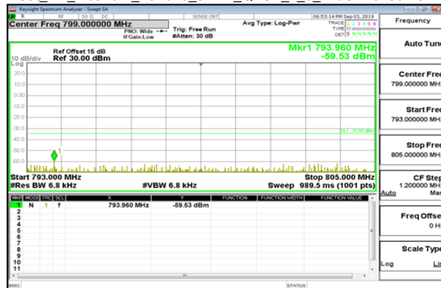
Cat_M1_Inband-2_Band13_5MHz_QPSK_1_0_MidCH23230-782
