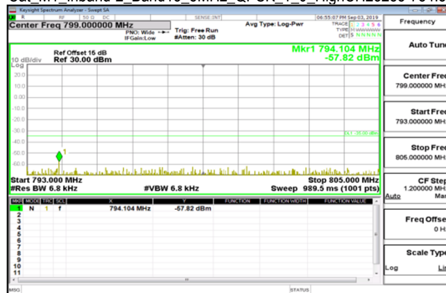
Cat_M1_Inband-2_Band13_5MHz_QPSK_1_0_HighCH23255-784.5
