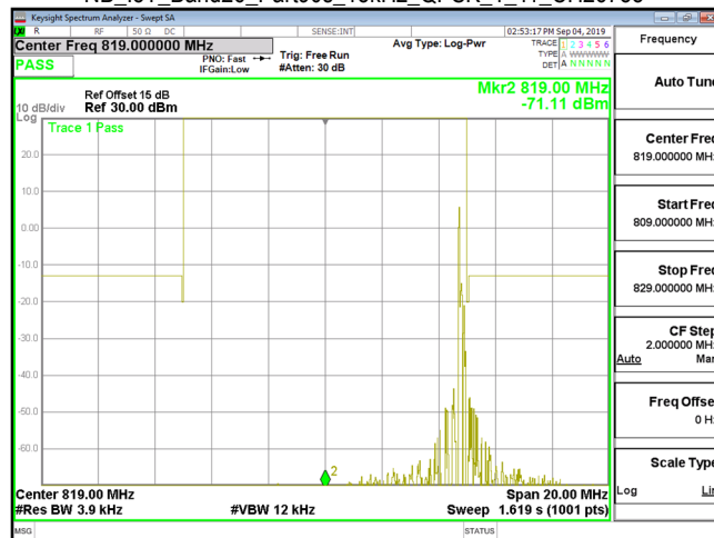
NB_IoT_Band26_Part90s_15kHz_QPSK_1_11_CH26788
