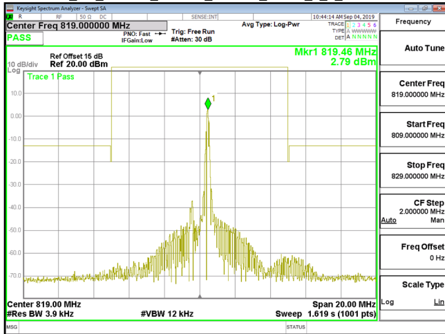
Cat_M1_Band26_Part90s_1.4MHz_QPSK_1_5_CH26740
