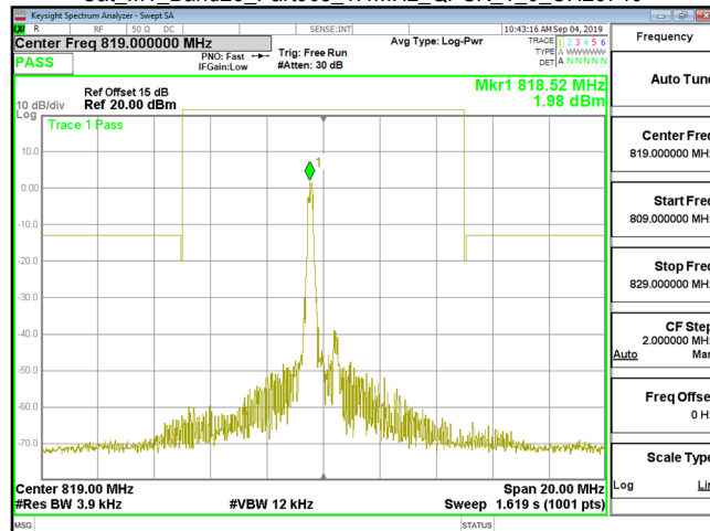
Cat_M1_Band26_Part90s_1.4MHz_QPSK_1_0_CH26740
