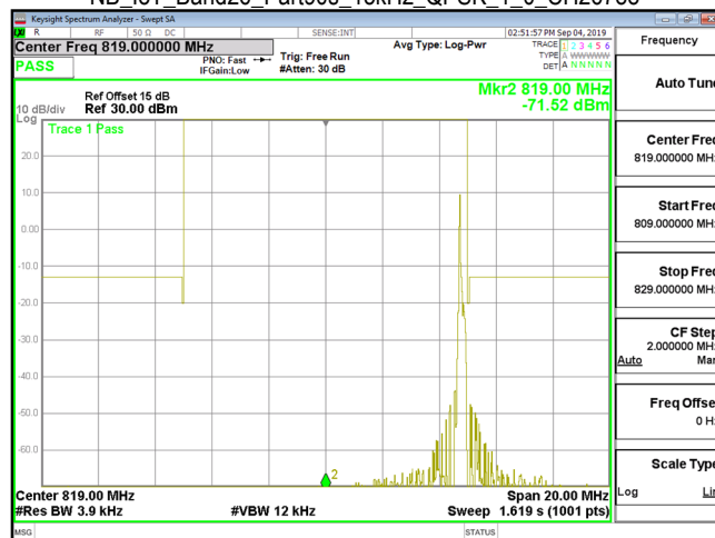
NB_IoT_Band26_Part90s_15kHz_QPSK_1_0_CH26788
