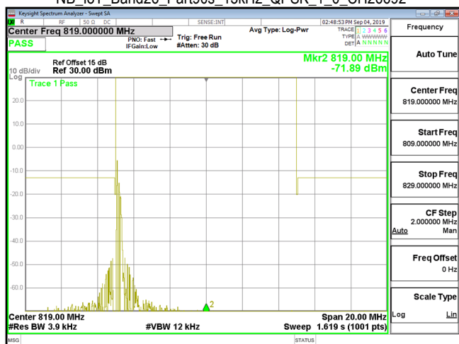
NB_IoT_Band26_Part90s_15kHz_QPSK_1_0_CH26740
