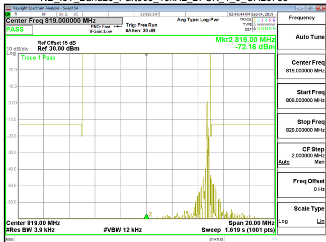
NB_IoT_Band26_Part90s_15kHz_BPSK_1_0_CH26788
