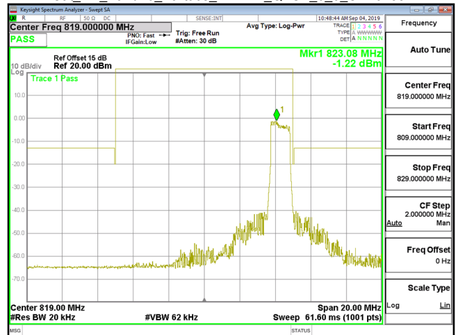
Cat_M1_Band26_Part90s_1.4MHz_QPSK_6_0_CH26783
