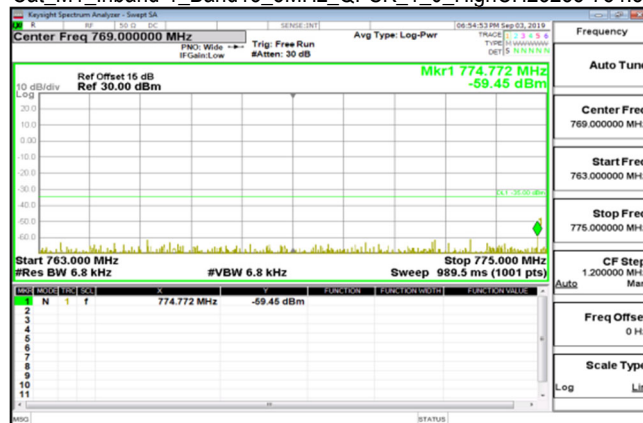
Cat_M1_Inband-1_Band13_5MHz_QPSK_1_0_HighCH23255-784.5
