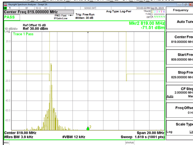
NB_IoT_Band26_Part90s_15kHz_QPSK_12_0_CH26692
