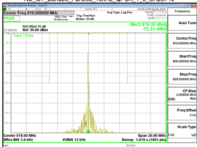
NB_IoT_Band26_Part90s_15kHz_QPSK_1_0_CH26740
