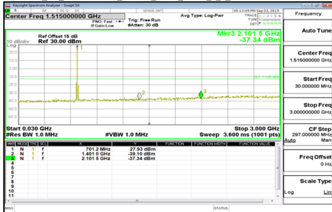
Cat_M1_30MHz~3GHz_Band12_3MHz_QPSK_1_0_LowCH23025-700.5
