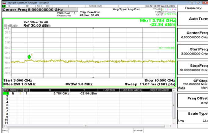
Cat_M1_3GHz~10GHz_Band13_5MHz_QPSK_1_0_LowCH23205-779.5
