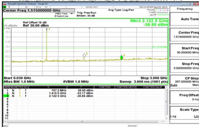
Cat_M1_30MHz~3GHz_Band12_3MHz_QPSK_1_0_MidCH23095-707.5
