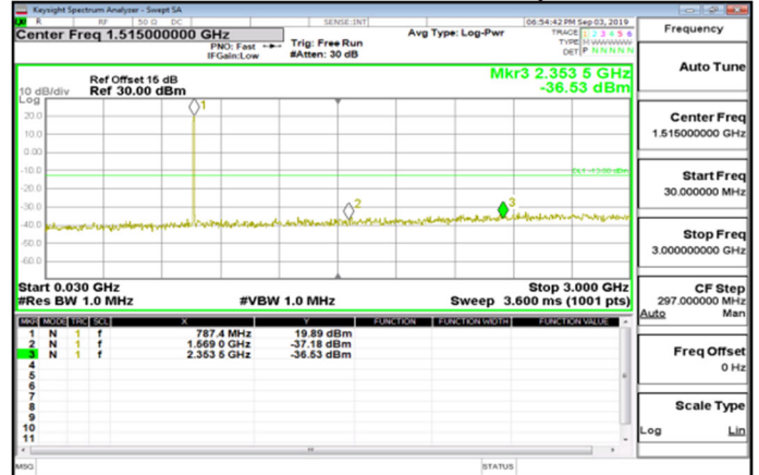
Cat_M1_30MHz~3GHz_Band13_5MHz_QPSK_1_0_HighCH23255-784.5
