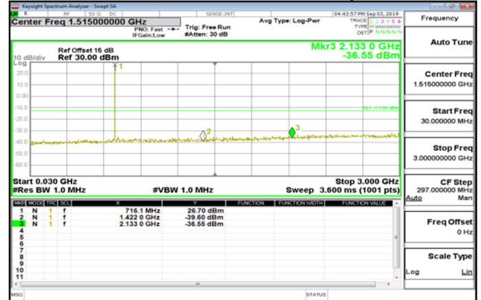
Cat M1_30MHz~3GHz_Band12_10MHz_QPSK_1_0_HighCH23130-711
