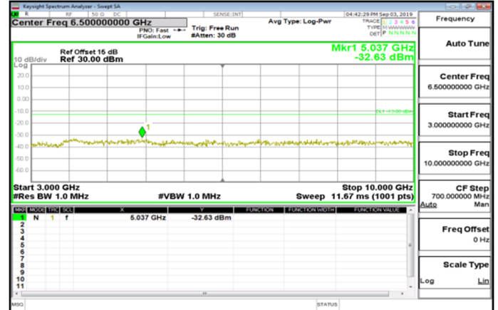
Cat M1_3GHz~10GHz_Band12_10MHz_QPSK_1_0_MidCH23095-707.5
