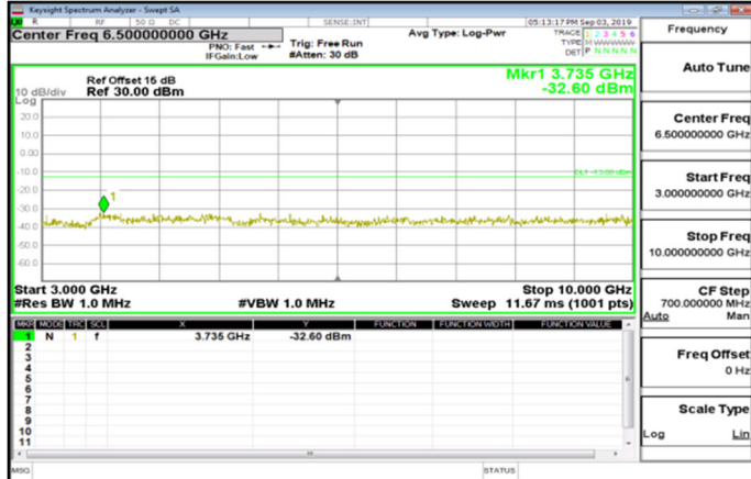
Cat_M1_3GHz~10GHz_Band12_3MHz_QPSK_1_0_LowCH23025-700.5
