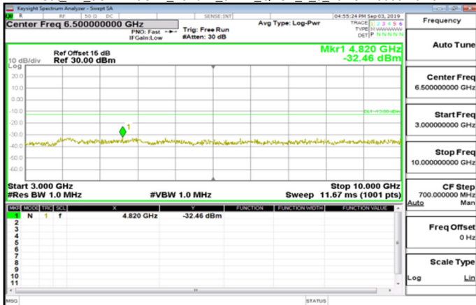
Cat_M1_3GHz~10GHz_Band12_5MHz_QPSK_1_0_LowCH23035-701.5
