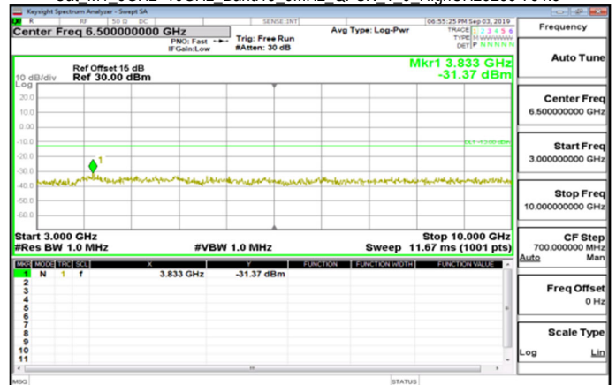
Cat_M1_3GHz~10GHz_Band13_5MHz_QPSK_1_0_HighCH23255-784.5
