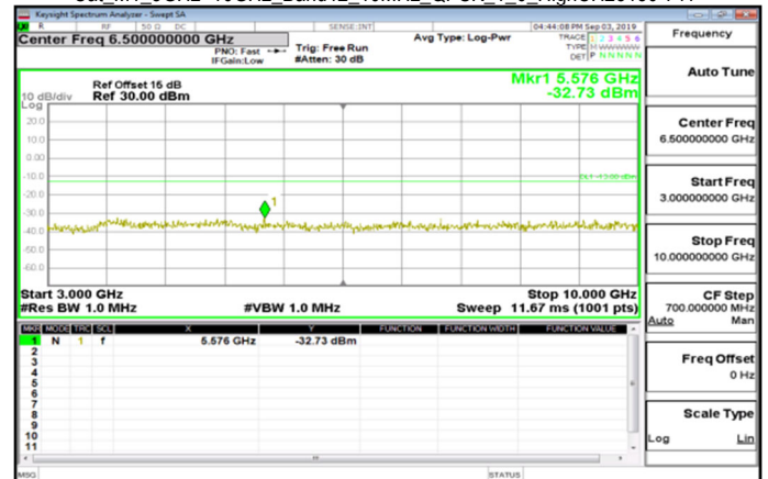
Cat M1_3GHz~10GHz_Band12_10MHz_QPSK_1_0_HighCH23130-711
