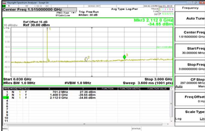
Cat M1_30MHz~3GHz_Band12_10MHz_QPSK_1_0_LowCH23060-704
