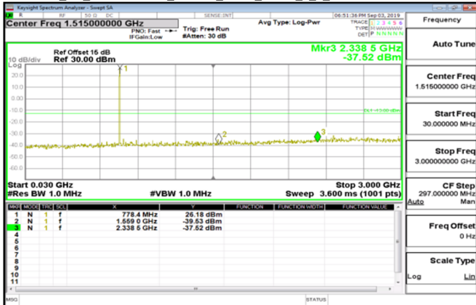
Cat_M1_30MHz~3GHz_Band13_5MHz_QPSK_1_0_LowCH23205-779.5
