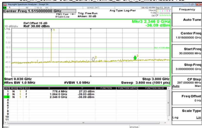
Cat_M1_30MHz~3GHz_Band13_10MHz_QPSK_1_0_MidCH23230-782
