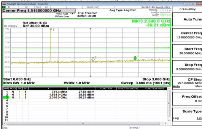
Cat_M1_30MHz~3GHz_Band13_5MHz_QPSK_1_0_MidCH23230-782
