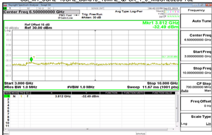
Cat_M1_3GHz~10GHz_Band13_10MHz_QPSK_1_0_MidCH23230-782
