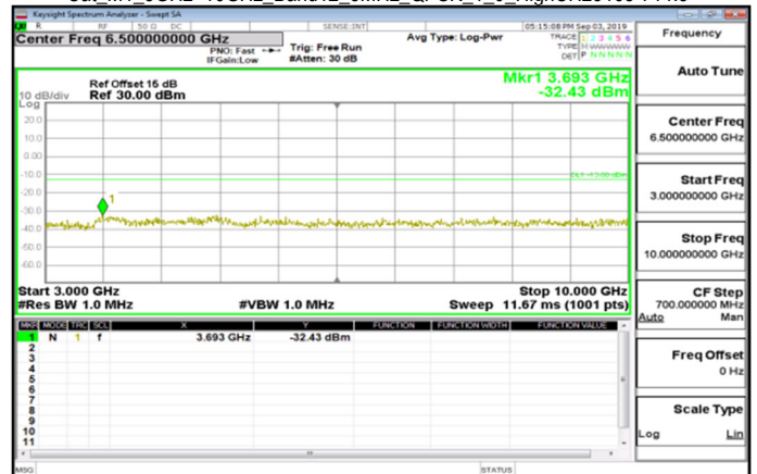
Cat_M1_3GHz~10GHz_Band12_3MHz_QPSK_1_0_HighCH23165-714.5
