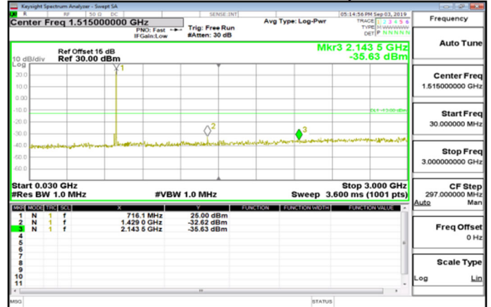
Cat_M1_30MHz~3GHz_Band12_3MHz_QPSK_1_0_HighCH23165-714.5
