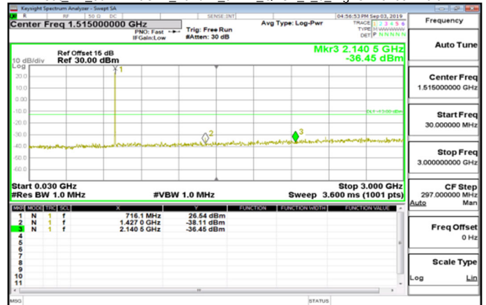
Cat_M1_30MHz~3GHz_Band12_5MHz_QPSK_1_0_HighCH23155-713.5
