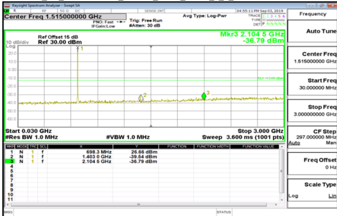
Cat_M1_30MHz~3GHz_Band12_5MHz_QPSK_1_0_LowCH23035-701.5
