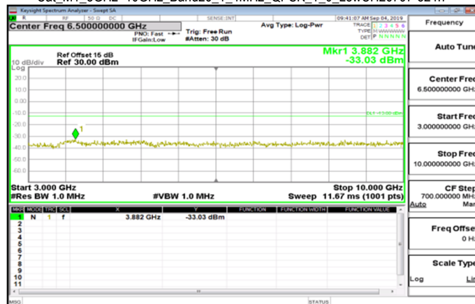
Cat_M1_3GHz~10GHz_Band26_1_4MHz_QPSK_1_0_LowCH26797-824.7
