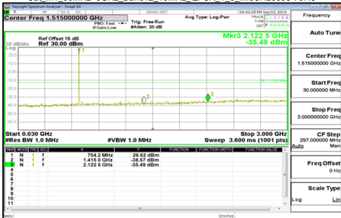
Cat M1_30MHz~3GHz_Band12_10MHz_QPSK_1_0_MidCH23095-707.5
