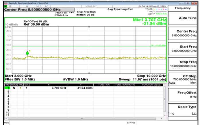
Cat_M1_3GHz~10GHz_Band12_5MHz_QPSK_1_0_MidCH23095-707.5
