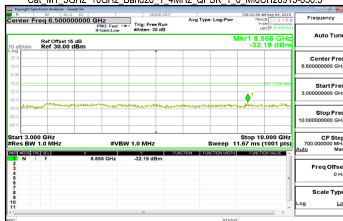
Cat_M1_3GHz~10GHz_Band26_1_4MHz_QPSK_1_0_MidCH26915-836.5
