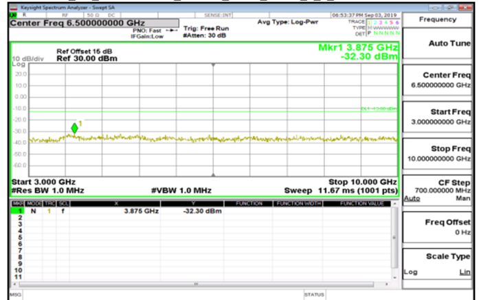
Cat_M1_3GHz~10GHz_Band13_5MHz_QPSK_1_0_MidCH23230-782
