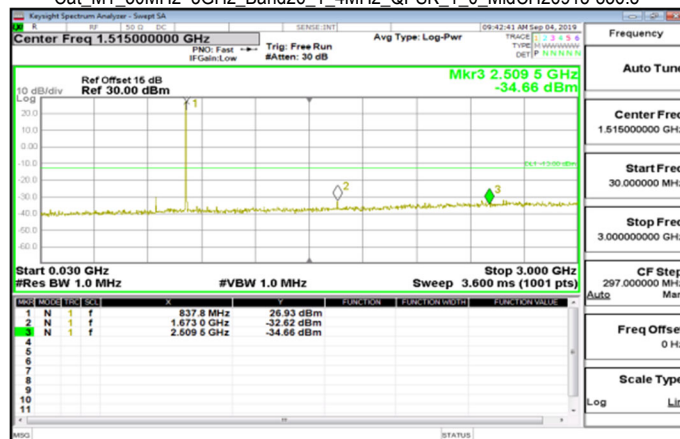
Cat_M1_30MHz~3GHz_Band26_1_4MHz_QPSK_1_0_MidCH26915-836.5
