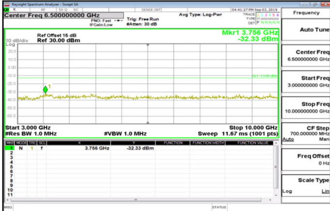
Cat M1_3GHz~10GHz_Band12_10MHz_QPSK_1_0_LowCH23060-704
