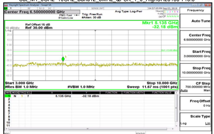
Cat_M1_3GHz~10GHz_Band12_5MHz_QPSK_1_0_HighCH23155-713.5
