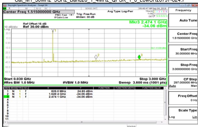
Cat_M1_30MHz~3GHz_Band26_1_4MHz_QPSK_1_0_LowCH26797-824.7
