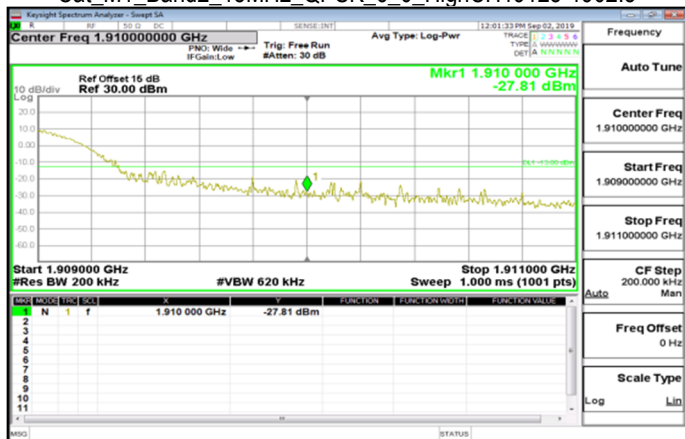
Cat_M1_Band2_15MHz_QPSK_6_0_HighCH19125-1902.5
