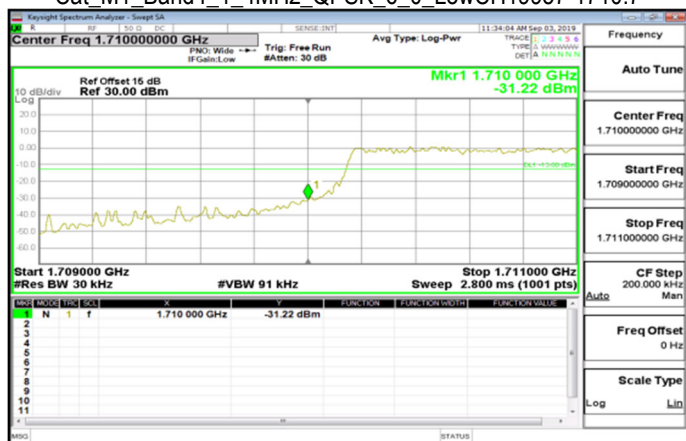
Cat_M1_Band4_1_4MHz_QPSK_6_0_LowCH19957-1710.7
