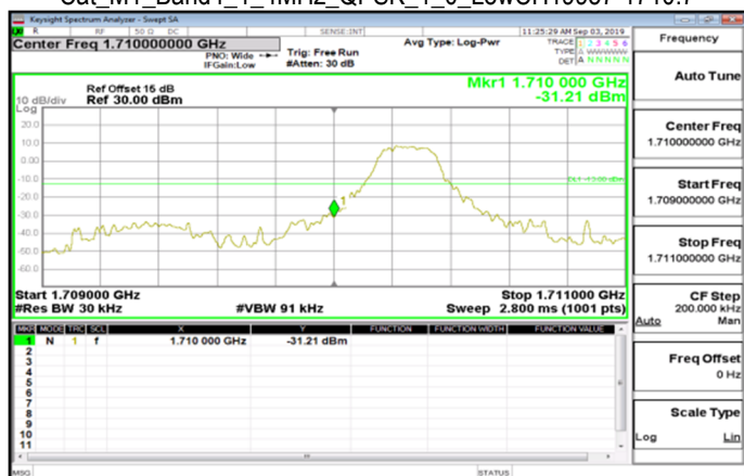
Cat_M1_Band4_1_4MHz_QPSK_1_0_LowCH19957-1710.7
