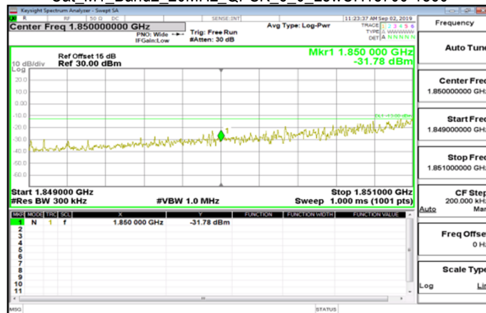
Cat_M1_Band2_20MHz_QPSK_6_0_LowCH18700-1860
