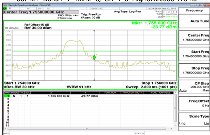
Cat_M1_Band4_1_4MHz_QPSK_1_5_HighCH20393-1754.3
