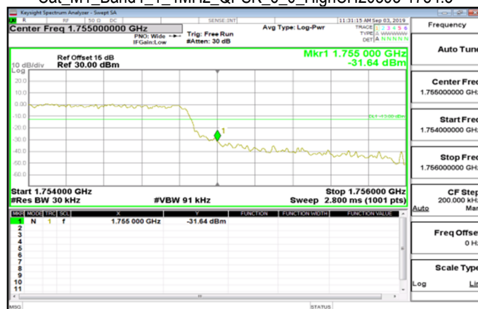
Cat_M1_Band4_1_4MHz_QPSK_6_0_HighCH20393-1754.3
