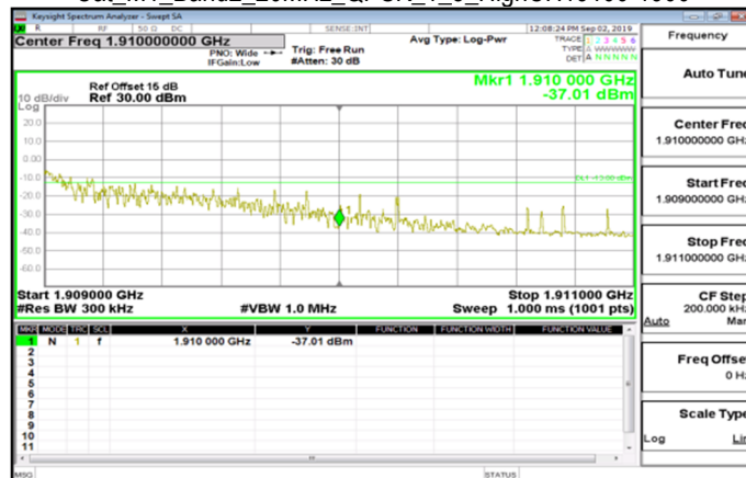
Cat_M1_Band2_20MHz_QPSK_1_5_HighCH19100-1900
