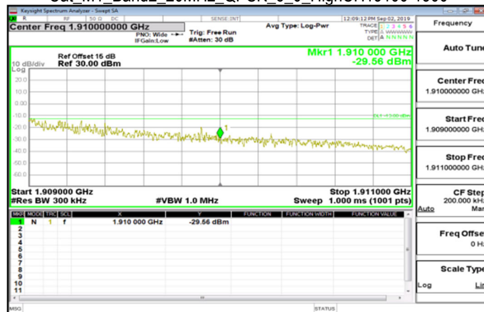
Cat_M1_Band2_20MHz_QPSK_6_0_HighCH19100-1900
