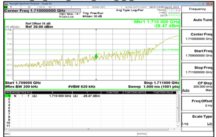
Cat_M1_Band4_15MHz_QPSK_1_0_LowCH20025-1717.5
