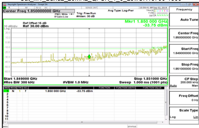
Cat_M1_Band2_20MHz_QPSK_1_0_LowCH18700-1860
