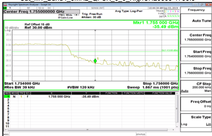
Cat_M1_Band4_3MHz_QPSK_6_0_HighCH20385-1753.5
