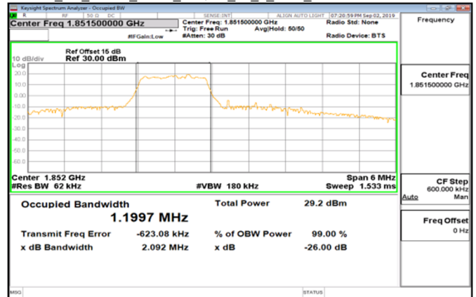
Cat_M1_Band2_3MHz_16QAM_15_0_Main_LowCH18615-1851.5
