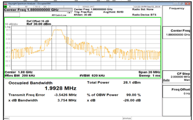
Cat_M1_Band2_10MHz_16QAM_50_0_Main_MidCH18900-1880
