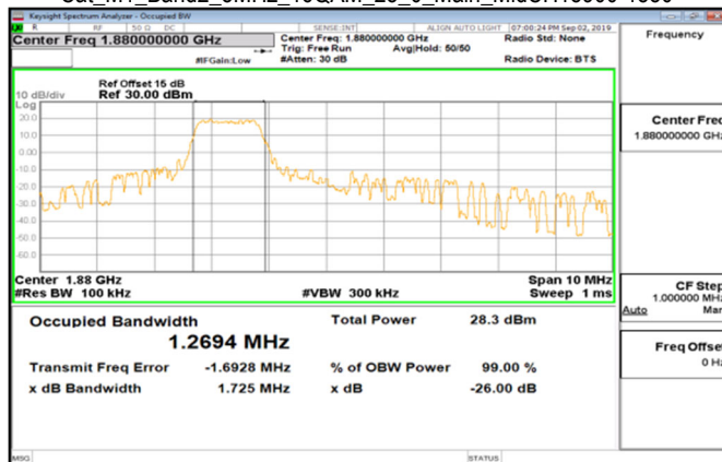
Cat_M1_Band2_5MHz_16QAM_25_0_Main_MidCH18900-1880
