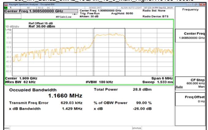
Cat_M1_Band2_3MHz_16QAM_15_0_Main_HighCH19185-1908.5
