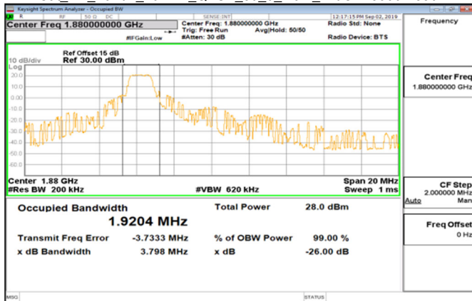
Cat_M1_Band2_10MHz_QPSK_50_0_Main_MidCH18900-1880
