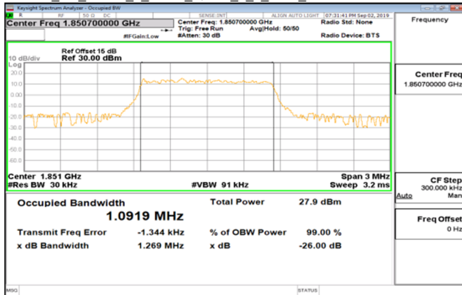
Cat M1_Band2_1_4MHz_QPSK_6_0_Main_LowCH18607-1850.7
