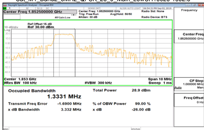
Cat_M1_Band2_5MHz_QPSK_25_0_Main_LowCH18625-1852.5
