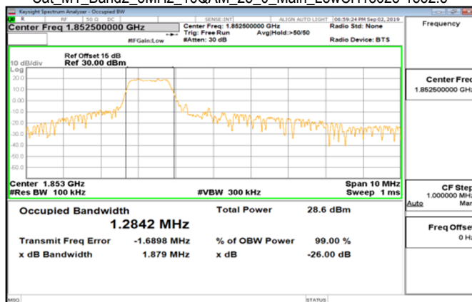
Cat_M1_Band2_5MHz_16QAM_25_0_Main_LowCH18625-1852.5
