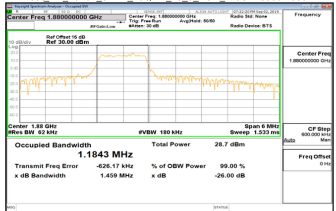
Cat_M1_Band2_3MHz_16QAM_15_0_Main_MidCH18900-1880
