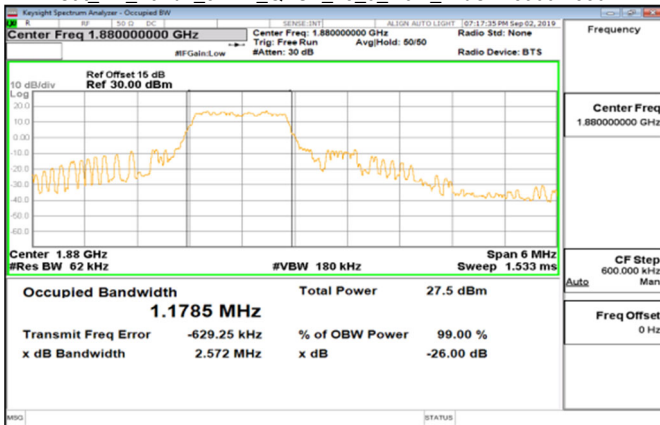
Cat_M1_Band2_3MHz_QPSK_15_0_Main_MidCH18900-1880
