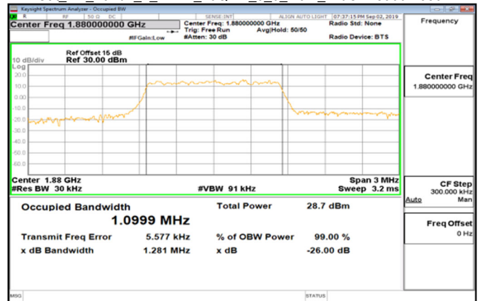
Cat M1_Band2_1_4MHz_16QAM_6_0_Main_MidCH18900-1880
