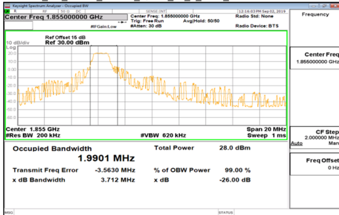
Cat_M1_Band2_10MHz_QPSK_50_0_Main_LowCH18650-1855
