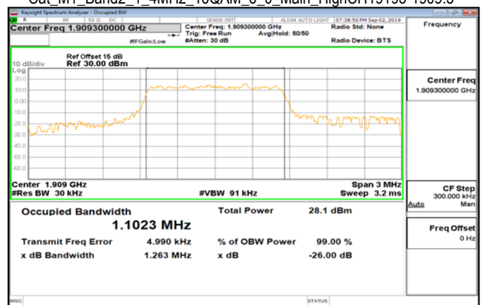
Cat M1_Band2_1_4MHz_16QAM_6_0_Main_HighCH19193-1909.3
