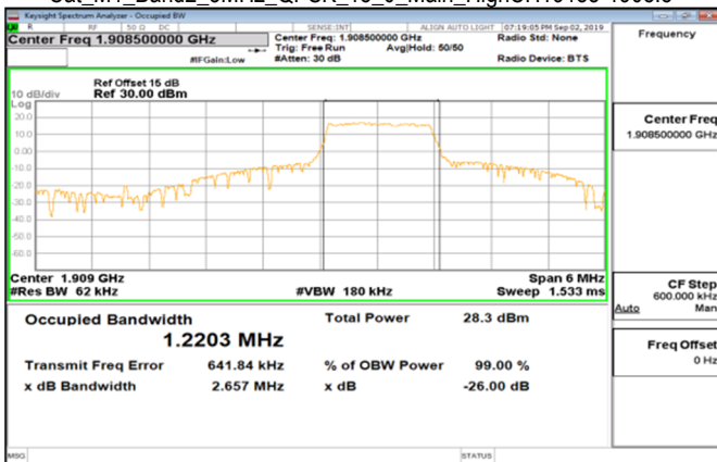
Cat_M1_Band2_3MHz_QPSK_15_0_Main_HighCH19185-1908.5
