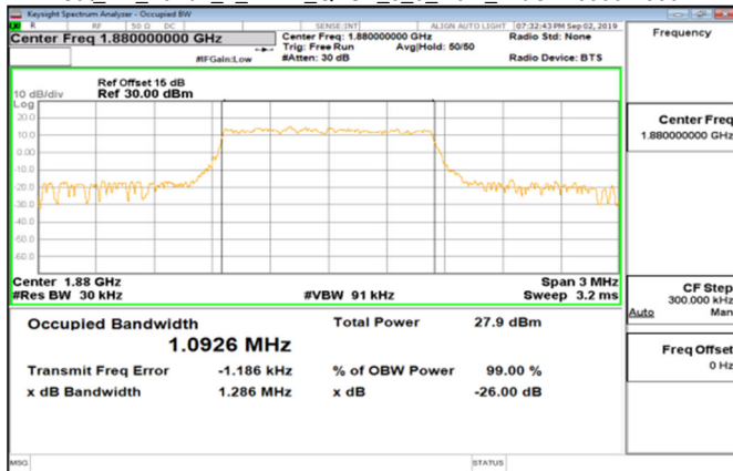
Cat M1_Band2_1_4MHz_QPSK_6_0_Main_MidCH18900-1880
