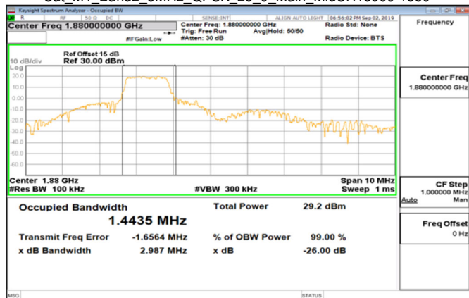
Cat_M1_Band2_5MHz_QPSK_25_0_Main_MidCH18900-1880
