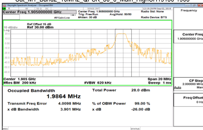
Cat_M1_Band2_10MHz_QPSK_50_0_Main_HighCH19150-1905
