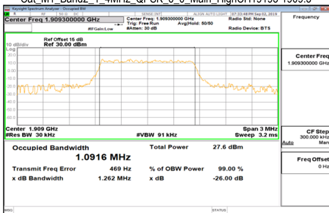
Cat M1_Band2_1_4MHz_QPSK_6_0_Main_HighCH19193-1909.3
