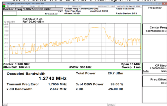
Cat_M1_Band2_5MHz_QPSK_25_0_Main_HighCH19175-1907.5
