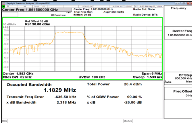
Cat_M1_Band2_3MHz_QPSK_15_0_Main_LowCH18615-1851.5
