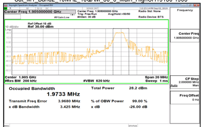
Cat_M1_Band2_10MHz_16QAM_50_0_Main_HighCH19150-1905
