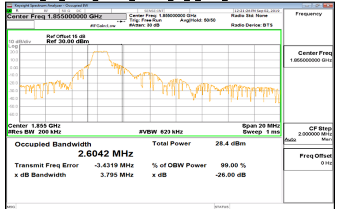
Cat_M1_Band2_10MHz_16QAM_50_0_Main_LowCH18650-1855
