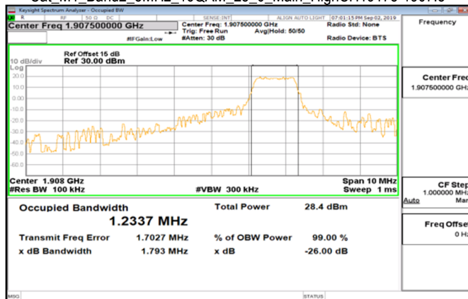
Cat_M1_Band2_5MHz_16QAM_25_0_Main_HighCH19175-1907.5
