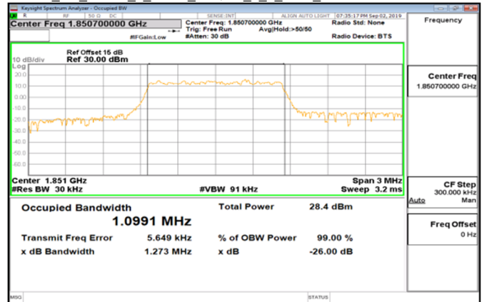
Cat M1_Band2_1_4MHz_16QAM_6_0_Main_LowCH18607-1850.7
