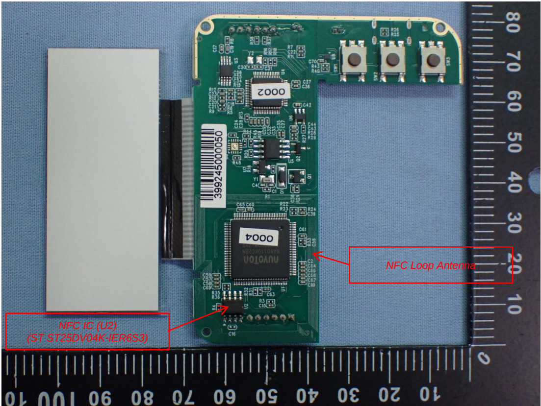
Figure 14 PCB (Back View)
