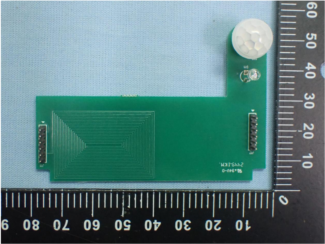
Figure 15 PCB (Front View)
