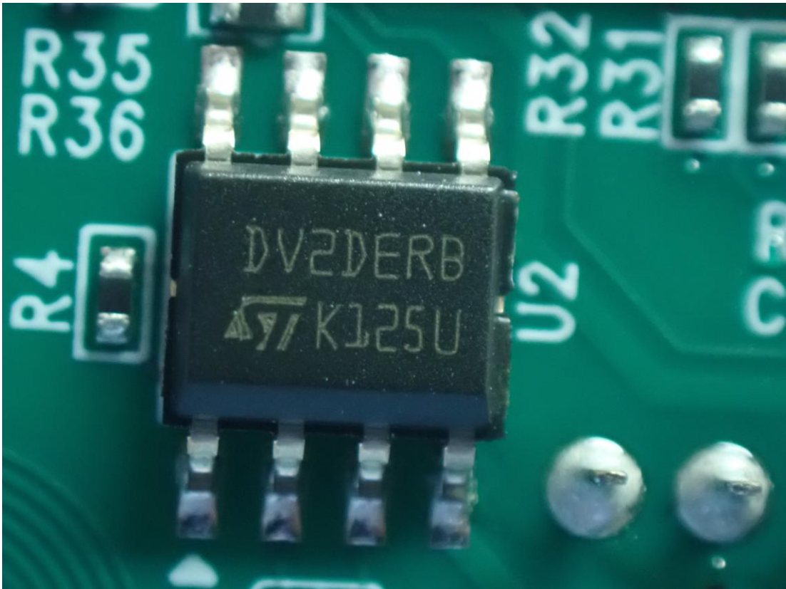
Figure 18 NFC IC (U2)(ST ST25DV04K-IER6S3) View
