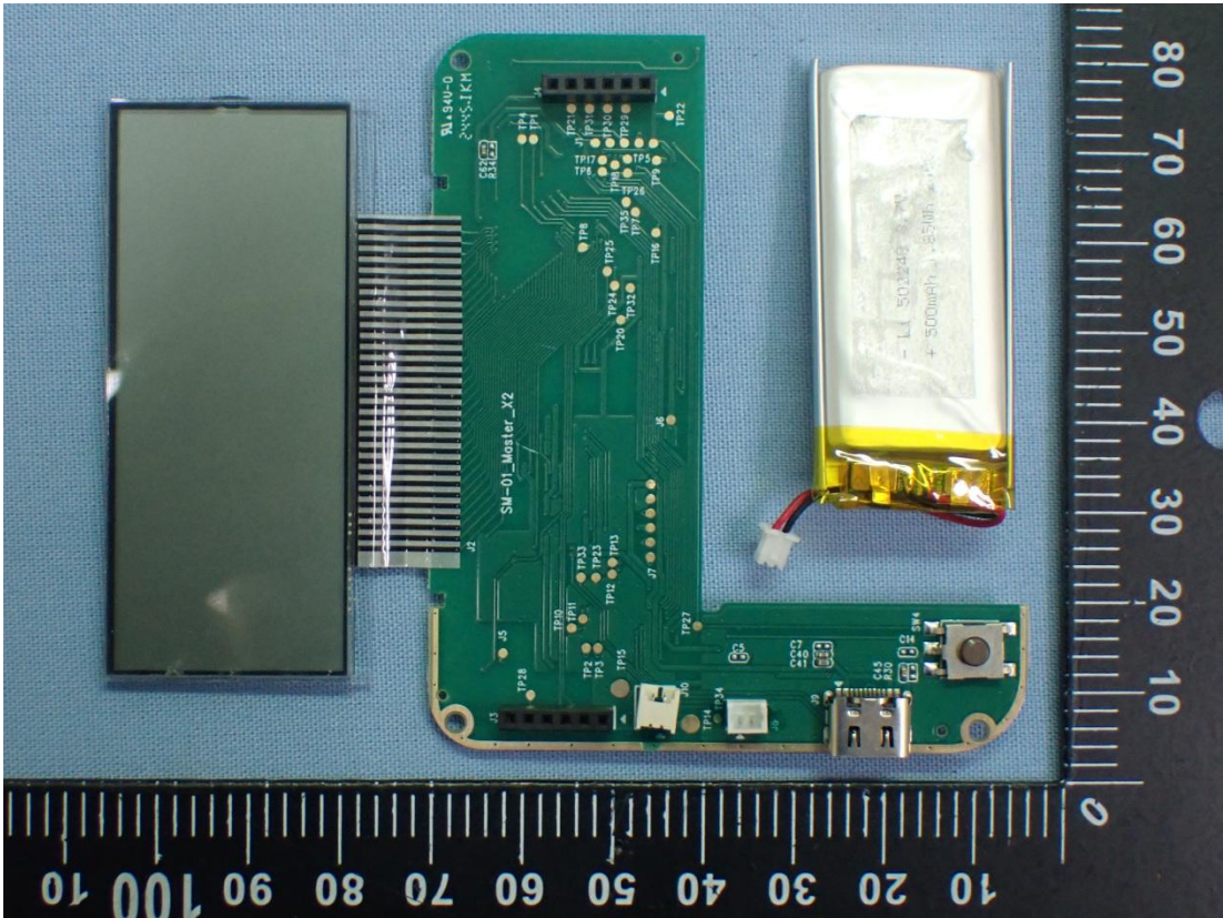
Figure 10 Internal View
