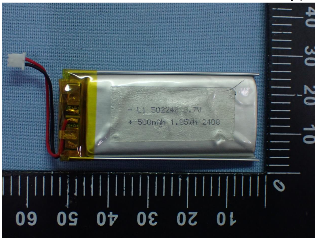
Figure 11 Battery (Front View)
