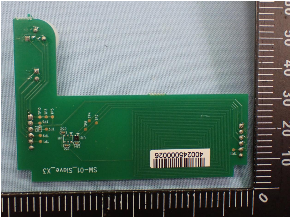
Figure 16 PCB (Back View)
