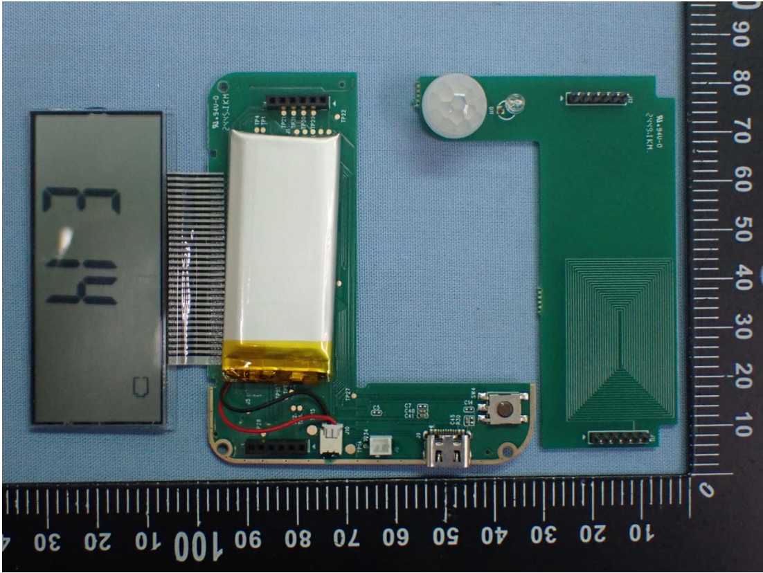
Figure 9 Internal View
