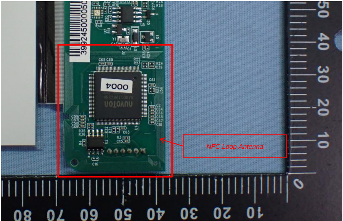
Figure 17 NFC Loop Antenna View
