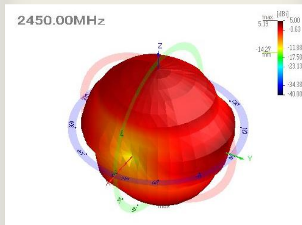
[3D Radiation Pattern]
