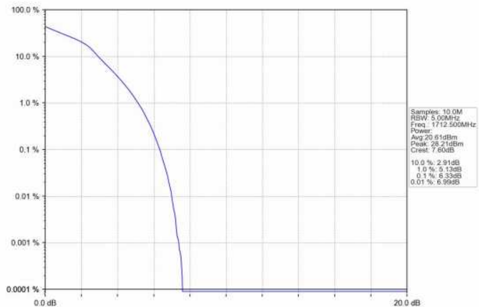
Band4_5MHz_16QAM_LCH_1712.5MHz_RB_25_0_NTNV
