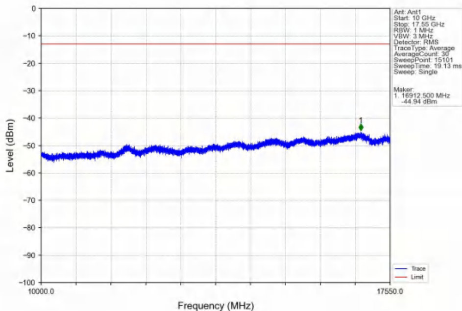
Band4_1.4MHz_QPSK_LCH_1710.7MHz_RB_1_0_NTNV
