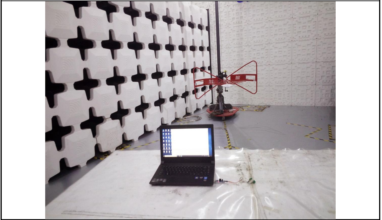
Radiated emission Test Setup (30 MHz~1 GHz)
