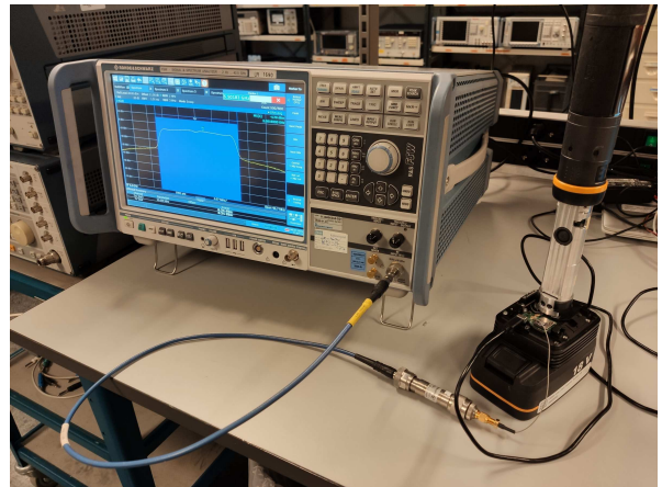
Conducted Test
