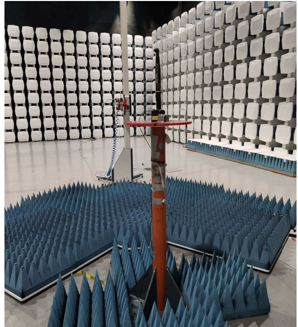
Radiated Emissions 1 – 18 GHz
