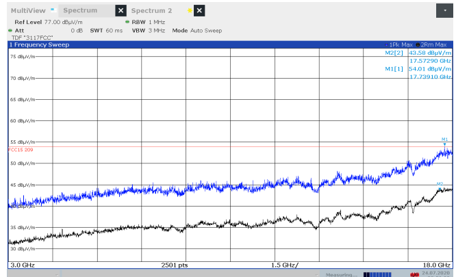
Radiated Emissions 3-18 GHz, 2437 MHz, 802.11b, 6Mb, Ant 1, VP
