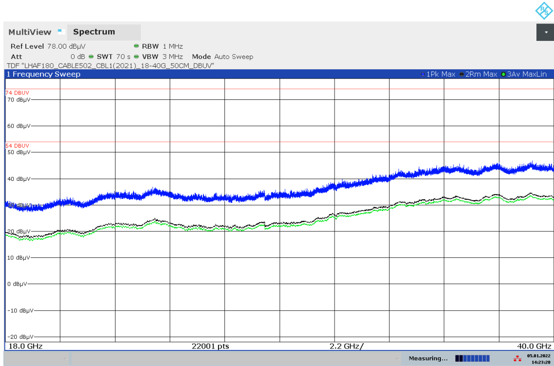
Plot 6: 18 GHz – 40 GHz, horizontal / vertical polarization
