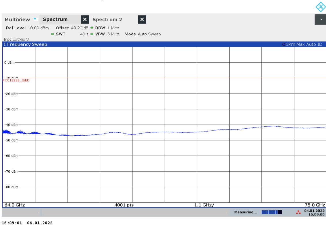
Plot 9: Out of Band 64 GHz – 75 GHz, antenna vertical / horizontal.
