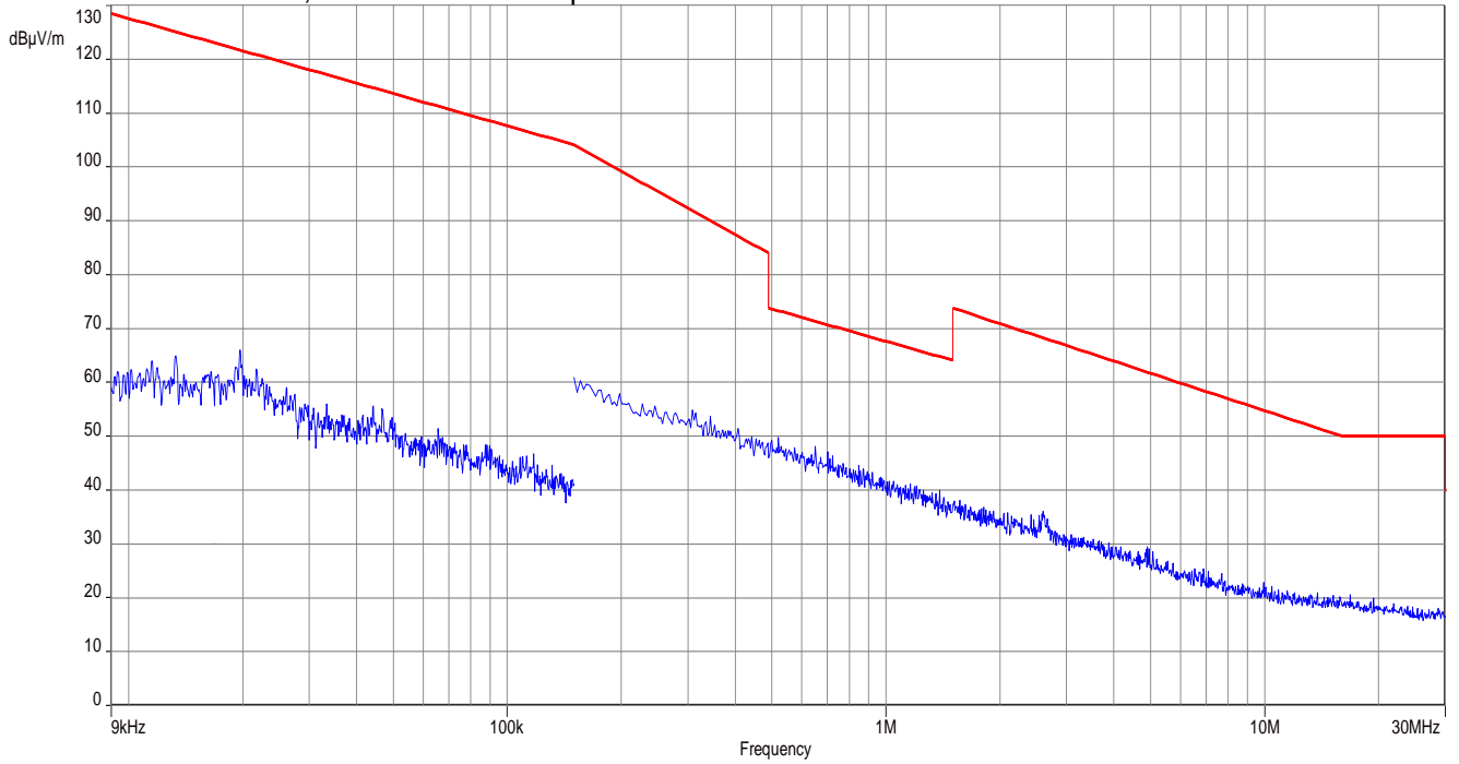
Plot 3: 9 kHz – 30 MHz, horizontal / vertical polarization
