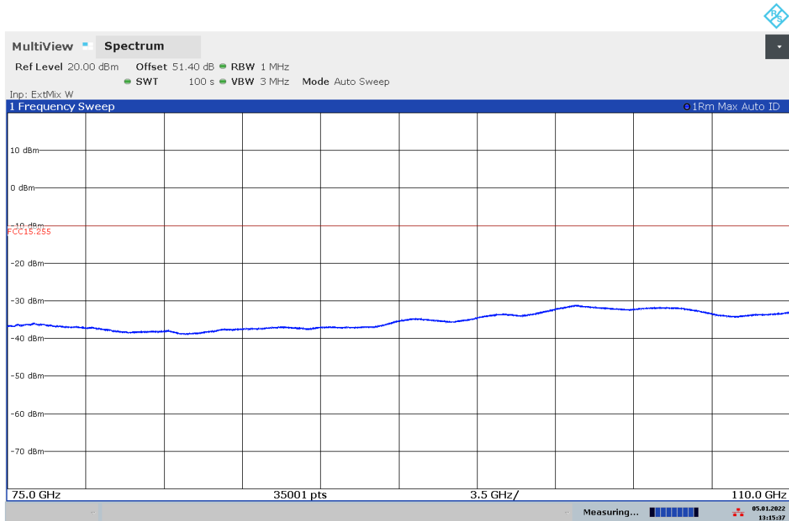
Plot 10: 75 GHz – 110 GHz, antenna vertical / horizontal
