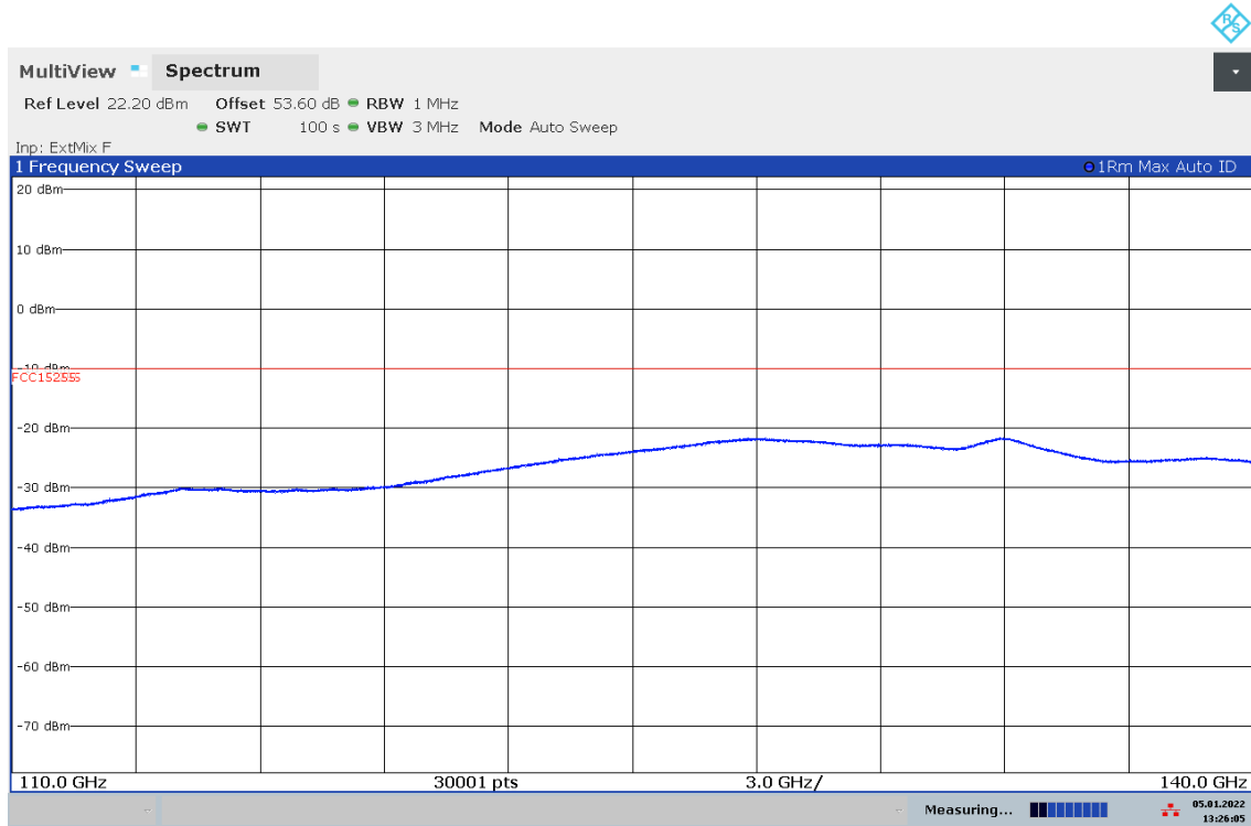
Plot 11: 110 GHz – 140 GHz, antenna vertical / horizontal
