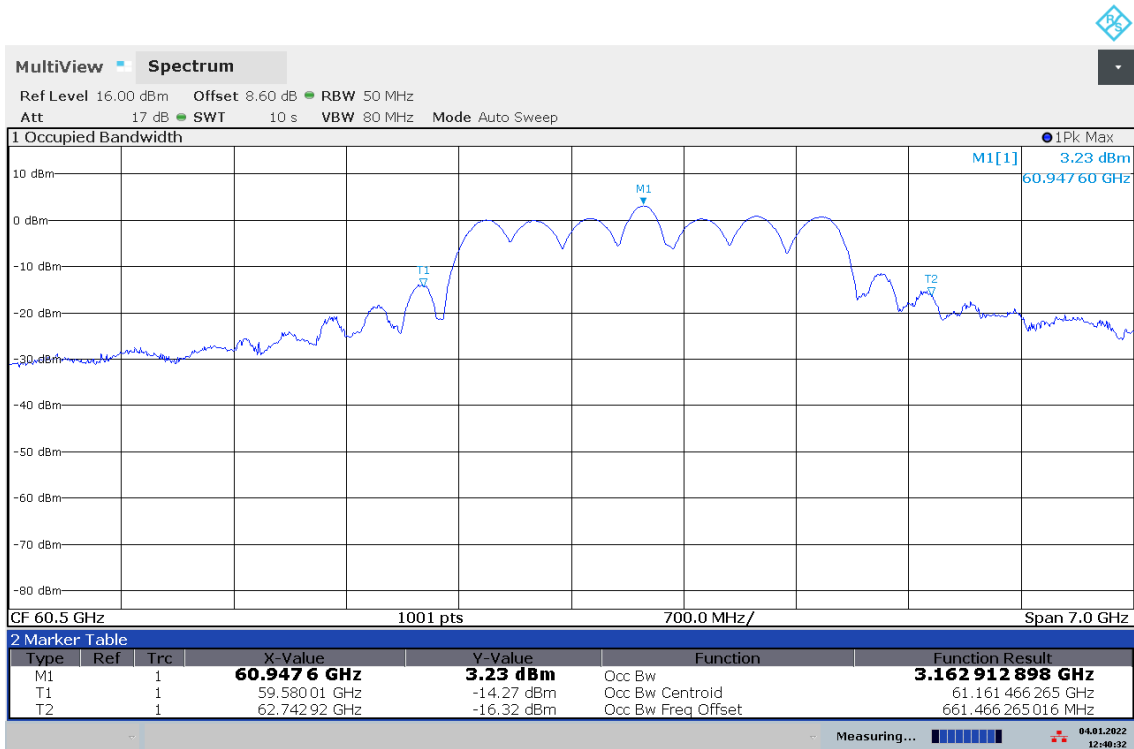
Plot 1: 99% OBW
