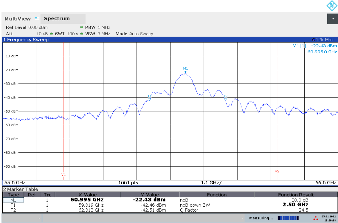
Plot 15: 20 dB-Bandwidth at V_{min}
