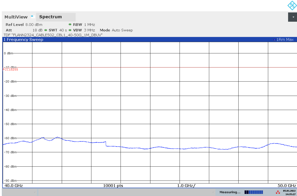
Plot 7: 40 GHz – 50 GHz, antenna vertical / horizontal
