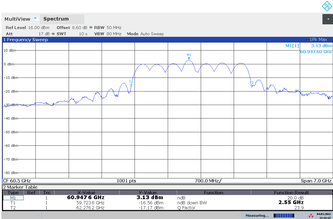
Plot 2: 20 dB OBW
