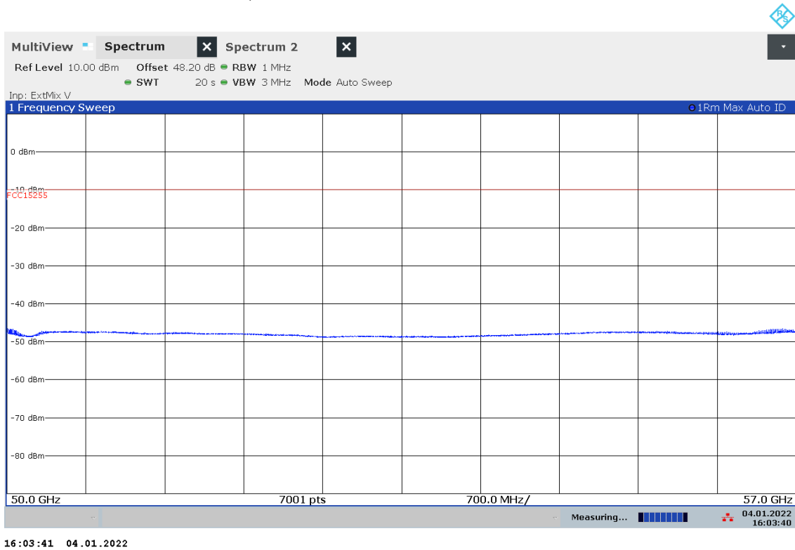
Plot 8: Out of Band 50 GHz – 57 GHz, antenna vertical / horizontal.
