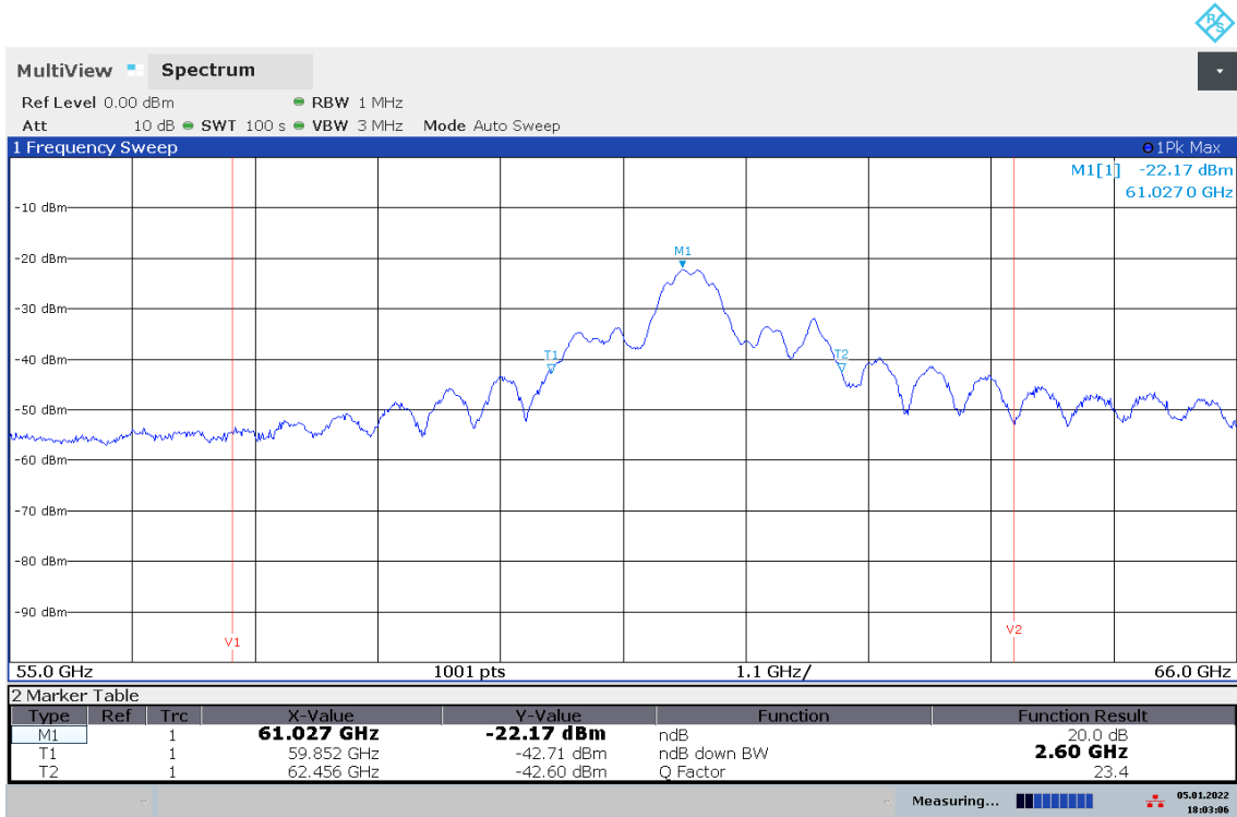
Plot 13: 20 dB-Bandwidth at T_{min}
