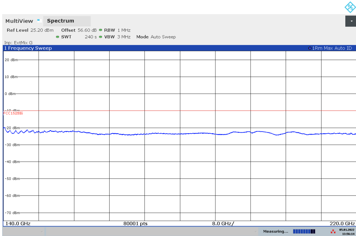
Plot 12: 140 GHz – 220 GHz, antenna vertical / horizontal
