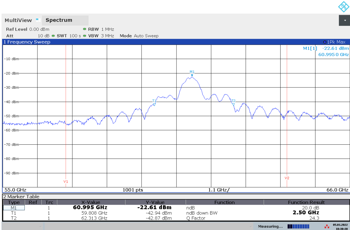
Plot 16: 20 dB Bandwidth at V_{max}
