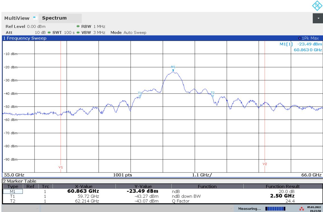
Plot 14: 20 dB Bandwidth at T_{max}
