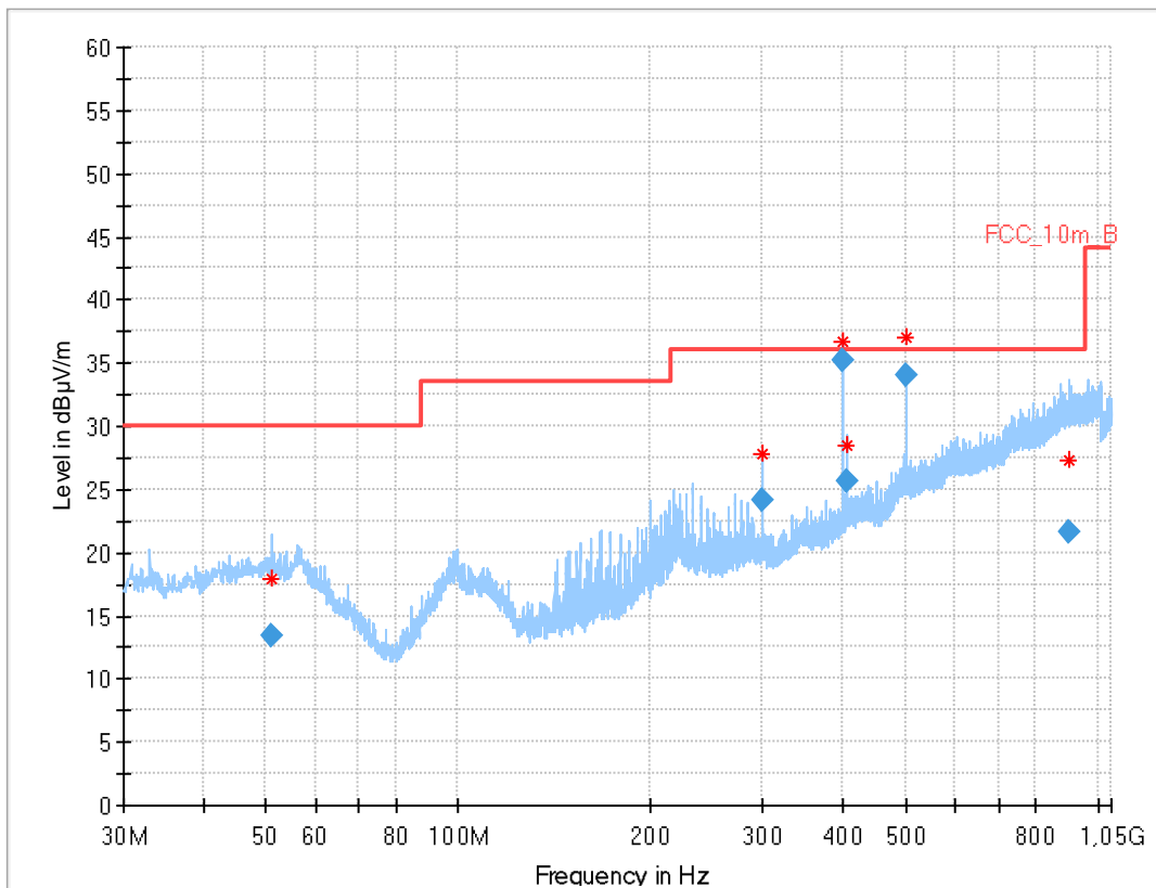
Plot 4: 30 MHz – 1 GHz, horizontal / vertical polarization
