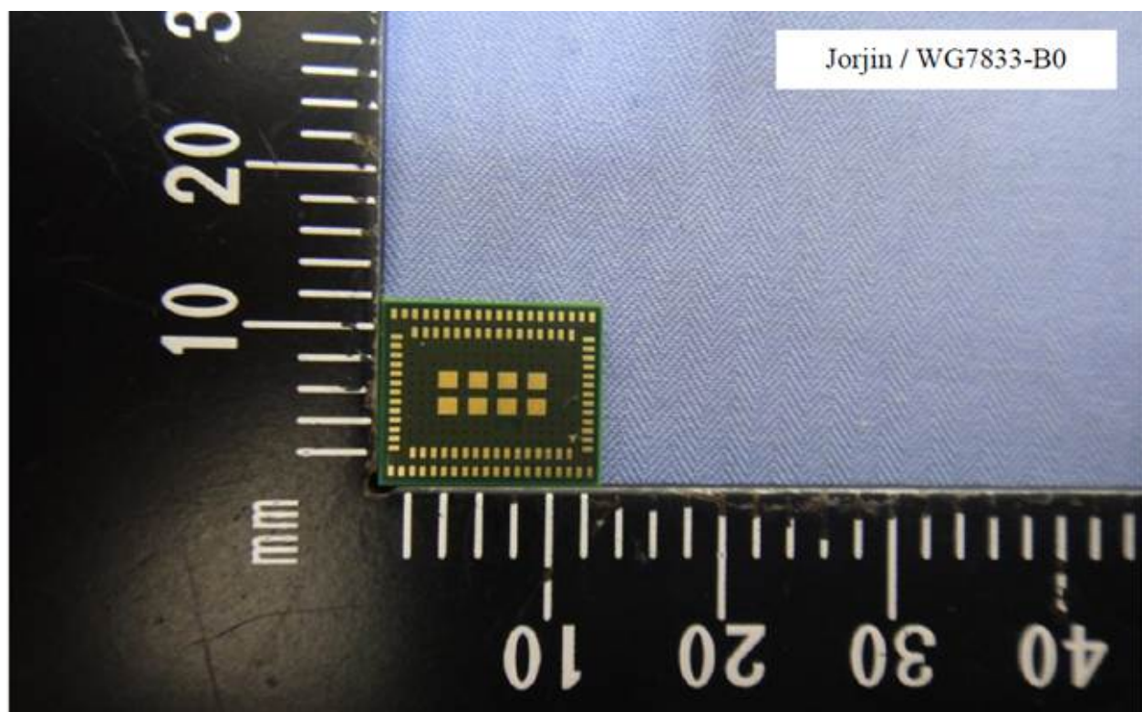
Figure 2: Bottom View
