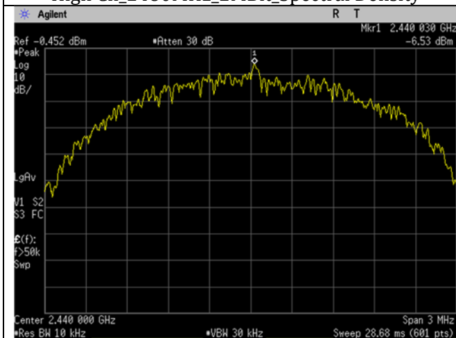
Mid Ch_2440MHz_2MBit_Spectral Density
