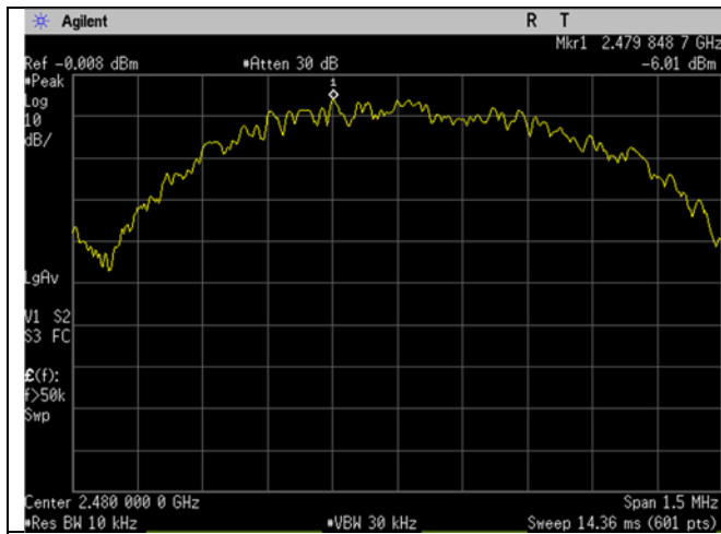
High Ch_2480MHz_1MBit_Spectral Density
