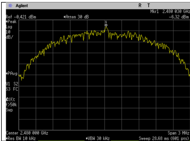
High Ch_2480MHz_2MBit_Spectral Density
