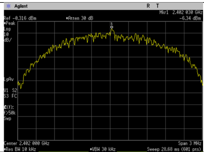
Low Ch_2402MHz_2MBit_Spectral Density
