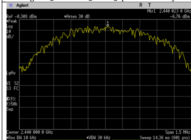
Mid Ch_2440MHz_1MBit_Spectral Density
