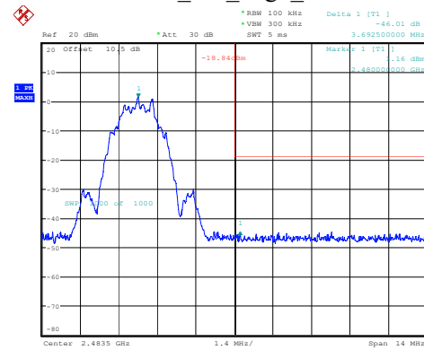
BLE_2M_High_Channel
