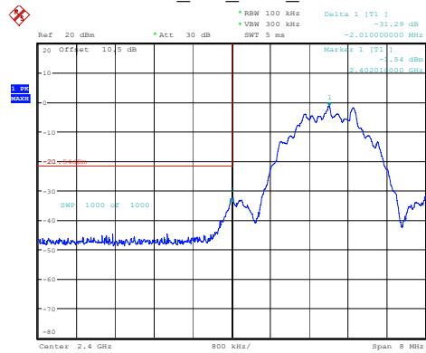
BLE_2M_Low_Channel
