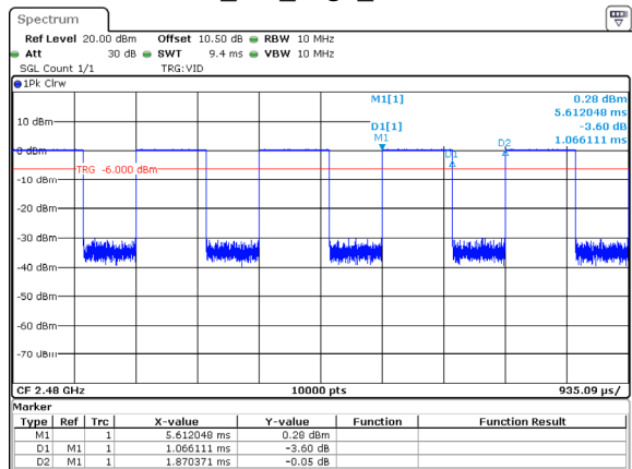
BLE_2M_High_Channel
