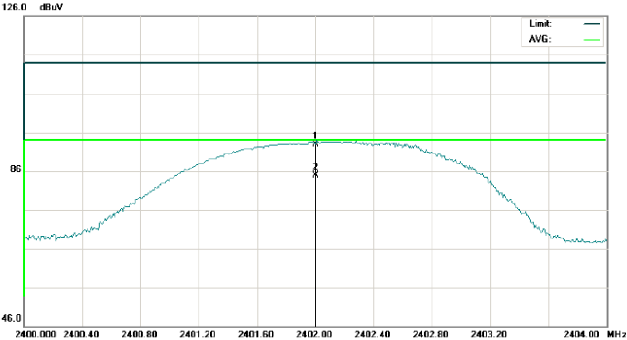
RADIATED EMISSION TEST- (ABOVE 1GHz)-LOW CHANNEL-HORIZONTAL
