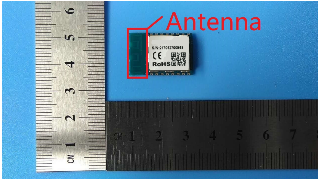
(1) EUT Photo
