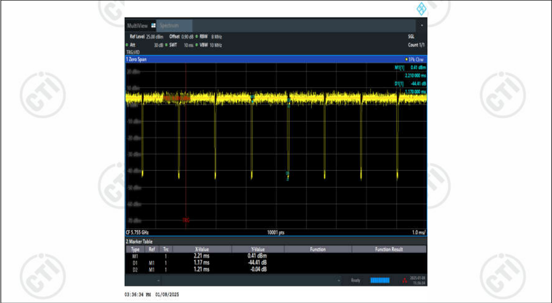
NTNV-11AX40ISO-Ant2-5755
