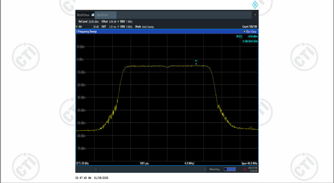
11AX20SISO-Ant2-5180-PASS
