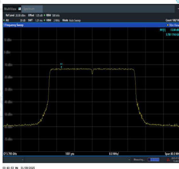
11AX40SISO-Ant2-5795-PASS
