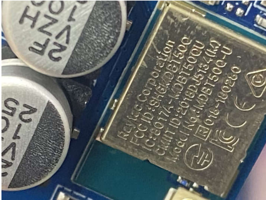
View of Product-49 (note:certified module's FCC ID:SH6MDBT500)
