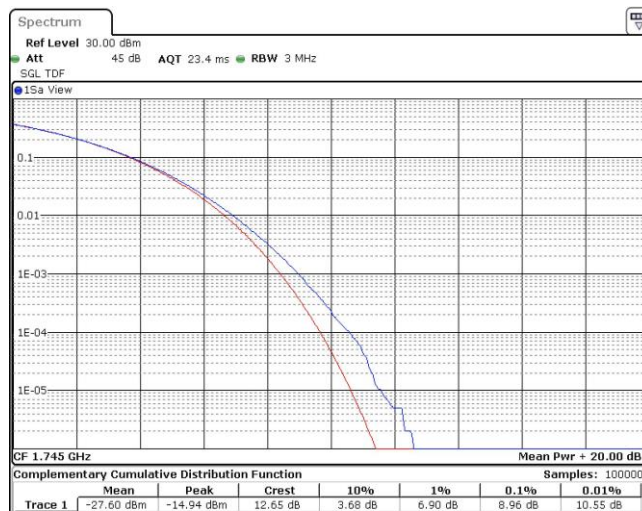
Band66-15MHz-QPSK-132322-75RB#0
