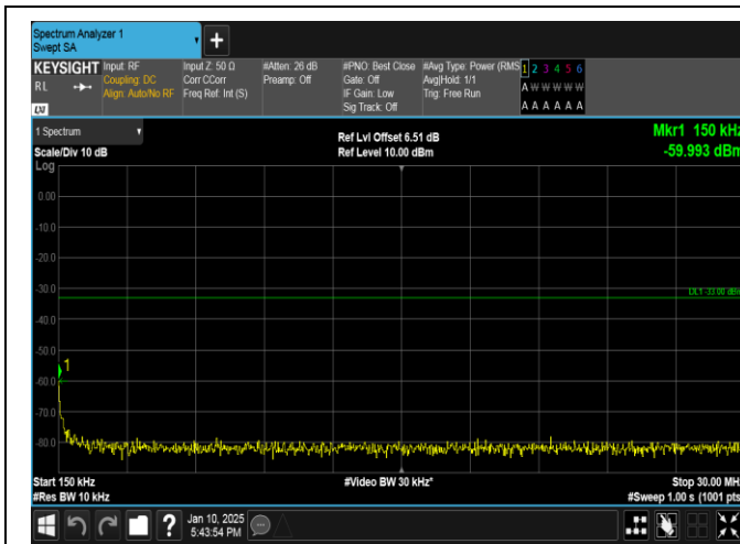
Band66-20MHz-16QAM-132322-1RB#99-0.15~30-PASS
