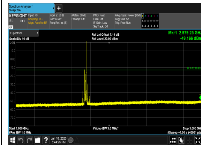
Band66-20MHz-16QAM-132322-1RB#99-1000~3000-PASS
