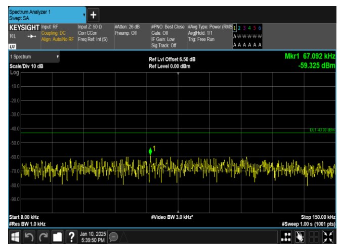
Band66-20MHz-QPSK-132322-1RB#0-0.009~0.15-PASS
