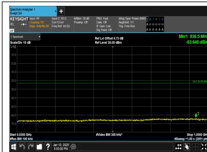
Band66-20MHz-QPSK-132572-100RB#0-30~1000-PASS
