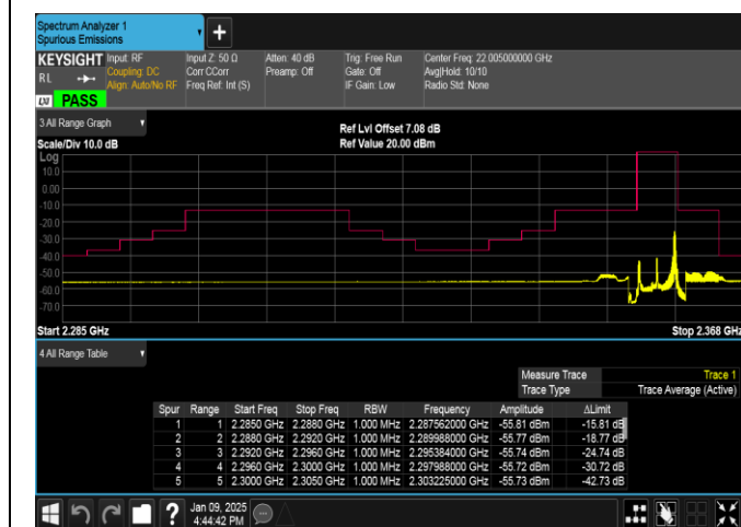
Band40(2350-2360)-5MHz-QPSK-39225-1RB#24-PASS
