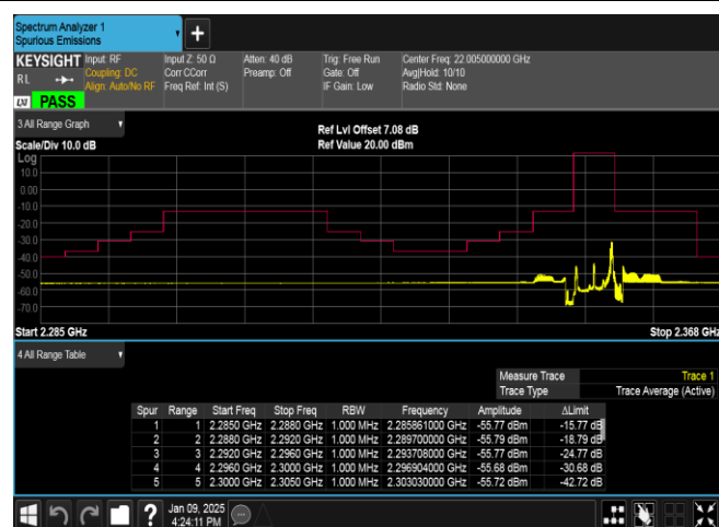
Band40(2350-2360)-5MHz-16QAM-39175-1RB#24-PASS
