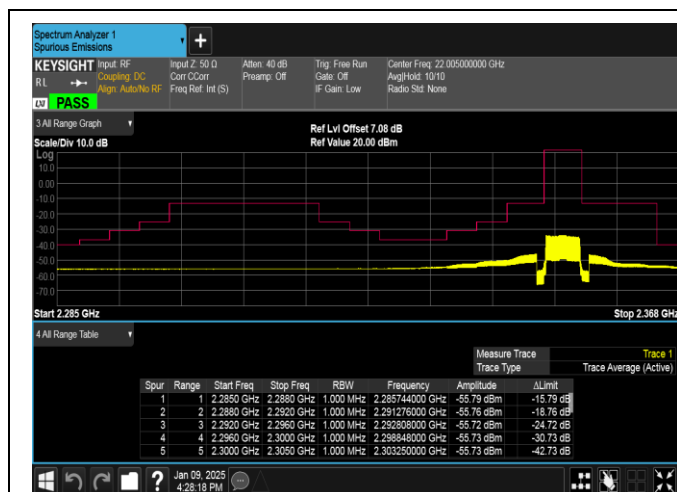
Band40(2350-2360)-5MHz-QPSK-39175-25RB#0-PASS
