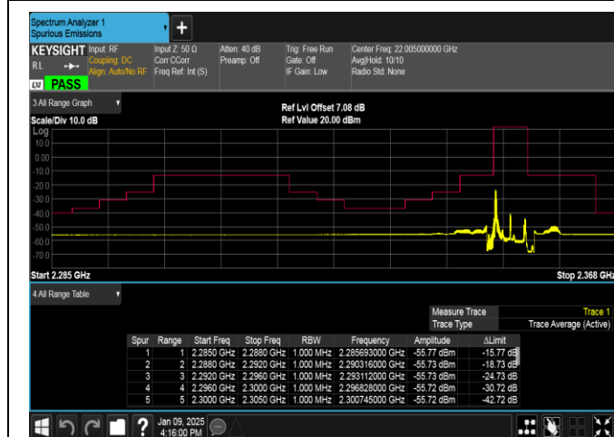
Band40(2350-2360)-5MHz-16QAM-39175-1RB#0-PASS
