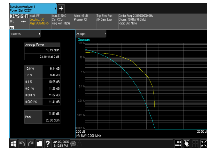
Band40(2350-2360)-10MHz-16QAM-39200-1RB#0-PASS
