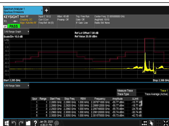
Band40(2350-2360)-5MHz-QPSK-39225-1RB#0-PASS
