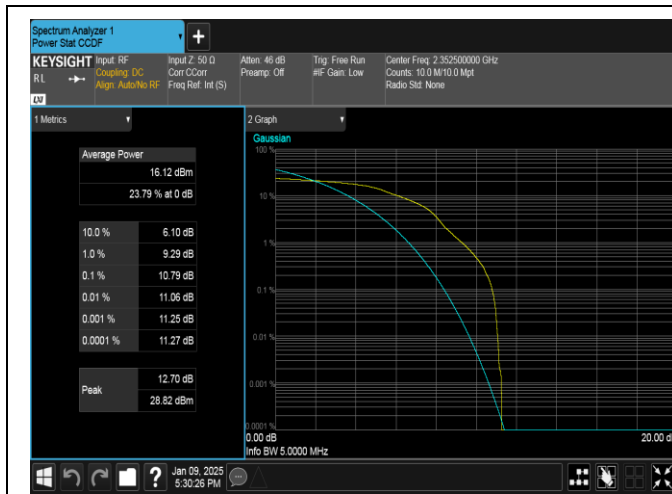
Band40(2350-2360)-5MHz-16QAM-39175-1RB#0-PASS
