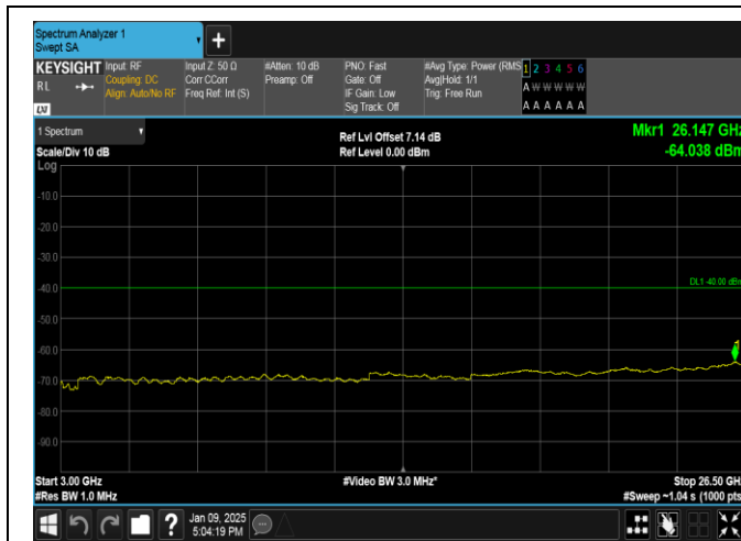
Band40(2350-2360)-5MHz-QPSK-39200-1RB#24-3000~26500-PASS
