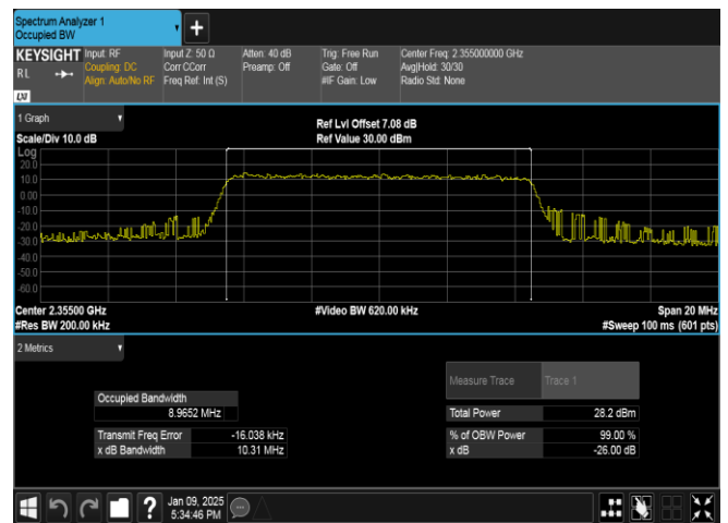
Band40(2350-2360)-10MHz-16QAM-39200-50RB#0-PASS
