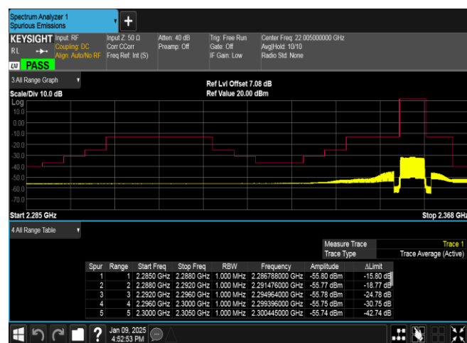
Band40(2350-2360)-5MHz-QPSK-39225-25RB#0-PASS
