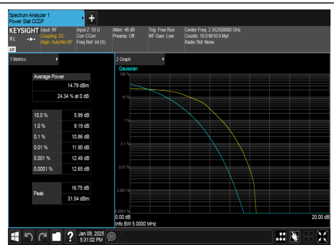
Band40(2350-2360)-5MHz-16QAM-39175-25RB#0-PASS
