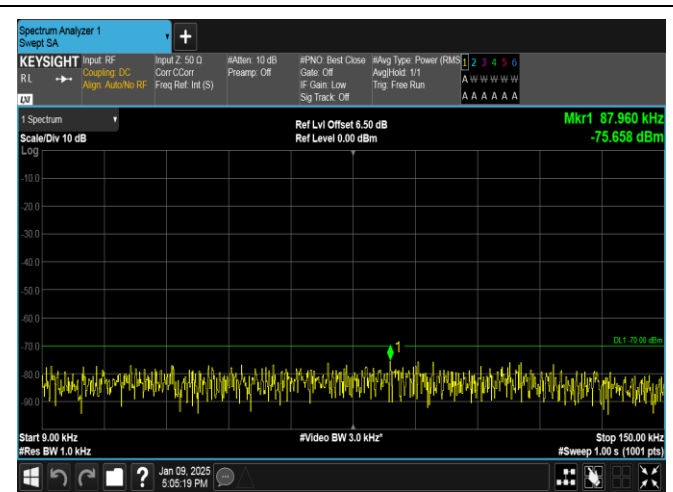
Band40(2350-2360)-5MHz-QPSK-39200-25RB#0-0.009~0.15-PASS
