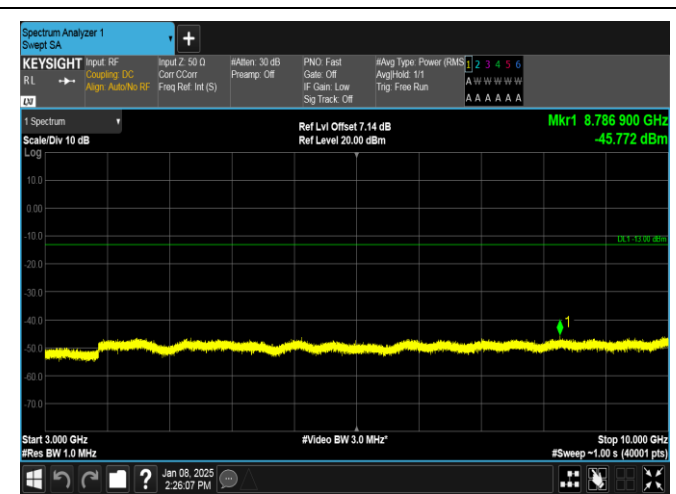
Band26(824-849)-1.4MHz-16QAM-27033-1RB#0-3000~10000-PASS
