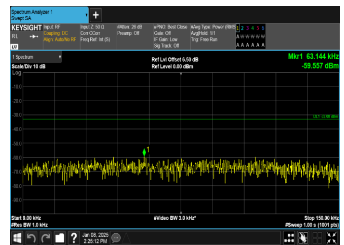
Band26(824-849)-1.4MHz-16QAM-27033-1RB#0-0.009~0.15-PASS
