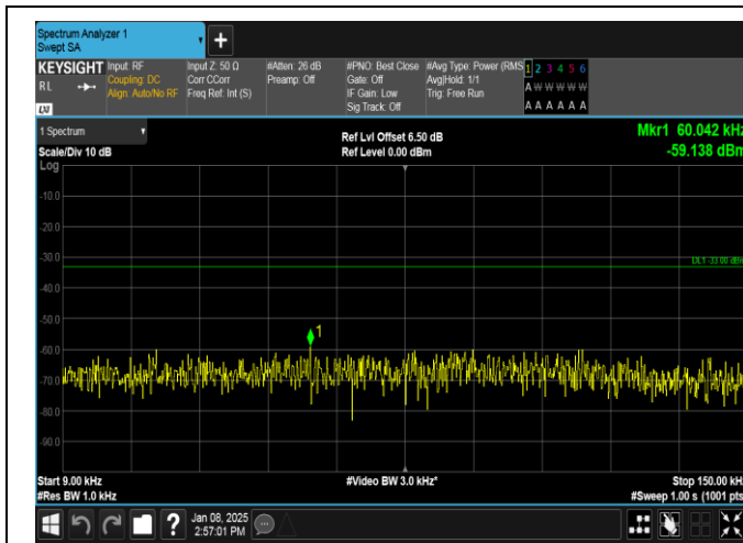
Band26(824-849)-3MHz-16QAM-26915-1RB#0-0.009~0.15-PASS
