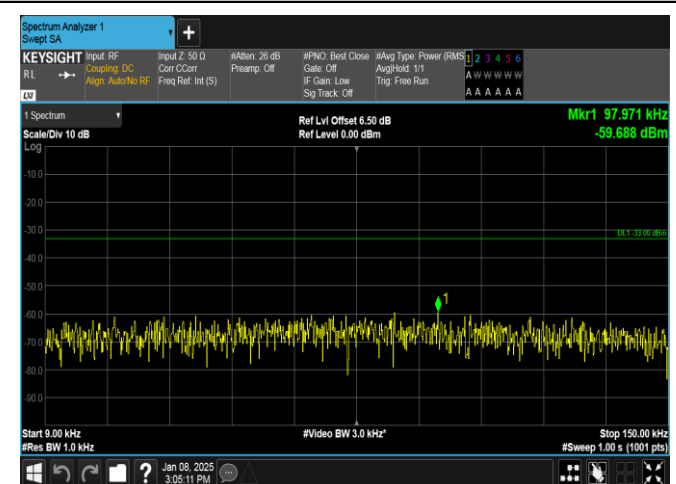
Band26(824-849)-3MHz-QPSK-27025-1RB#14-0.009~0.15-PASS
