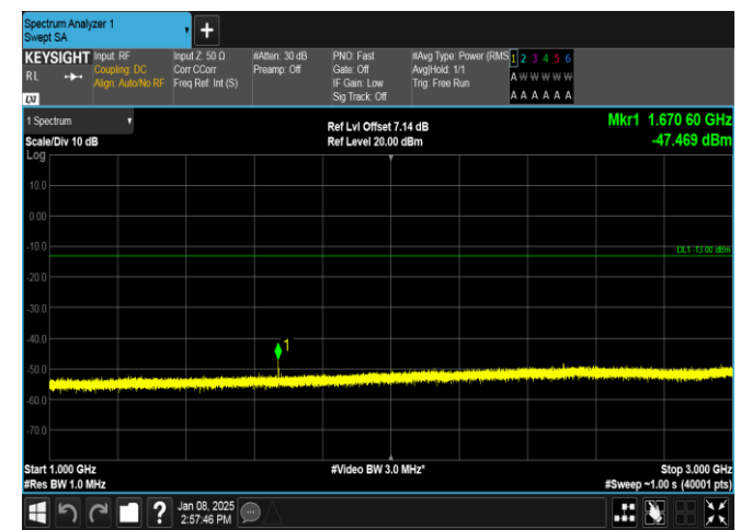
Band26(824-849)-3MHz-16QAM-26915-1RB#0-1000~3000-PASS
