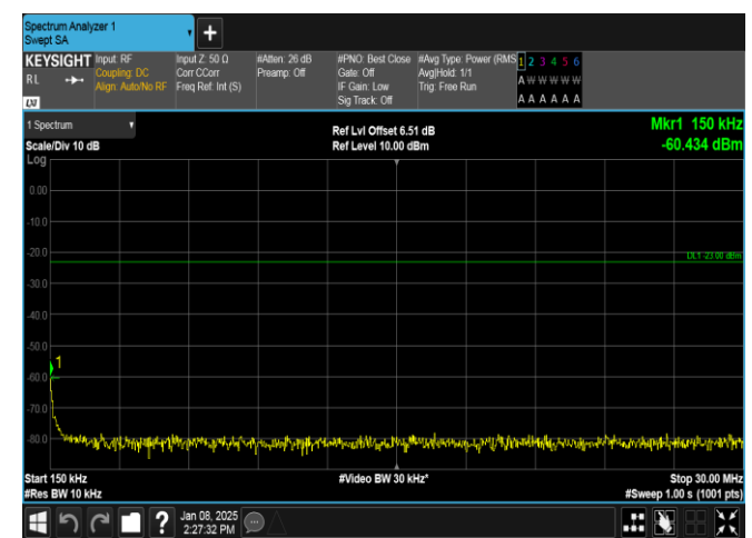
Band26(824-849)-1.4MHz-16QAM-27033-1RB#5-0.15~30-PASS
