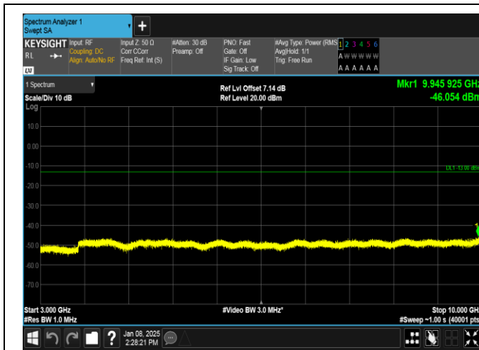
Band26(824-849)-1.4MHz-16QAM-27033-1RB#5-3000~10000-PASS
