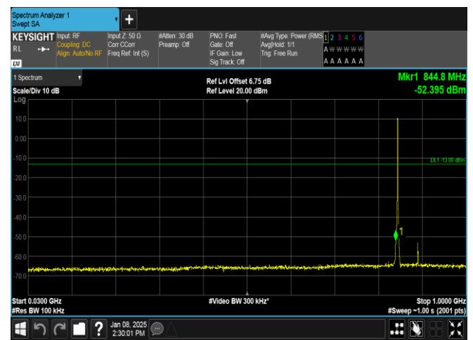
Band26(824-849)-1.4MHz-16QAM-27033-6RB#0-30~1000-PASS
