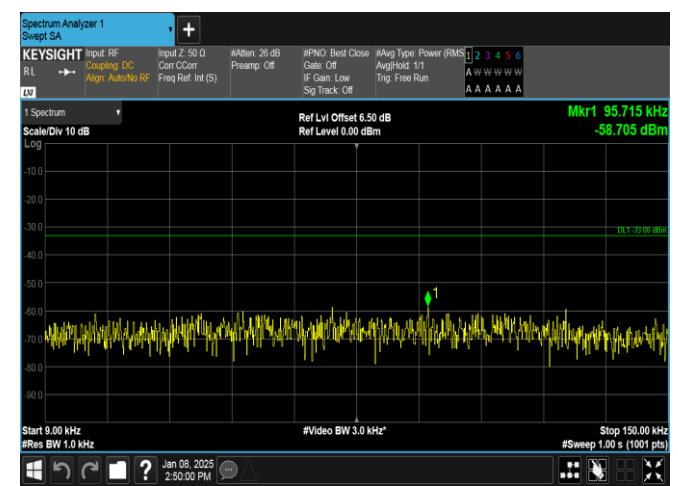
Band26(824-849)-3MHz-16QAM-26805-1RB#0-0.009~0.15-PASS
