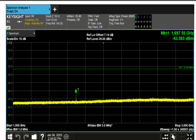
Band26(824-849)-1.4MHz-16QAM-27033-1RB#5-1000~3000-PASS
