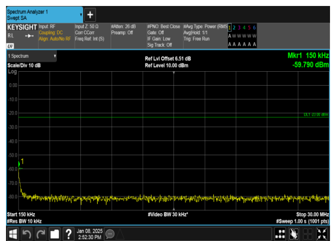
Band26(824-849)-3MHz-16QAM-26805-1RB#14-0.15~30-PASS
