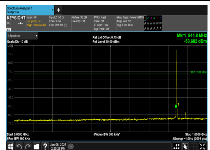
Band26(824-849)-1.4MHz-16QAM-27033-1RB#0-30~1000-PASS
