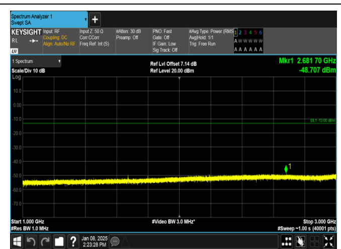
Band26(824-849)-1.4MHz-16QAM-26915-6RB#0-1000~3000-PASS
