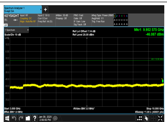
Band26(824-849)-3MHz-QPSK-26915-1RB#0-3000~10000-PASS
