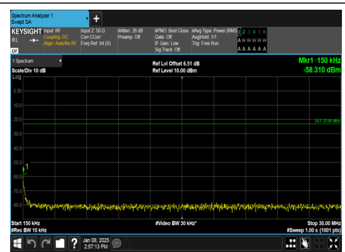
Band26(824-849)-3MHz-16QAM-26915-1RB#0-0.15~30-PASS
