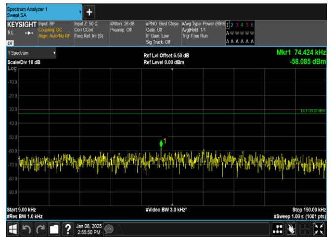
Band26(824-849)-3MHz-QPSK-26915-1RB#0-0.009~0.15-PASS
