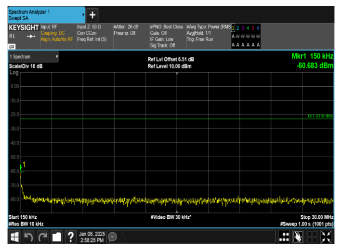
Band26(824-849)-3MHz-QPSK-26915-1RB#14-0.15~30-PASS
