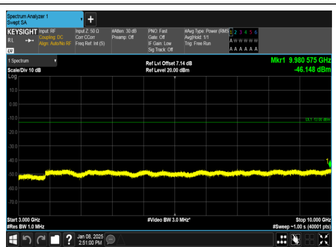
Band26(824-849)-3MHz-16QAM-26805-1RB#0-3000~10000-PASS
