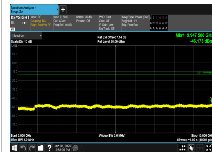
Band26(824-849)-3MHz-16QAM-26915-1RB#0-3000~10000-PASS
