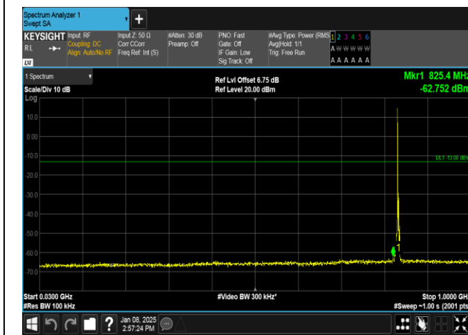
Band26(824-849)-3MHz-16QAM-26915-1RB#0-30~1000-PASS
