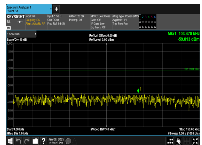
Band26(824-849)-3MHz-16QAM-26915-1RB#14-0.009~0.15-PASS
