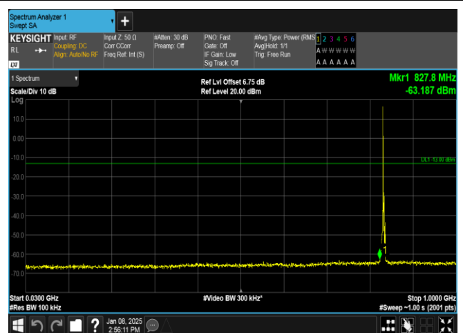
Band26(824-849)-3MHz-QPSK-26915-1RB#0-30~1000-PASS
