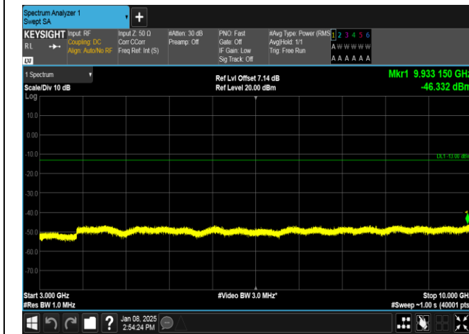
Band26(824-849)-3MHz-QPSK-26805-15RB#0-3000~10000-PASS
