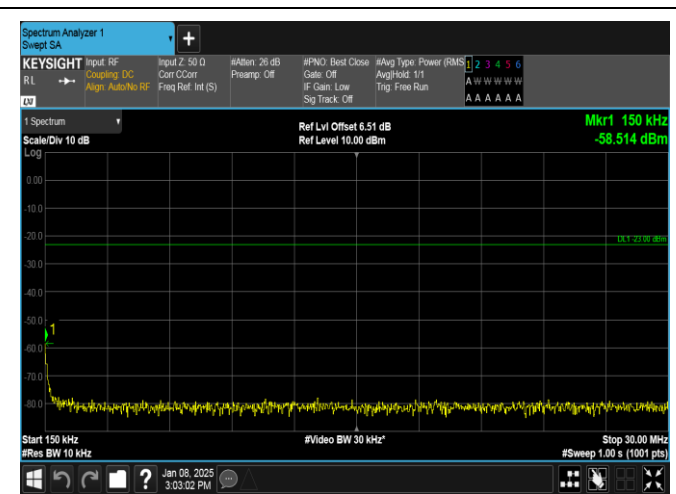
Band26(824-849)-3MHz-QPSK-27025-1RB#0-0.15~30-PASS
