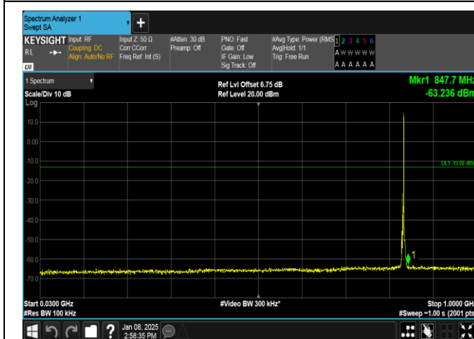
Band26(824-849)-3MHz-QPSK-26915-1RB#14-30~1000-PASS
