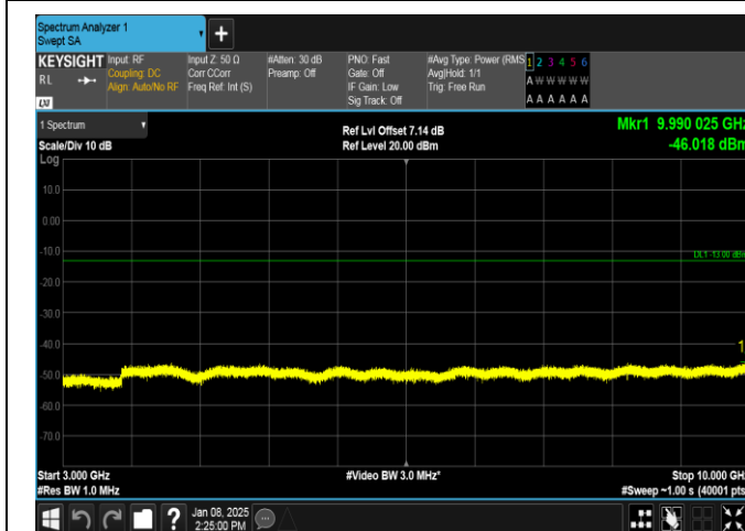
Band26(824-849)-1.4MHz-QPSK-27033-1RB#0-3000~10000-PASS
