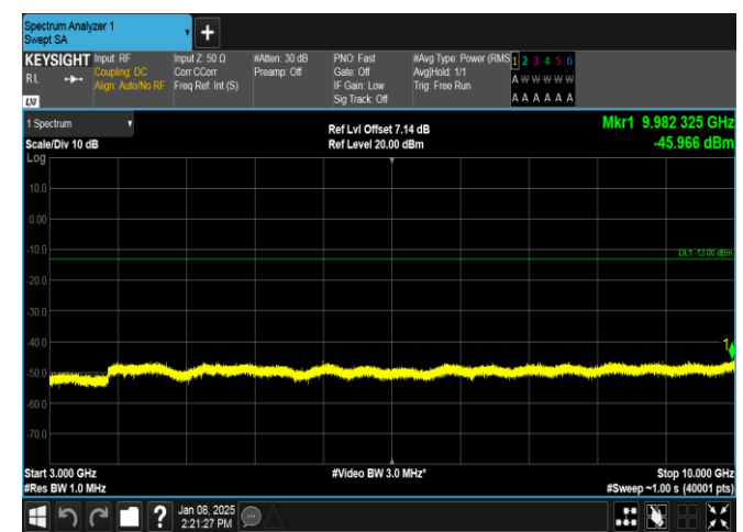
Band26(824-849)-1.4MHz-16QAM-26915-1RB#5-3000~10000-PASS
