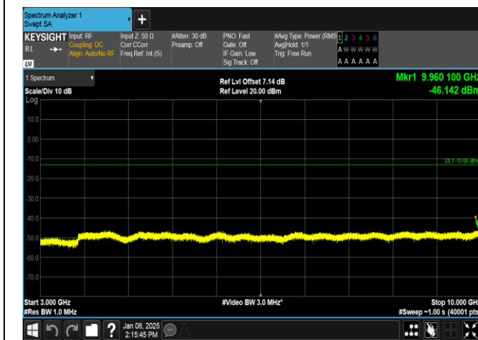
Band26(824-849)-1.4MHz-QPSK-26797-6RB#0-3000~10000-PASS
