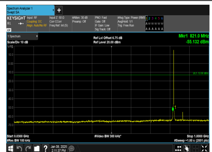
Band26(824-849)-1.4MHz-16QAM-26797-1RB#0-30~1000-PASS
