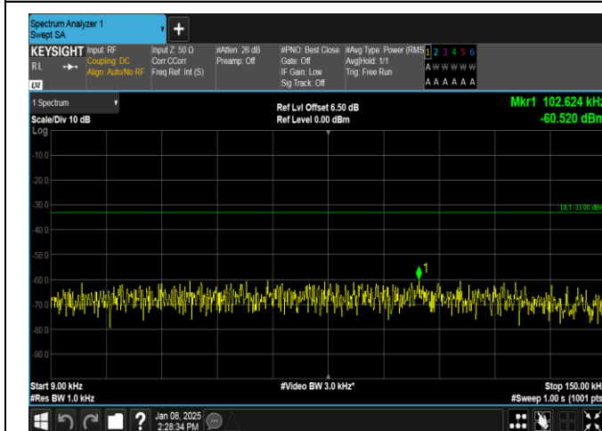
Band26(824-849)-1.4MHz-QPSK-27033-6RB#0-0.009~0.15-PASS
