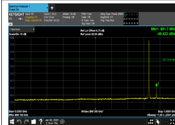
Band26(824-849)-1.4MHz-QPSK-26915-1RB#5-30~1000-PASS
