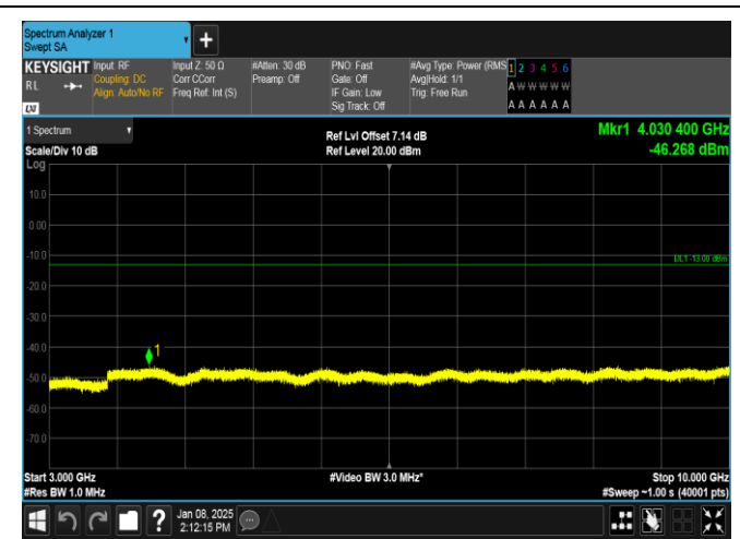
Band26(824-849)-1.4MHz-16QAM-26797-1RB#0-3000~10000-PASS
