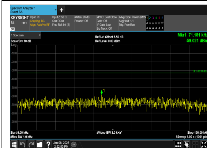
Band26(824-849)-1.4MHz-16QAM-26915-6RB#0-0.009~0.15-PASS
