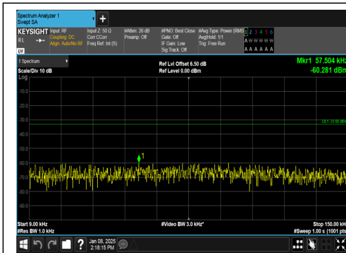
Band26(824-849)-1.4MHz-16QAM-26915-1RB#0-0.009~0.15-PASS
