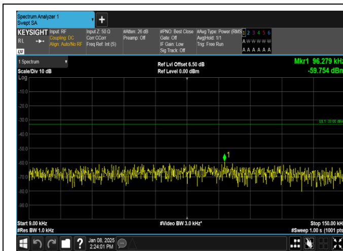
Band26(824-849)-1.4MHz-QPSK-27033-1RB#0-0.009~0.15-PASS
