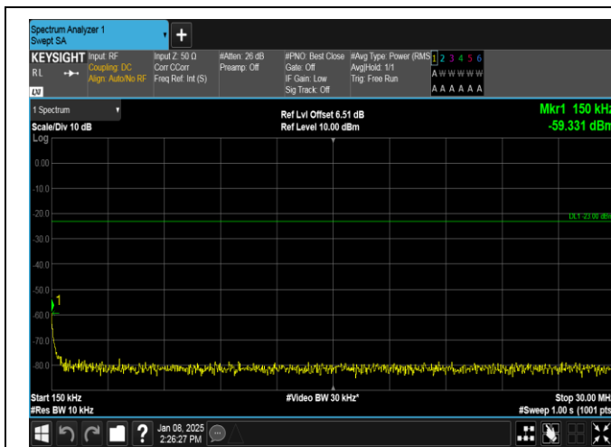
Band26(824-849)-1.4MHz-QPSK-27033-1RB#5-0.15~30-PASS
