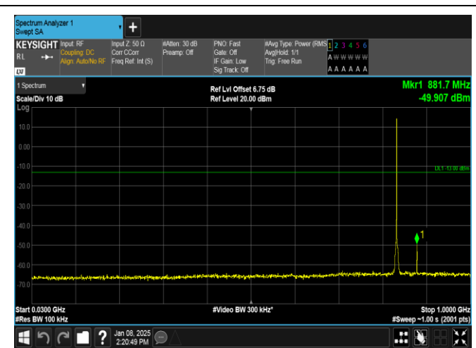
Band26(824-849)-1.4MHz-16QAM-26915-1RB#5-30~1000-PASS
