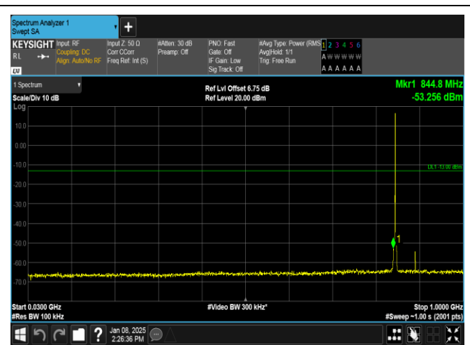
Band26(824-849)-1.4MHz-QPSK-27033-1RB#5-30~1000-PASS
