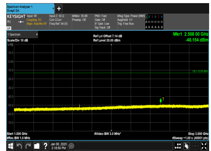
Band26(824-849)-1.4MHz-16QAM-26915-1RB#0-1000~3000-PASS
