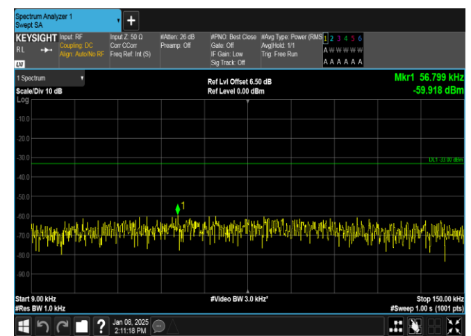
Band26(824-849)-1.4MHz-16QAM-26797-1RB#0-0.009~0.15-PASS
