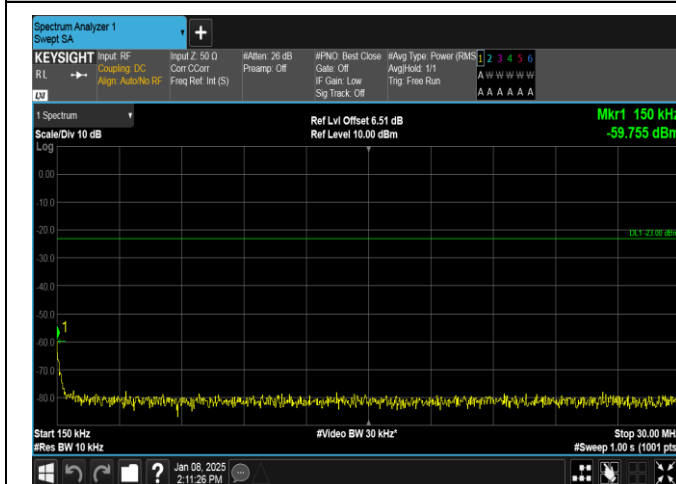
Band26(824-849)-1.4MHz-16QAM-26797-1RB#0-0.15~30-PASS
