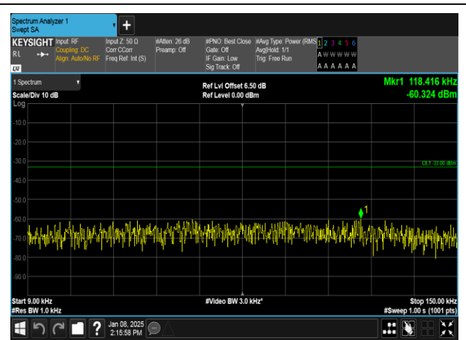
Band26(824-849)-1.4MHz-16QAM-26797-6RB#0-0.009~0.15-PASS
