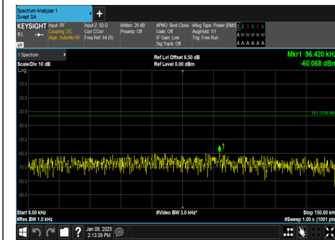
Band26(824-849)-1.4MHz-16QAM-26797-1RB#5-0.009~0.15-PASS
