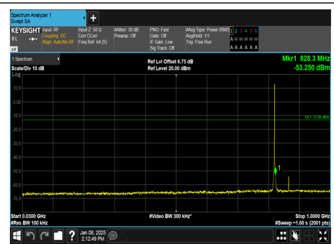
Band26(824-849)-1.4MHz-QPSK-26797-1RB#5-30~1000-PASS
