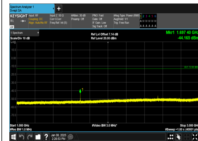
Band26(824-849)-1.4MHz-QPSK-27033-1RB#5-1000~3000-PASS
