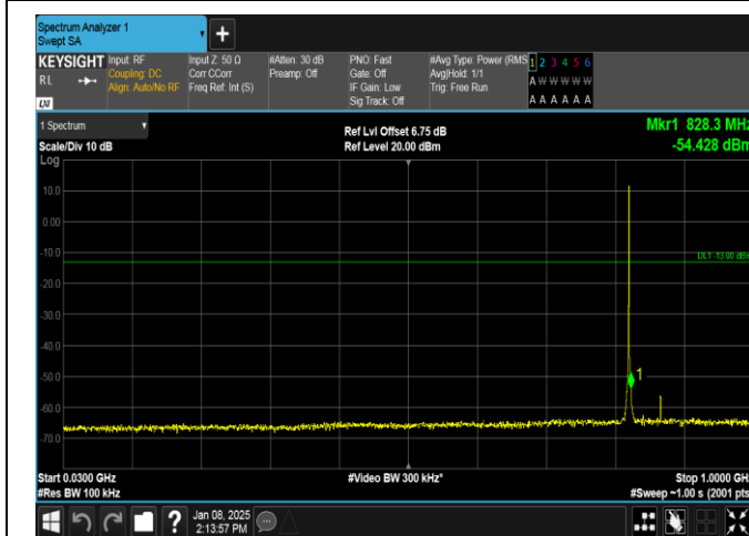
Band26(824-849)-1.4MHz-16QAM-26797-1RB#5-30~1000-PASS
