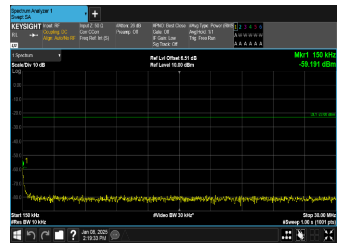
Band26(824-849)-1.4MHz-QPSK-26915-1RB#5-0.15~30-PASS
