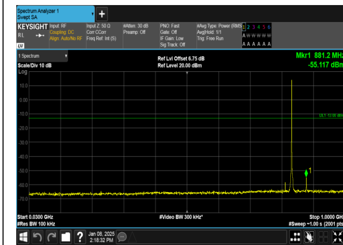
Band26(824-849)-1.4MHz-16QAM-26915-1RB#0-30~1000-PASS
