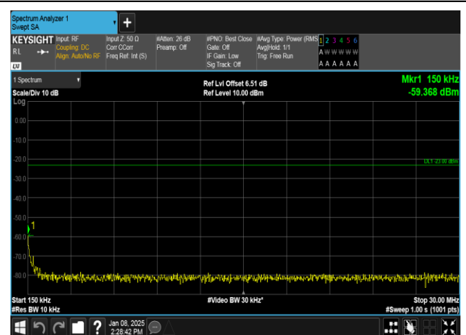
Band26(824-849)-1.4MHz-QPSK-27033-6RB#0-0.15~30-PASS
