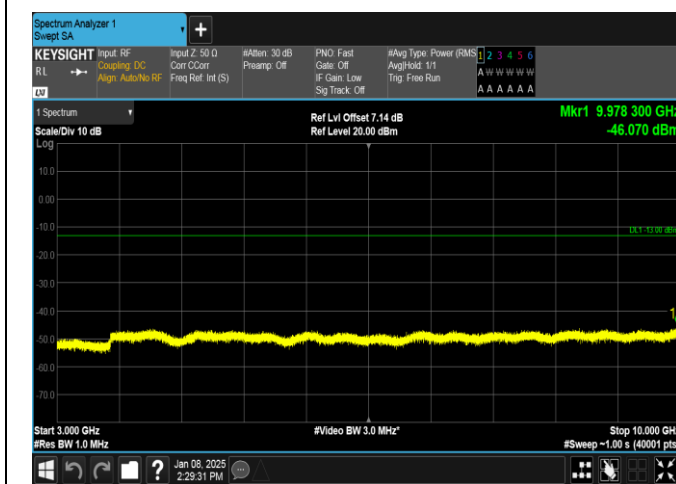
Band26(824-849)-1.4MHz-QPSK-27033-6RB#0-3000~10000-PASS
