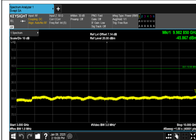
Band26(824-849)-1.4MHz-16QAM-26915-1RB#0-3000~10000-PASS
