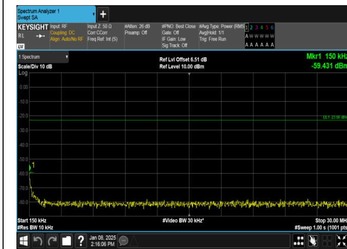
Band26(824-849)-1.4MHz-16QAM-26797-6RB#0-0.15~30-PASS
