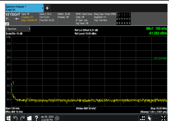
Band26(824-849)-1.4MHz-16QAM-26915-6RB#0-0.15~30-PASS
