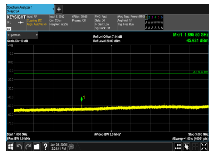
Band26(824-849)-1.4MHz-QPSK-27033-1RB#0-1000~3000-PASS
