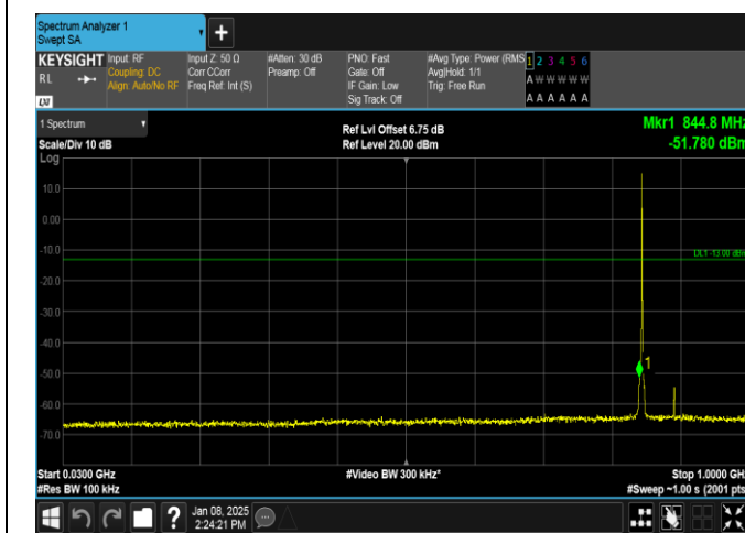
Band26(824-849)-1.4MHz-QPSK-27033-1RB#0-30~1000-PASS
