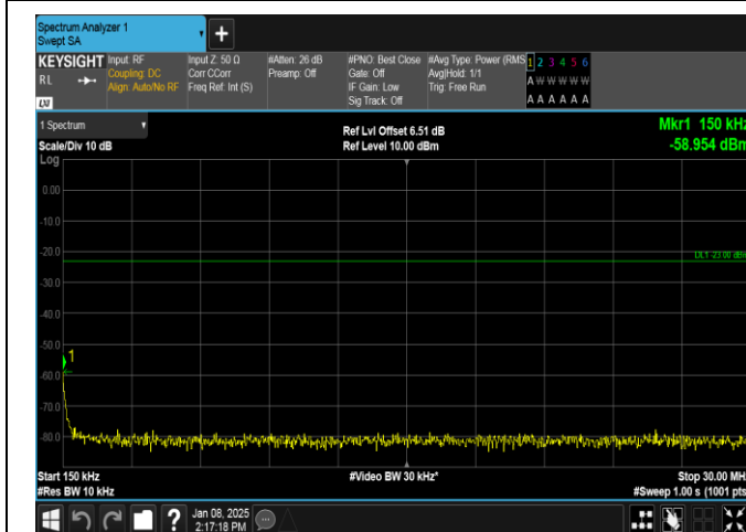
Band26(824-849)-1.4MHz-QPSK-26915-1RB#0-0.15~30-PASS
