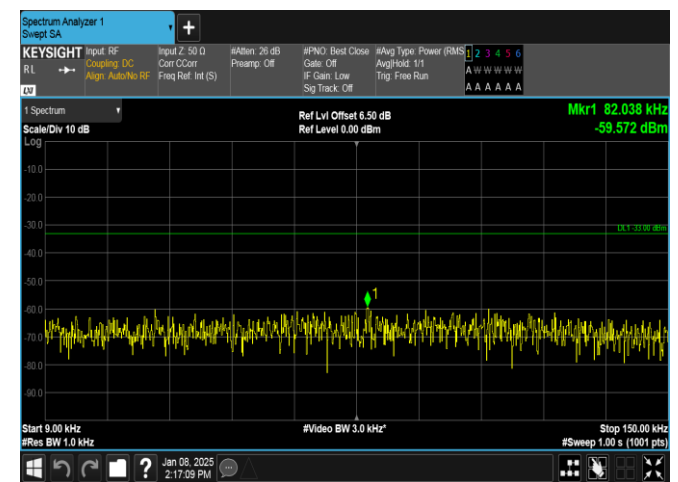
Band26(824-849)-1.4MHz-QPSK-26915-1RB#0-0.009~0.15-PASS
