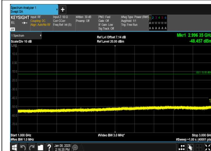
Band26(824-849)-1.4MHz-16QAM-26797-6RB#0-1000~3000-PASS
