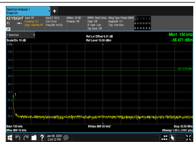
Band26(824-849)-1.4MHz-QPSK-27033-1RB#0-0.15~30-PASS
