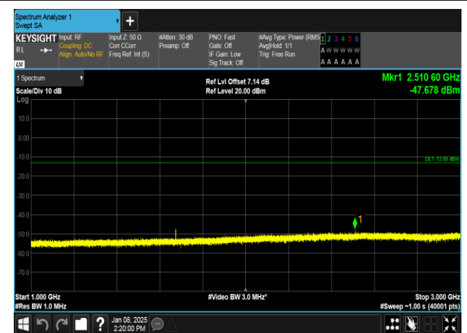
Band26(824-849)-1.4MHz-QPSK-26915-1RB#5-1000~3000-PASS
