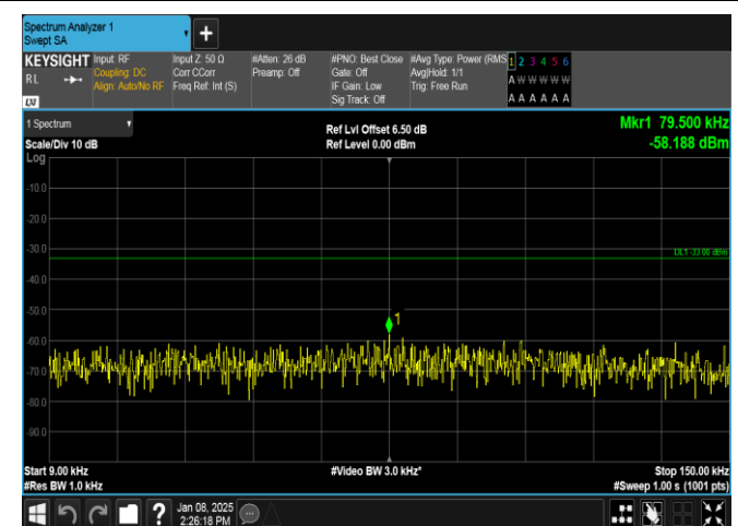
Band26(824-849)-1.4MHz-QPSK-27033-1RB#5-0.009~0.15-PASS
