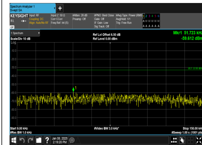
Band26(824-849)-1.4MHz-QPSK-26915-1RB#5-0.009~0.15-PASS
