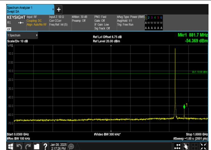
Band26(824-849)-1.4MHz-QPSK-26915-1RB#0-30~1000-PASS
