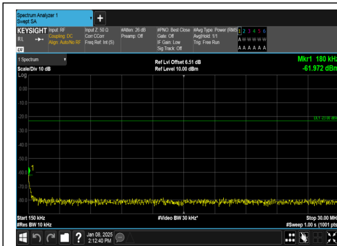
Band26(824-849)-1.4MHz-QPSK-26797-1RB#5-0.15~30-PASS
