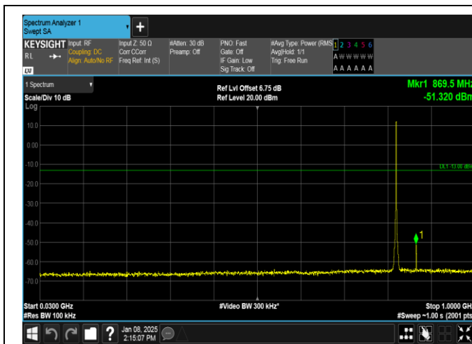
Band26(824-849)-1.4MHz-QPSK-26797-6RB#0-30~1000-PASS
