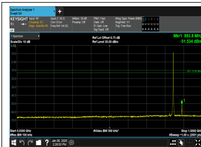
Band26(824-849)-1.4MHz-QPSK-27033-6RB#0-30~1000-PASS
