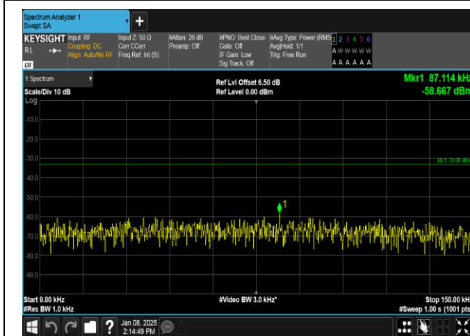
Band26(824-849)-1.4MHz-QPSK-26797-6RB#0-0.009~0.15-PASS
