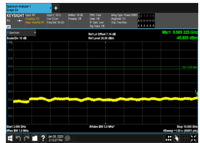
Band26(824-849)-1.4MHz-QPSK-26797-1RB#5-3000~10000-PASS
