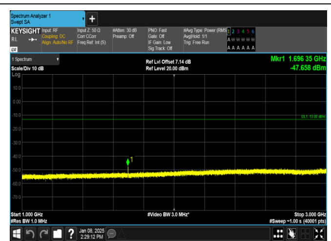
Band26(824-849)-1.4MHz-QPSK-27033-6RB#0-1000~3000-PASS
