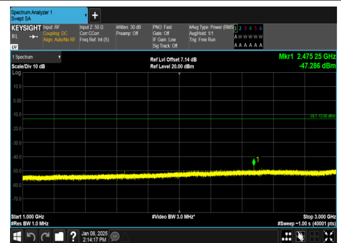
Band26(824-849)-1.4MHz-16QAM-26797-1RB#5-1000~3000-PASS
