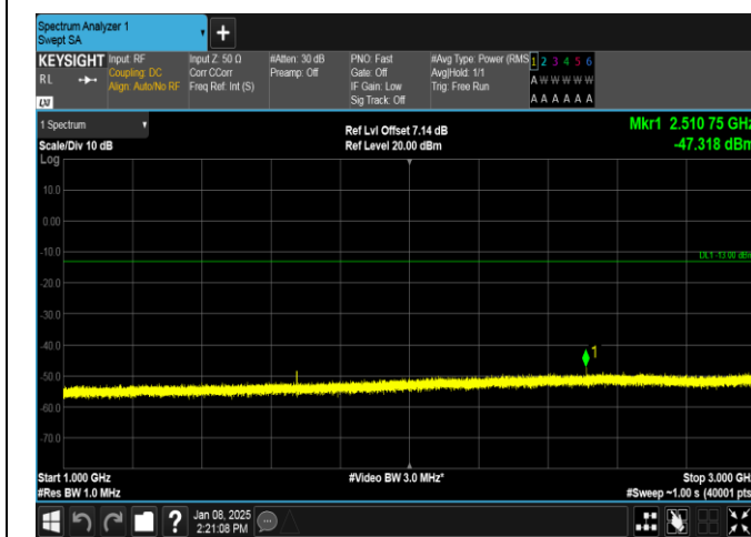
Band26(824-849)-1.4MHz-16QAM-26915-1RB#5-1000~3000-PASS
