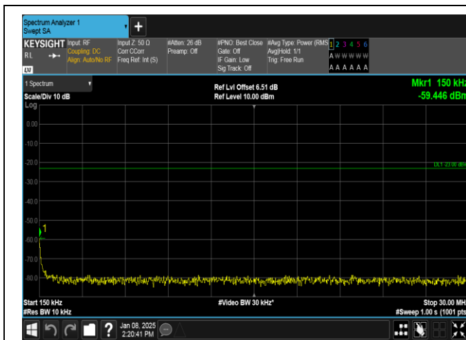
Band26(824-849)-1.4MHz-16QAM-26915-1RB#5-0.15~30-PASS
