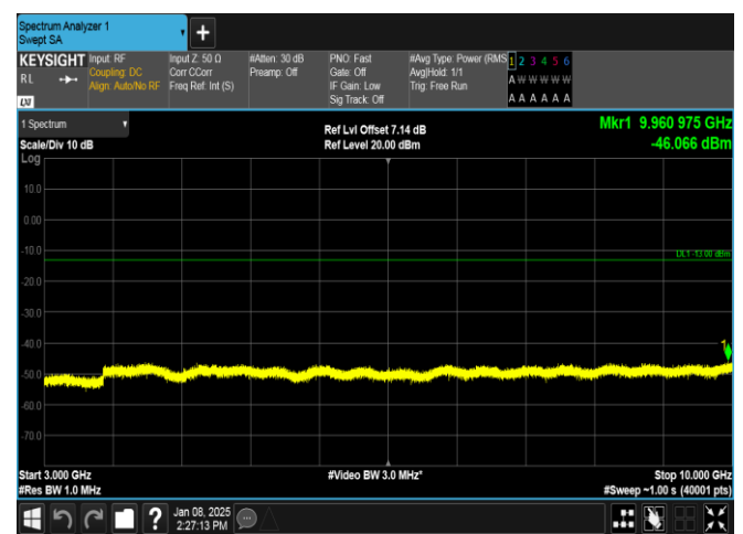
Band26(824-849)-1.4MHz-QPSK-27033-1RB#5-3000~10000-PASS
