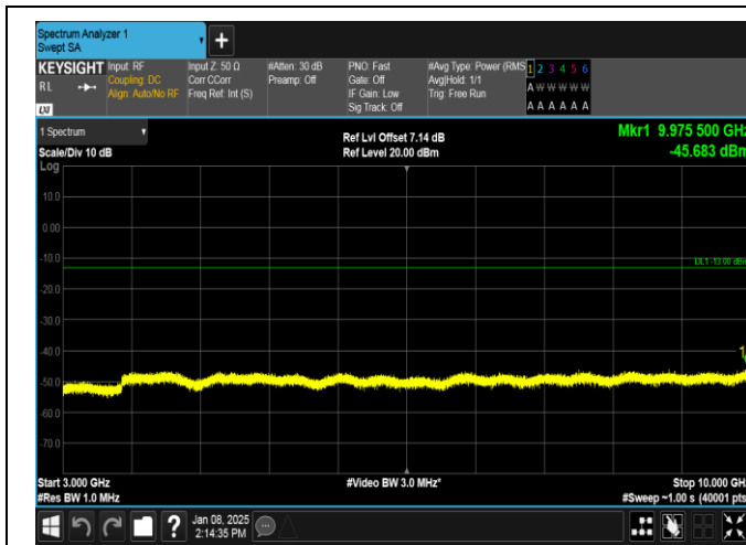
Band26(824-849)-1.4MHz-16QAM-26797-1RB#5-3000~10000-PASS
