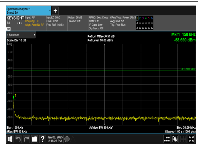
Band26(824-849)-1.4MHz-16QAM-26915-1RB#0-0.15~30-PASS
