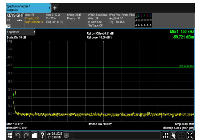
Band26(824-849)-1.4MHz-16QAM-26797-1RB#5-0.15~30-PASS
