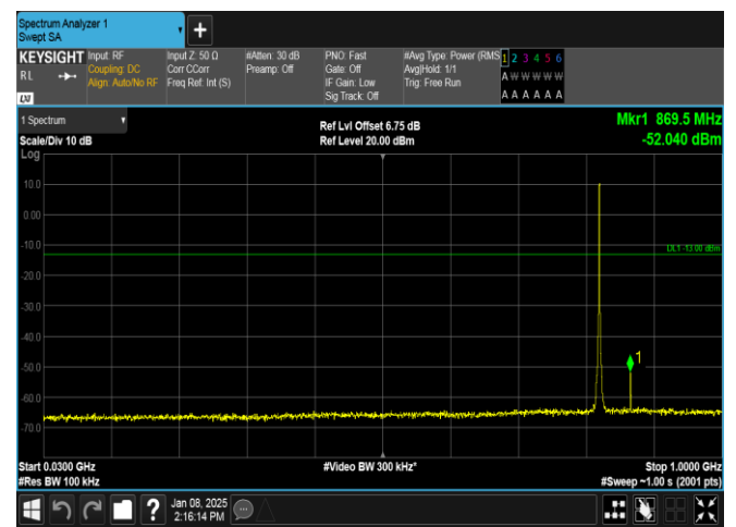
Band26(824-849)-1.4MHz-16QAM-26797-6RB#0-30~1000-PASS
