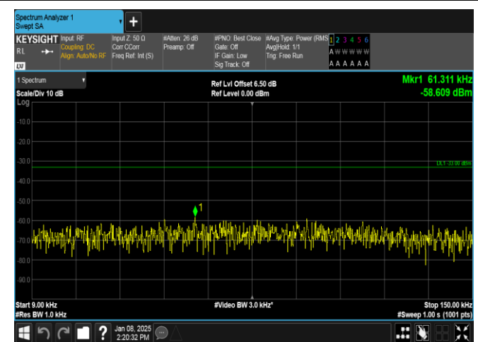
Band26(824-849)-1.4MHz-16QAM-26915-1RB#5-0.009~0.15-PASS
