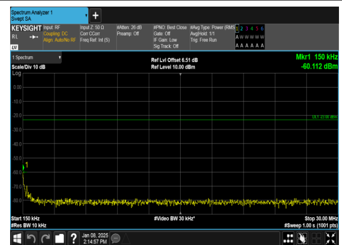
Band26(824-849)-1.4MHz-QPSK-26797-6RB#0-0.15~30-PASS
