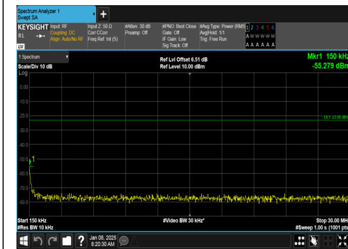
Band26(814-824)-1.4MHz-16QAM-26783-6RB#0-0.15~30-PASS
