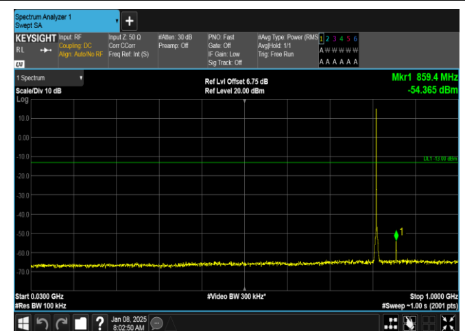
Band26(814-824)-1.4MHz-16QAM-26697-1RB#0-30~1000-PASS
