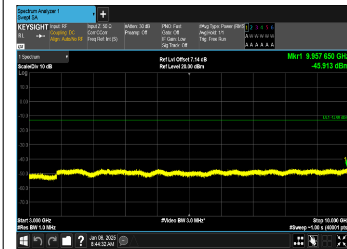
Band26(814-824)-3MHz-QPSK-26705-15RB#0-3000~10000-PASS
