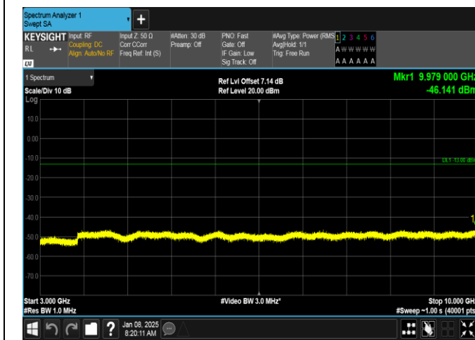
Band26(814-824)-1.4MHz-QPSK-26783-6RB#0-3000~10000-PASS
