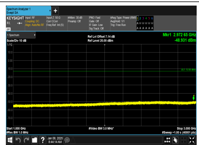
Band26(814-824)-3MHz-QPSK-26705-15RB#0-1000~3000-PASS
