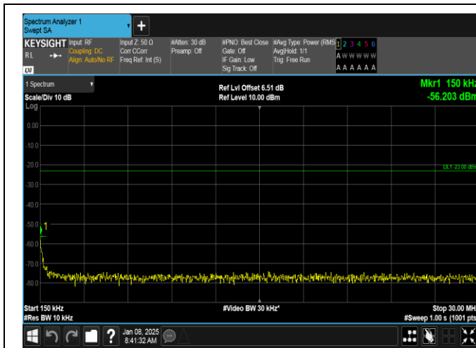
Band26(814-824)-3MHz-QPSK-26705-1RB#14-0.15~30-PASS
