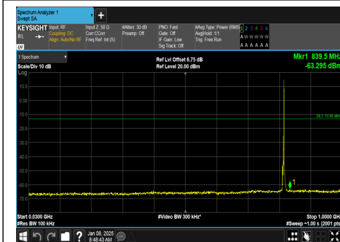
Band26(814-824)-3MHz-QPSK-26740-1RB#14-30~1000-PASS
