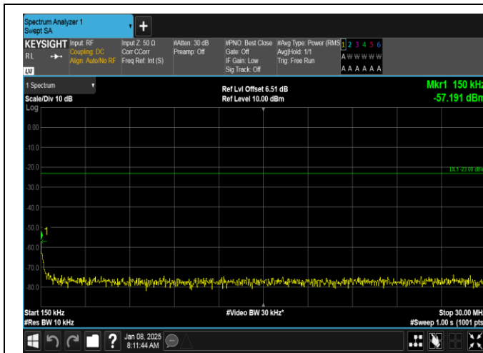
Band26(814-824)-1.4MHz-16QAM-26740-1RB#5-0.15~30-PASS
