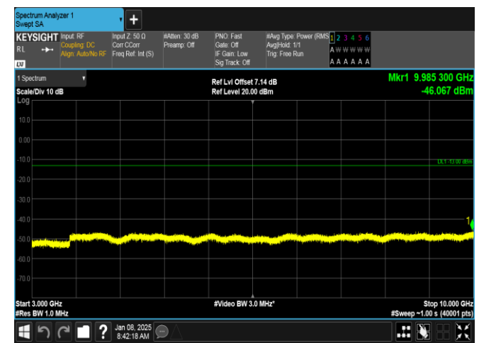
Band26(814-824)-3MHz-QPSK-26705-1RB#14-3000~10000-PASS
