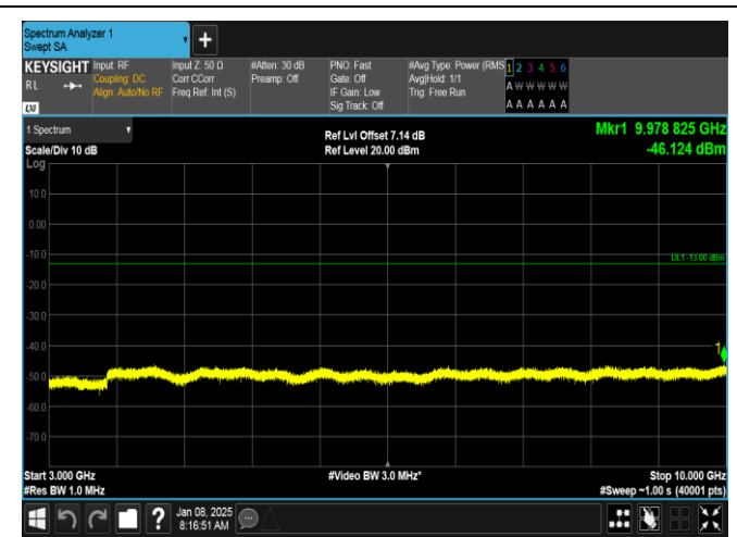
Band26(814-824)-1.4MHz-16QAM-26783-1RB#0-3000~10000-PASS
