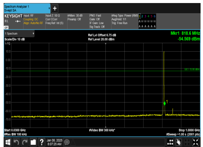
Band26(814-824)-1.4MHz-16QAM-26697-6RB#0-30~1000-PASS
