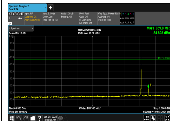
Band26(814-824)-1.4MHz-16QAM-26697-1RB#5-30~1000-PASS
