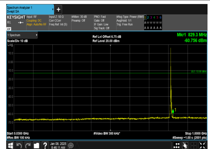
Band26(814-824)-3MHz-QPSK-26740-1RB#0-30~1000-PASS
