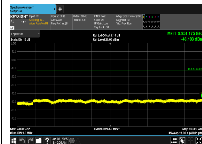
Band26(814-824)-3MHz-QPSK-26705-1RB#0-3000~10000-PASS
