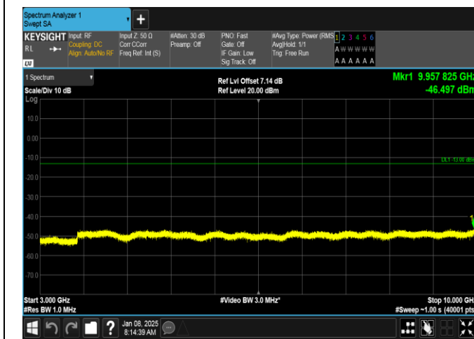
Band26(814-824)-1.4MHz-16QAM-26740-6RB#0-3000~10000-PASS
