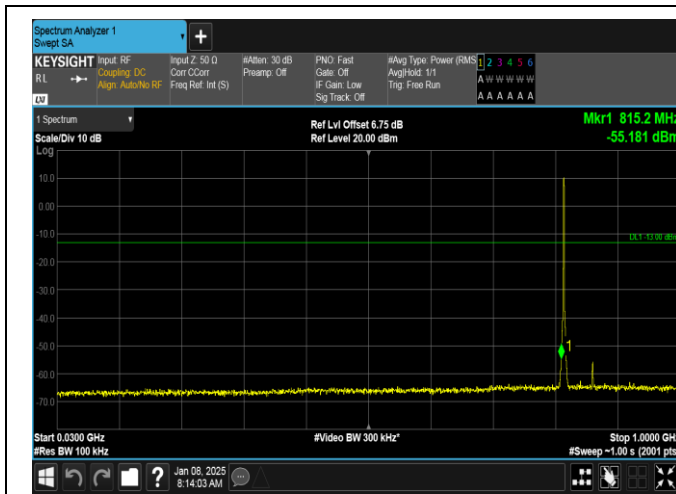
Band26(814-824)-1.4MHz-16QAM-26740-6RB#0-30~1000-PASS
