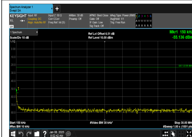
Band26(814-824)-1.4MHz-16QAM-26697-1RB#0-0.15~30-PASS
