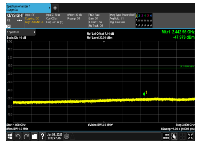
Band26(814-824)-3MHz-QPSK-26705-1RB#0-1000~3000-PASS
