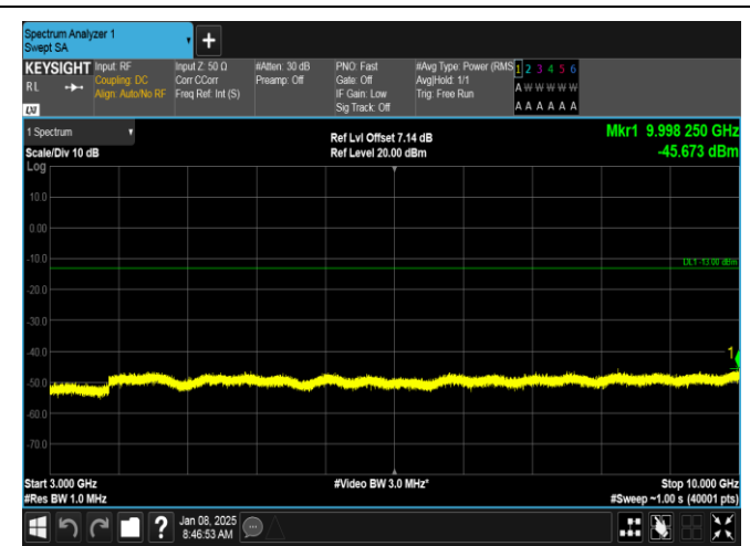
Band26(814-824)-3MHz-QPSK-26740-1RB#0-3000~10000-PASS
