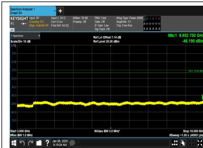
Band26(814-824)-1.4MHz-16QAM-26783-1RB#5-3000~10000-PASS
