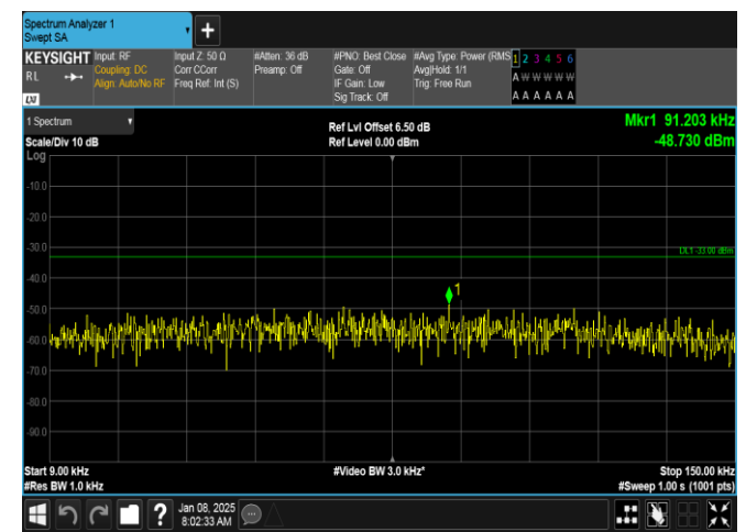
Band26(814-824)-1.4MHz-16QAM-26697-1RB#0-0.009~0.15-PASS
