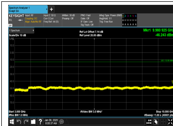
Band26(814-824)-1.4MHz-16QAM-26697-1RB#5-3000~10000-PASS
