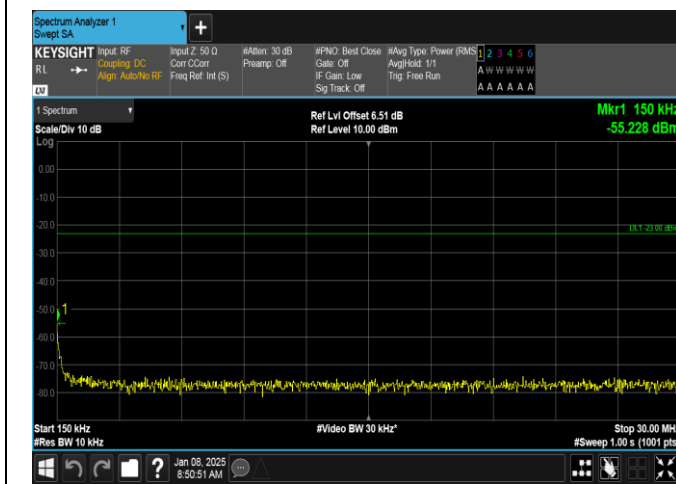
Band26(814-824)-3MHz-QPSK-26740-15RB#0-0.15~30-PASS
