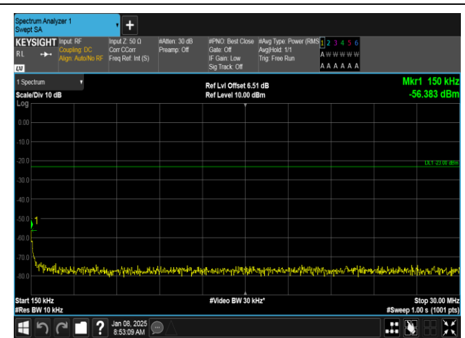
Band26(814-824)-3MHz-QPSK-26775-1RB#0-0.15~30-PASS
