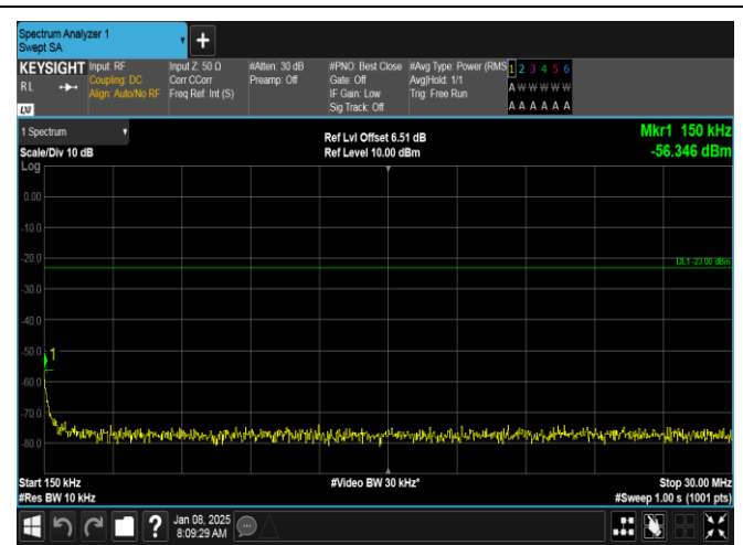
Band26(814-824)-1.4MHz-16QAM-26740-1RB#0-0.15~30-PASS
