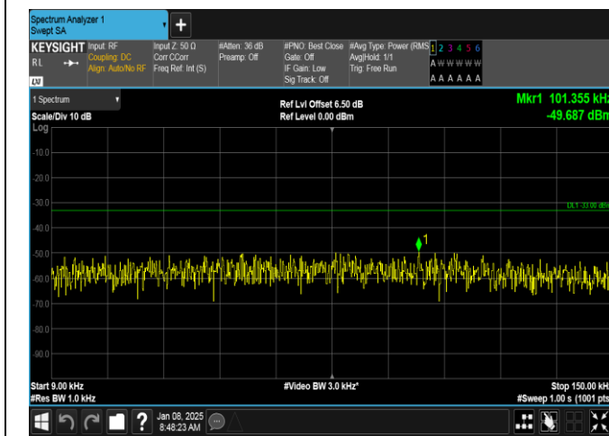
Band26(814-824)-3MHz-QPSK-26740-1RB#14-0.009~0.15-PASS
