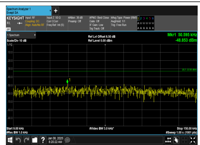
Band26(814-824)-1.4MHz-16QAM-26783-6RB#0-0.009~0.15-PASS
