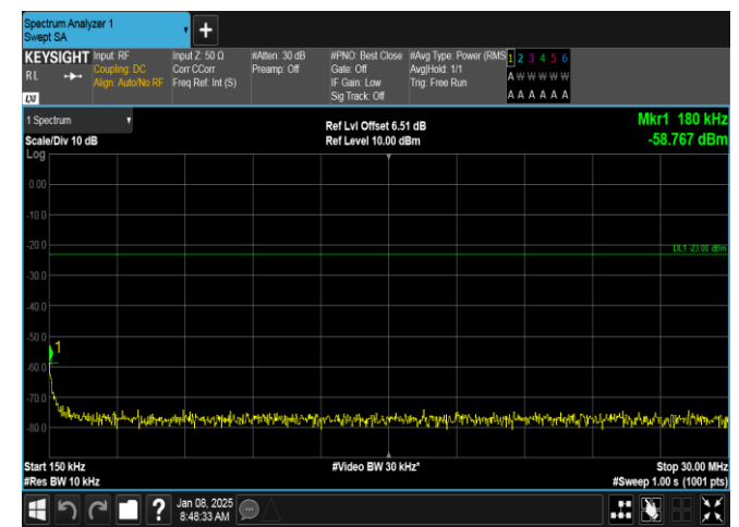
Band26(814-824)-3MHz-QPSK-26740-1RB#14-0.15~30-PASS
