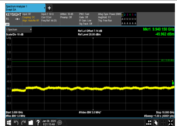
Band26(814-824)-1.4MHz-16QAM-26783-6RB#0-3000~10000-PASS
