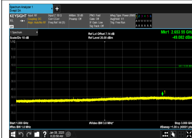
Band26(814-824)-1.4MHz-16QAM-26783-6RB#0-1000~3000-PASS
