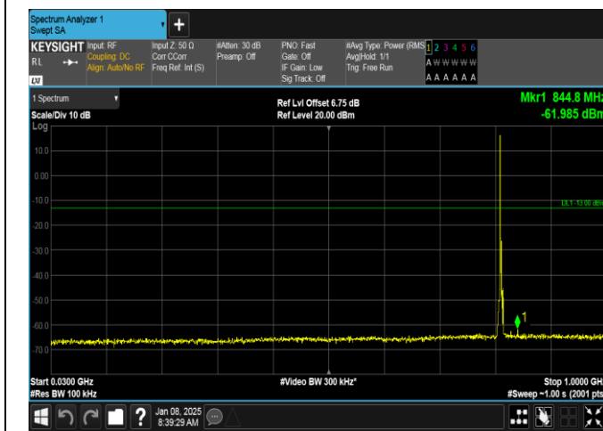
Band26(814-824)-3MHz-QPSK-26705-1RB#0-30~1000-PASS
