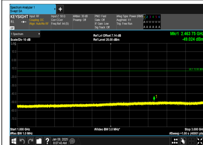
Band26(814-824)-1.4MHz-16QAM-26697-6RB#0-1000~3000-PASS
