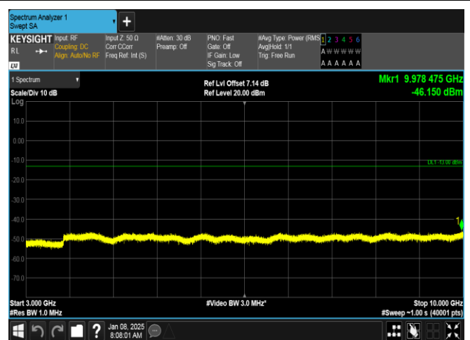
Band26(814-824)-1.4MHz-16QAM-26697-6RB#0-3000~10000-PASS
