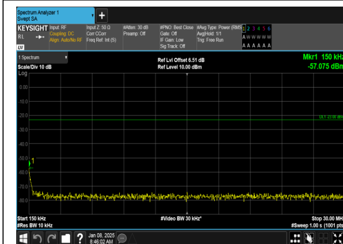
Band26(814-824)-3MHz-QPSK-26740-1RB#0-0.15~30-PASS
