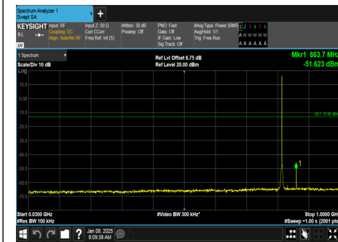
Band26(814-824)-1.4MHz-16QAM-26740-1RB#0-30~1000-PASS
