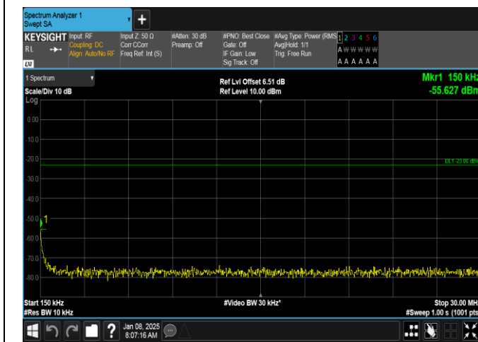
Band26(814-824)-1.4MHz-16QAM-26697-6RB#0-0.15~30-PASS
