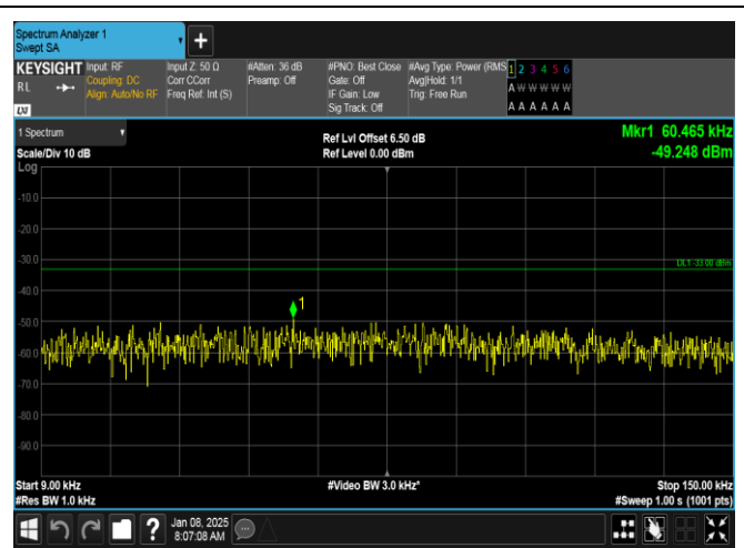
Band26(814-824)-1.4MHz-16QAM-26697-6RB#0-0.009~0.15-PASS
