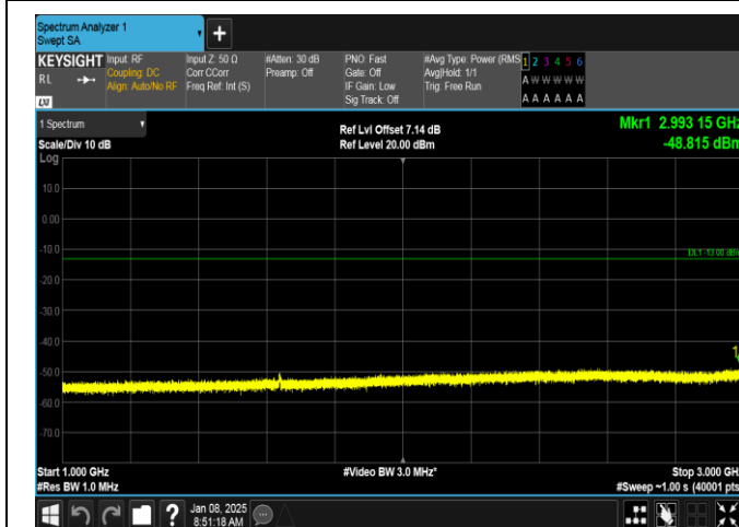
Band26(814-824)-3MHz-QPSK-26740-15RB#0-1000~3000-PASS
