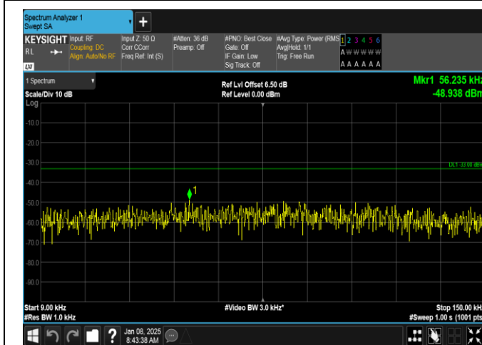
Band26(814-824)-3MHz-QPSK-26705-15RB#0-0.009~0.15-PASS
