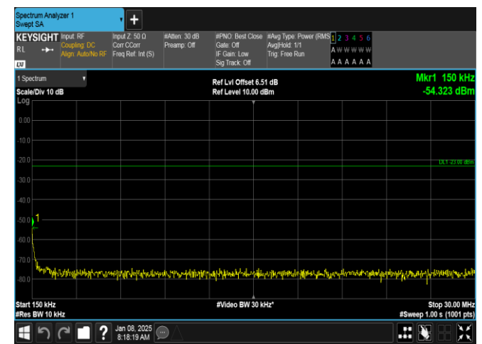
Band26(814-824)-1.4MHz-16QAM-26783-1RB#5-0.15~30-PASS
