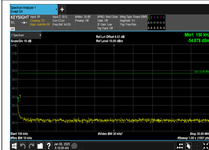
Band26(814-824)-1.4MHz-16QAM-26783-1RB#0-0.15~30-PASS
