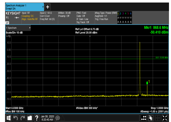
Band26(814-824)-1.4MHz-16QAM-26783-6RB#0-30~1000-PASS
