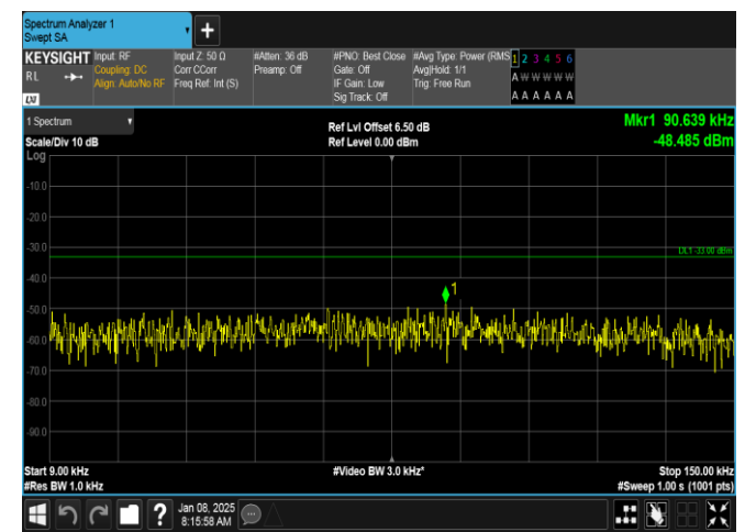
Band26(814-824)-1.4MHz-16QAM-26783-1RB#0-0.009~0.15-PASS
