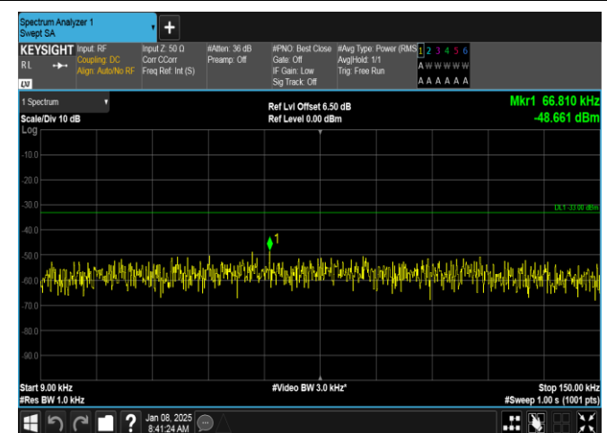
Band26(814-824)-3MHz-QPSK-26705-1RB#14-0.009~0.15-PASS
