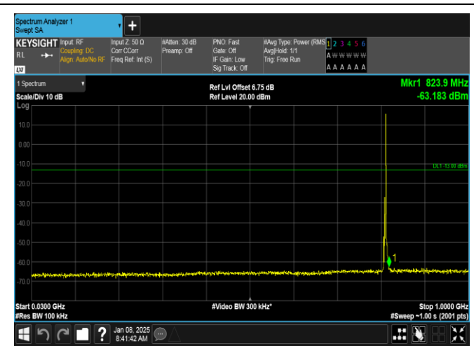
Band26(814-824)-3MHz-QPSK-26705-1RB#14-30~1000-PASS
