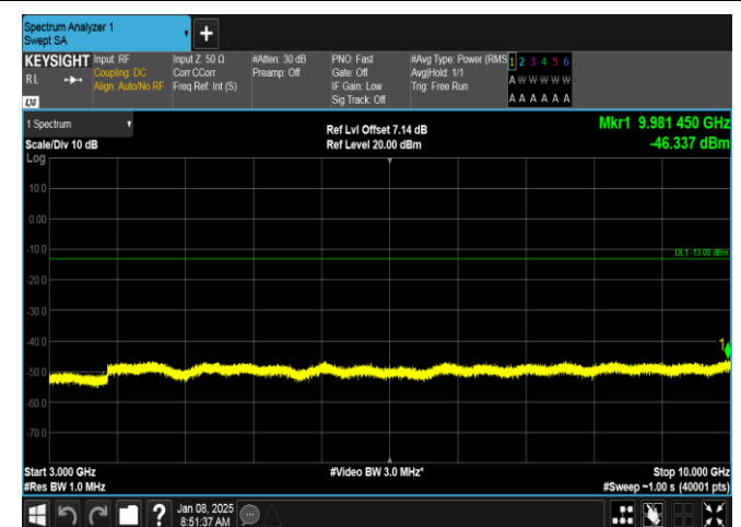
Band26(814-824)-3MHz-QPSK-26740-15RB#0-3000~10000-PASS
