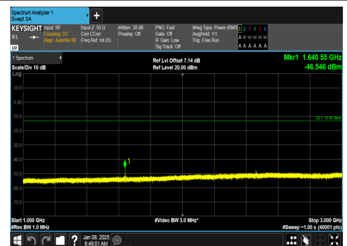
Band26(814-824)-3MHz-QPSK-26740-1RB#14-1000~3000-PASS
