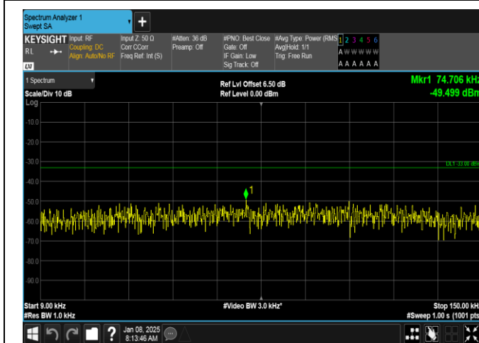
Band26(814-824)-1.4MHz-16QAM-26740-6RB#0-0.009~0.15-PASS
