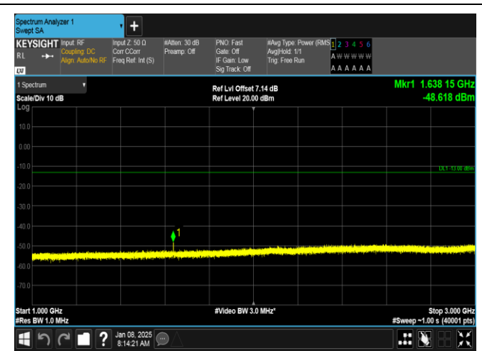
Band26(814-824)-1.4MHz-16QAM-26740-6RB#0-1000~3000-PASS
