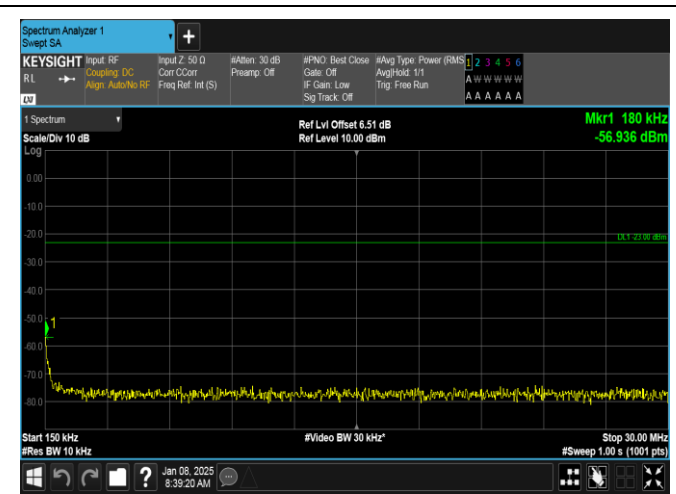
Band26(814-824)-3MHz-QPSK-26705-1RB#0-0.15~30-PASS
