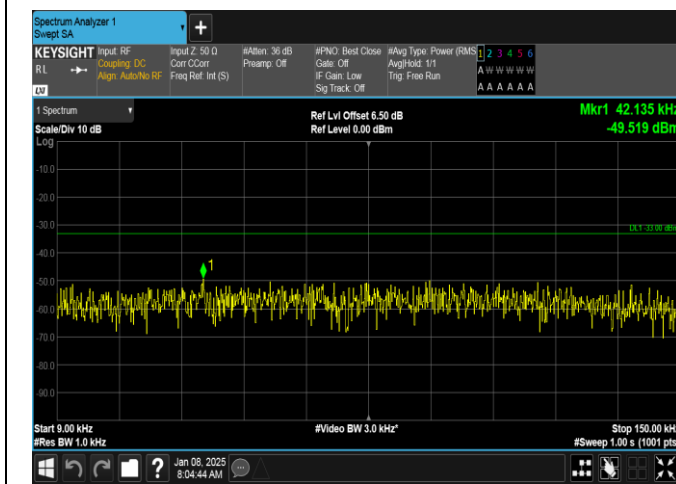
Band26(814-824)-1.4MHz-16QAM-26697-1RB#5-0.009~0.15-PASS
