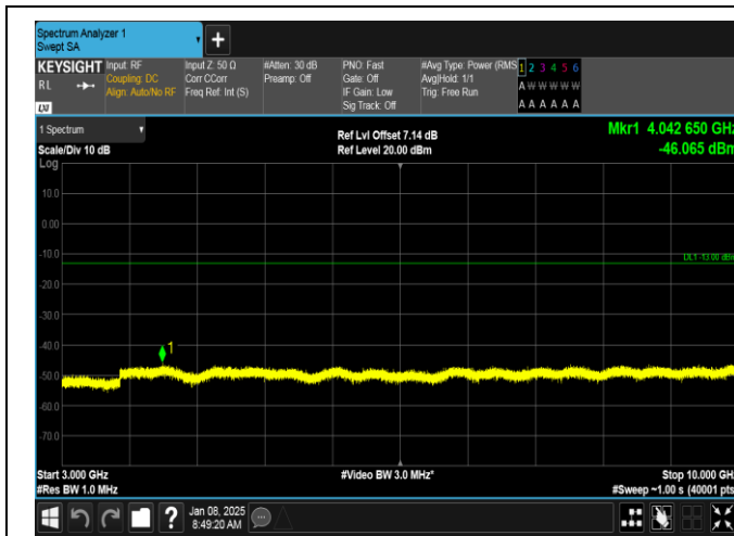
Band26(814-824)-3MHz-QPSK-26740-1RB#14-3000~10000-PASS
