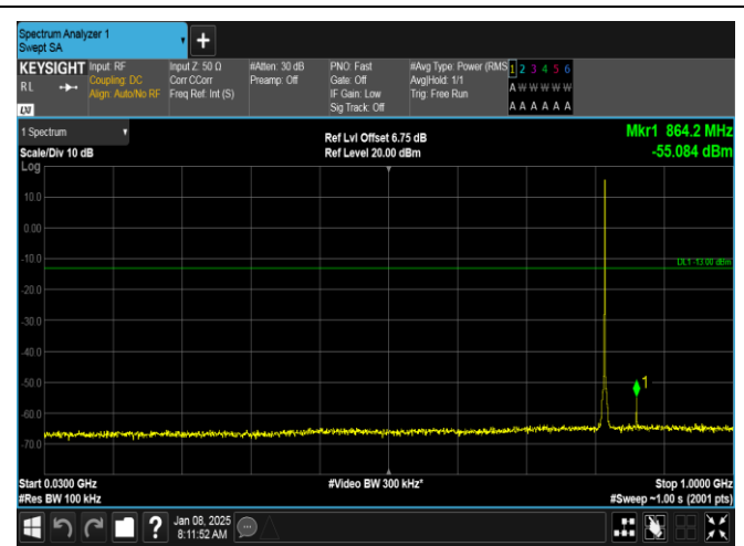
Band26(814-824)-1.4MHz-16QAM-26740-1RB#5-30~1000-PASS
