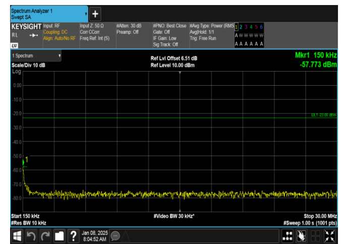
Band26(814-824)-1.4MHz-16QAM-26697-1RB#5-0.15~30-PASS
