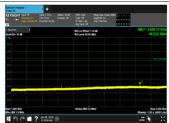
Band26(814-824)-1.4MHz-QPSK-26783-6RB#0-1000~3000-PASS
