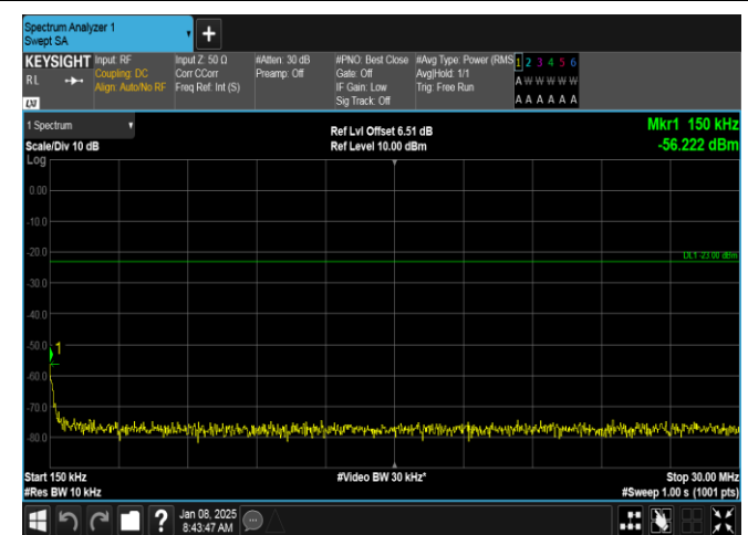
Band26(814-824)-3MHz-QPSK-26705-15RB#0-0.15~30-PASS
