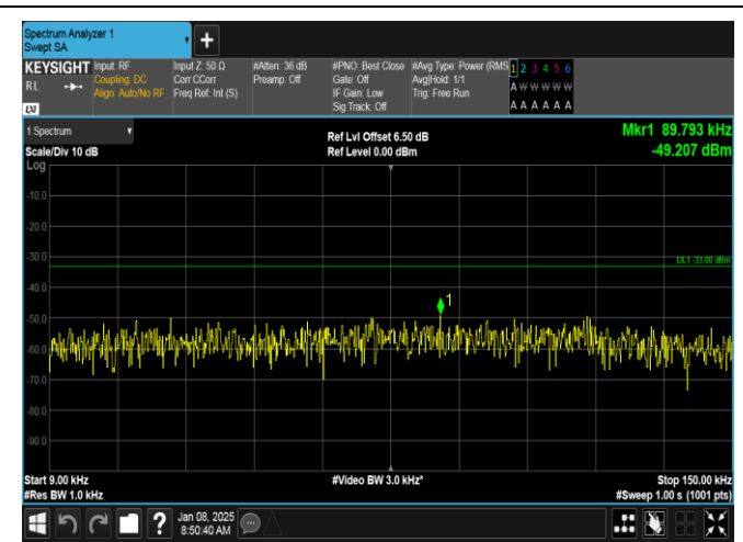
Band26(814-824)-3MHz-QPSK-26740-15RB#0-0.009~0.15-PASS
