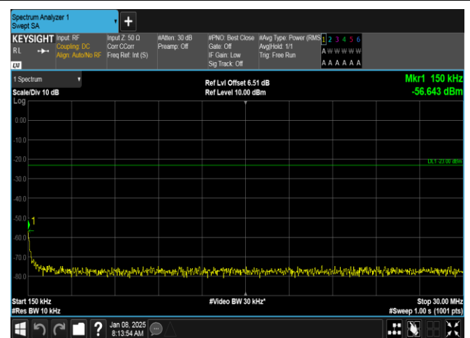
Band26(814-824)-1.4MHz-16QAM-26740-6RB#0-0.15~30-PASS
