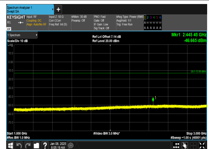
Band26(814-824)-1.4MHz-16QAM-26697-1RB#5-1000~3000-PASS
