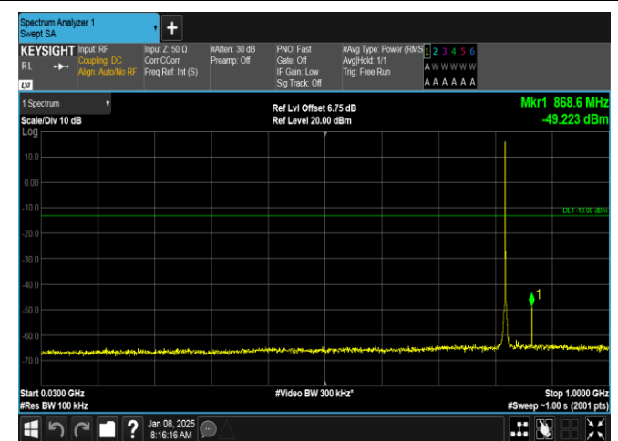
Band26(814-824)-1.4MHz-16QAM-26783-1RB#0-30~1000-PASS
