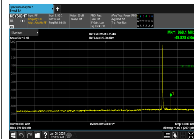
Band26(814-824)-1.4MHz-16QAM-26783-1RB#5-30~1000-PASS
