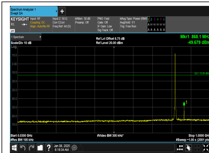
Band26(814-824)-1.4MHz-QPSK-26783-6RB#0-30~1000-PASS
