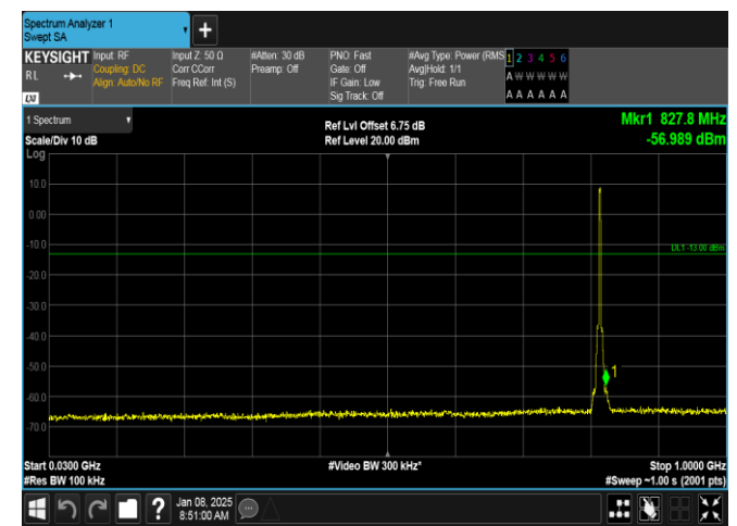
Band26(814-824)-3MHz-QPSK-26740-15RB#0-30~1000-PASS
