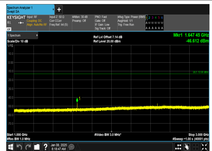
Band26(814-824)-1.4MHz-16QAM-26783-1RB#5-1000~3000-PASS
