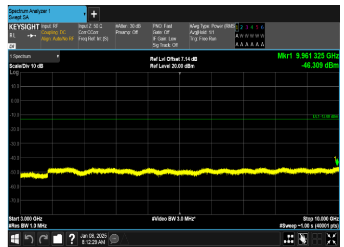
Band26(814-824)-1.4MHz-16QAM-26740-1RB#5-3000~10000-PASS
