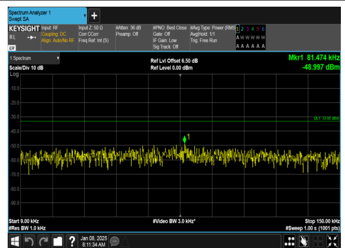
Band26(814-824)-1.4MHz-16QAM-26740-1RB#5-0.009~0.15-PASS
