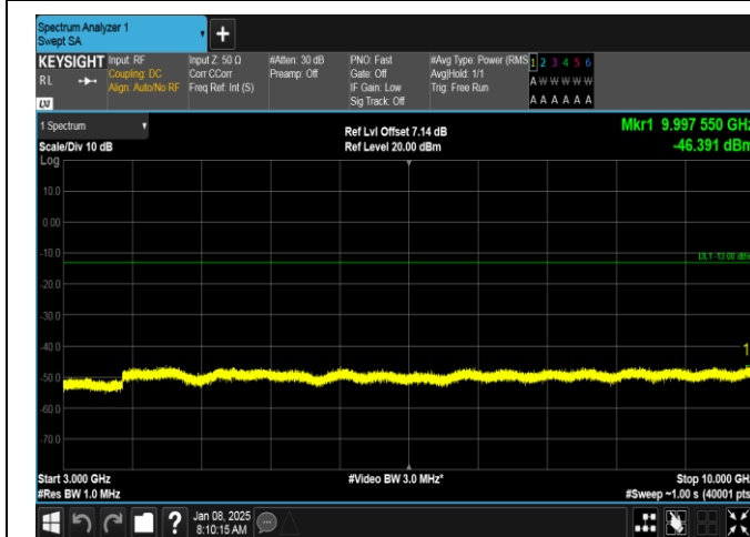
Band26(814-824)-1.4MHz-16QAM-26740-1RB#0-3000~10000-PASS
