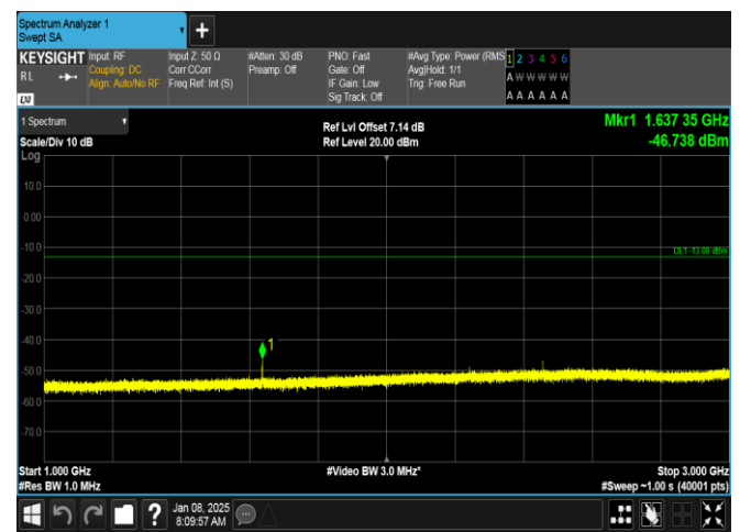
Band26(814-824)-1.4MHz-16QAM-26740-1RB#0-1000~3000-PASS
