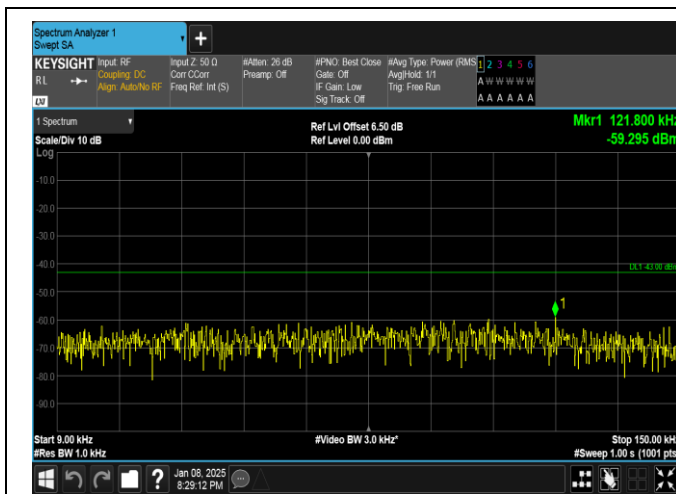
Band25-15MHz-QPSK-26615-1RB#0-0.009~0.15-PASS
