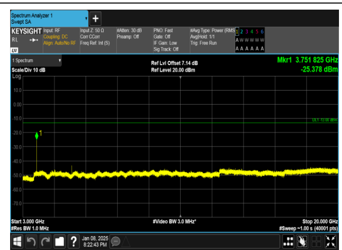
Band25-15MHz-QPSK-26365-1RB#0-3000~20000-PASS
