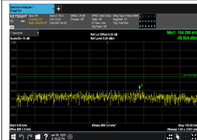
Band25-15MHz-QPSK-26115-75RB#0-0.009~0.15-PASS
