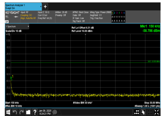
Band25-15MHz-QPSK-26365-1RB#74-0.15~30-PASS
