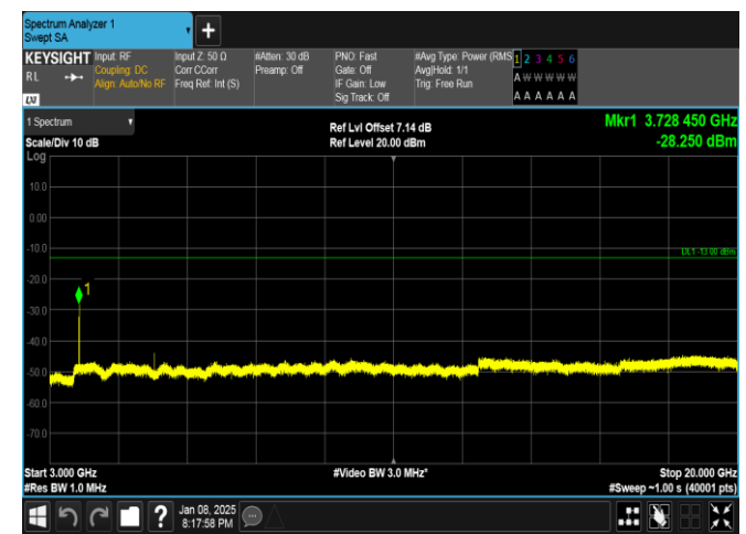
Band25-15MHz-QPSK-26115-1RB#74-3000~20000-PASS
