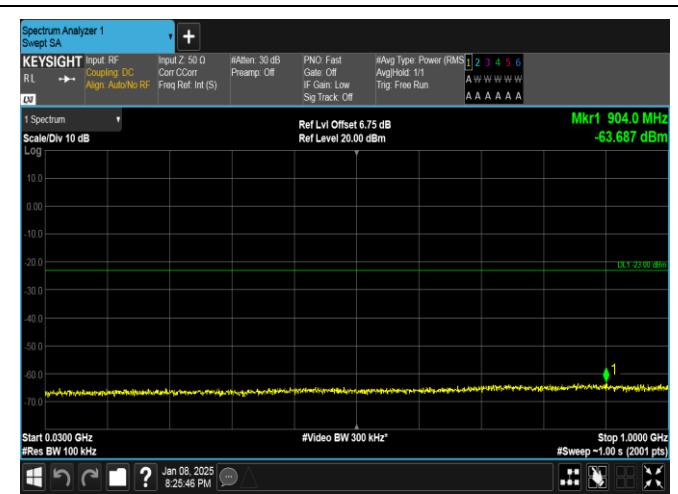
Band25-15MHz-16QAM-26365-1RB#74-30~1000-PASS
