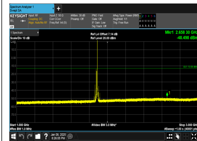
Band25-15MHz-16QAM-26365-1RB#74-1000~3000-PASS
