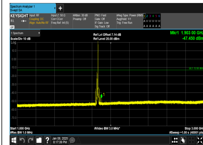
Band25-15MHz-QPSK-26115-1RB#74-1000~3000-PASS
