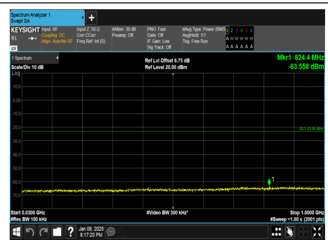
Band25-15MHz-QPSK-26115-1RB#74-30~1000-PASS
