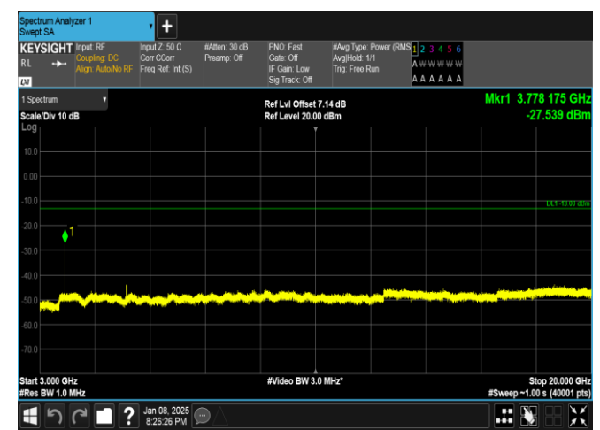
Band25-15MHz-16QAM-26365-1RB#74-3000~20000-PASS
