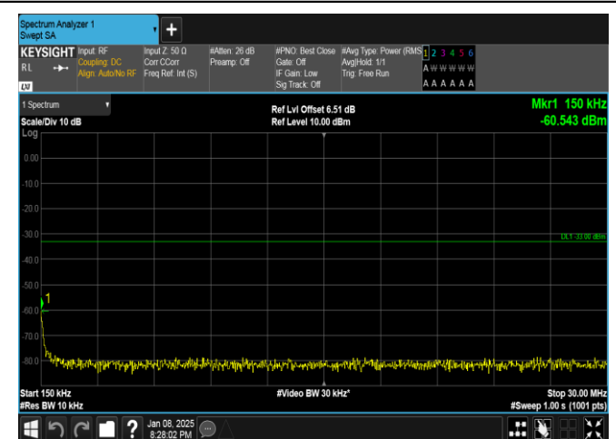
Band25-15MHz-16QAM-26365-75RB#0-0.15~30-PASS
