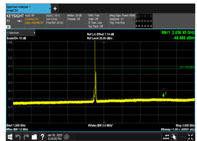
Band25-15MHz-QPSK-26615-1RB#0-1000~3000-PASS
