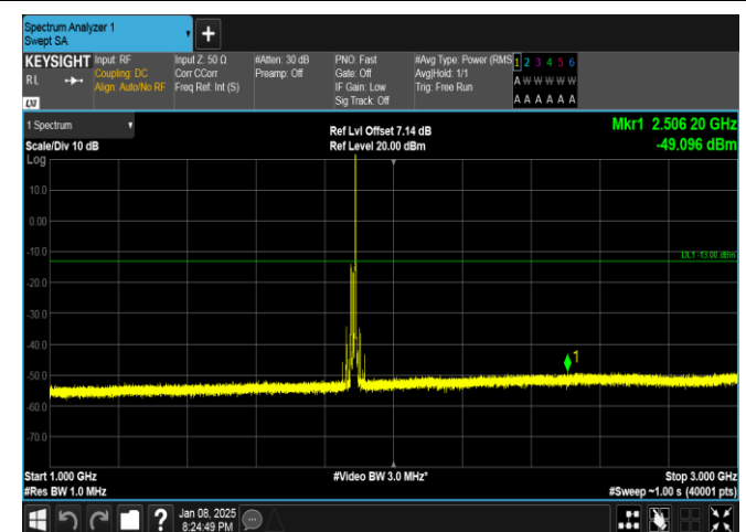
Band25-15MHz-QPSK-26365-1RB#74-1000~3000-PASS
