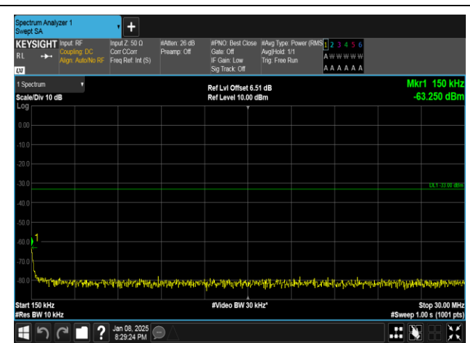
Band25-15MHz-QPSK-26615-1RB#0-0.15~30-PASS
