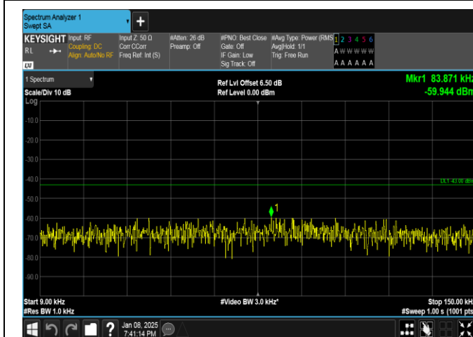
Band25-10MHz-QPSK-26640-50RB#0-0.009~0.15-PASS
