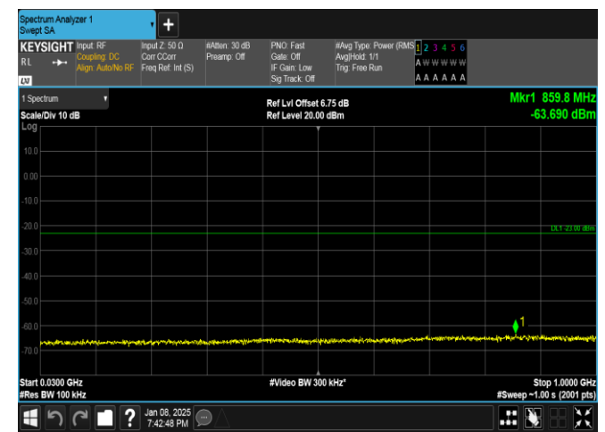
Band25-10MHz-16QAM-26640-50RB#0-30~1000-PASS
