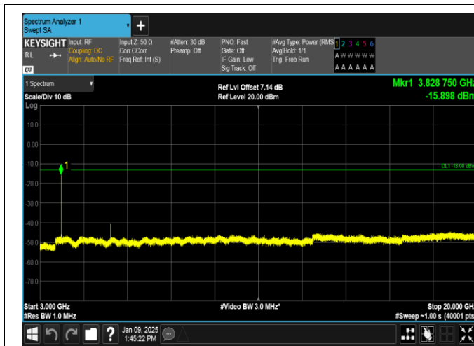
Band25-10MHz-16QAM-26640-1RB#49-3000~20000-PASS
