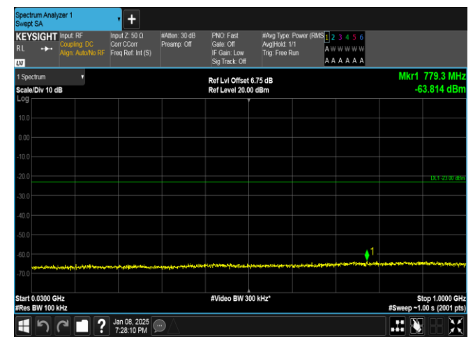
Band25-10MHz-16QAM-26090-50RB#0-30~1000-PASS
