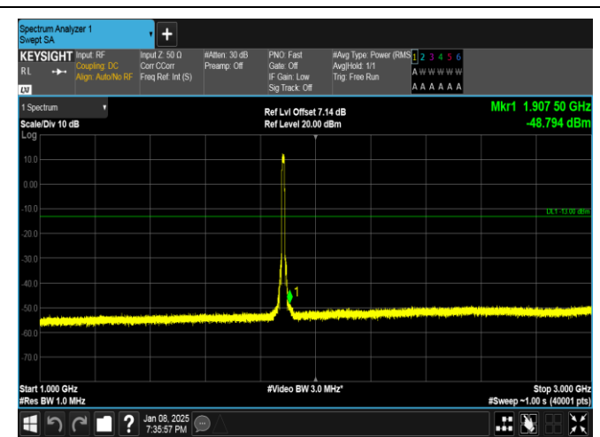
Band25-10MHz-16QAM-26365-50RB#0-1000~3000-PASS
