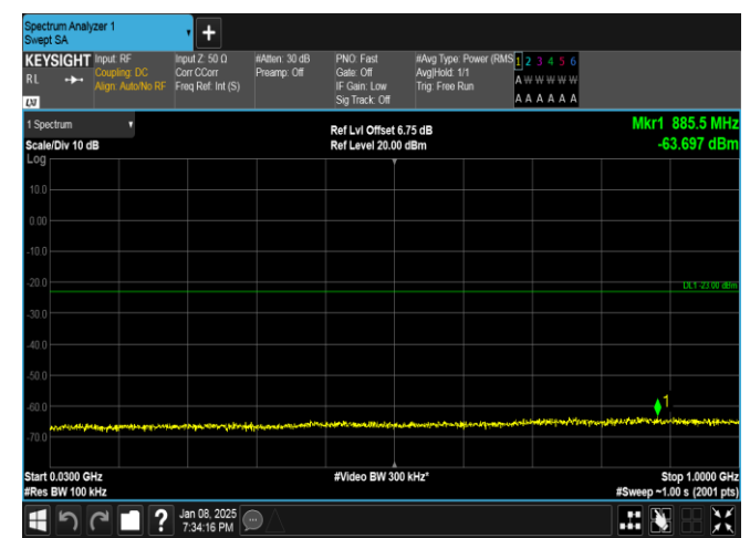
Band25-10MHz-QPSK-26365-50RB#0-30~1000-PASS
