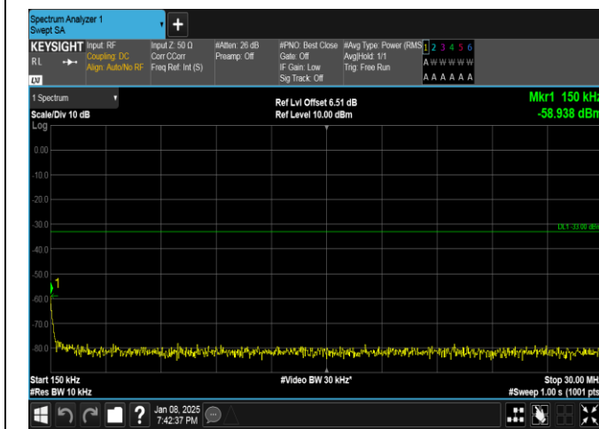
Band25-10MHz-16QAM-26640-50RB#0-0.15~30-PASS
