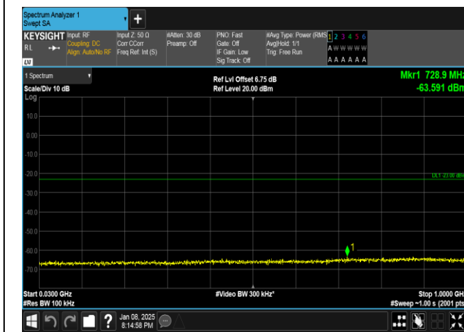
Band25-15MHz-QPSK-26115-1RB#0-30~1000-PASS
