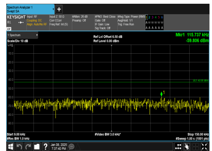
Band25-10MHz-16QAM-26640-1RB#0-0.009~0.15-PASS
