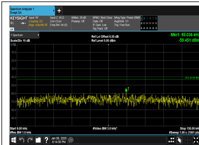
Band25-15MHz-QPSK-26115-1RB#0-0.009~0.15-PASS
