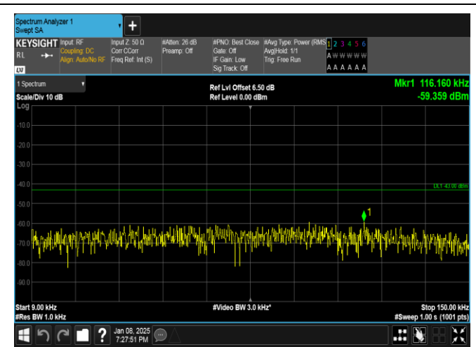
Band25-10MHz-16QAM-26090-50RB#0-0.009~0.15-PASS
