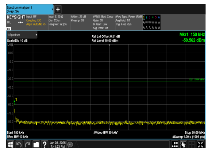
Band25-10MHz-QPSK-26640-50RB#0-0.15~30-PASS
