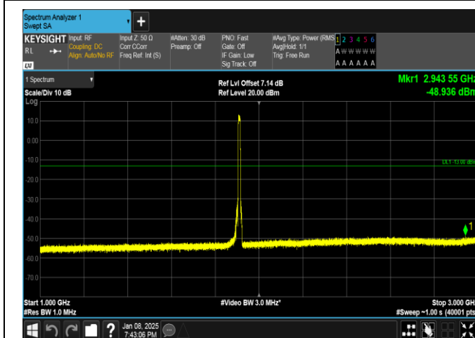
Band25-10MHz-16QAM-26640-50RB#0-1000~3000-PASS
