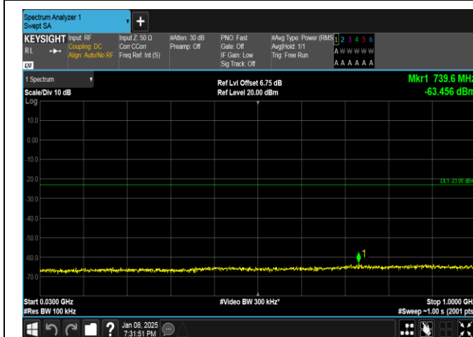
Band25-10MHz-QPSK-26365-1RB#49-30~1000-PASS
