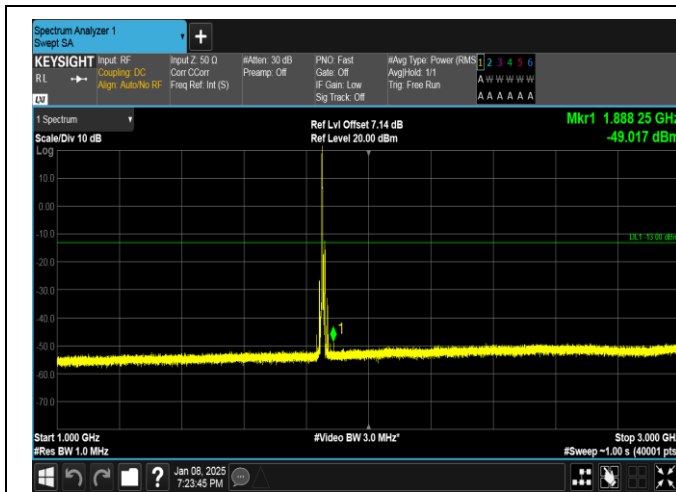
Band25-10MHz-16QAM-26090-1RB#0-1000~3000-PASS
