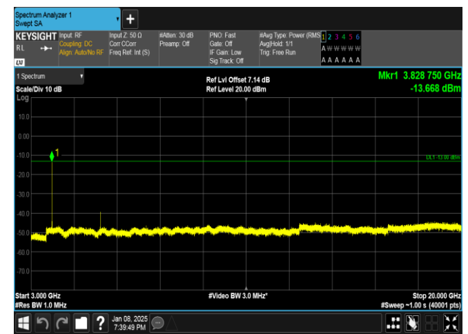
Band25-10MHz-QPSK-26640-1RB#49-3000~20000-PASS
