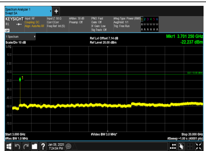
Band25-10MHz-16QAM-26090-1RB#0-3000~20000-PASS
