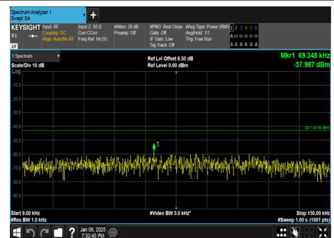
Band25-10MHz-16QAM-26365-1RB#49-0.009~0.15-PASS
