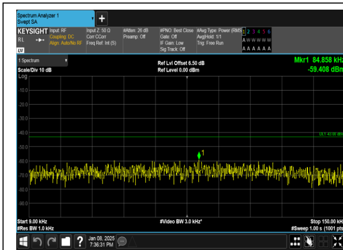
Band25-10MHz-QPSK-26640-1RB#0-0.009~0.15-PASS
