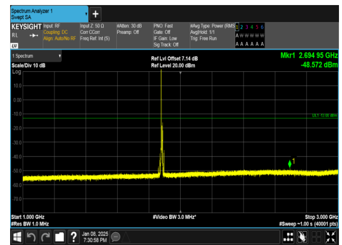
Band25-10MHz-16QAM-26365-1RB#0-1000~3000-PASS
