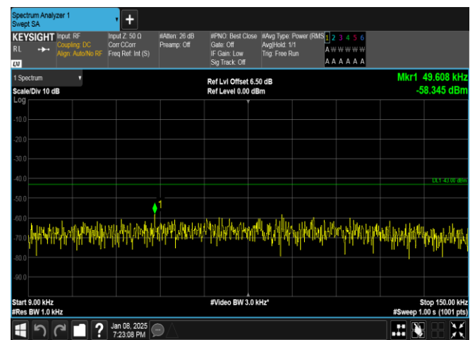
Band25-10MHz-16QAM-26090-1RB#0-0.009~0.15-PASS
