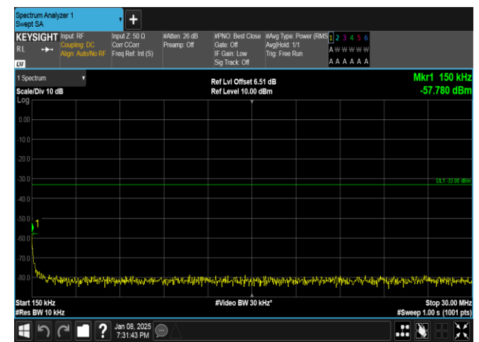
Band25-10MHz-QPSK-26365-1RB#49-0.15~30-PASS
