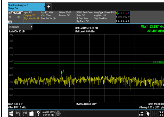
Band25-10MHz-16QAM-26090-1RB#49-0.009~0.15-PASS
