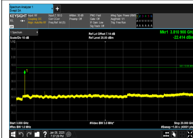
Band25-10MHz-QPSK-26640-1RB#0-3000~20000-PASS
