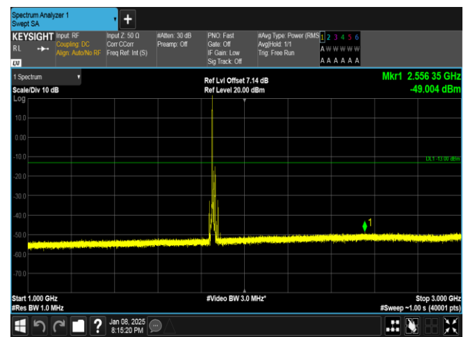
Band25-15MHz-QPSK-26115-1RB#0-1000~3000-PASS
