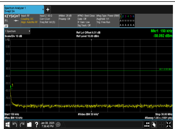
Band25-10MHz-QPSK-26640-1RB#0-0.15~30-PASS
