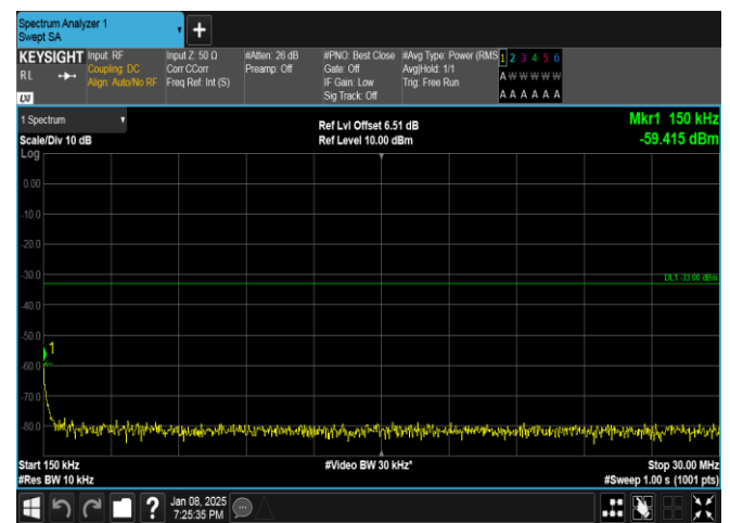
Band25-10MHz-16QAM-26090-1RB#49-0.15~30-PASS
