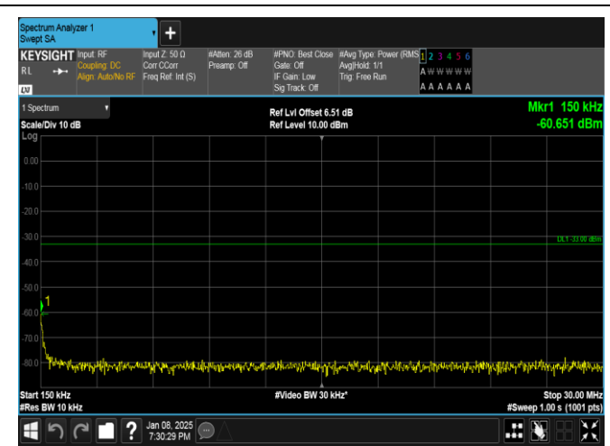
Band25-10MHz-16QAM-26365-1RB#0-0.15~30-PASS
