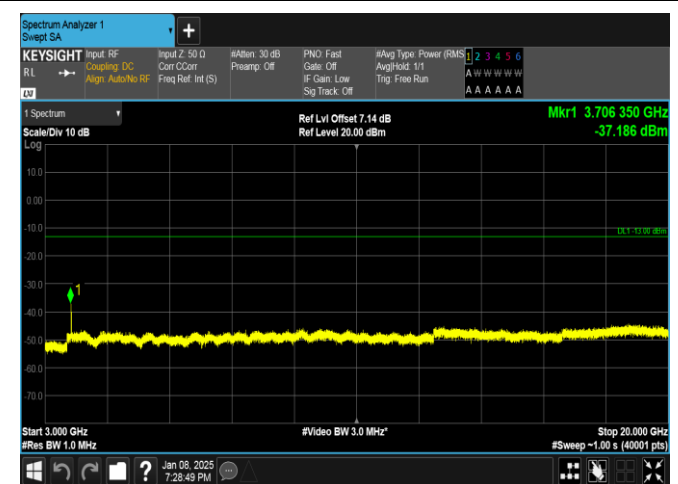
Band25-10MHz-16QAM-26090-50RB#0-3000~20000-PASS
