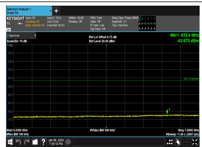
Band25-10MHz-QPSK-26640-1RB#49-30~1000-PASS
