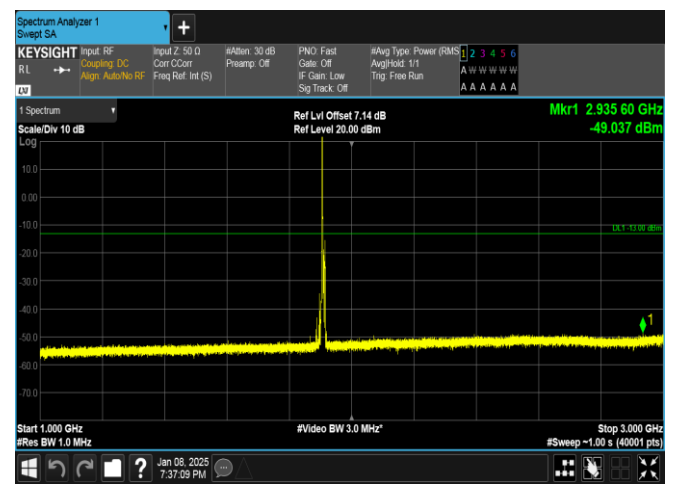
Band25-10MHz-QPSK-26640-1RB#0-1000~3000-PASS
