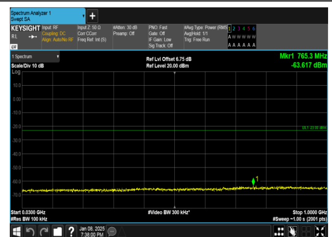
Band25-10MHz-16QAM-26640-1RB#0-30~1000-PASS
