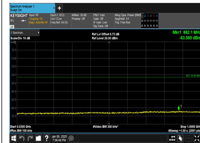
Band25-10MHz-QPSK-26640-1RB#0-30~1000-PASS
