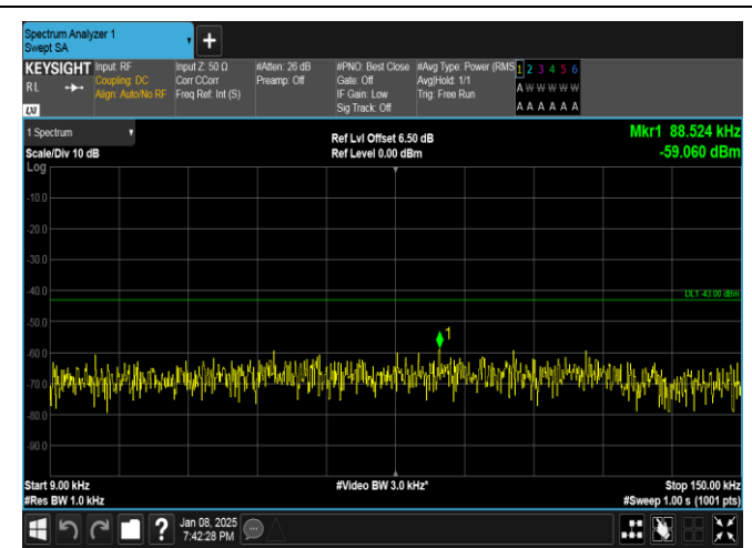
Band25-10MHz-16QAM-26640-50RB#0-0.009~0.15-PASS
