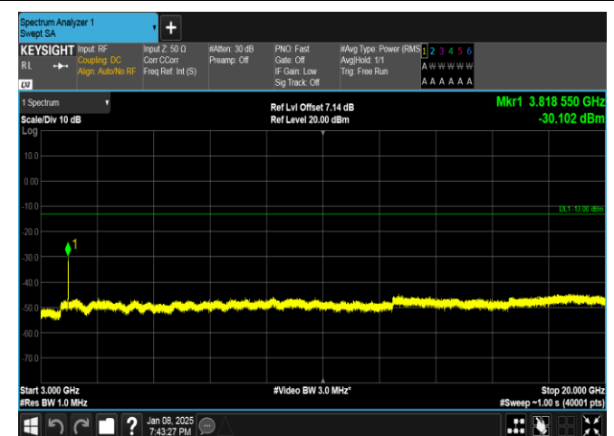
Band25-10MHz-16QAM-26640-50RB#0-3000~20000-PASS
