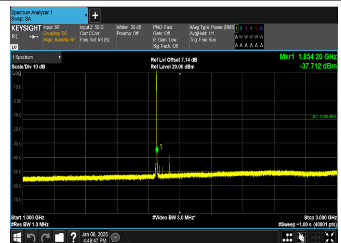
Band25-1.4MHz-16QAM-26047-1RB#5-1000~3000-PASS
