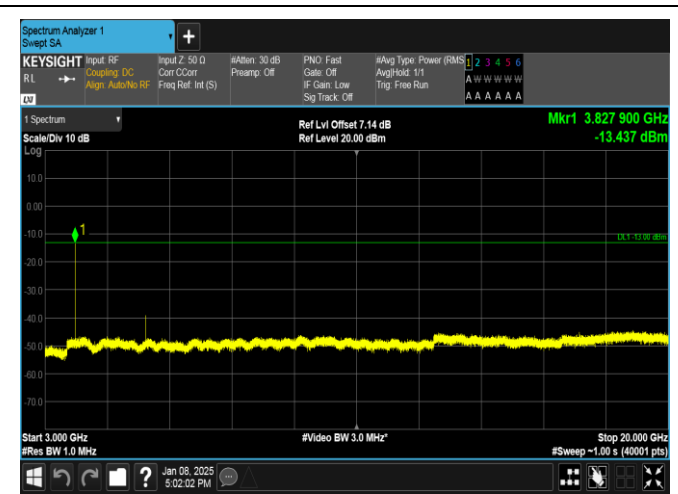
Band25-1.4MHz-16QAM-26683-1RB#0-3000~20000-PASS
