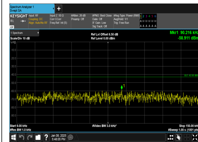
Band25-3MHz-QPSK-26365-1RB#14-0.009~0.15-PASS
