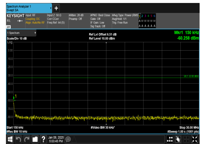
Band25-1.4MHz-16QAM-26683-1RB#5-0.15~30-PASS
