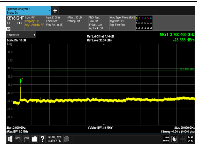
Band25-1.4MHz-16QAM-26047-1RB#0-3000~20000-PASS
