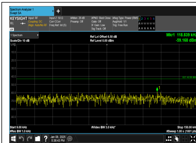
Band25-3MHz-QPSK-26055-1RB#0-0.009~0.15-PASS
