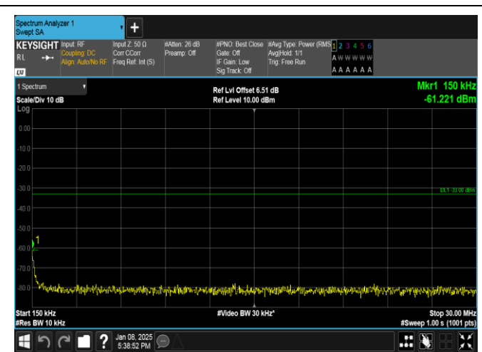
Band25-3MHz-QPSK-26055-1RB#0-0.15~30-PASS
