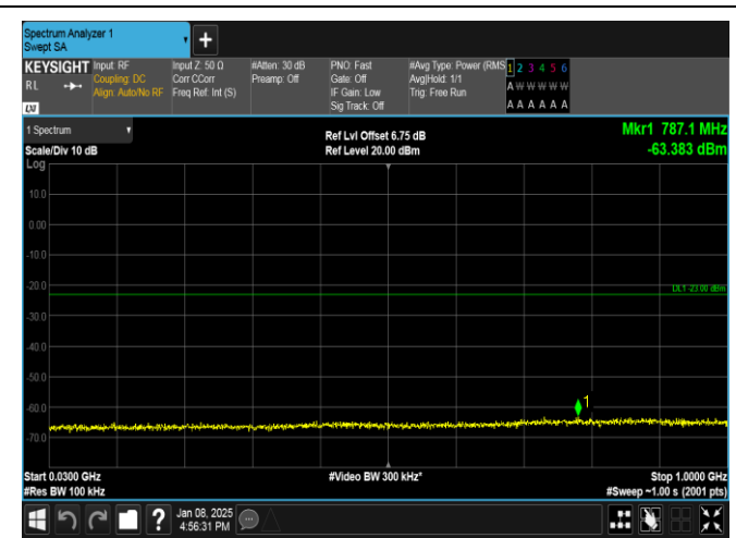
Band25-1.4MHz-16QAM-26365-1RB#5-30~1000-PASS
