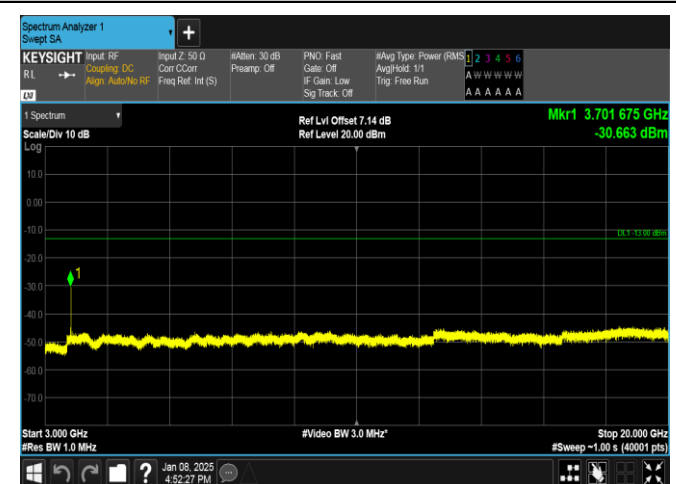
Band25-1.4MHz-16QAM-26047-6RB#0-3000~20000-PASS
