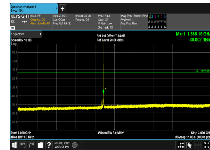
Band25-1.4MHz-16QAM-26365-1RB#5-1000~3000-PASS
