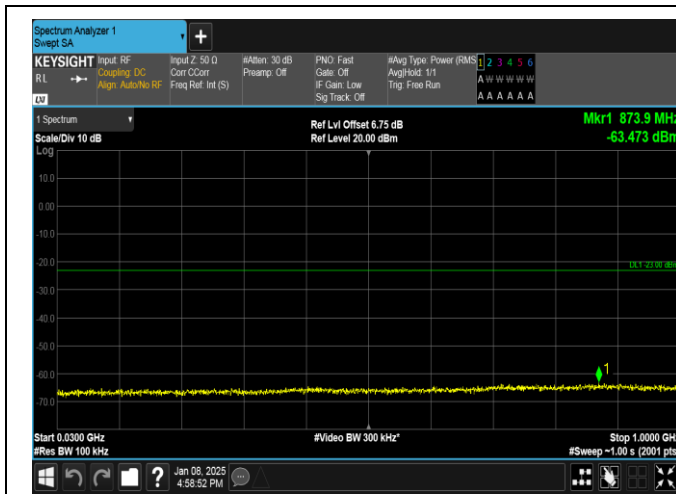
Band25-1.4MHz-16QAM-26365-6RB#0-30~1000-PASS
