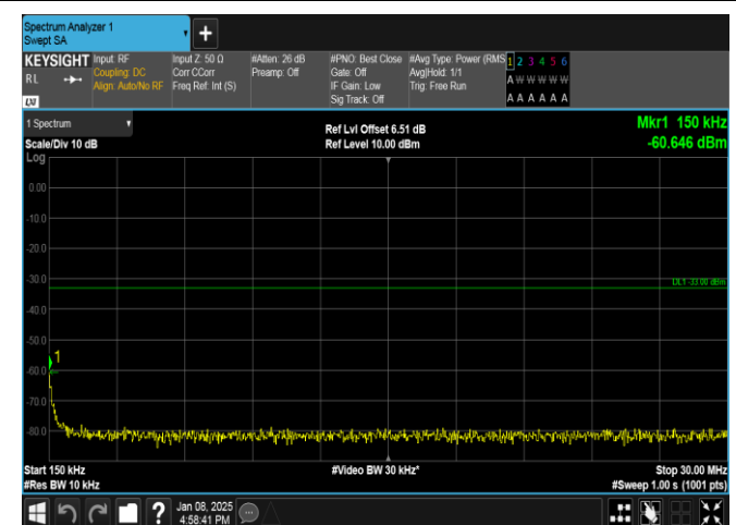
Band25-1.4MHz-16QAM-26365-6RB#0-0.15~30-PASS
