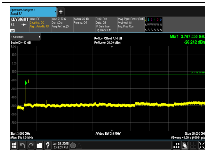
Band25-3MHz-QPSK-26365-1RB#14-3000~20000-PASS
