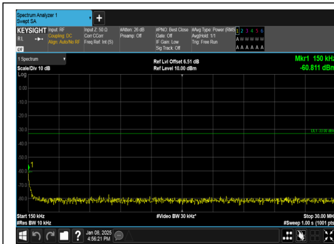
Band25-1.4MHz-16QAM-26365-1RB#5-0.15~30-PASS
