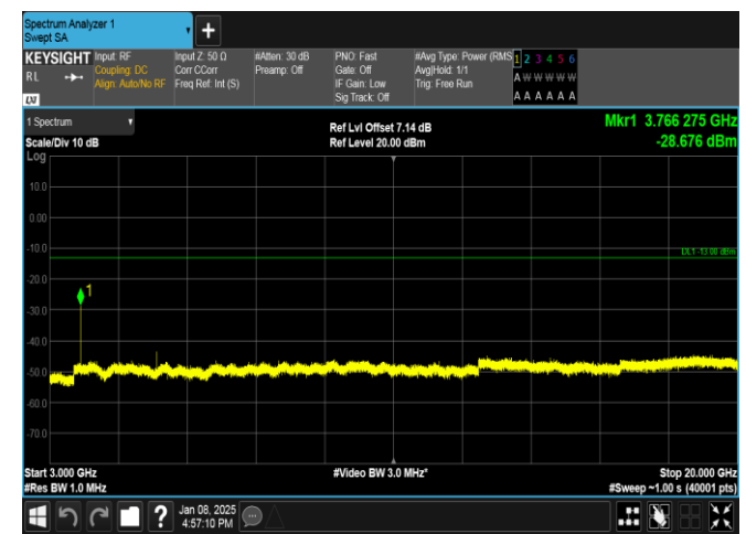
Band25-1.4MHz-16QAM-26365-1RB#5-3000~20000-PASS
