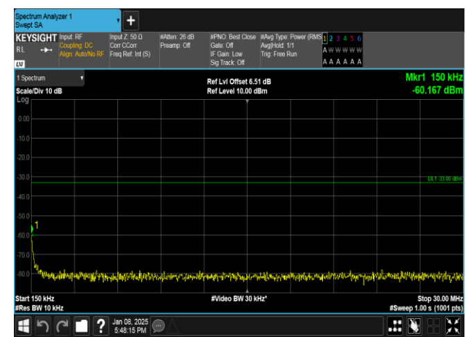
Band25-3MHz-QPSK-26365-1RB#14-0.15~30-PASS
