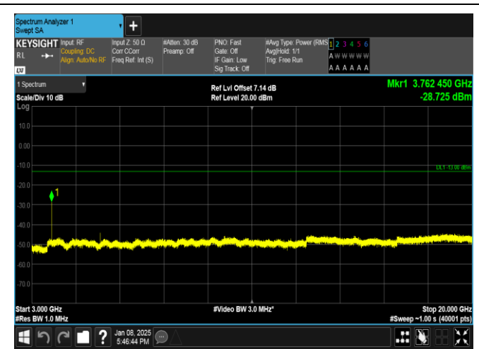
Band25-3MHz-QPSK-26365-1RB#0-3000~20000-PASS
