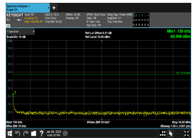
Band25-1.4MHz-16QAM-26047-1RB#5-0.15~30-PASS
