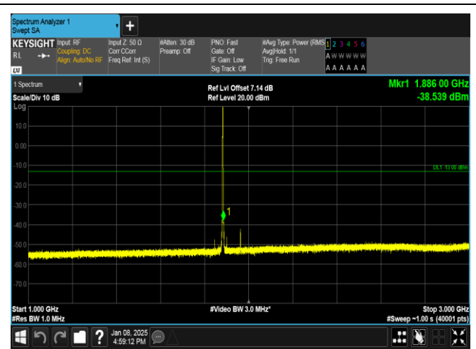
Band25-1.4MHz-16QAM-26365-6RB#0-1000~3000-PASS
