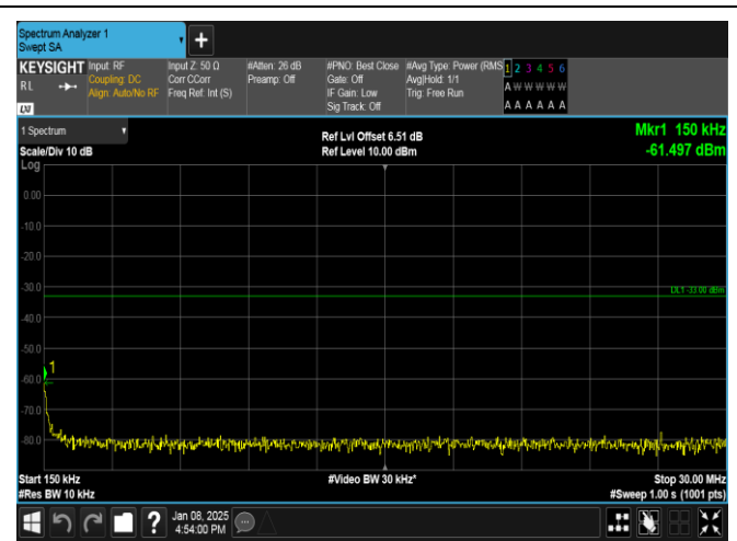
Band25-1.4MHz-16QAM-26365-1RB#0-0.15~30-PASS
