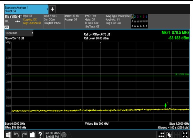
Band25-3MHz-QPSK-26365-1RB#0-30~1000-PASS
