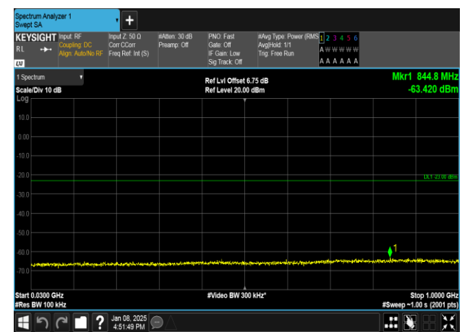
Band25-1.4MHz-16QAM-26047-6RB#0-30~1000-PASS
