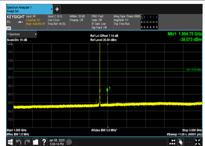
Band25-1.4MHz-16QAM-26683-1RB#5-1000~3000-PASS
