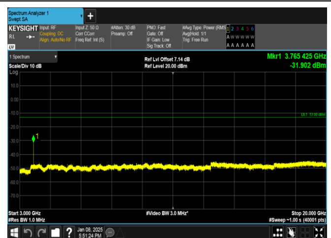
Band25-3MHz-QPSK-26365-15RB#0-3000~20000-PASS
