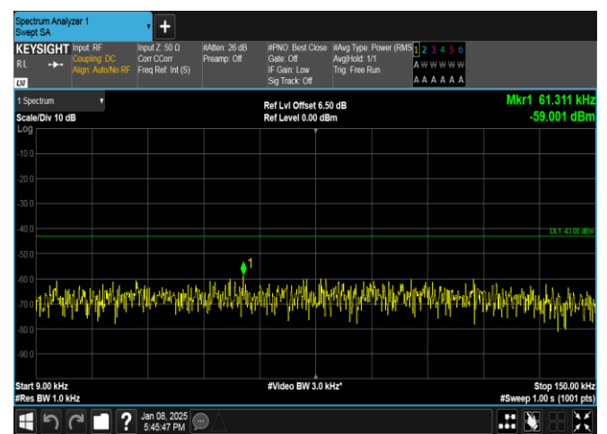
Band25-3MHz-QPSK-26365-1RB#0-0.009~0.15-PASS
