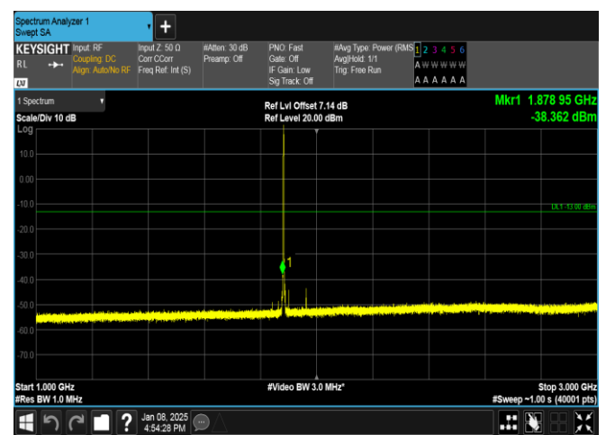
Band25-1.4MHz-16QAM-26365-1RB#0-1000~3000-PASS
