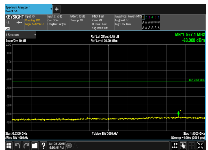
Band25-3MHz-QPSK-26365-15RB#0-30~1000-PASS
