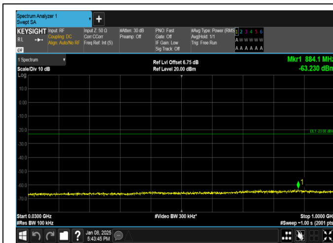
Band25-3MHz-QPSK-26055-15RB#0-30~1000-PASS
