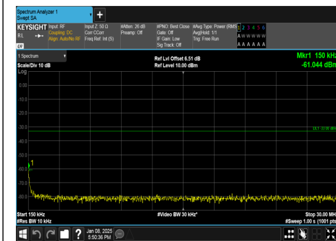
Band25-3MHz-QPSK-26365-15RB#0-0.15~30-PASS
