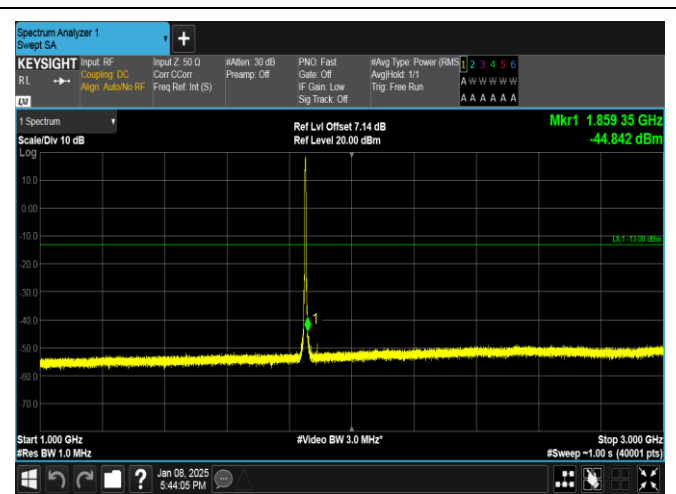
Band25-3MHz-QPSK-26055-15RB#0-1000~3000-PASS
