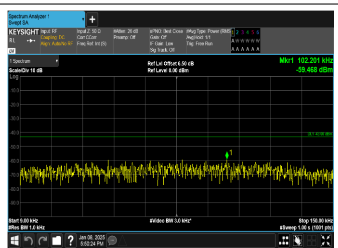
Band25-3MHz-QPSK-26365-15RB#0-0.009~0.15-PASS
