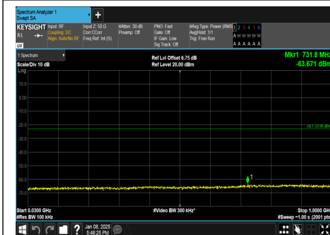
Band25-3MHz-QPSK-26365-1RB#14-30~1000-PASS
