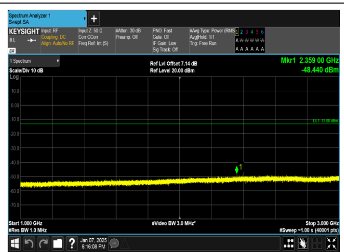
Band13-10MHz-16QAM-23230-1RB#49-1000~3000-PASS
