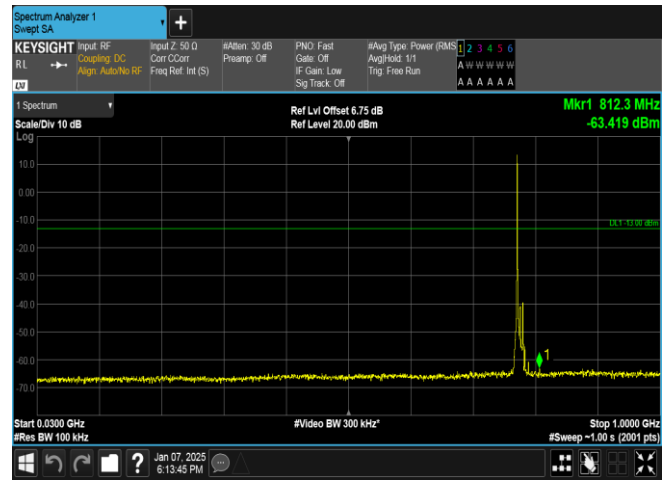
Band13-10MHz-16QAM-23230-1RB#0-30~1000-PASS
