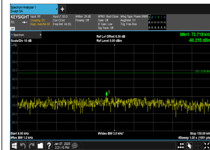
Band12-1.4MHz-QPSK-23017-6RB#0-0.009~0.15-PASS
