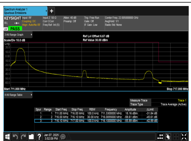
Band12-5MHz-QPSK-23155-1RB#0-PASS
