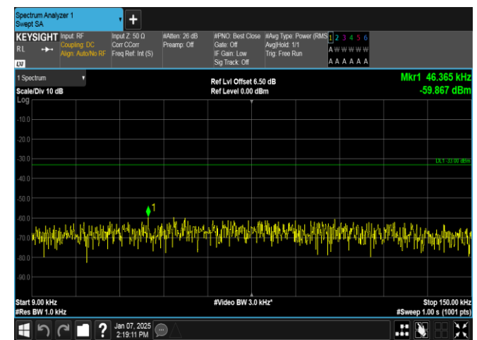
Band12-1.4MHz-QPSK-23017-1RB#5-0.009~0.15-PASS
