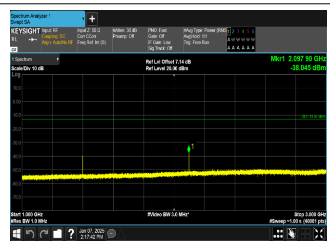
Band12-1.4MHz-QPSK-23017-1RB#0-1000~3000-PASS
