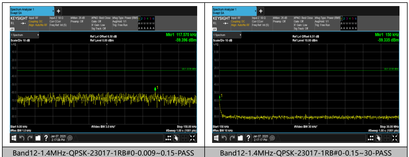
Band12-1.4MHz-QPSK-23017-1RB#0-0.009~0.15-PASS
