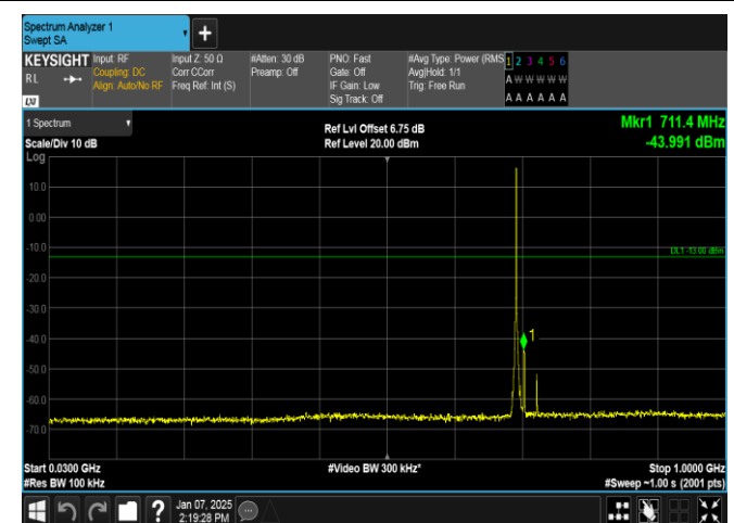
Band12-1.4MHz-QPSK-23017-1RB#5-30~1000-PASS
