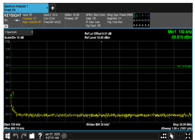
Band5-1.4MHz-QPSK-20643-6RB#0-0.15~30-PASS
