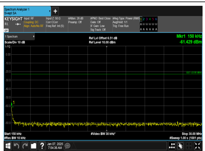
Band5-1.4MHz-16QAM-20407-1RB#5-0.15~30-PASS
