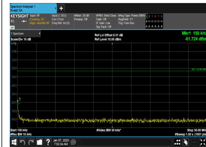
Band5-1.4MHz-16QAM-20407-1RB#0-0.15~30-PASS
