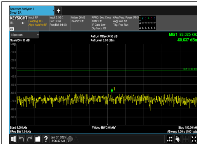
Band5-1.4MHz-16QAM-20643-1RB#5-0.009~0.15-PASS
