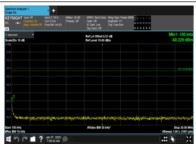
Band5-1.4MHz-QPSK-20525-1RB#5-0.15~30-PASS
