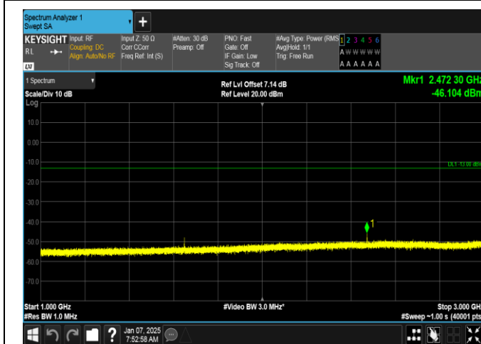
Band5-1.4MHz-16QAM-20407-1RB#0-1000~3000-PASS
