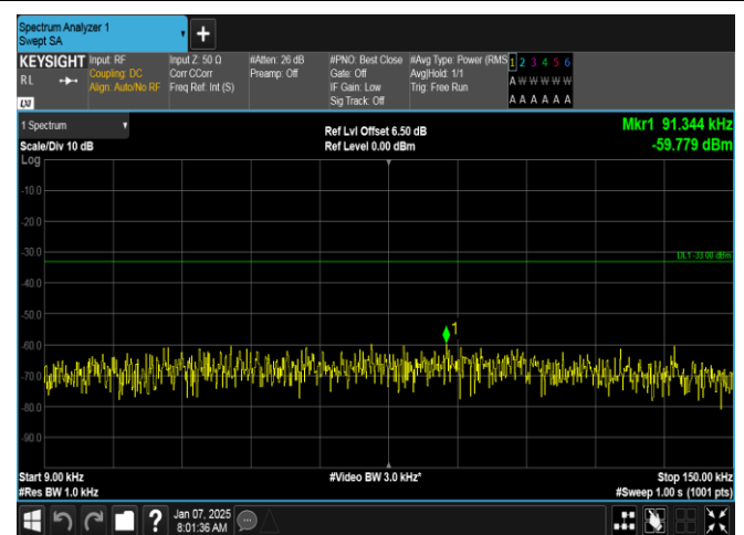
Band5-1.4MHz-QPSK-20525-6RB#0-0.009~0.15-PASS
