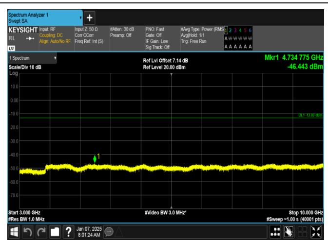
Band5-1.4MHz-16QAM-20525-1RB#5-3000~10000-PASS
