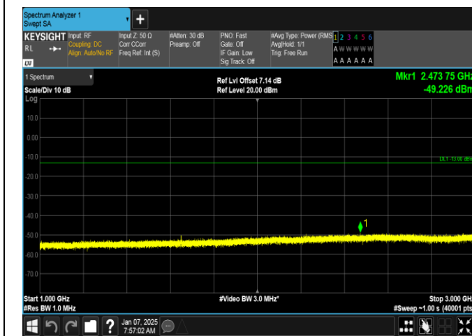
Band5-1.4MHz-16QAM-20407-6RB#0-1000~3000-PASS
