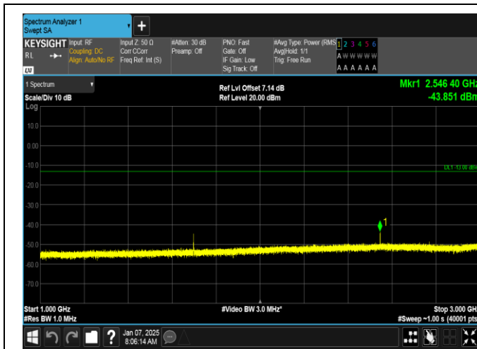
Band5-1.4MHz-QPSK-20643-1RB#5-1000~3000-PASS
