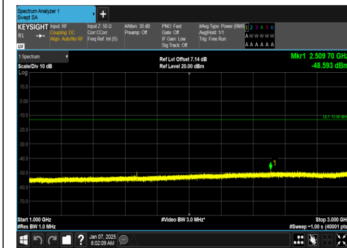
Band5-1.4MHz-QPSK-20525-6RB#0-1000~3000-PASS
