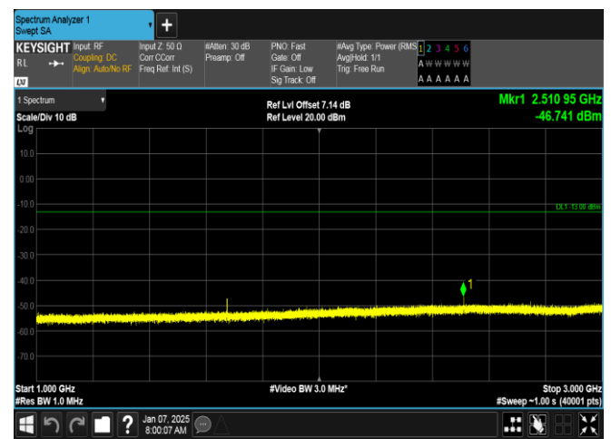
Band5-1.4MHz-QPSK-20525-1RB#5-1000~3000-PASS
