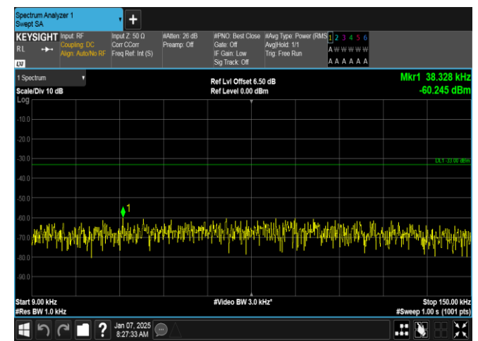
Band5-3MHz-QPSK-20415-1RB#14-0.009~0.15-PASS
