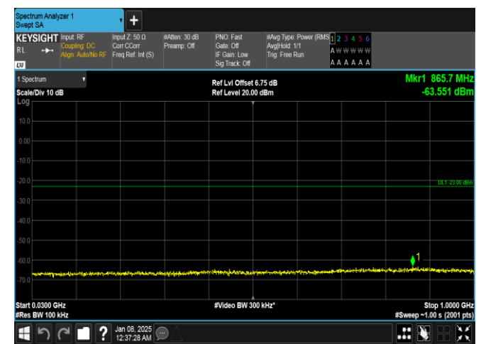
Band4-20MHz-16QAM-20300-1RB#0-30~1000-PASS
