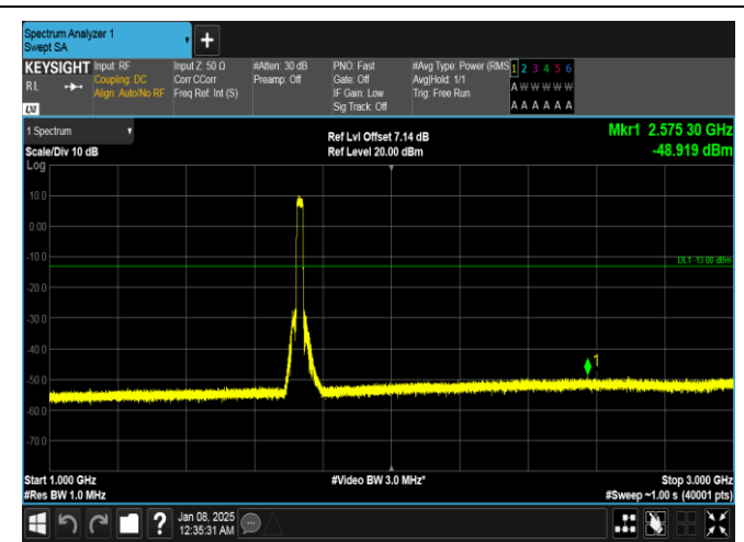
Band4-20MHz-16QAM-20175-100RB#0-1000~3000-PASS
