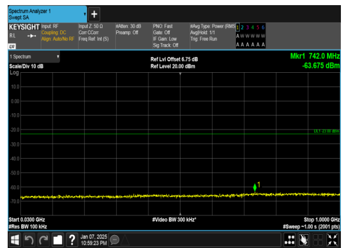
Band4-10MHz-16QAM-20350-50RB#0-30~1000-PASS
