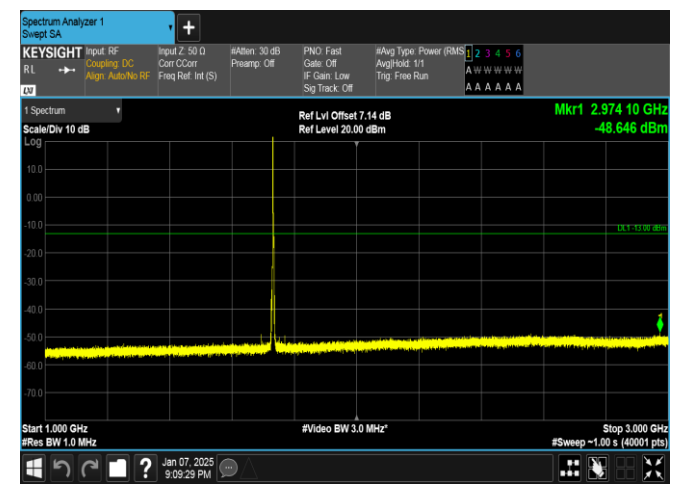
Band4-3MHz-16QAM-20175-1RB#0-1000~3000-PASS
