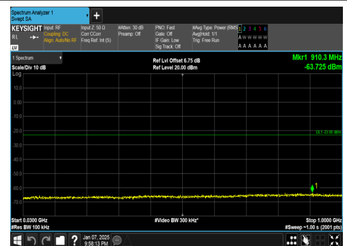
Band4-5MHz-QPSK-20175-1RB#0-30~1000-PASS
