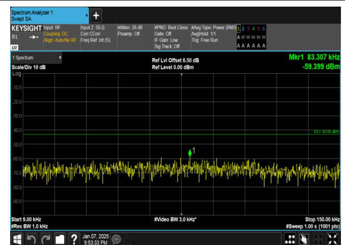
Band4-5MHz-QPSK-19975-1RB#24-0.009~0.15-PASS
