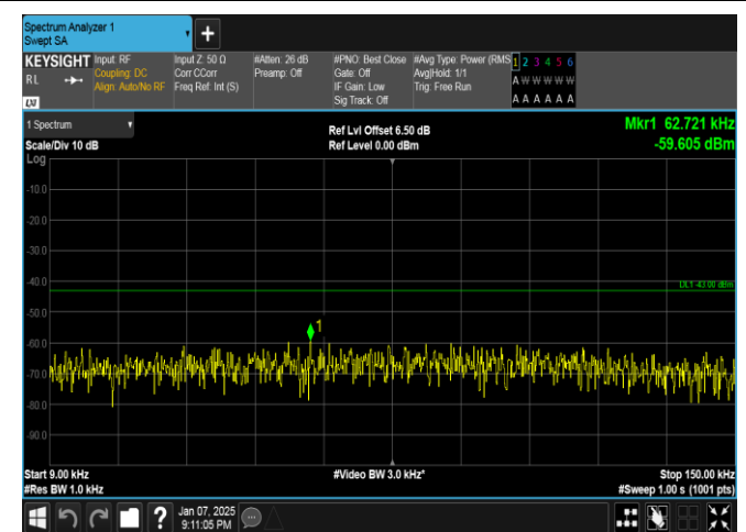
Band4-3MHz-16QAM-20175-1RB#14-0.009~0.15-PASS
