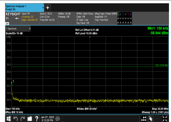
Band4-3MHz-16QAM-20175-15RB#0-0.15~30-PASS
