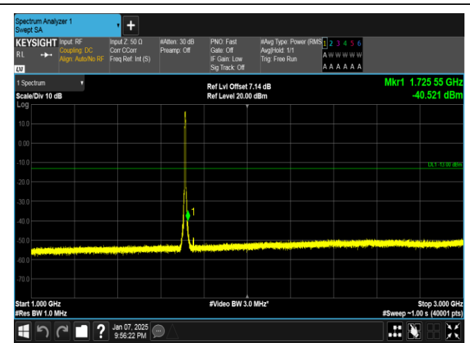
Band4-5MHz-QPSK-19975-25RB#0-1000~3000-PASS
