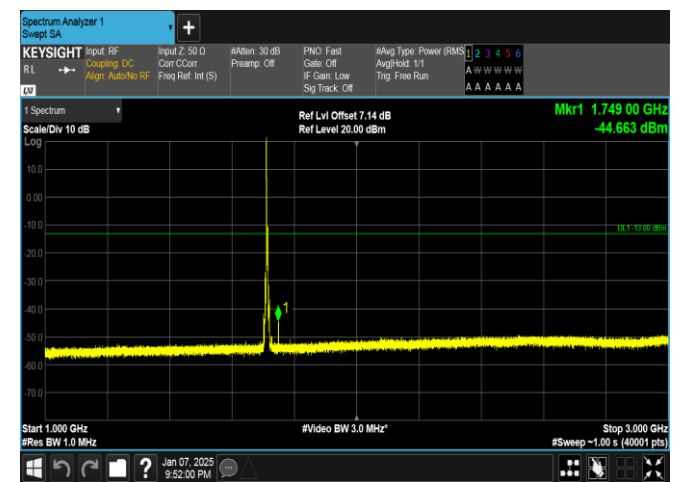
Band4-5MHz-QPSK-19975-1RB#0-1000~3000-PASS
