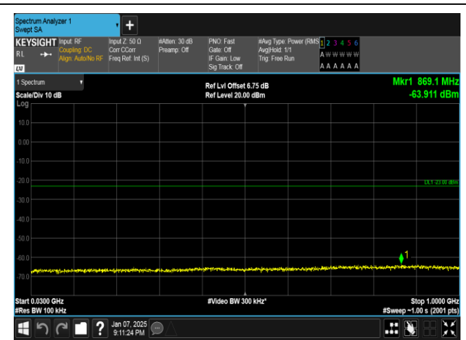
Band4-3MHz-16QAM-20175-1RB#14-30~1000-PASS
