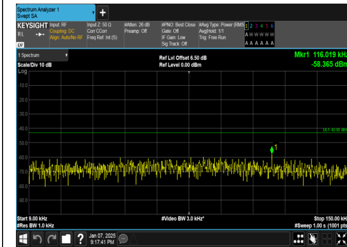
Band4-3MHz-16QAM-20385-1RB#14-0.009~0.15-PASS
