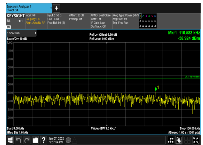
Band4-5MHz-QPSK-20175-1RB#0-0.009~0.15-PASS
