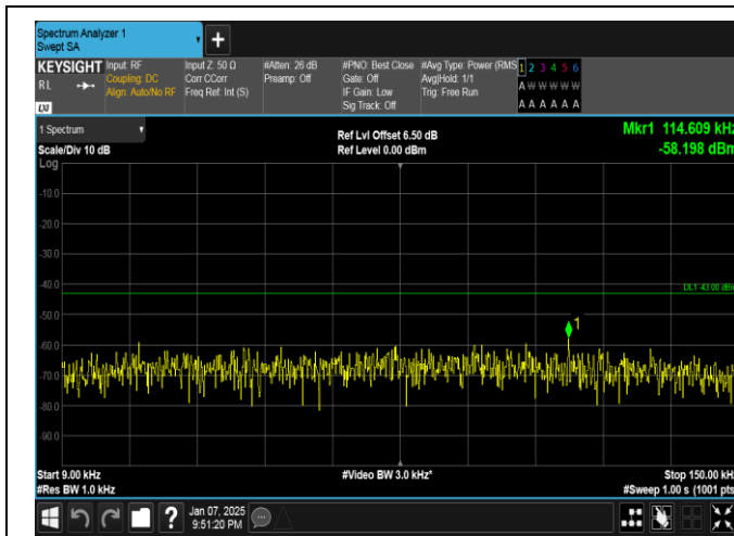
Band4-5MHz-QPSK-19975-1RB#0-0.009~0.15-PASS
