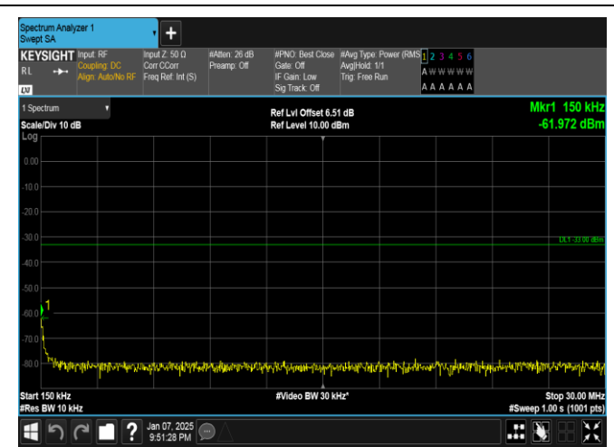
Band4-5MHz-QPSK-19975-1RB#0-0.15~30-PASS
