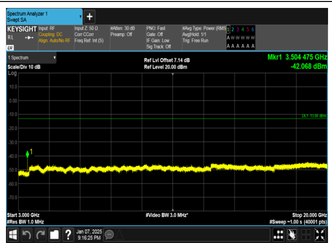
Band4-3MHz-16QAM-20385-1RB#0-3000~20000-PASS
