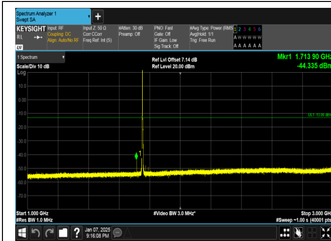
Band4-3MHz-16QAM-20385-1RB#0-1000~3000-PASS
