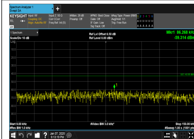
Band4-3MHz-16QAM-20175-15RB#0-0.009~0.15-PASS
