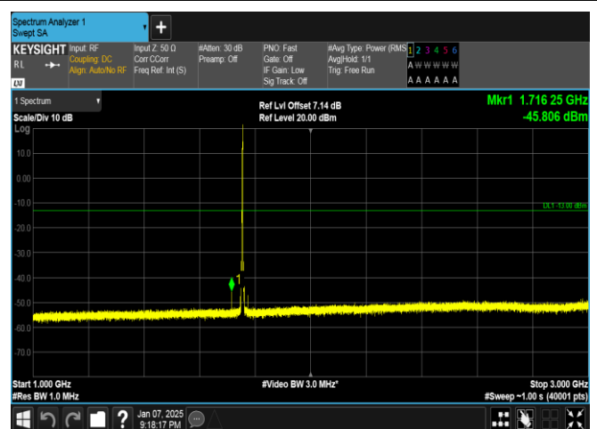
Band4-3MHz-16QAM-20385-1RB#14-1000~3000-PASS
