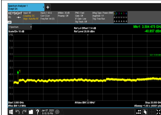
Band4-3MHz-QPSK-20385-1RB#0-3000~20000-PASS
