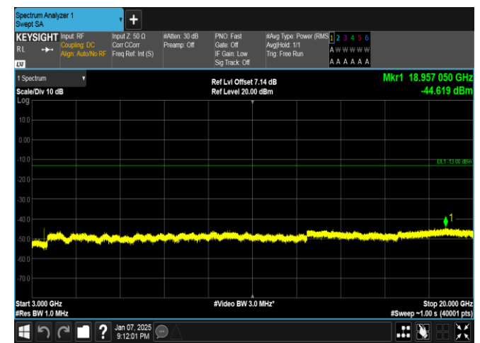
Band4-3MHz-16QAM-20175-1RB#14-3000~20000-PASS
