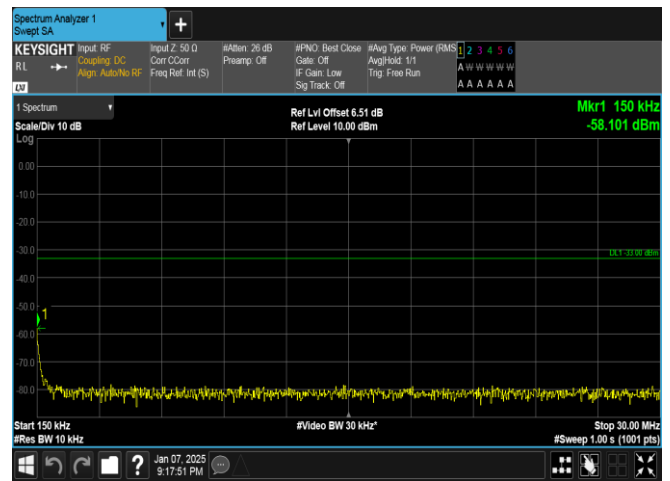
Band4-3MHz-16QAM-20385-1RB#14-0.15~30-PASS
