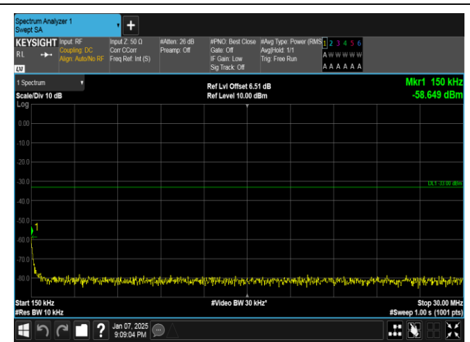
Band4-3MHz-16QAM-20175-1RB#0-0.15~30-PASS
