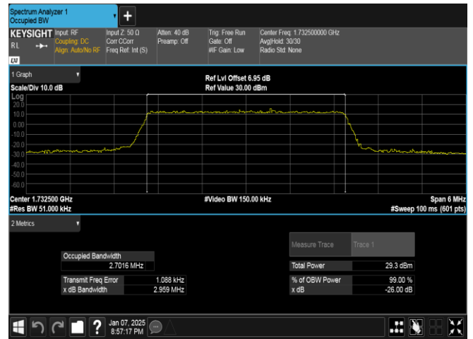
Band4-3MHz-QPSK-20175-15RB#0-PASS
