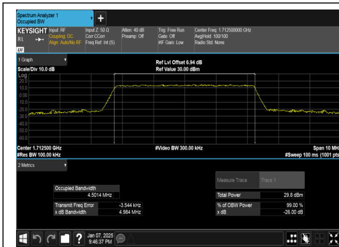
Band4-5MHz-QPSK-19975-25RB#0-PASS
