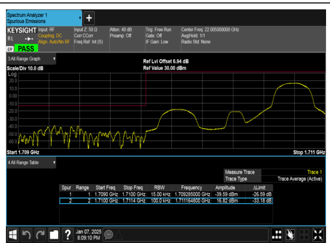
Band4-1.4MHz-16QAM-19957-1RB#5-PASS
