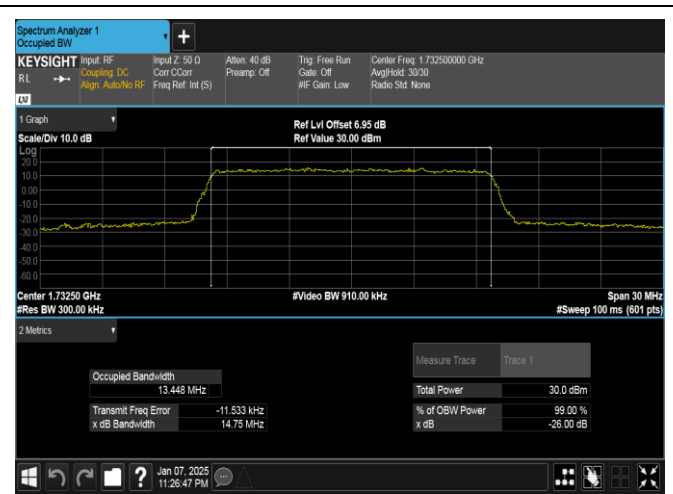
Band4-15MHz-QPSK-20175-75RB#0-PASS
