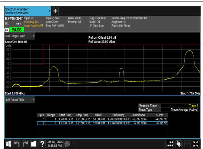
Band4-5MHz-QPSK-19975-1RB#24-PASS
