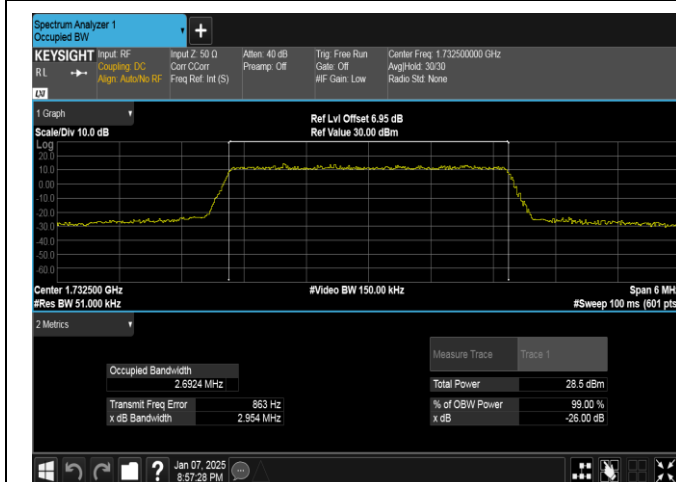
Band4-3MHz-16QAM-20175-15RB#0-PASS
