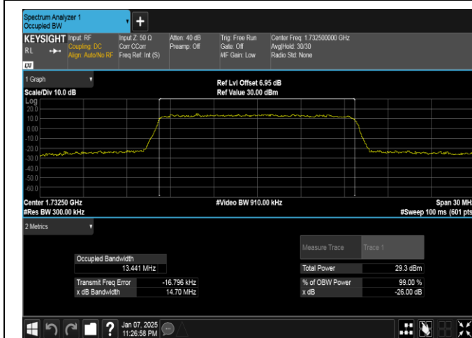
Band4-15MHz-16QAM-20175-75RB#0-PASS
