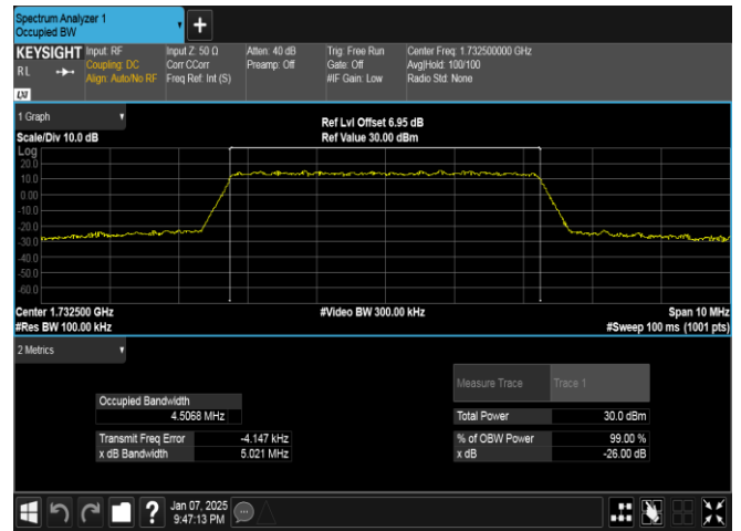
Band4-5MHz-QPSK-20175-25RB#0-PASS
