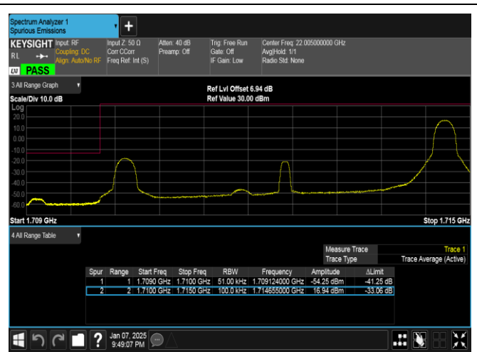
Band4-5MHz-16QAM-19975-1RB#24-PASS
