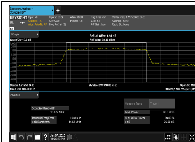
Band4-15MHz-QPSK-2025-75RB#0-PASS
