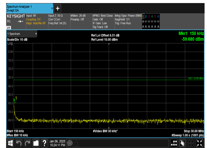
Band2-15MHz-16QAM-18675-1RB#74-0.15~30-PASS
