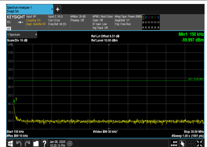
Band2-15MHz-QPSK-18675-75RB#0-0.15~30-PASS
