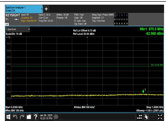
Band2-15MHz-QPSK-18675-1RB#74-30~1000-PASS
