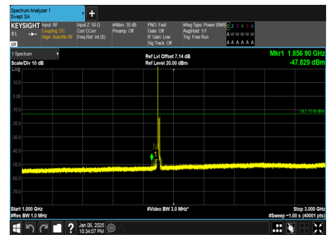
Band2-15MHz-QPSK-19125-1RB#0-1000~3000-PASS
