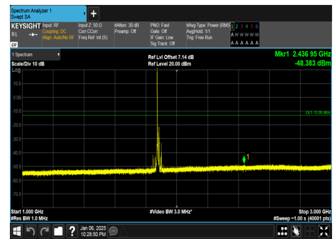
Band2-15MHz-16QAM-18900-1RB#0-1000~3000-PASS
