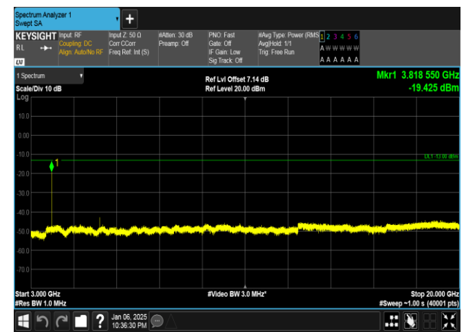
Band2-15MHz-QPSK-19125-1RB#74-3000~20000-PASS
