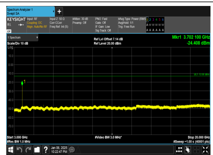
Band2-15MHz-16QAM-18675-1RB#0-3000~20000-PASS
