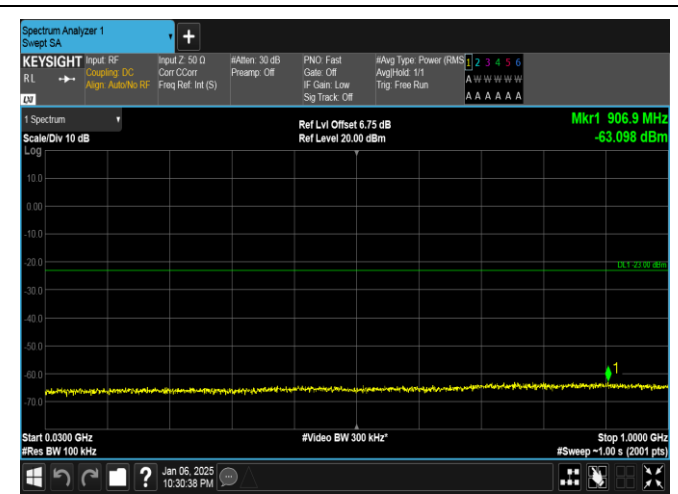
Band2-15MHz-16QAM-18900-1RB#74-30~1000-PASS
