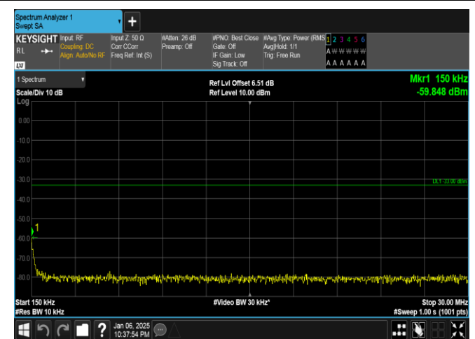
Band2-15MHz-QPSK-19125-75RB#0-0.15~30-PASS
