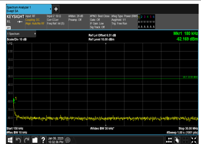
Band2-15MHz-16QAM-18900-75RB#0-0.15~30-PASS
