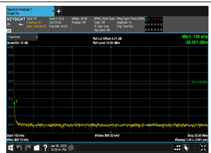
Band2-15MHz-QPSK-19125-1RB#0-0.15~30-PASS
