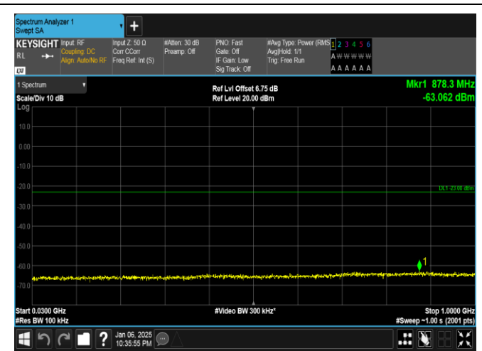
Band2-15MHz-QPSK-19125-1RB#74-30~1000-PASS
