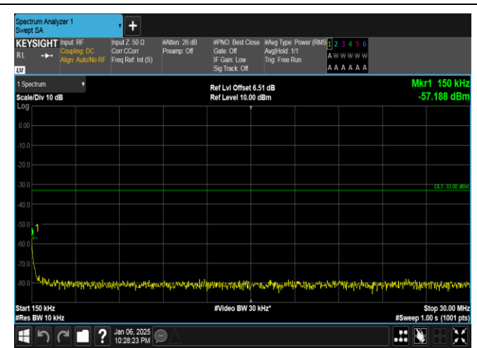
Band2-15MHz-16QAM-18900-1RB#0-0.15~30-PASS
