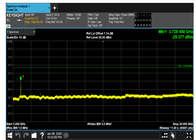
Band2-15MHz-QPSK-18675-1RB#74-3000~20000-PASS
