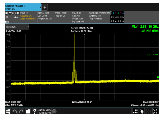
Band2-15MHz-16QAM-18675-1RB#74-1000~3000-PASS
