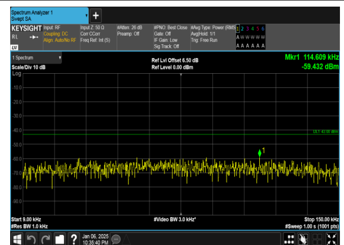
Band2-15MHz-QPSK-19125-1RB#74-0.009~0.15-PASS
