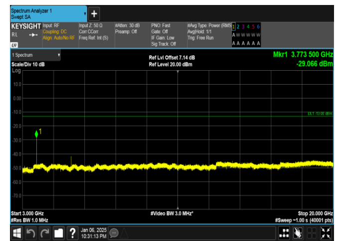
Band2-15MHz-16QAM-18900-1RB#74-3000~20000-PASS
