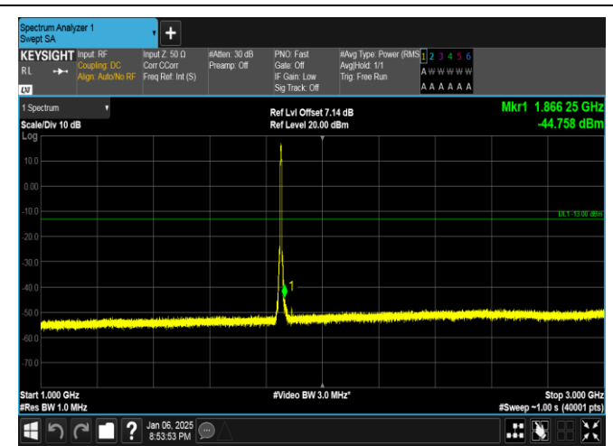
Band2-5MHz-QPSK-18625-25RB#0-1000~3000-PASS
