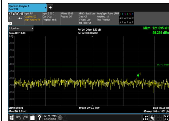
Band2-5MHz-QPSK-18625-25RB#0-0.009~0.15-PASS
