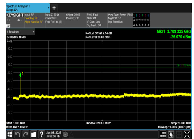
Band2-5MHz-QPSK-18625-1RB#24-3000~20000-PASS
