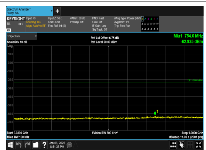
Band2-5MHz-QPSK-18625-1RB#24-30~1000-PASS
