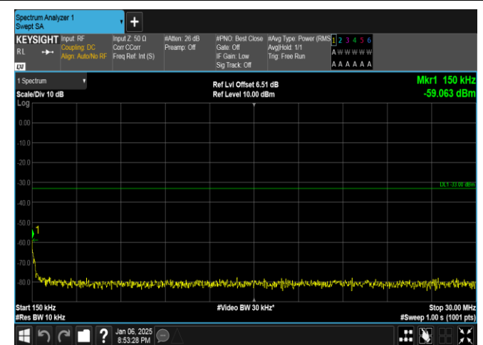
Band2-5MHz-QPSK-18625-25RB#0-0.15~30-PASS
