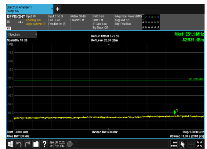
Band2-3MHz-16QAM-18615-15RB#0-30~1000-PASS
