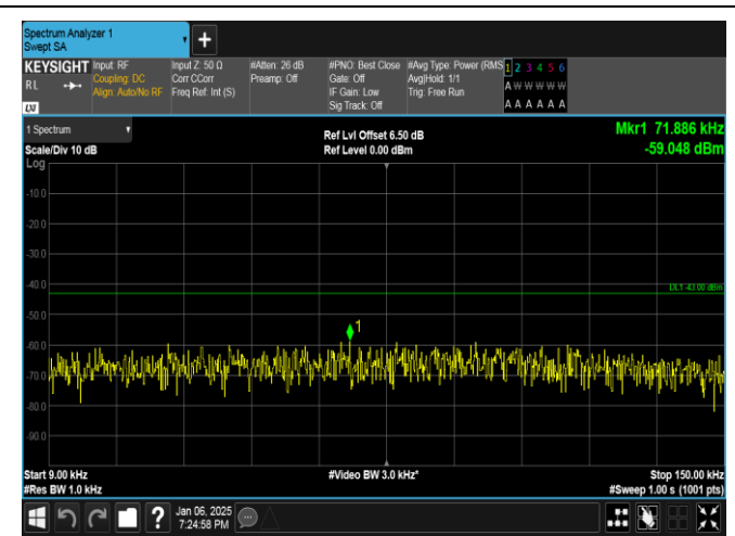
Band2-1.4MHz-QPSK-18900-6RB#0-0.009~0.15-PASS
