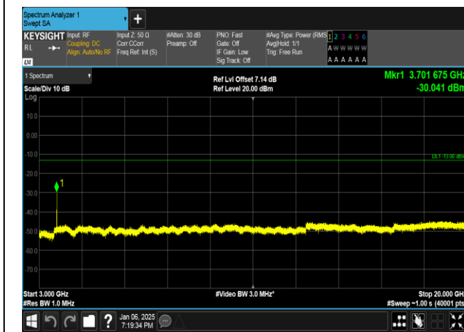
Band2-1.4MHz-QPSK-18607-6RB#0-3000~20000-PASS
