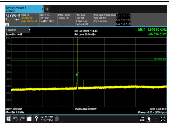
Band2-1.4MHz-QPSK-18607-6RB#0-1000~3000-PASS
