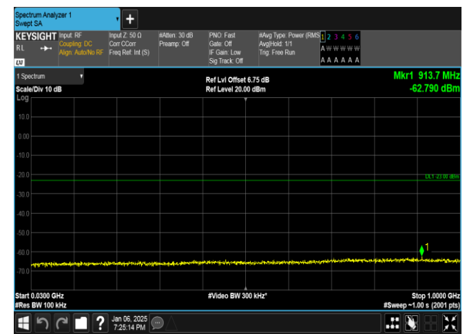
Band2-1.4MHz-QPSK-18900-6RB#0-30~1000-PASS
