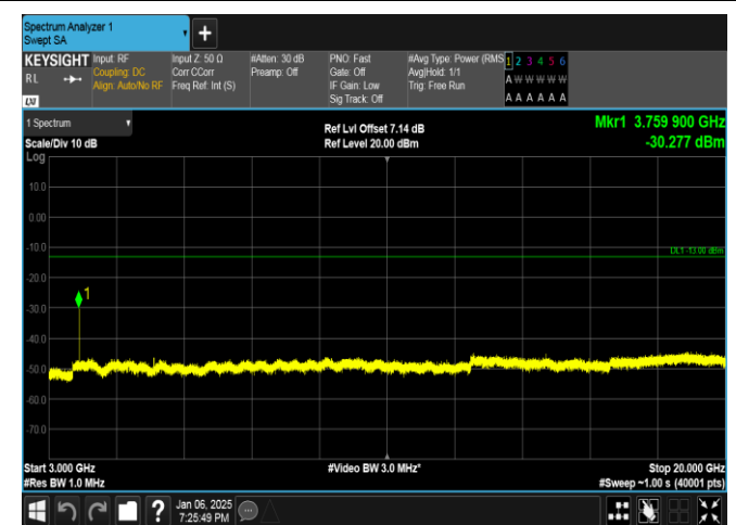
Band2-1.4MHz-QPSK-18900-6RB#0-3000~20000-PASS
