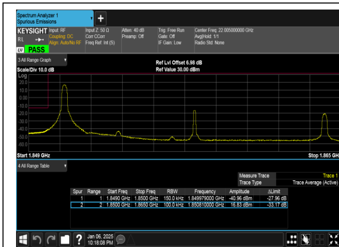
Band2-15MHz-16QAM-18675-1RB#0-PASS
