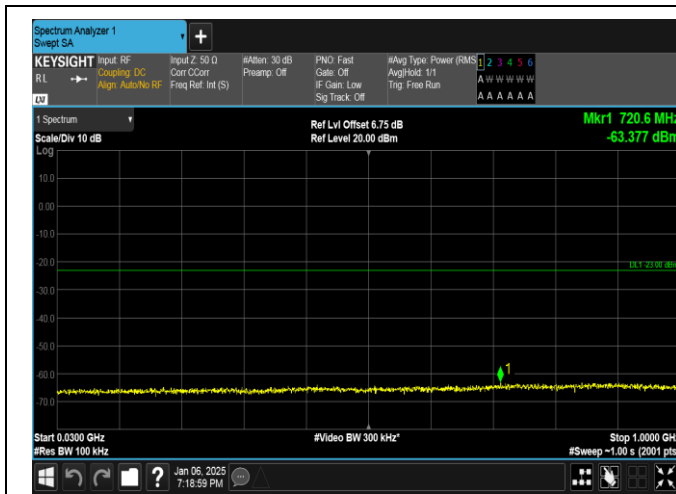
Band2-1.4MHz-QPSK-18607-6RB#0-30~1000-PASS
