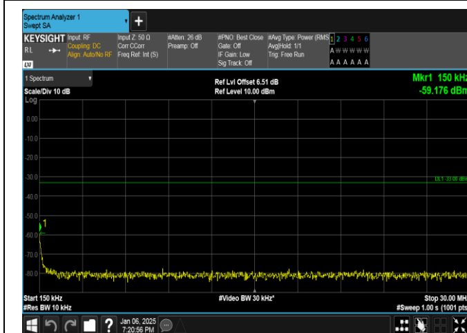
Band2-1.4MHz-QPSK-18900-1RB#0-0.15~30-PASS
