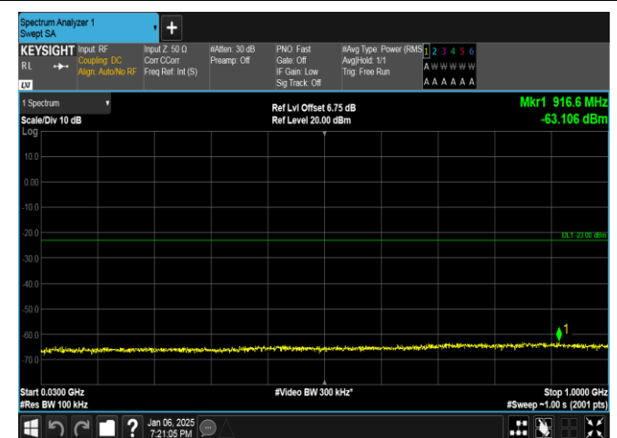
Band2-1.4MHz-QPSK-18900-1RB#0-30~1000-PASS
