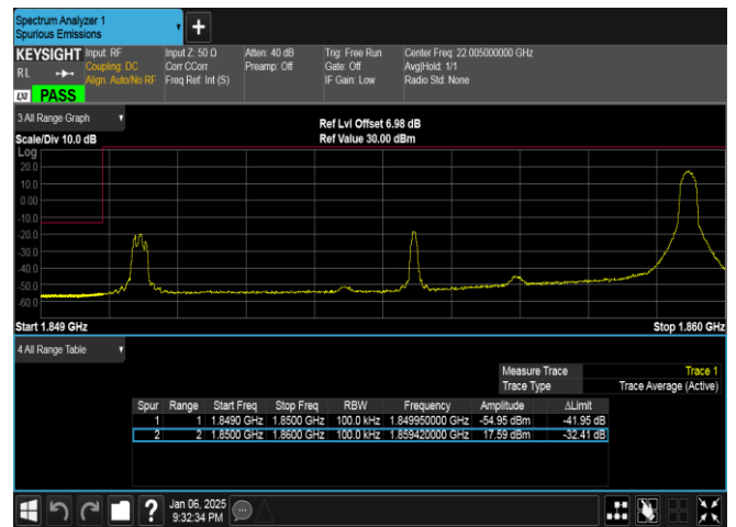
Band2-10MHz-16QAM-18650-1RB#49-PASS
