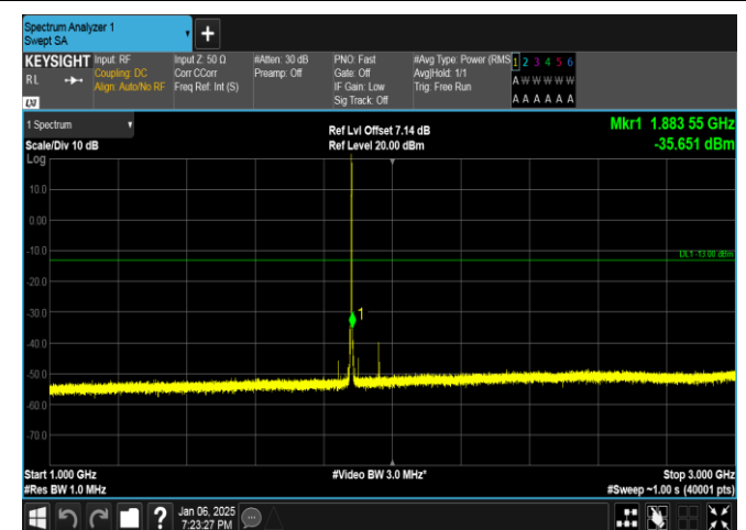
Band2-1.4MHz-QPSK-18900-1RB#5-1000~3000-PASS
