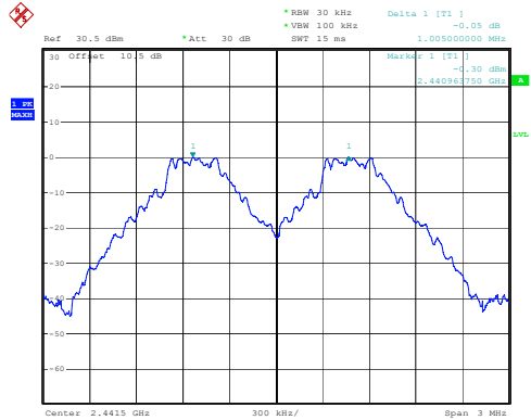
DH1_Middle 1.005MHz
