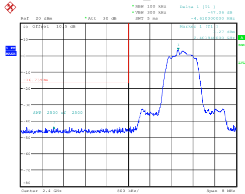
2DH1_Low
