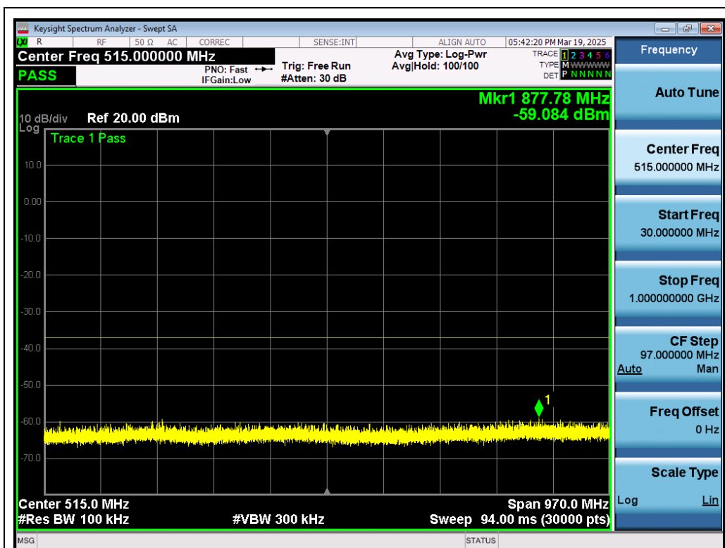
Test_Graph_802.11ax80_ANT1_5290_MCS0_Frequency Band 1
