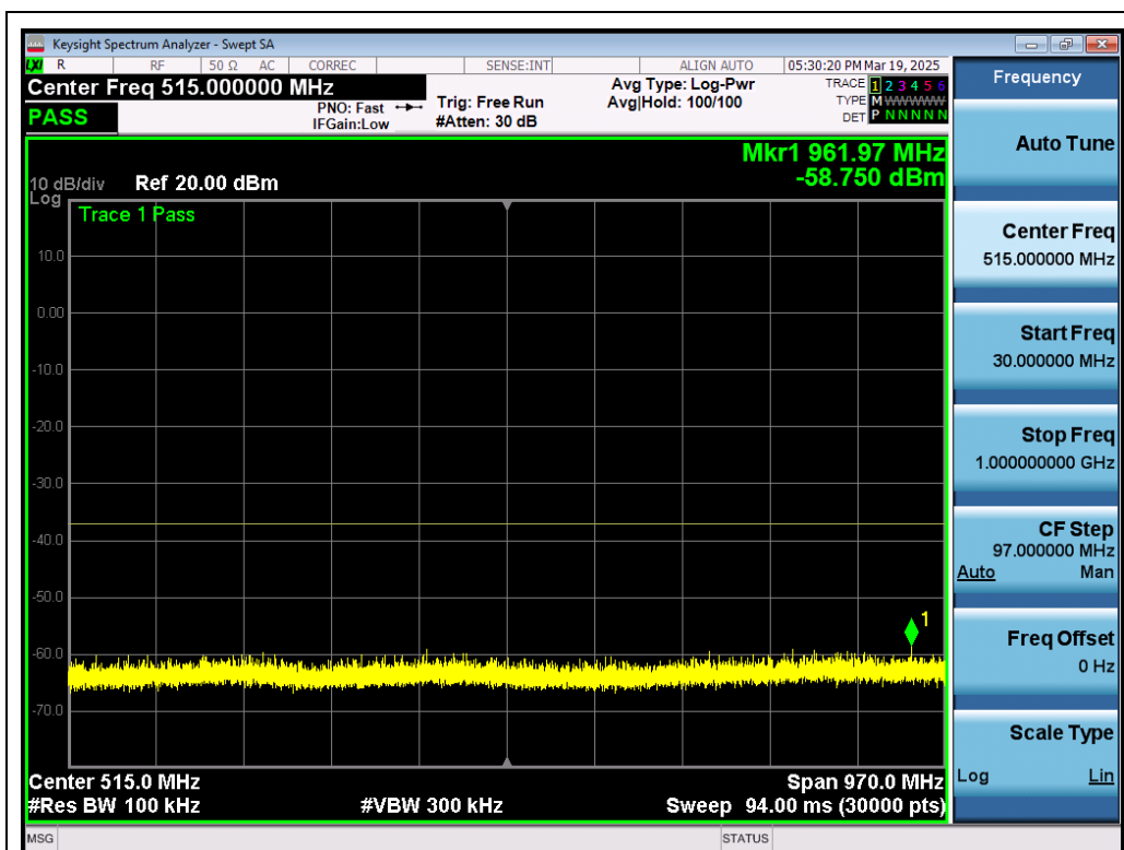
Test_Graph_802.11n40_ANT1_5270_MCS0_Frequency Band 1
