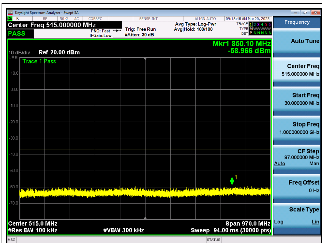
Test_Graph_802.11n40_ANT1_5755_MCS0_Frequency Band1
