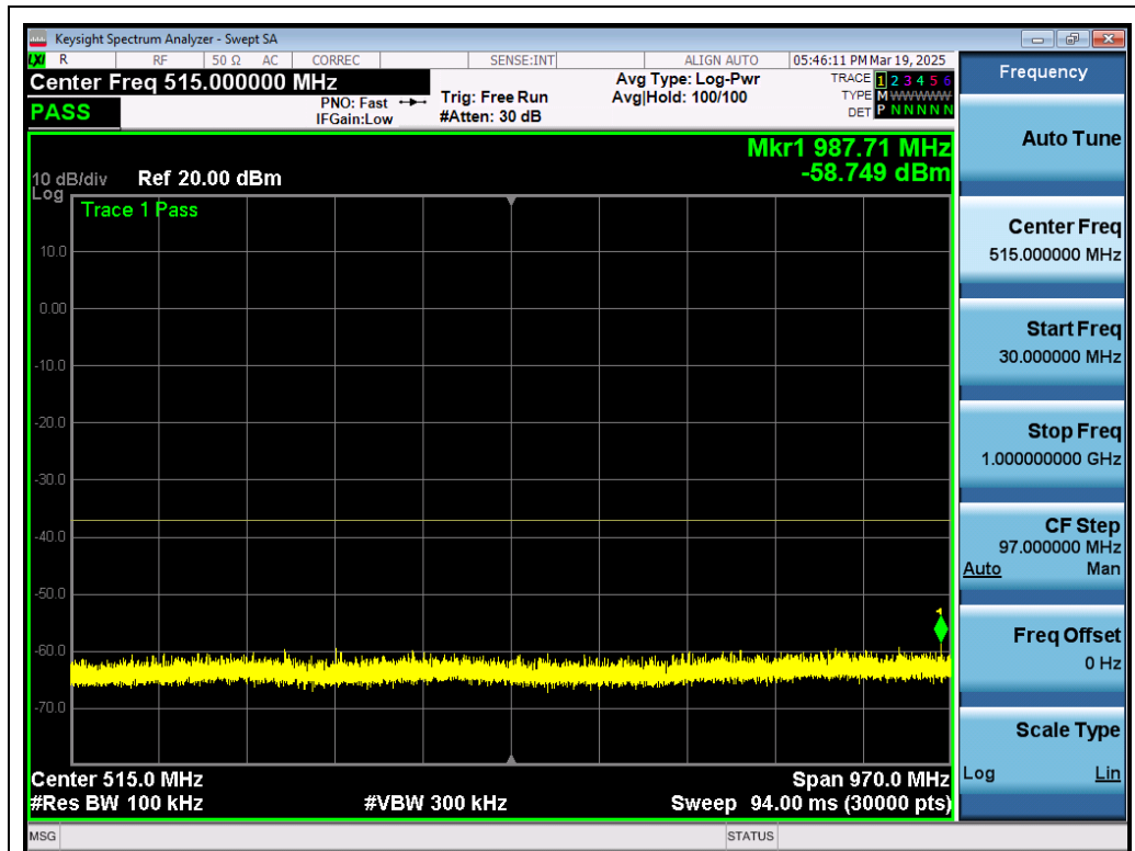
Test_Graph_802.11a_ANT1_5500_6Mbps_Frequency Band 1
