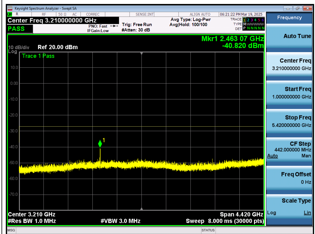
Test_Graph_802.11ax80_ANT1_5610_MCS0_Frequency Band 2
