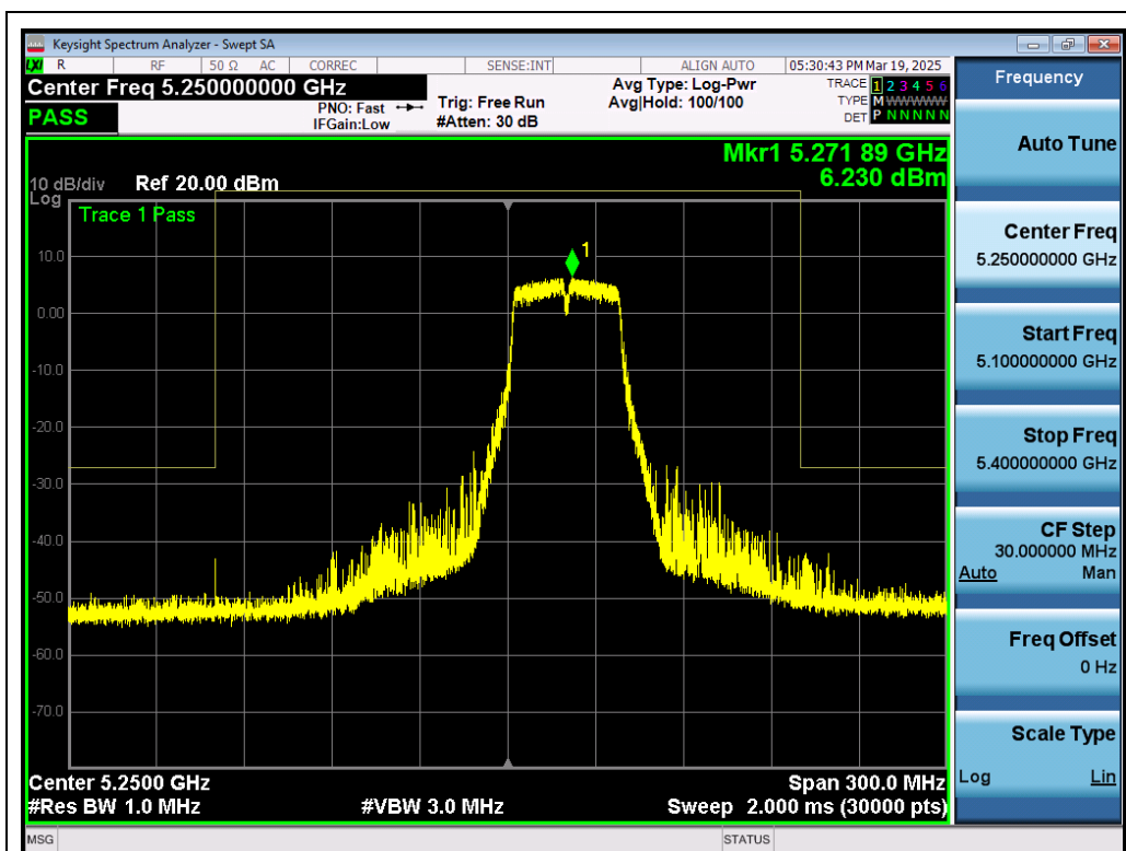
Test_Graph_802.11n40_ANT1_5270_MCS0_Frequency Band 3
