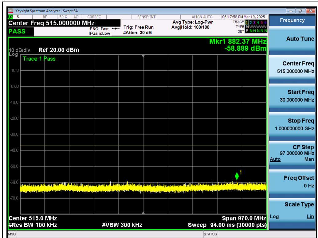
Test_Graph_802.11ax80_ANT1_5530_MCS0_Frequency Band 1
