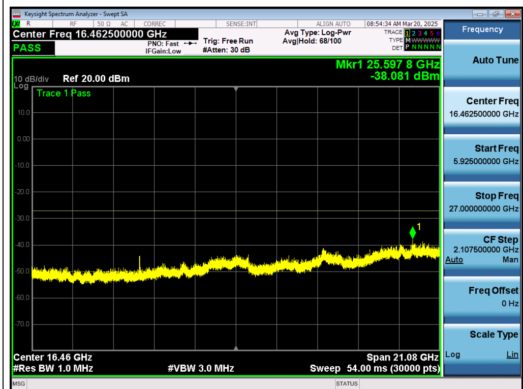
Test_Graph_802.11a_ANT1_5745_6Mbps_Frequency Band4
