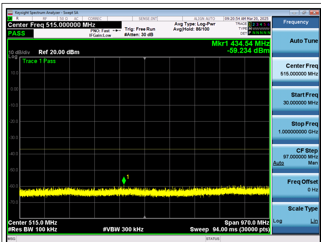
Test_Graph_802.11n40_ANT1_5795_MCS0_Frequency Band1
