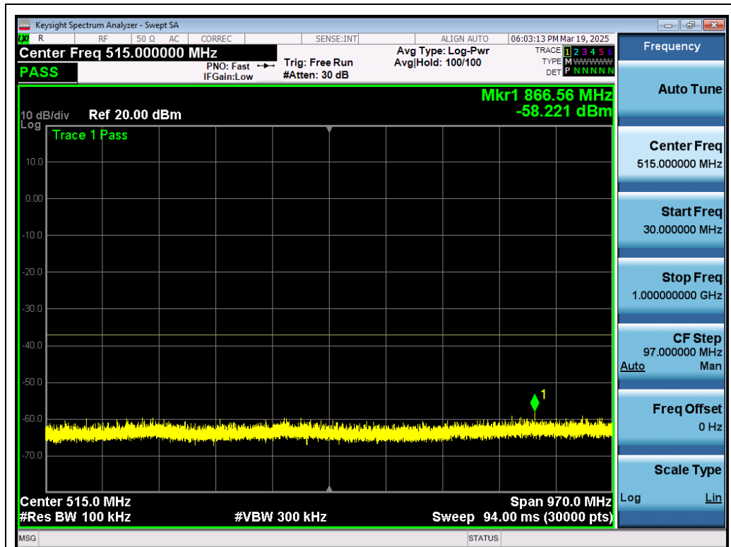
Test_Graph_802.11n40_ANT1_5670_MCS0_Frequency Band 1
