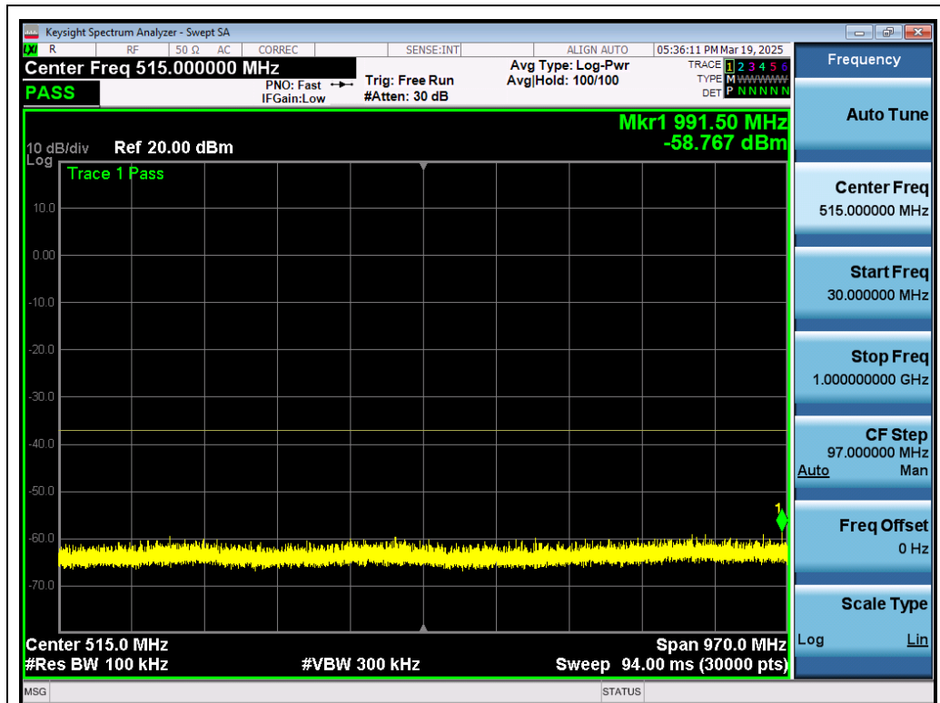
Test_Graph_802.11ac80_ANT1_5290_MCS0_Frequency Band 1
