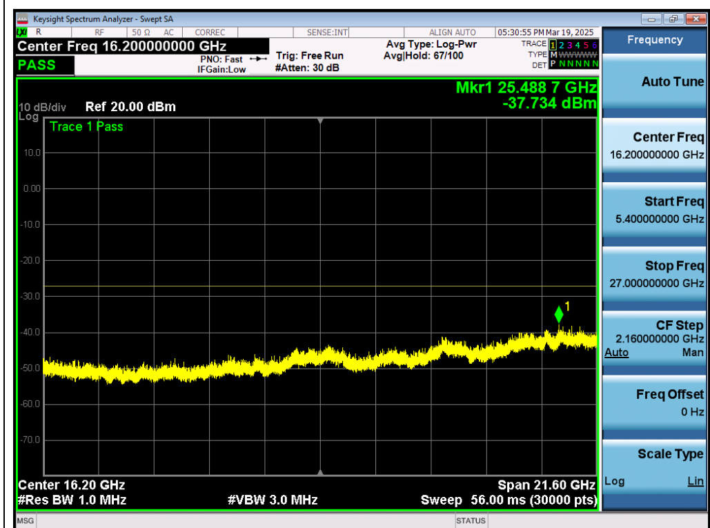
Test_Graph_802.11n40_ANT1_5270_MCS0_Frequency Band 4
