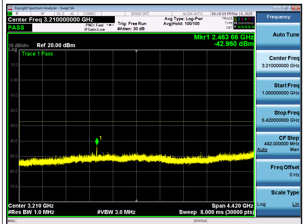
Test_Graph_802.11ax80_ANT1_5530_MCS0_Frequency Band 2
