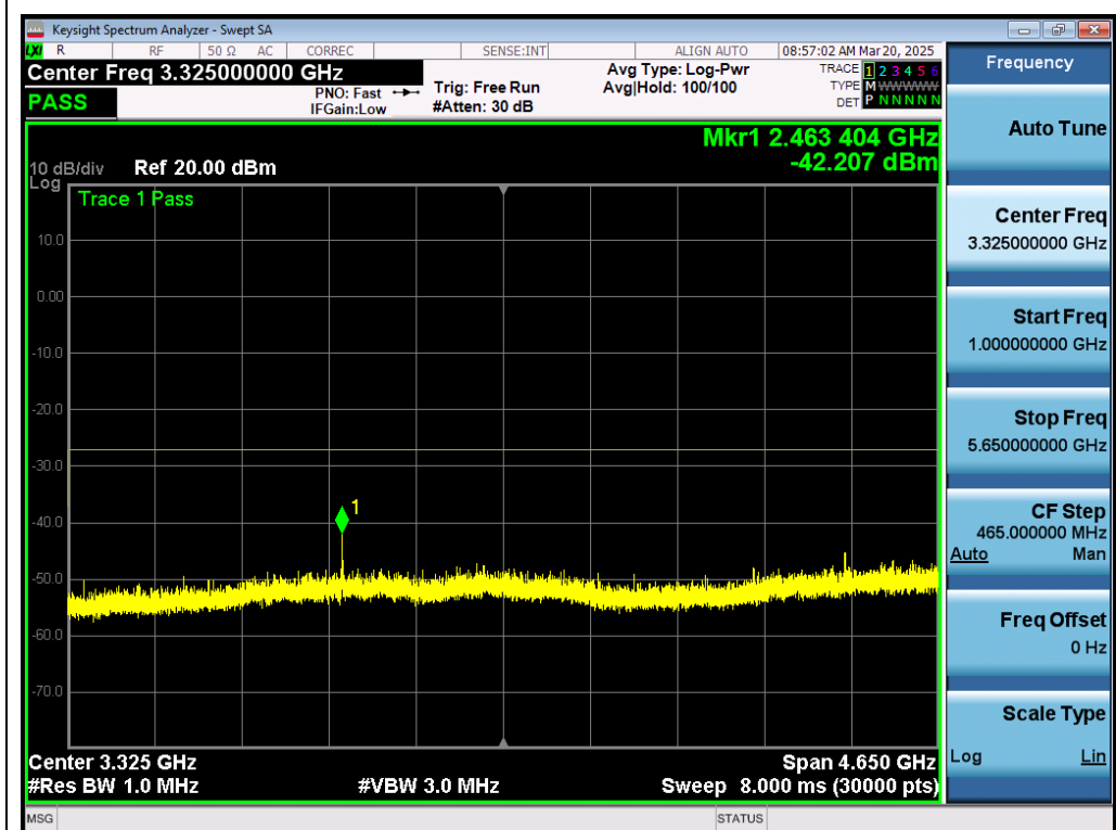
Test_Graph_802.11a_ANT1_5825_6Mbps_Frequency Band2
