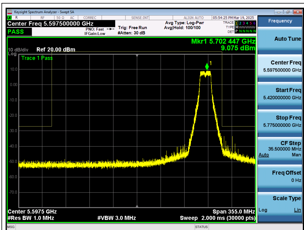
Test_Graph_802.11a_ANT1_5700_6Mbps_Frequency Band 3
