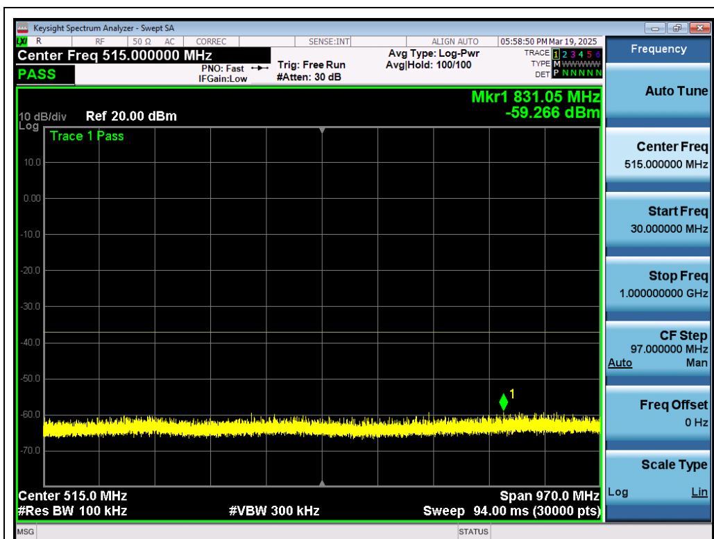
Test_Graph_802.11n40_ANT1_5510_MCS0_Frequency Band 1
