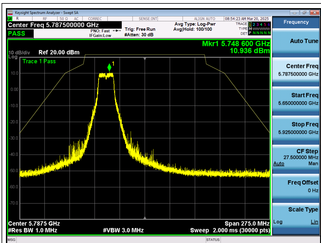
Test_Graph_802.11a_ANT1_5745_6Mbps_Frequency Band3
