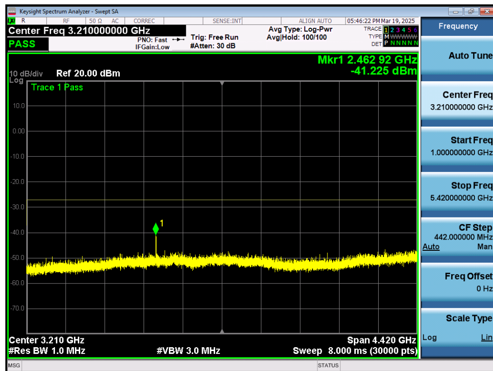
Test_Graph_802.11a_ANT1_5500_6Mbps_Frequency Band 2
