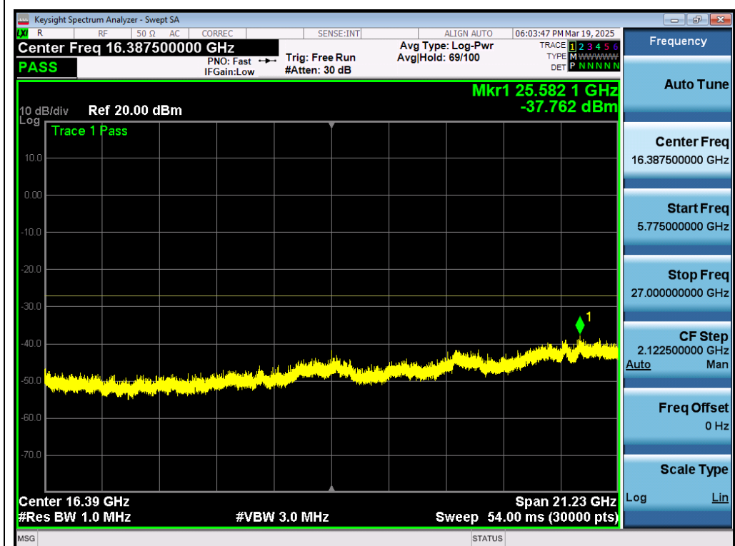
Test_Graph_802.11n40_ANT1_5670_MCS0_Frequency Band 4
