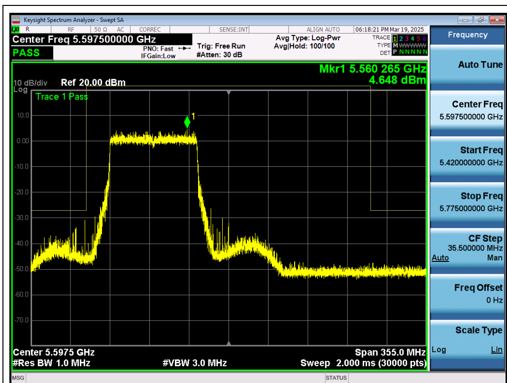
Test_Graph_802.11ax80_ANT1_5530_MCS0_Frequency Band 3
