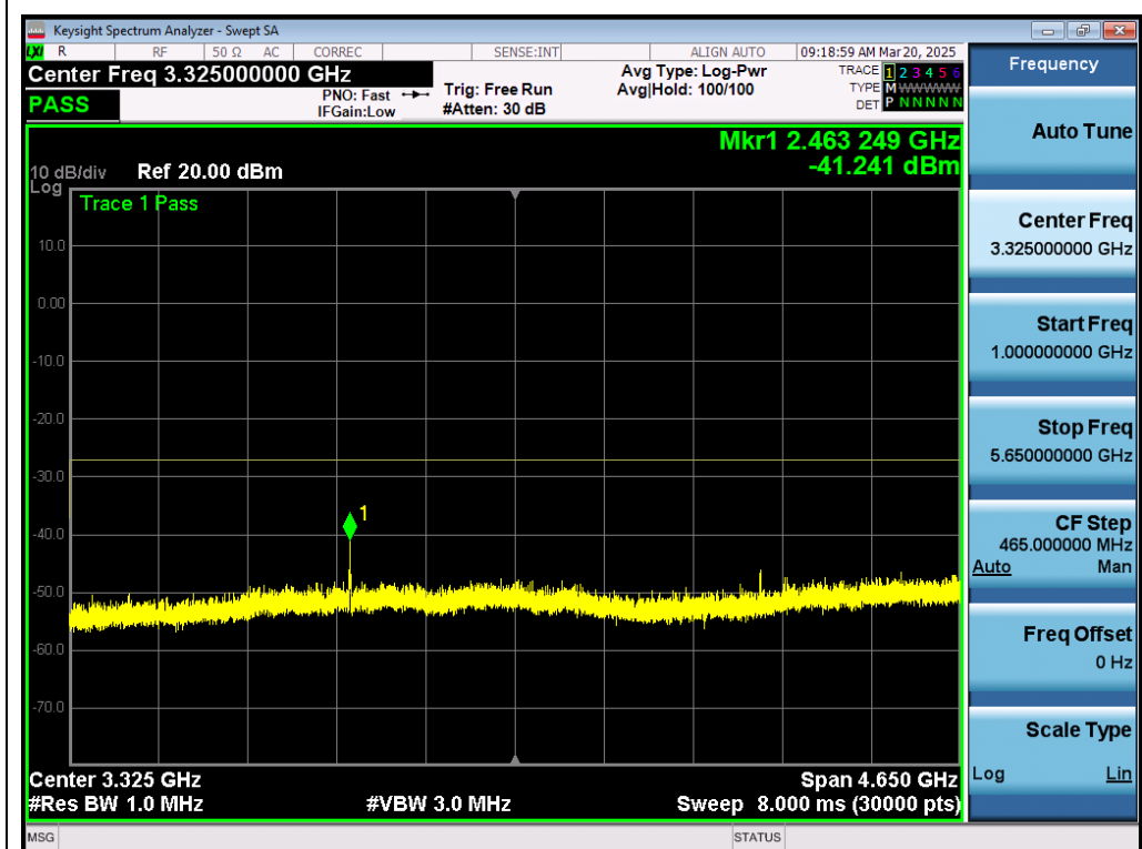
Test_Graph_802.11n40_ANT1_5755_MCS0_Frequency Band2
