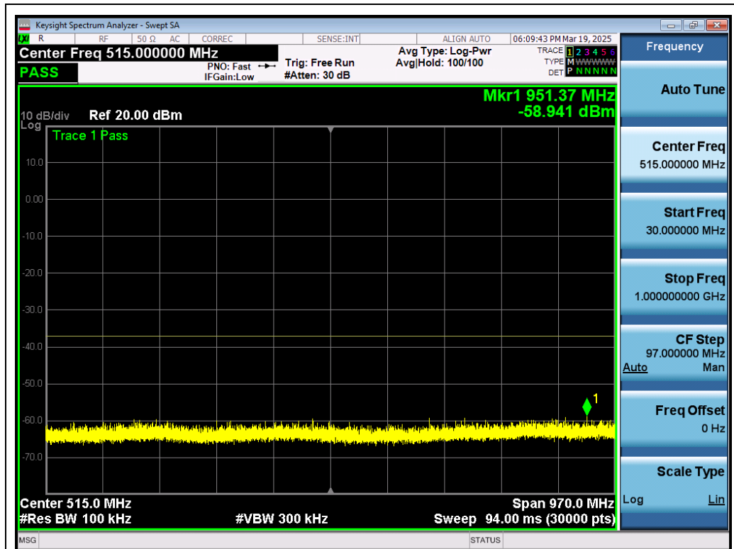
Test_Graph_802.11ac80_ANT1_5530_MCS0_Frequency Band 1
