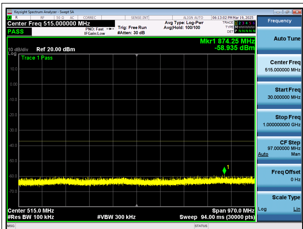
Test_Graph_802.11ac80_ANT1_5610_MCS0_Frequency Band 1
