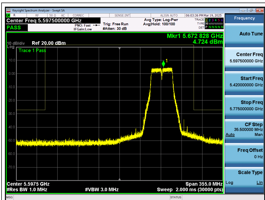
Test_Graph_802.11n40_ANT1_5670_MCS0_Frequency Band 3
