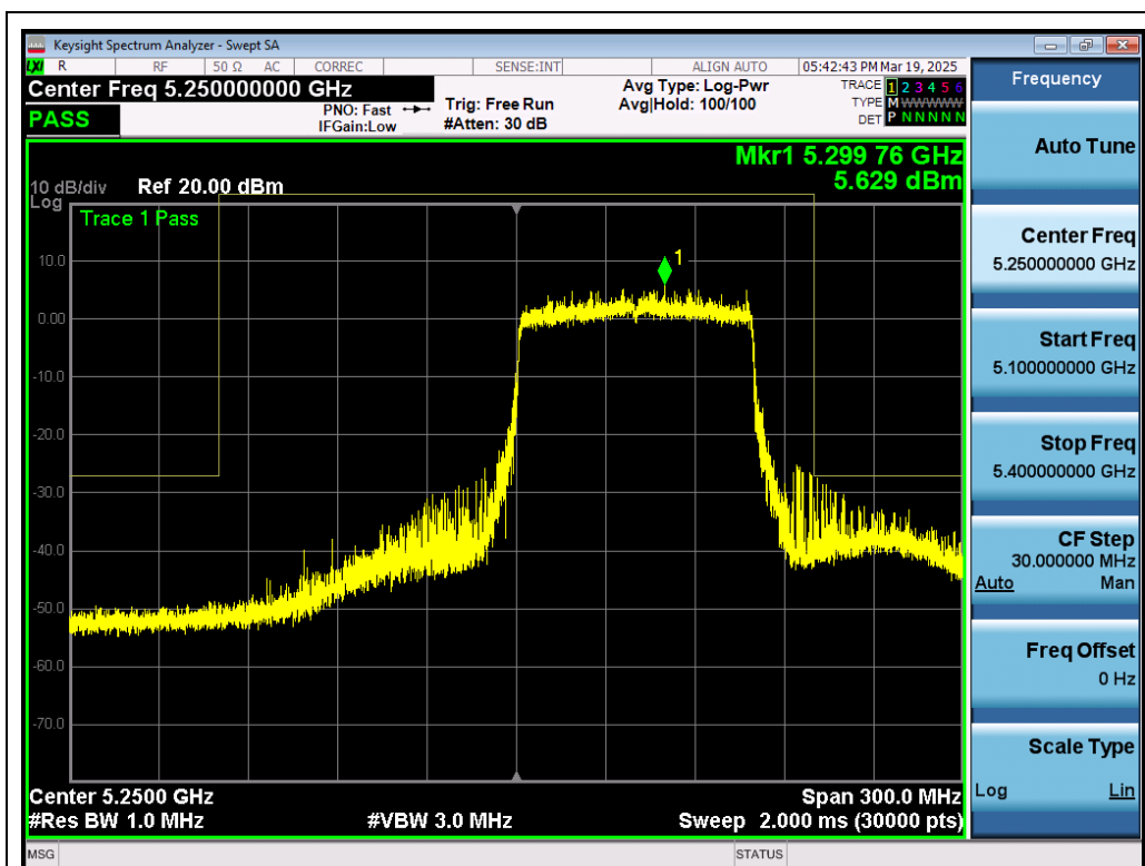
Test_Graph_802.11ax80_ANT1_5290_MCS0_Frequency Band 3
