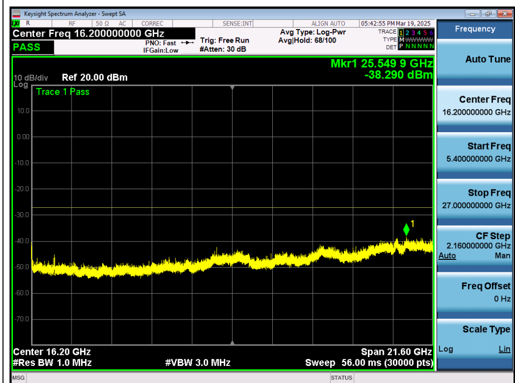
Test_Graph_802.11ax80_ANT1_5290_MCS0_Frequency Band 4
