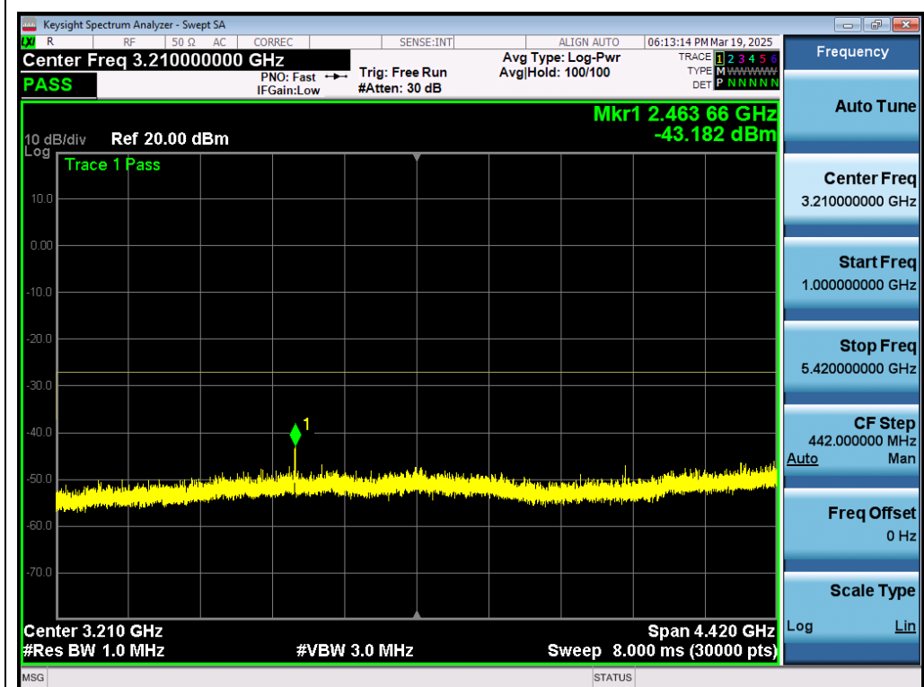
Test_Graph_802.11ac80_ANT1_5610_MCS0_Frequency Band 2
