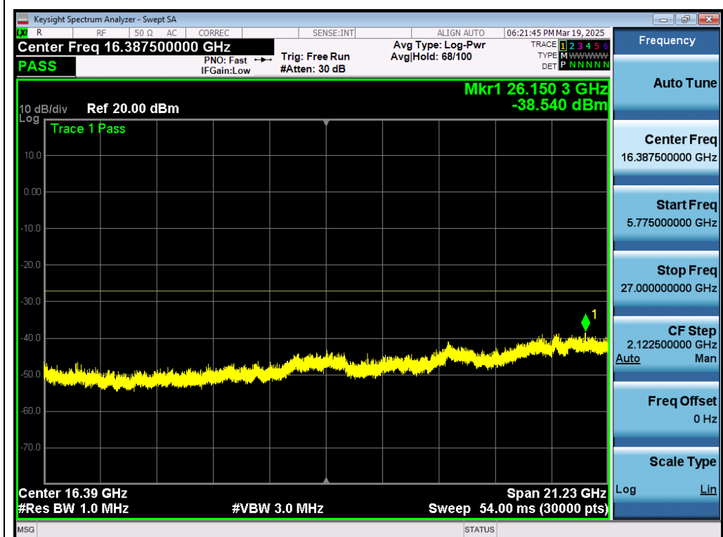
Test Graph 802.11ax80 ANT1 5610 MCS0 Frequency Band 4
