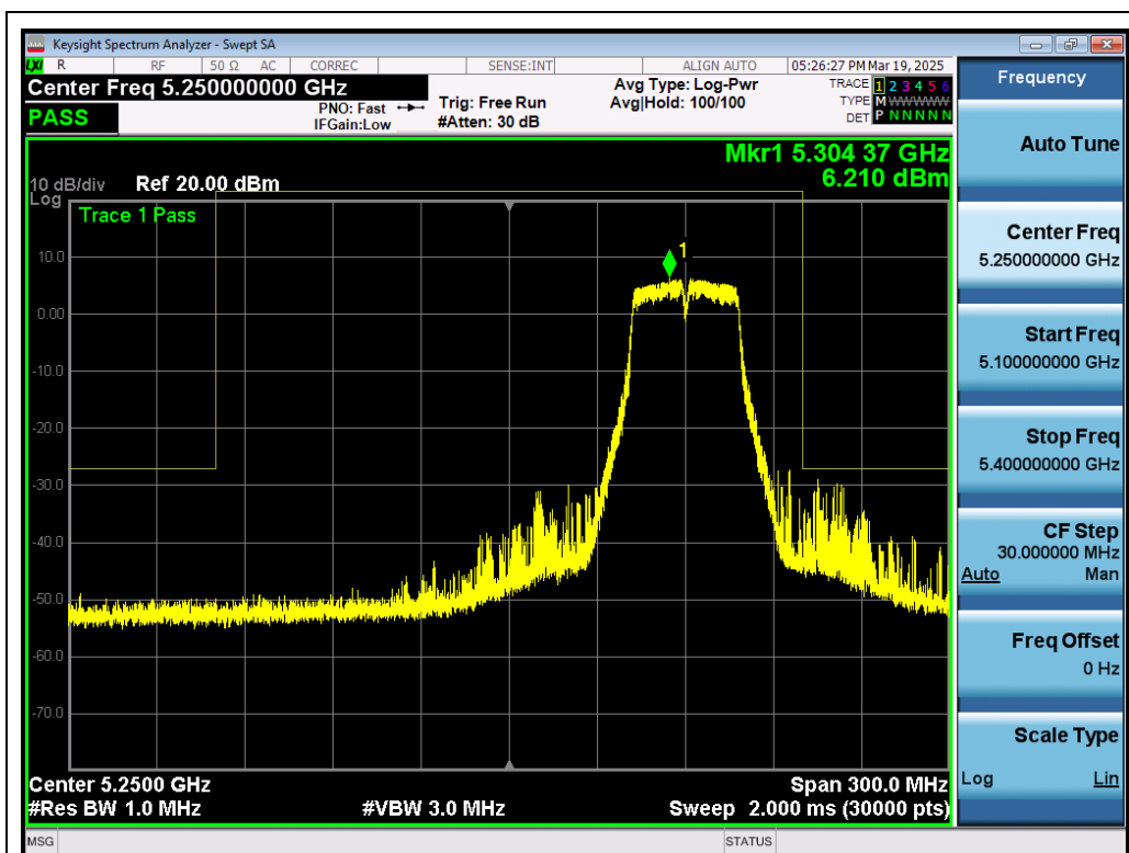
Test_Graph_802.11n40_ANT1_5310_MCS0_Frequency Band 3
