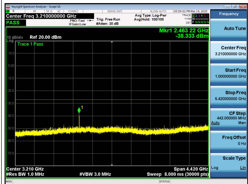
Test_Graph_802.11n40_ANT1_5510_MCS0_Frequency Band 2
