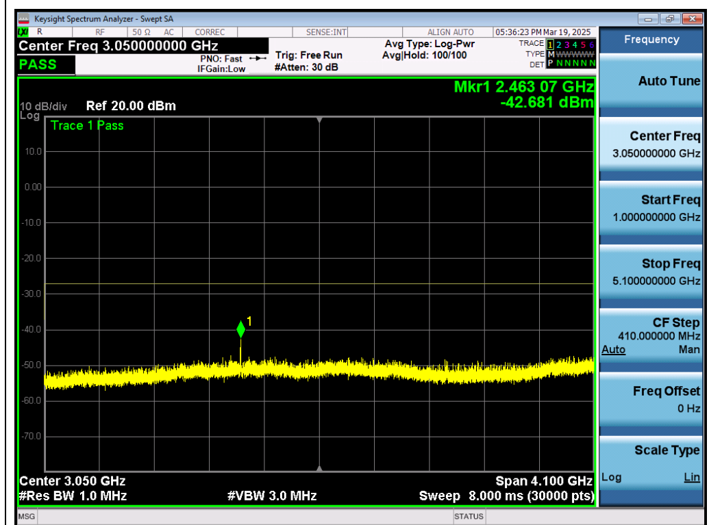
Test_Graph_802.11ac80_ANT1_5290_MCS0_Frequency Band 2
