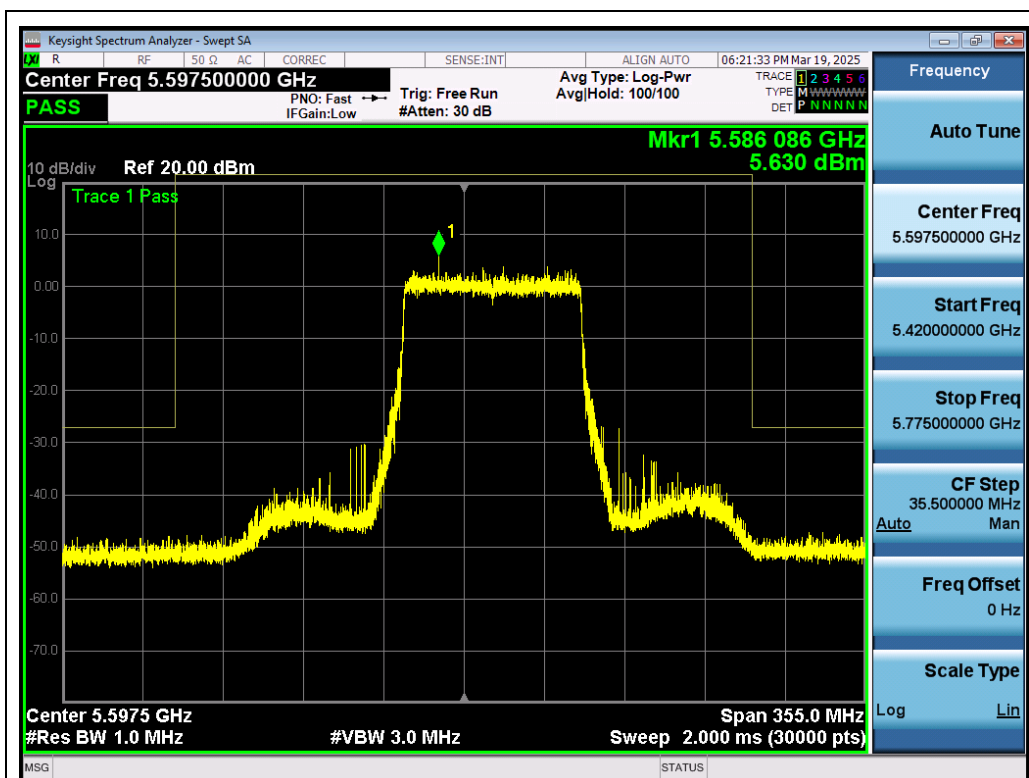
Test Graph 802.11ax80 ANT1 5610 MCS0 Frequency Band 3
