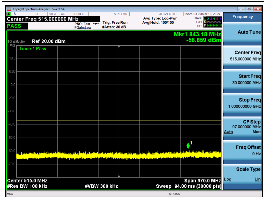
Test_Graph_802.11n40_ANT1_5310_MCS0_Frequency Band 1
