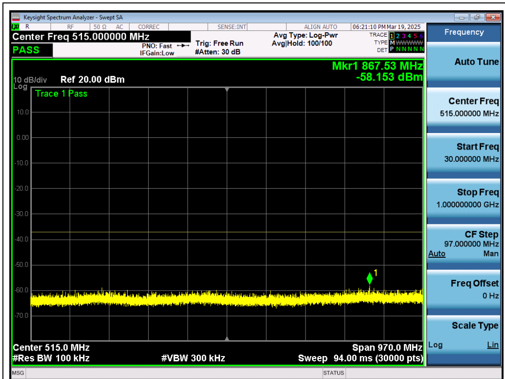
Test_Graph_802.11ax80_ANT1_5610_MCS0_Frequency Band 1
