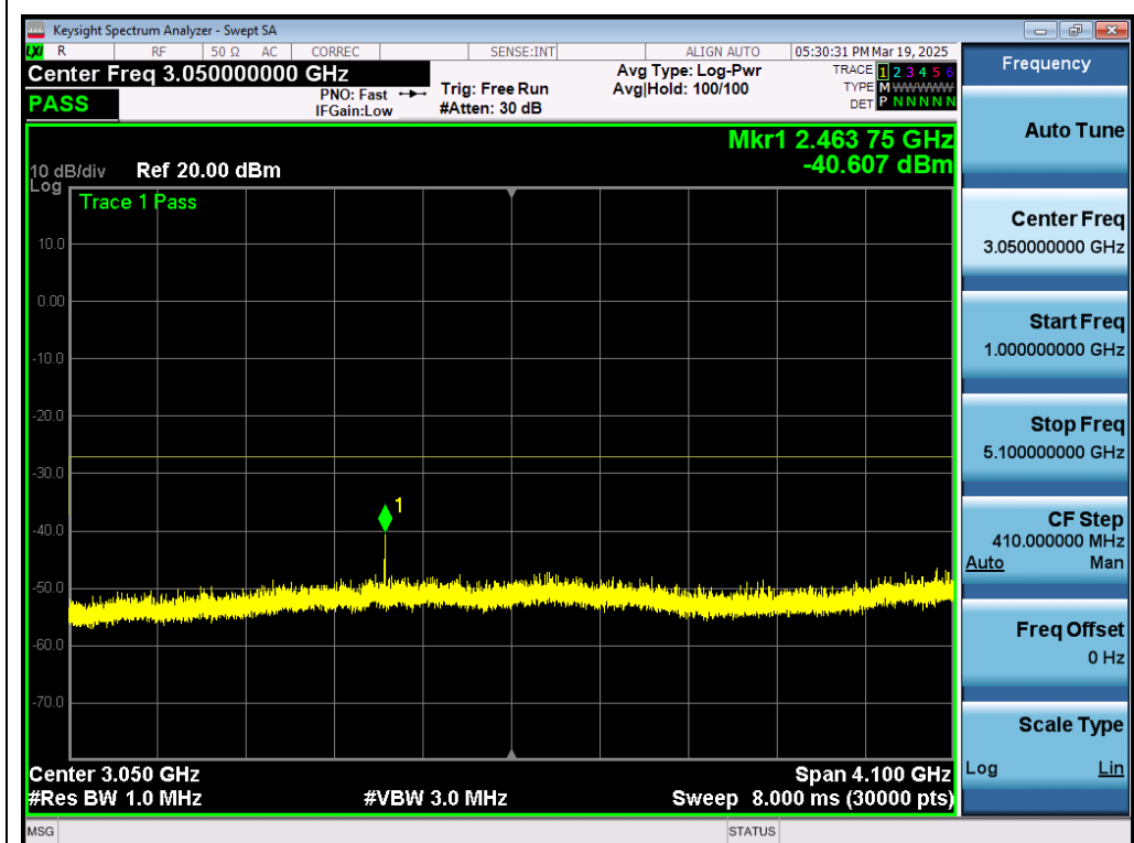
Test_Graph_802.11n40_ANT1_5270_MCS0_Frequency Band 2
