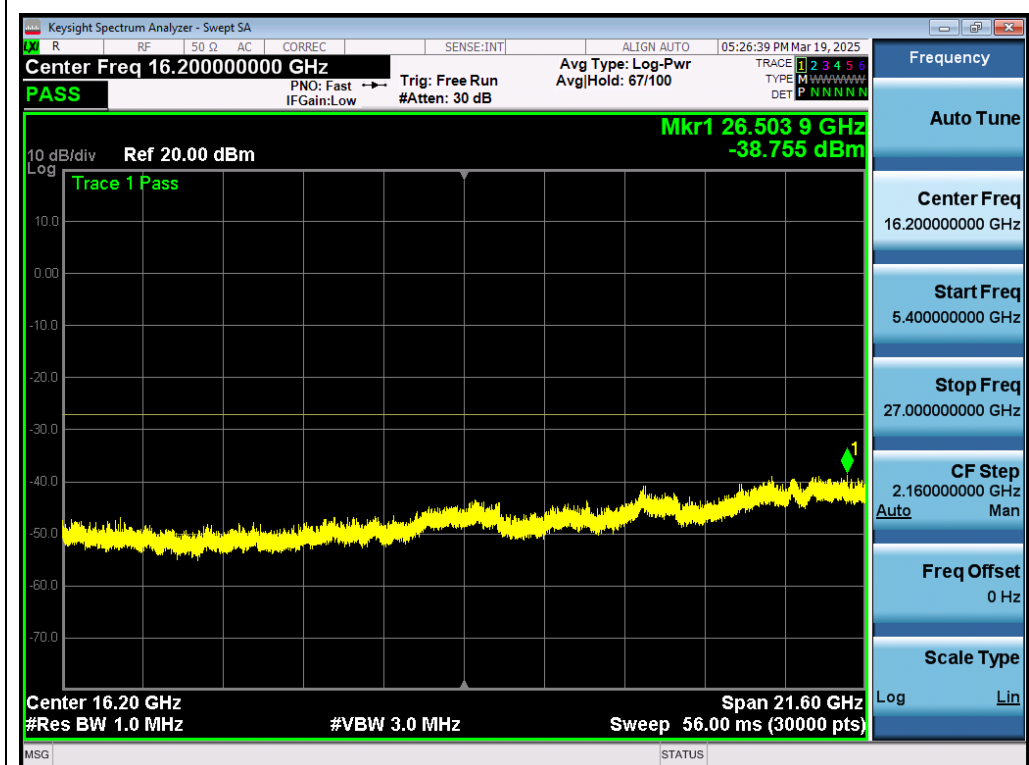
Test_Graph_802.11n40_ANT1_5310_MCS0_Frequency Band 4
