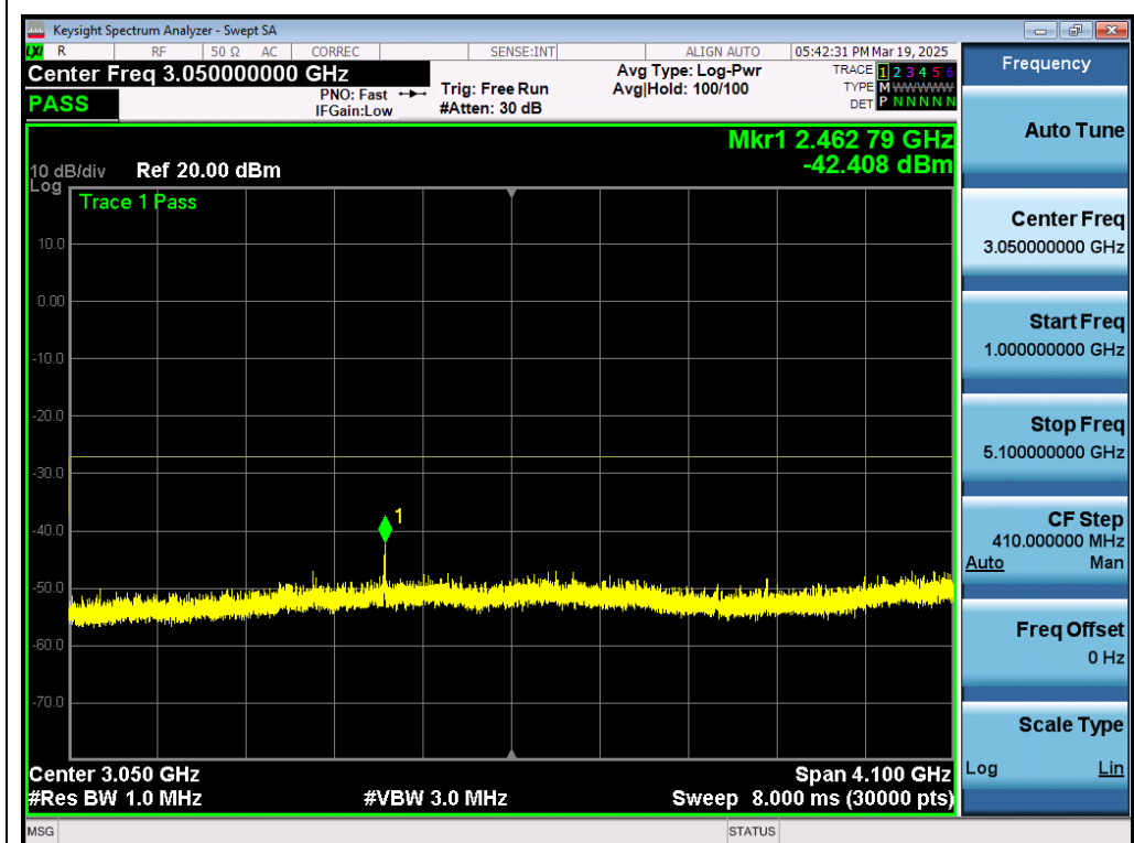
Test_Graph_802.11ax80_ANT1_5290_MCS0_Frequency Band 2
