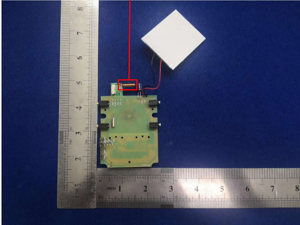
433.92MHz Spring antenna
