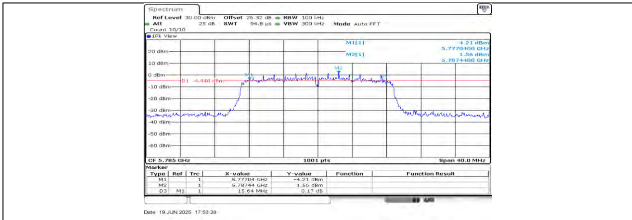
11N20SISO_Ant1_5785
