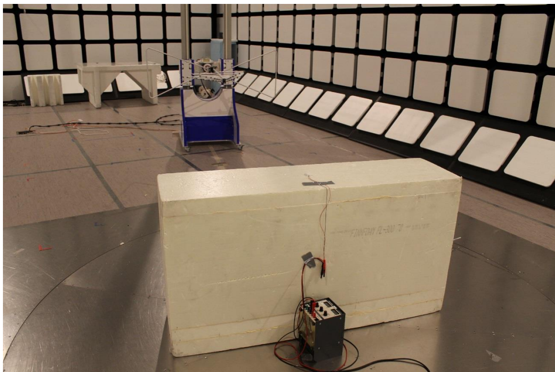
Photograph 5. Radiated Spurious Emissions 30 – 1000 MHz
