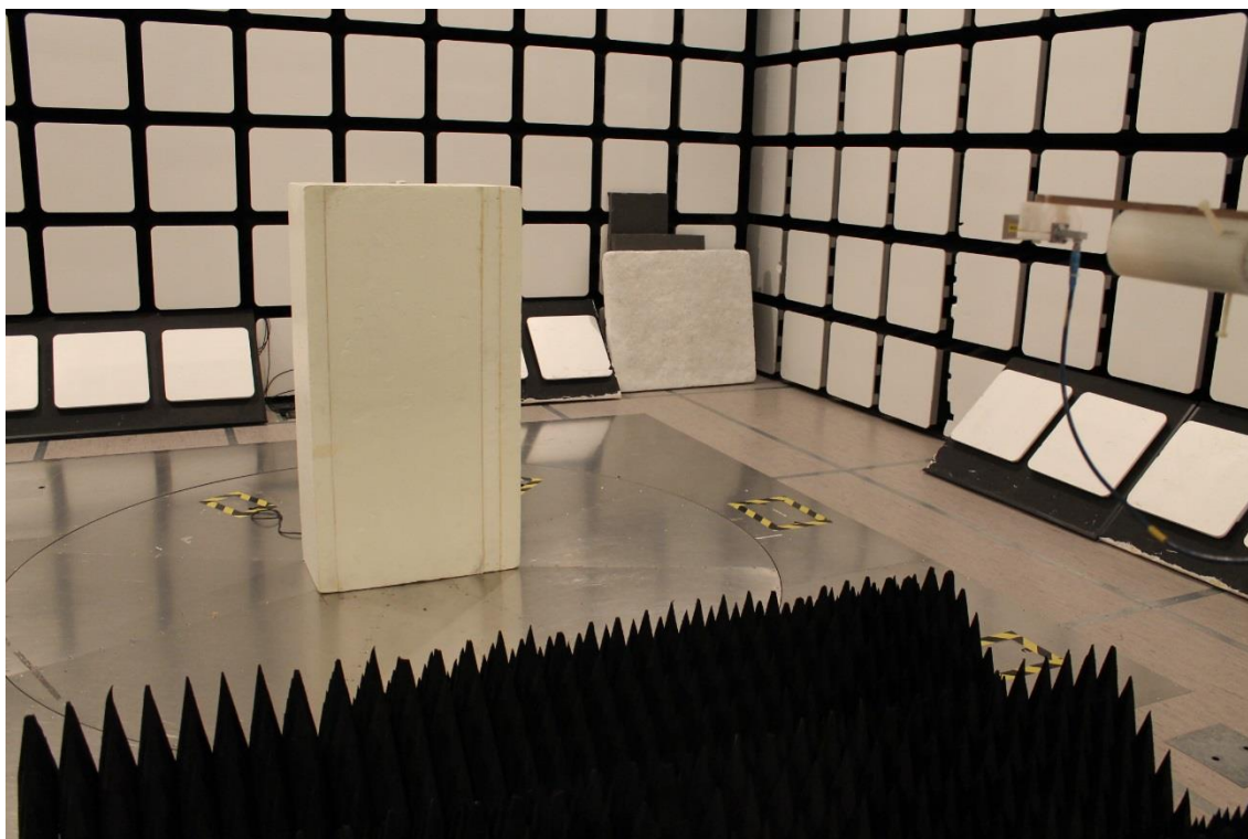
Photograph 7. Radiated Spurious Emissions 18 – 26.5 GHz
