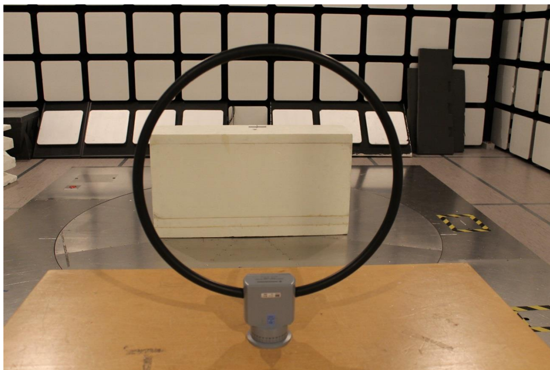
Photograph 4. Radiated Spurious Emissions 9 kHz – 30 MHz
