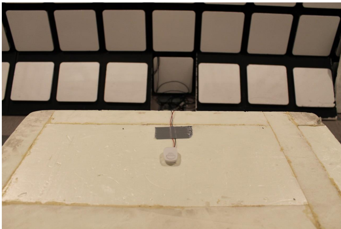
Photograph 8. EUT on table
