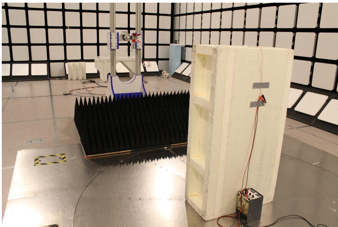
Photograph 6. Radiated Spurious Emissions 1 – 18 GHz
