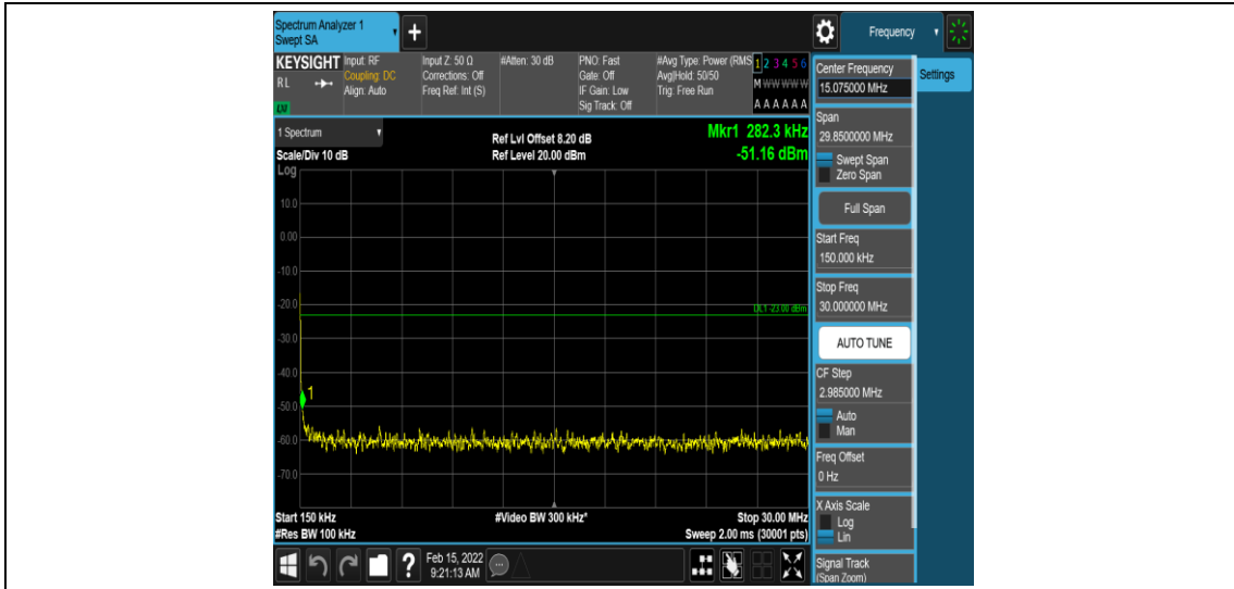
Band12-3MHz-16QAM-23025-1-0-Low-0.15-30--51.16-PASS
