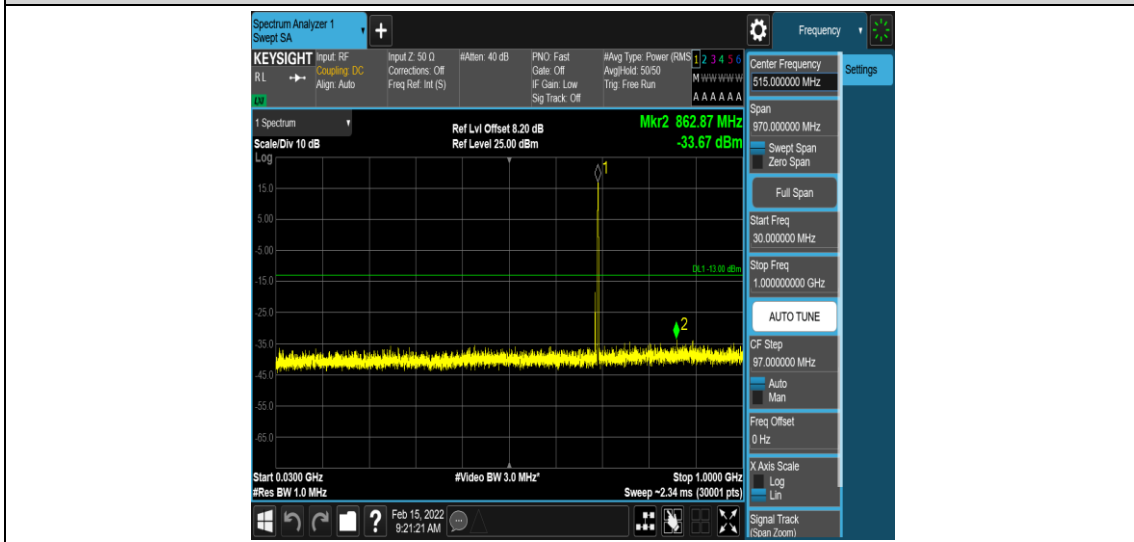
Band12-3MHz-16QAM-23025-1-0-Low-30-1000--33.67-PASS
