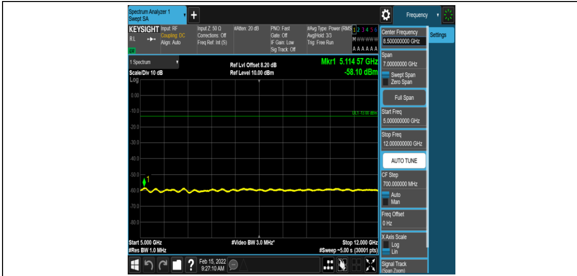
Band12-3MHz-QPSK-23165-1-0-High-5000-12000--58.1-PASS
