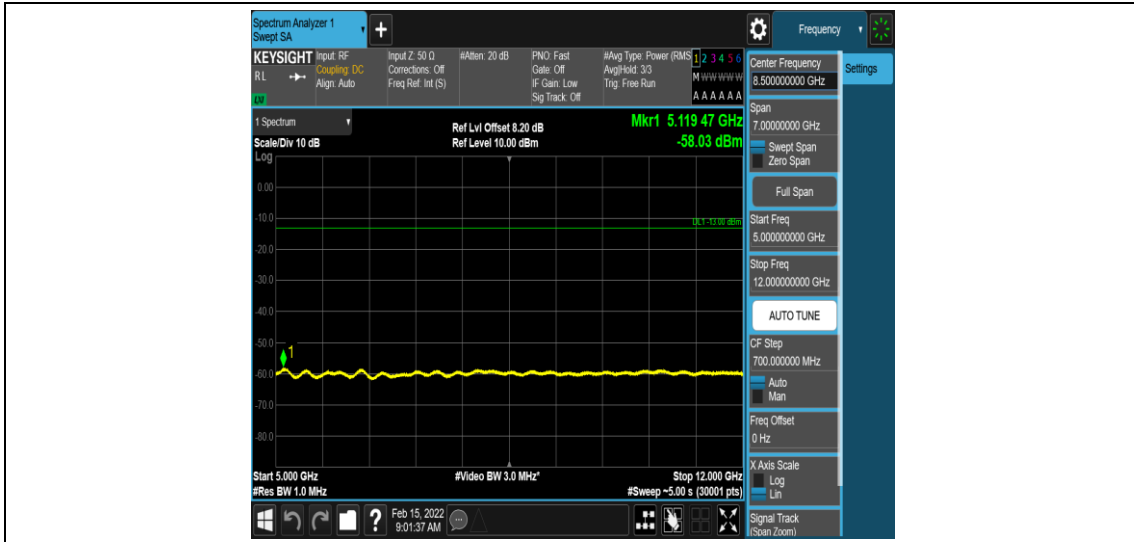
Band12-1.4MHz-16QAM-23017-1-0-Low-5000-12000--58.03-PASS
