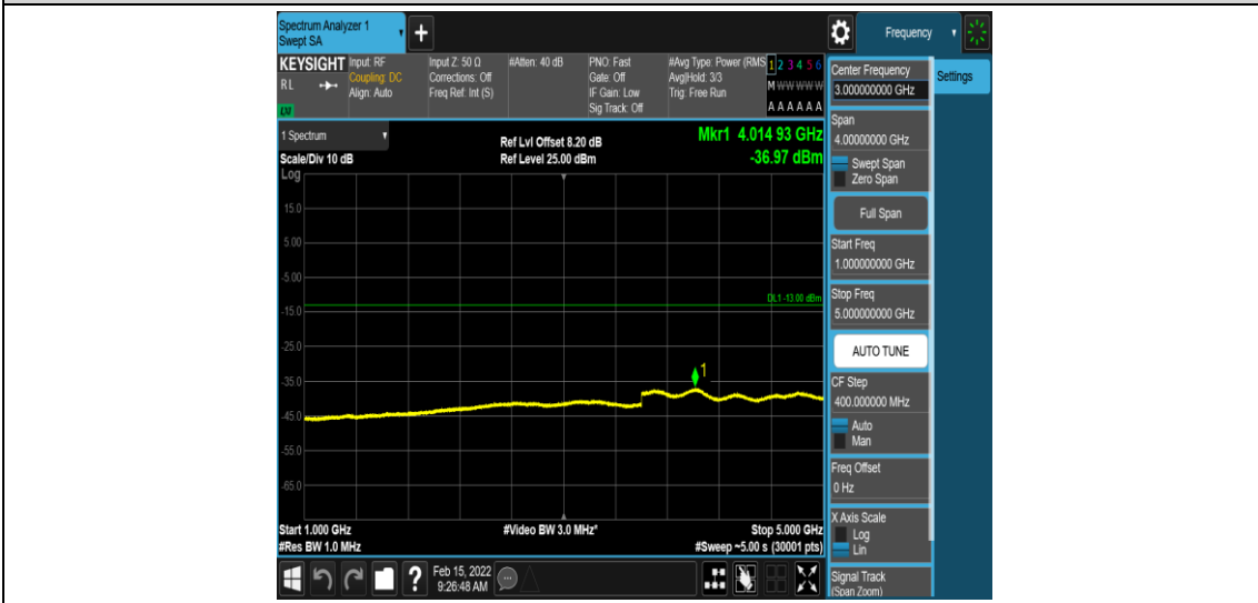
Band12-3MHz-QPSK-23165-1-0-High-1000-5000--36.97-PASS
