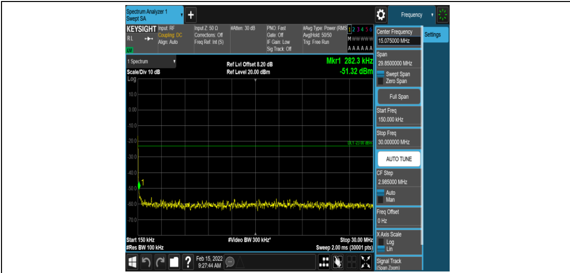
Band12-3MHz-16QAM-23165-1-0-High-0.15-30--51.32-PASS
