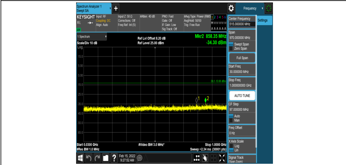
Band12-3MHz-16QAM-23165-1-0-High-30-1000--34.3-PASS
