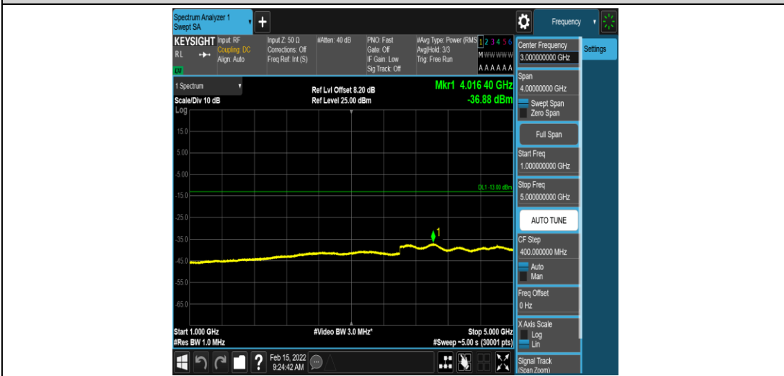
Band12-3MHz-16QAM-23095-1-0-Low-1000-5000--36.88-PASS
