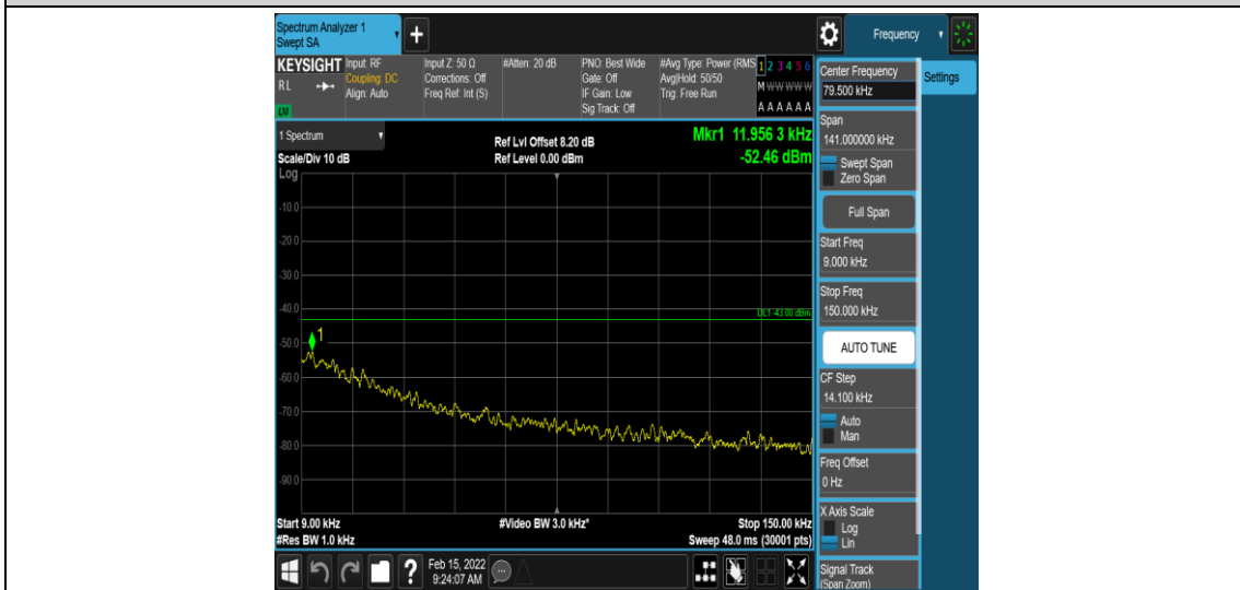
Band12-3MHz-16QAM-23095-1-0-Low-0.009-0.15--52.46-PASS
