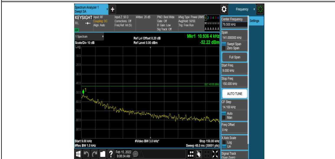
Band12-1.4MHz-16QAM-23173-1-0-High-0.009-0.15--52.22-PASS
