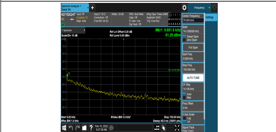
Band12-3MHz-16QAM-23165-1-0-High-0.009-0.15--51.2-PASS
