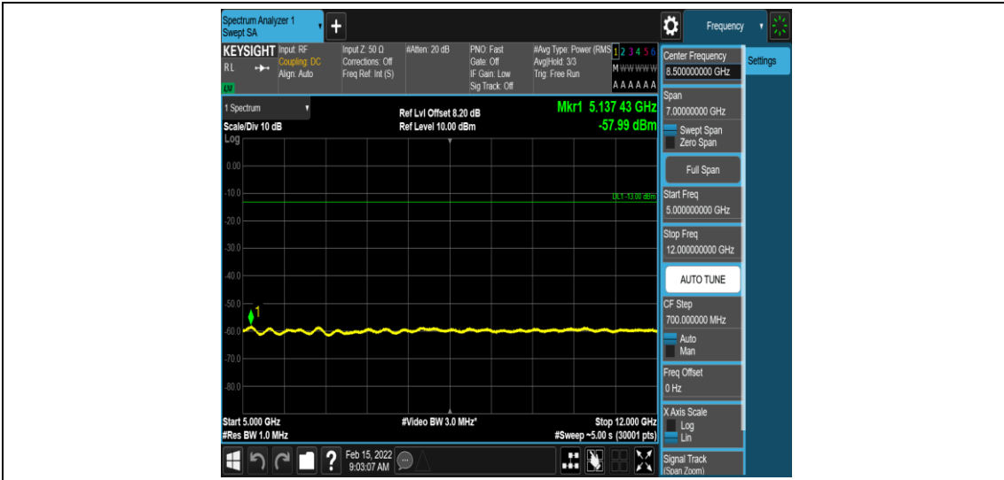
Band12-1.4MHz-QPSK-23095-1-0-Low-5000-12000--57.99-PASS
