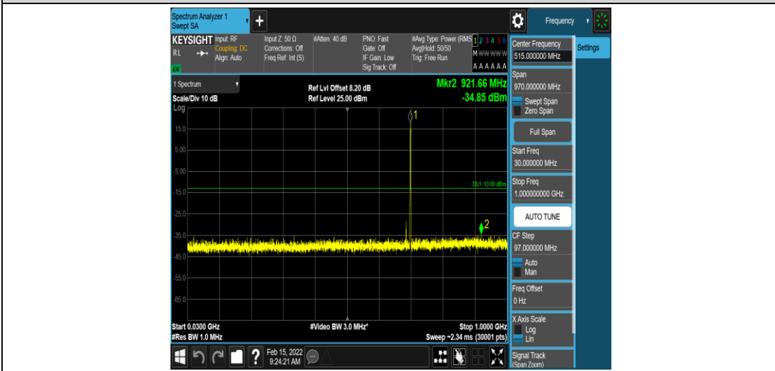
Band12-3MHz-16QAM-23095-1-0-Low-30-1000--34.85-PASS
