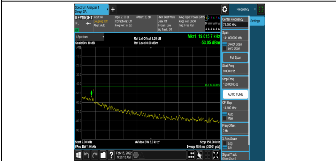
Band12-3MHz-QPSK-23165-1-0-High-0.009-0.15--53.05-PASS
