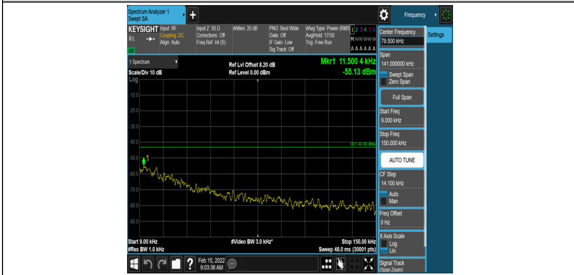
Band12-1.4MHz-16QAM-23095-1-0-Low-0.009-0.15--55.14-PASS
