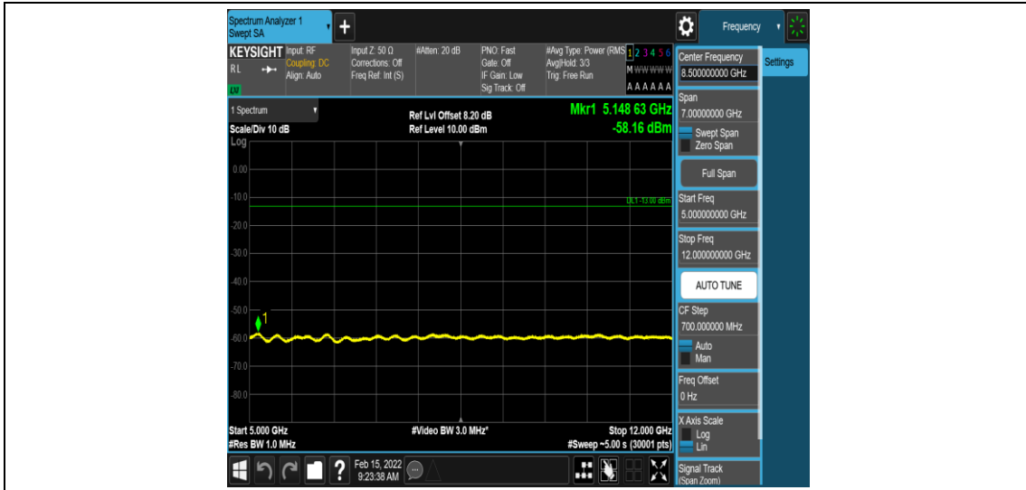
Band12-3MHz-QPSK-23095-1-0-Low-5000-12000--58.17-PASS
