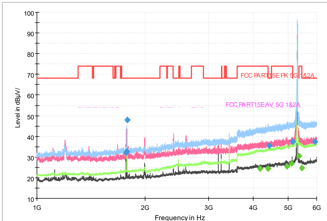
Fig.311 Radiated emission: 802.11ac(20M),CH60, 1GHz-6GHz
