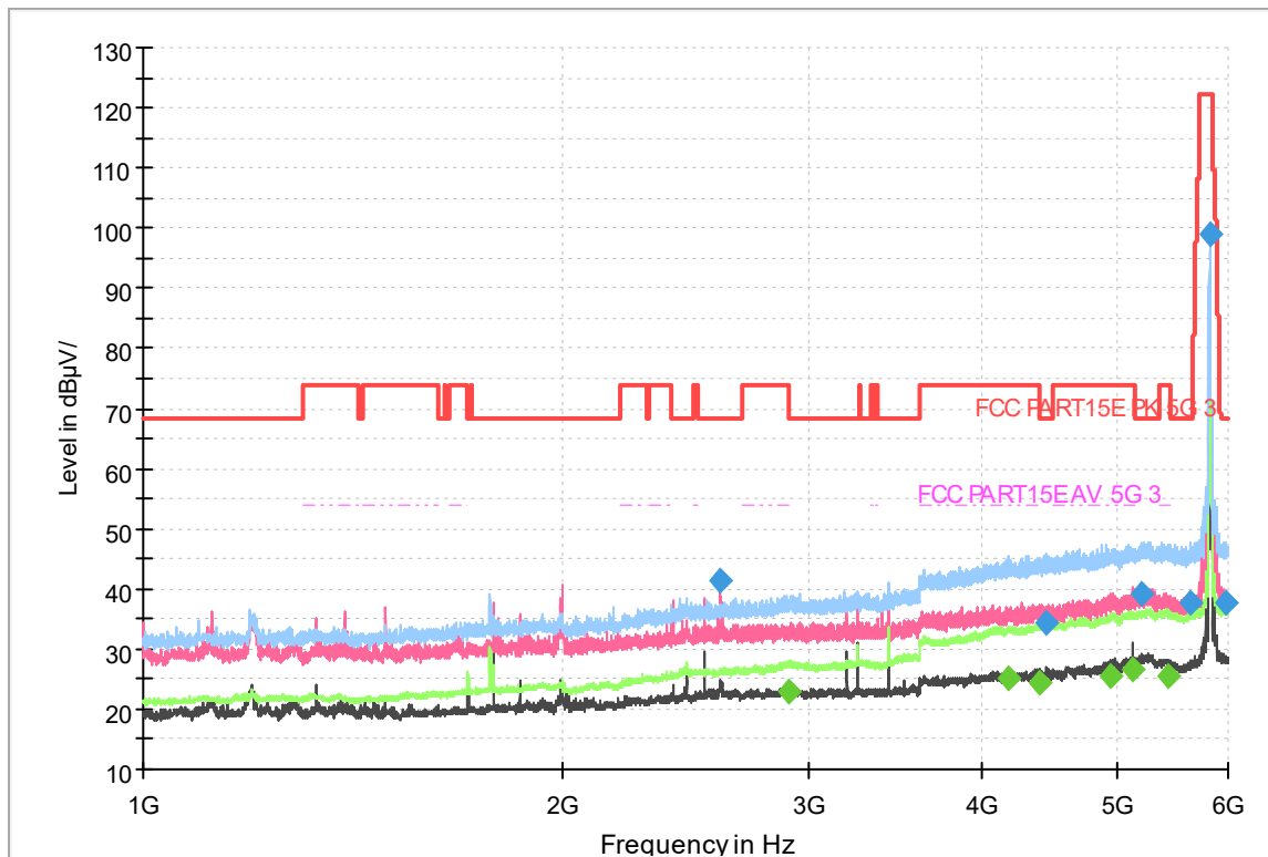
Fig.325 Radiated emission: 802.11ac(20M),CH165, 1GHz-6GHz
