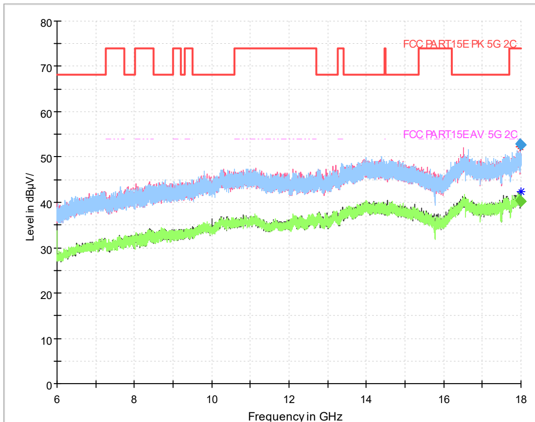
Fig.316 Radiated emission: 802.11ac(20M),CH100, 6GHz-18GHz
