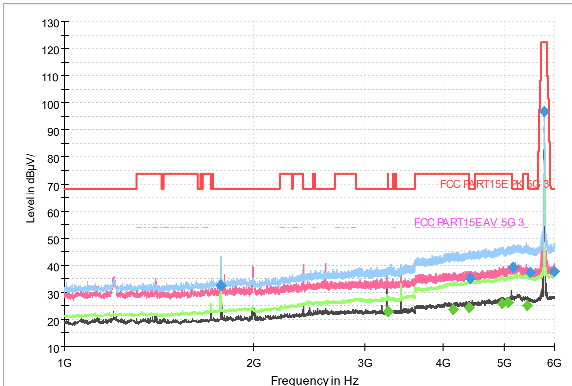
Fig.3.23 Radiated emission: 802.11ac(20M),CH157, 1GHz-6GHz
