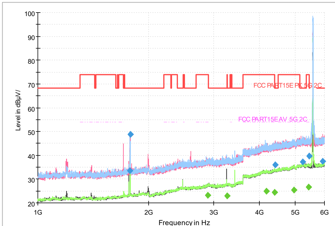
Fig.317 Radiated emission: 802.11ac(20M),CH116, 1GHz-6GHz
