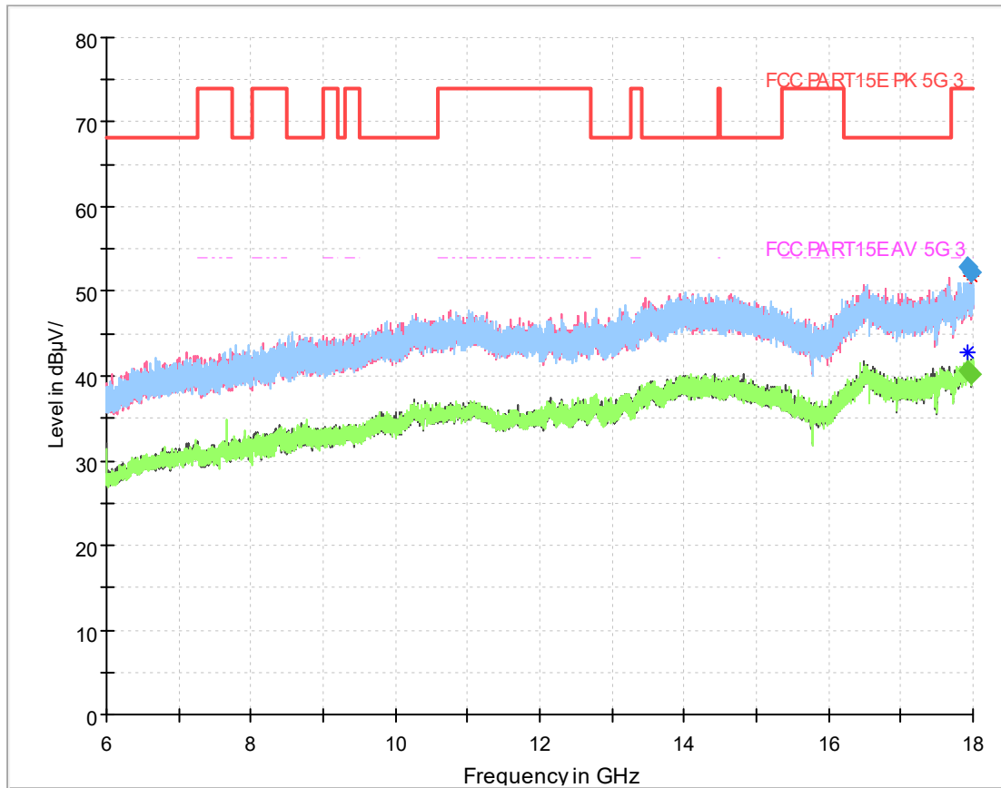
Fig.324 Radiated emission: 802.11ac(20M),CH157, 6GHz-18GHz
