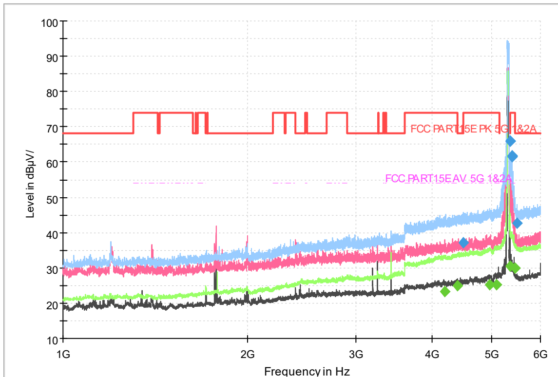
Fig.333 Radiated emission: 802.11ac(40M),CH62, 1GHz-6GHz
