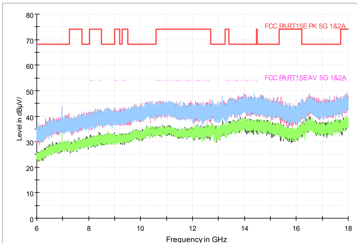
Fig.334 Radiated emission: 802.11ac(40M),CH62, 6GHz-18GHz
