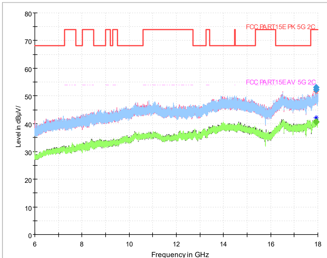
Fig.320 Radiated emission: 802.11ac(20M),CH140, 6GHz-18GHz
