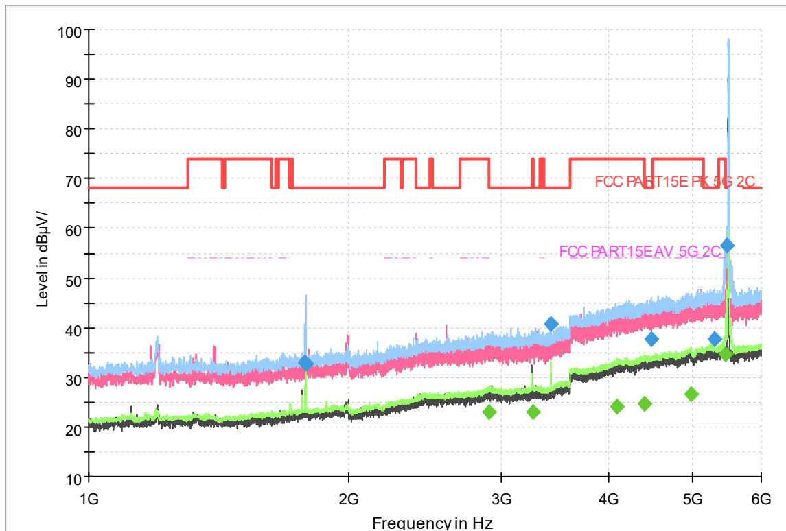
Fig.315 Radiated emission: 802.11ac(20M),CH100, 1GHz-6GHz
