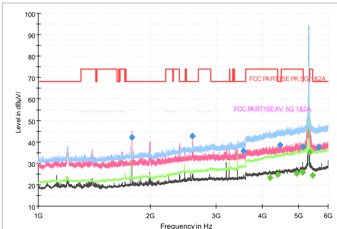
Fig.313 Radiated emission: 802.11ac(20M),CH64, 1GHz-6GHz
