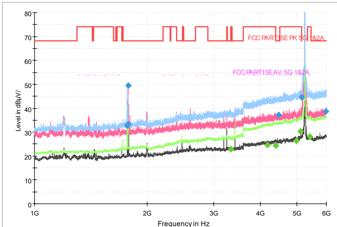
Fig.309 Radiated emission: 802.11ac(20M),CH52, 1GHz-6GHz
