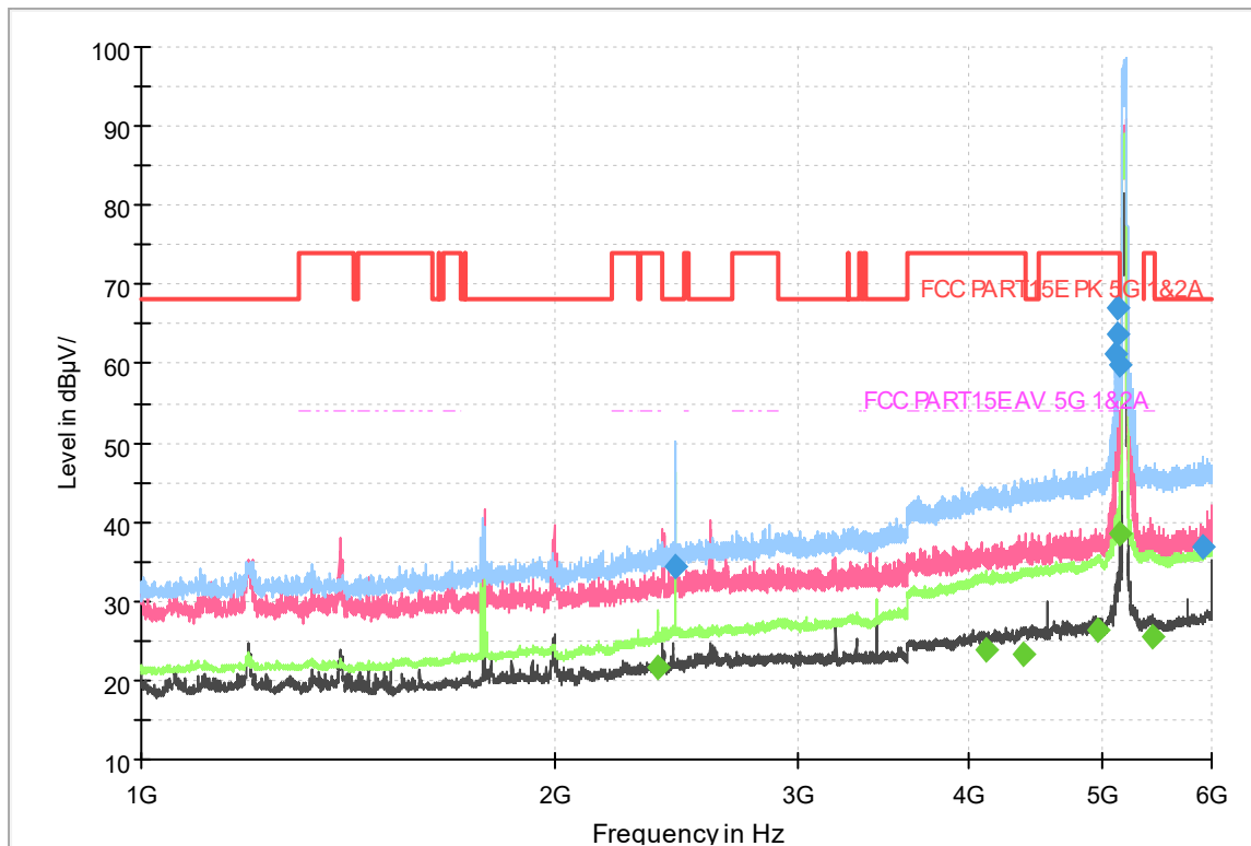
Fig.327 Radiated emission: 802.11ac(40M),CH38, 1GHz-6GHz
