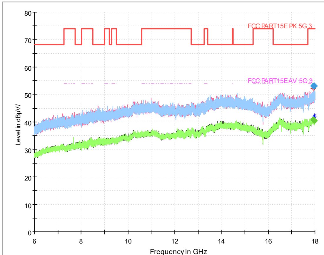
Fig.322 Radiated emission: 802.11ac(20M),CH149, 6GHz-18GHz
