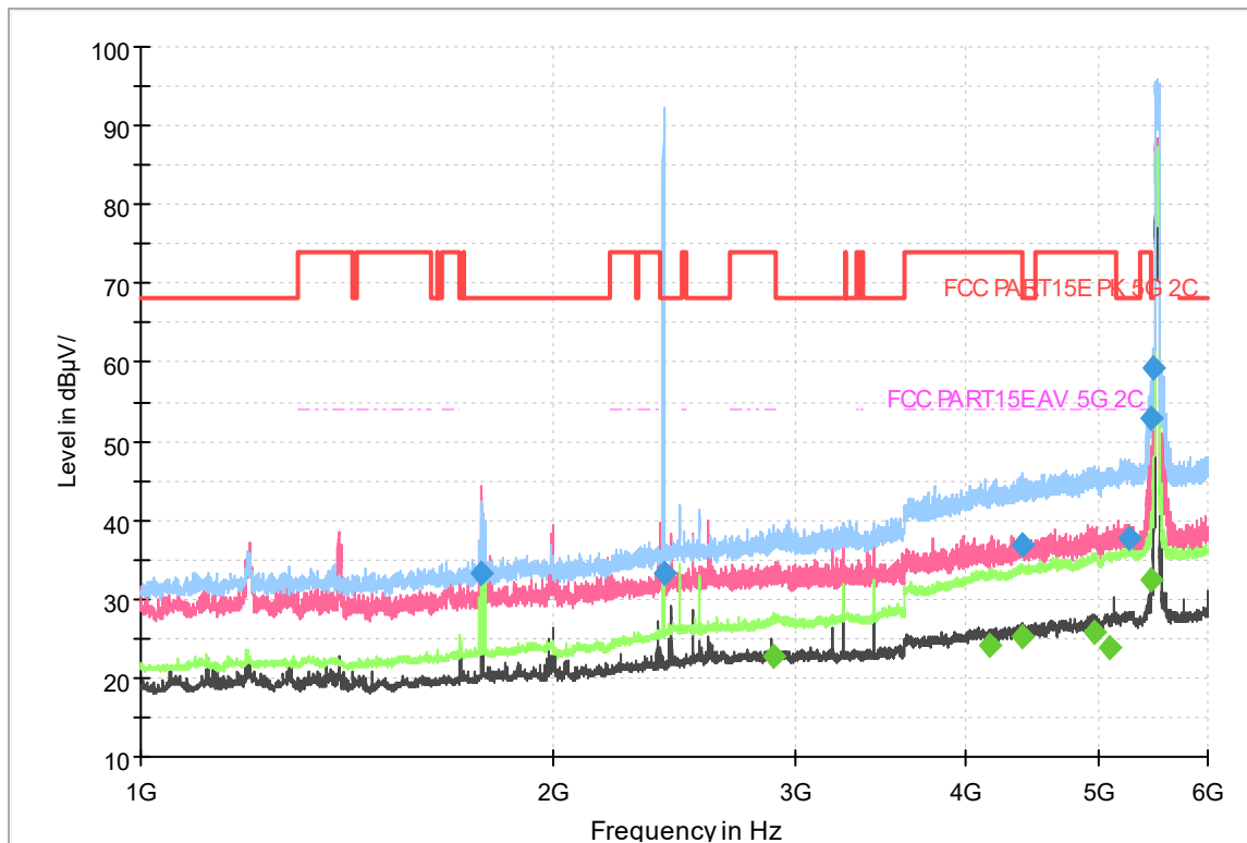
Fig.335 Radiated emission: 802.11ac(40M),CH102, 1GHz-6GHz
