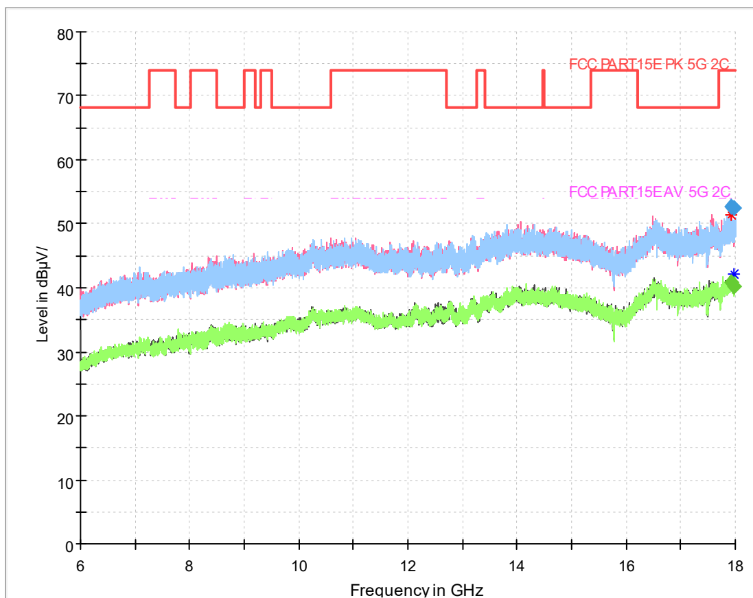
Fig.336 Radiated emission: 802.11ac(40M),CH102, 6GHz-18GHz
