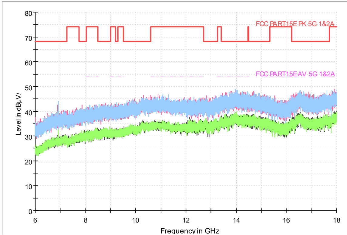
Fig.328 Radiated emission: 802.11ac(40M),CH38, 6GHz-18GHz
