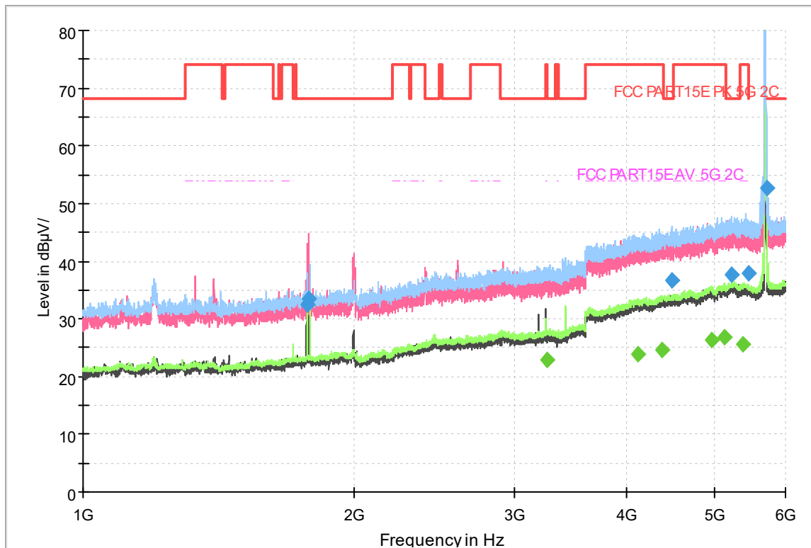
Fig.319 Radiated emission: 802.11ac(20M),CH140, 1GHz-6GHz
