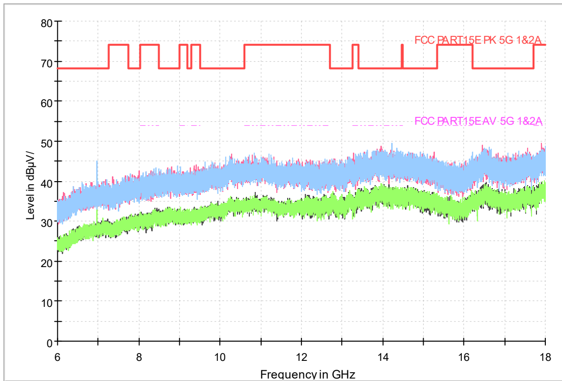
Fig.312 Radiated emission: 802.11ac(20M),CH60, 6GHz-18GHz
