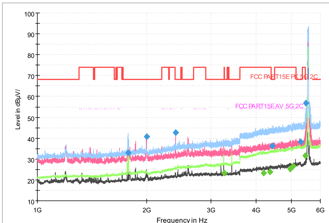
Fig.337 Radiated emission: 802.11ac(40M),CH118, 1GHz-6GHz
