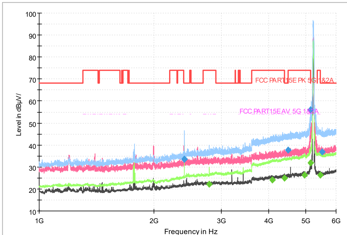
Fig.329 Radiated emission: 802.11ac(40M),CH46, 1GHz-6GHz
