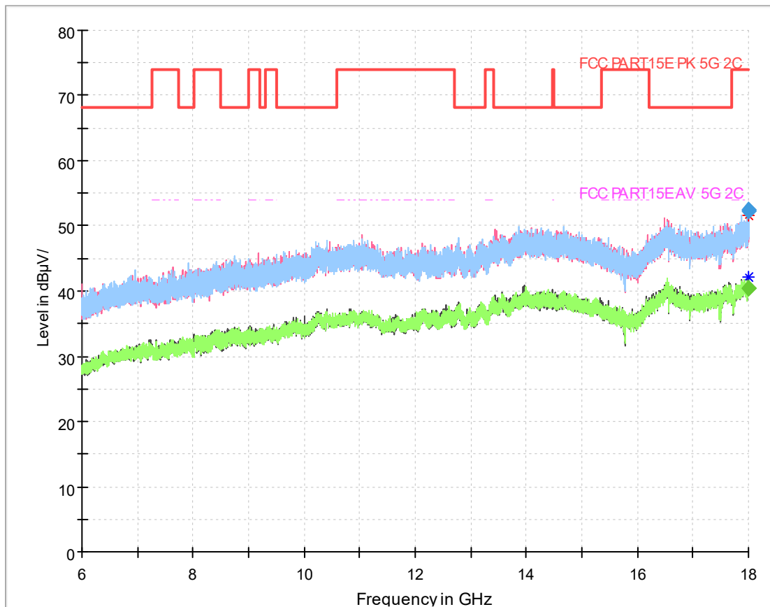
Fig.338 Radiated emission: 802.11ac(40M),CH118, 6GHz-18GHz
