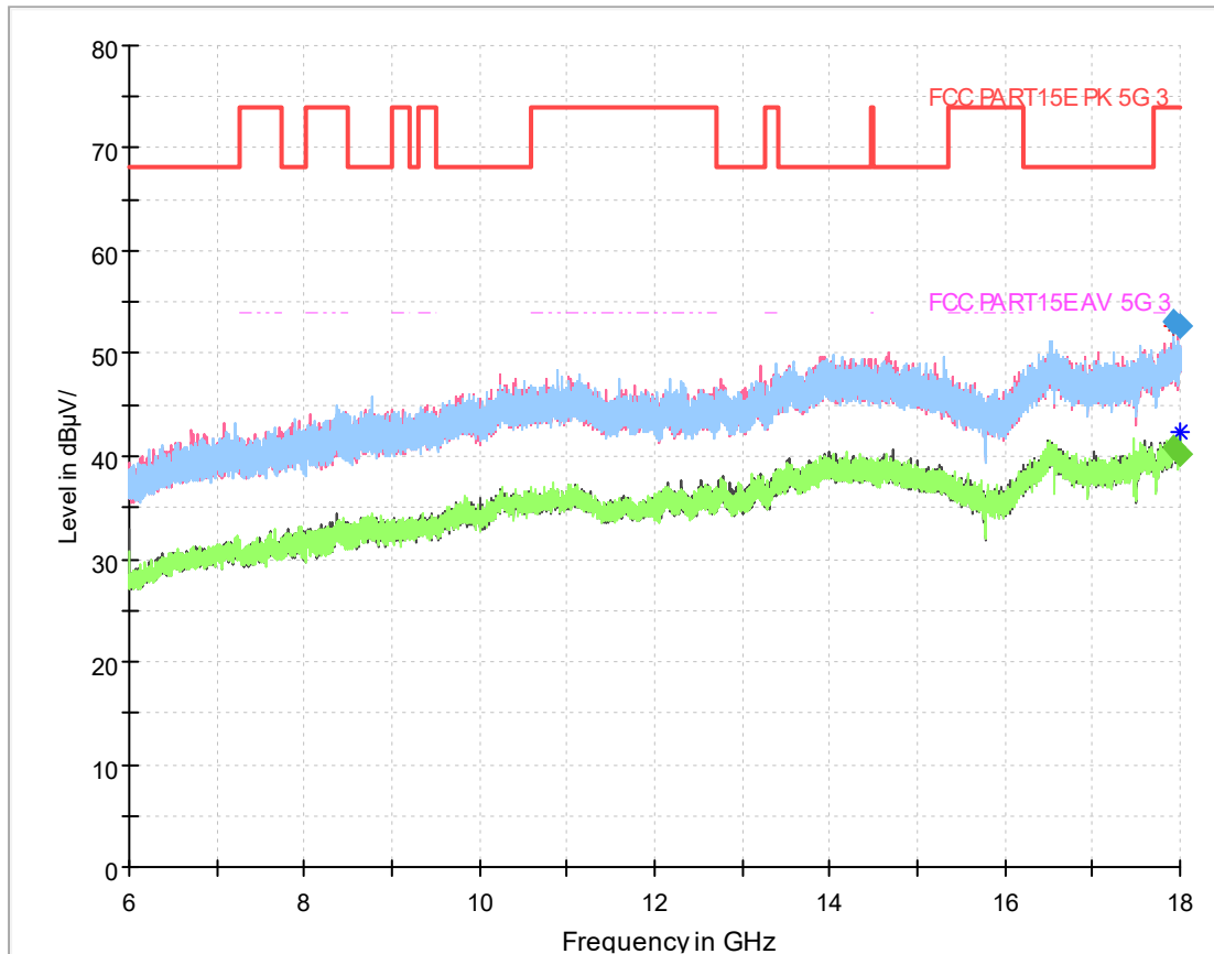
Fig.326 Radiated emission: 802.11ac(20M),CH165, 6GHz-18GHz
