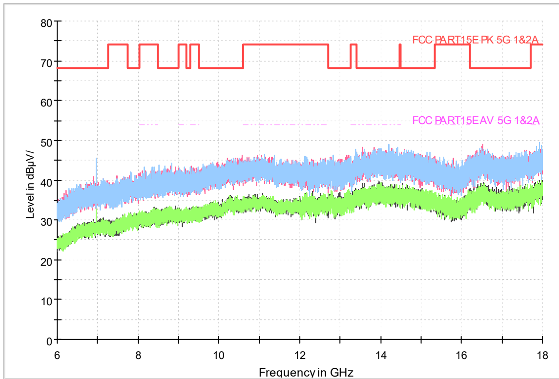
Fig.332 Radiated emission: 802.11ac(40M),CH54, 6GHz-18GHz
