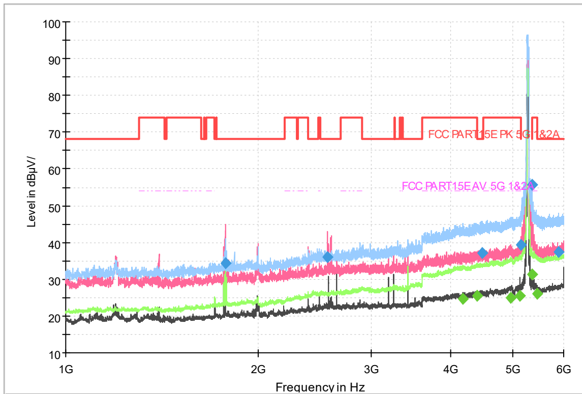
Fig.331 Radiated emission: 802.11ac(40M),CH54, 1GHz-6GHz
