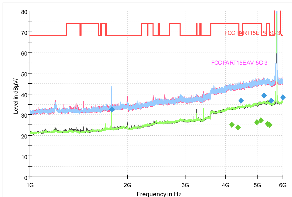
Fig.321 Radiated emission: 802.11ac(20M),CH149, 1GHz-6GHz
