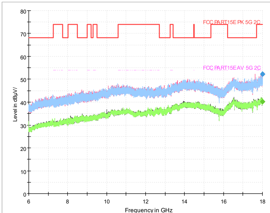
Fig.318 Radiated emission: 802.11ac(20M),CH116, 6GHz-18GHz
