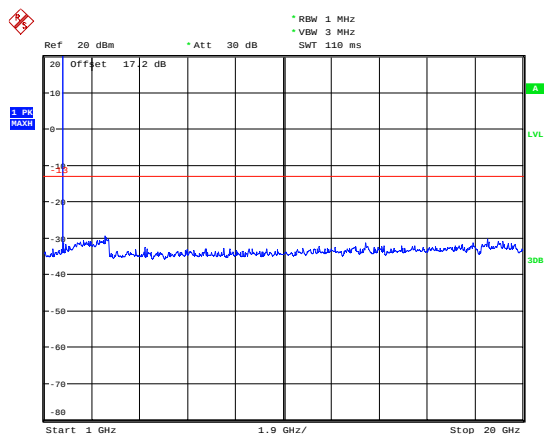
WCDMA Band IV CH-High 1GHz ~20GHz
