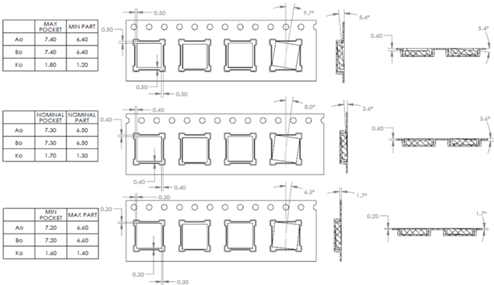
Figure 9.3. Tape information
