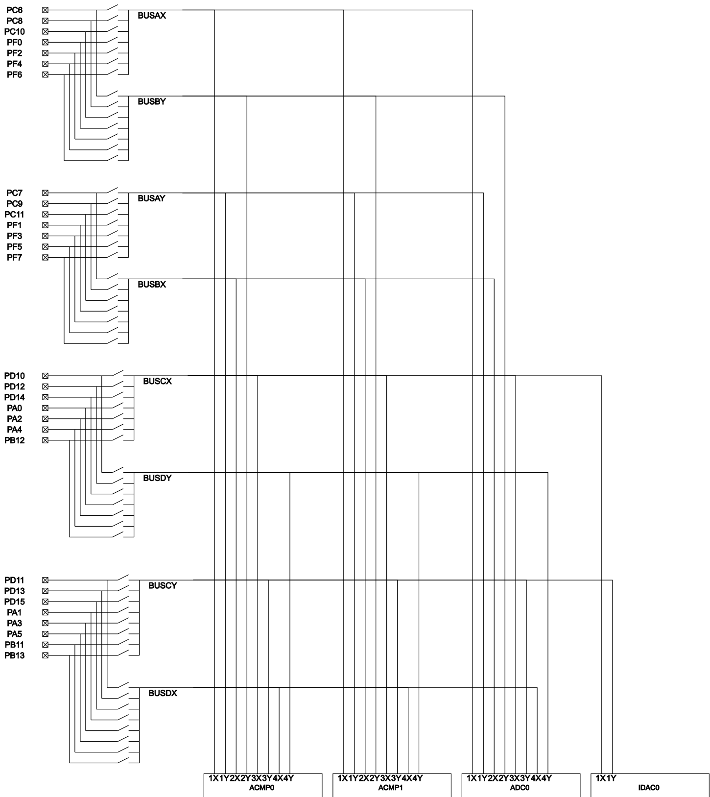
Figure 7.2. BGM121/BGM123 APORT
