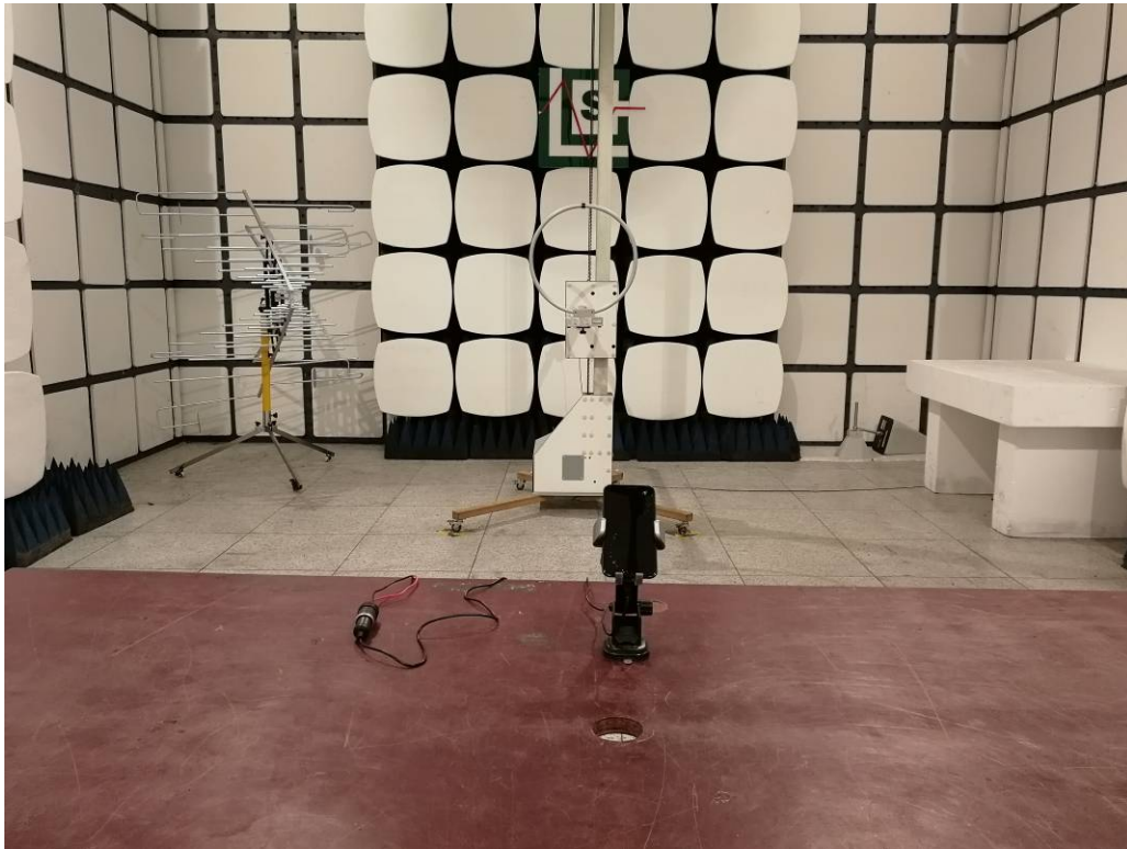
Radiated Emission below 30MHz- Car Charger charge mode
