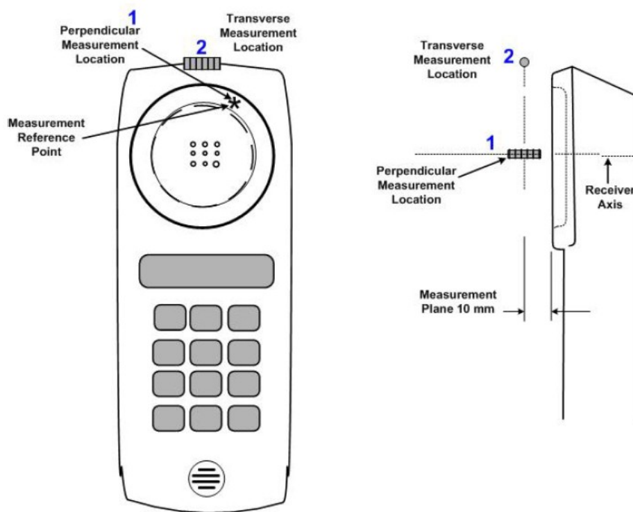
Fig2.2 A typical EUT reference and plane for T-Coil measurement
