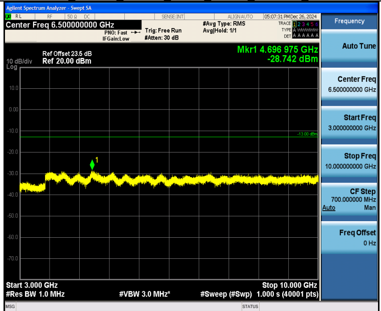
Band26 1.4MHz 16QAM 26783 1RB#5 3000~10000 3000~10000
