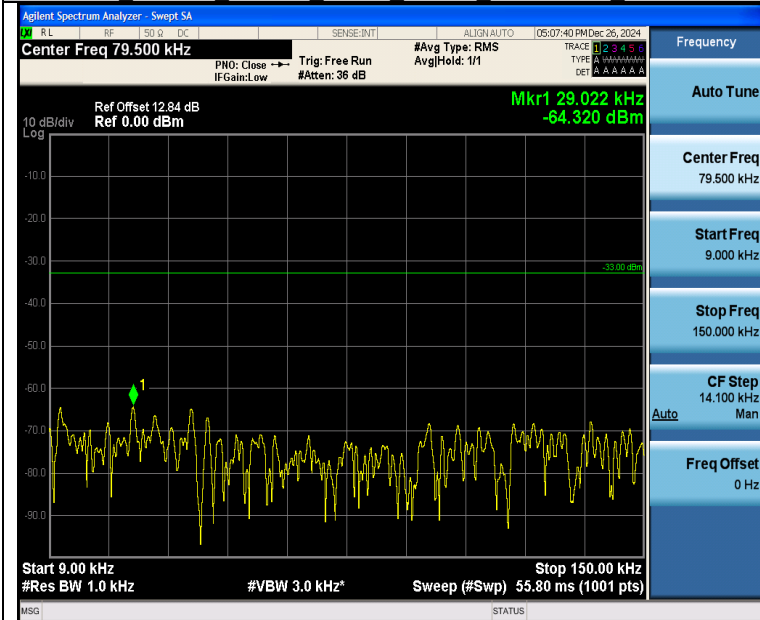
Band26 1.4MHz_QPSK 26783 6RB#0 0.009~0.15 0.009~0.15
