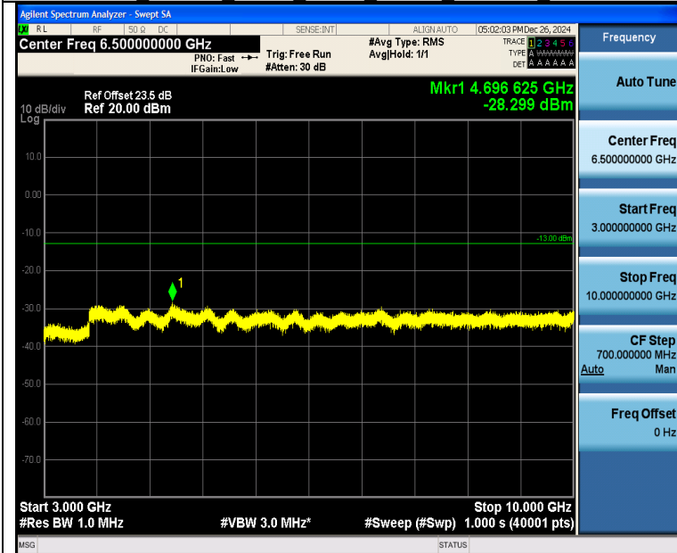
Band26 1.4MHz QPSK 26740 6RB#0 3000~10000 3000~10000
