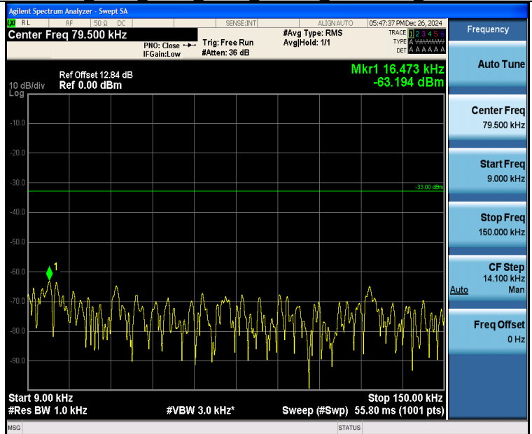
Band26_3MHz_16QAM_26705_1RB#14_0.009~0.15_0.009~0.15
