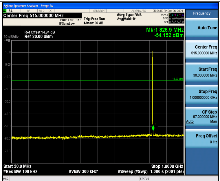
Band26 1.4MHz 16QAM 26783 1RB#5 30~1000 30~1000
