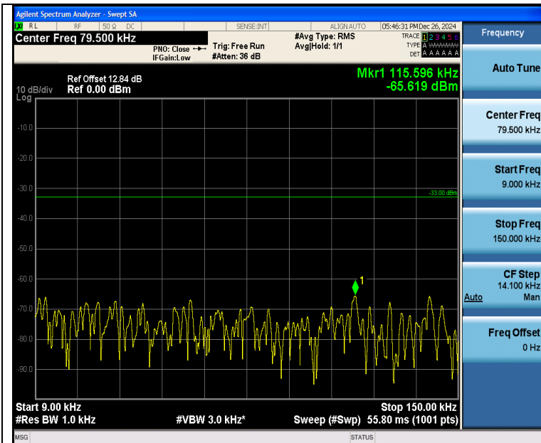
Band26 3MHz QPSK 26705 1RB#14 0.009~0.15 0.009~0.15
