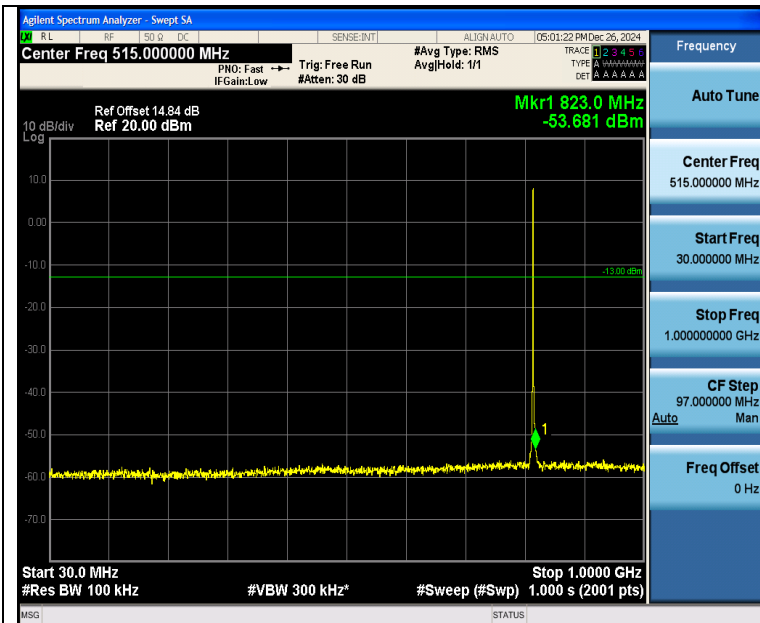
Band26 1.4MHz QPSK 26740 6RB#0 30~1000 30~1000
