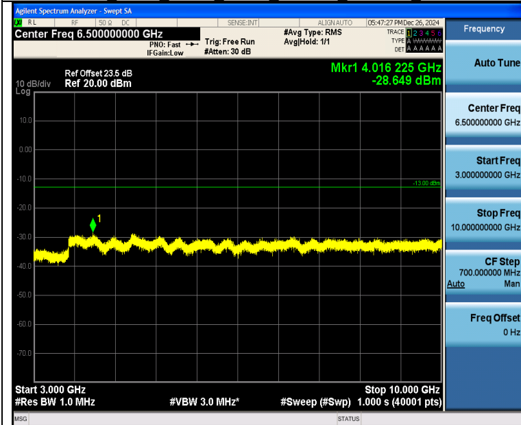
Band26_3MHz_QPSK_26705_1RB#14_3000~10000_3000~10000
