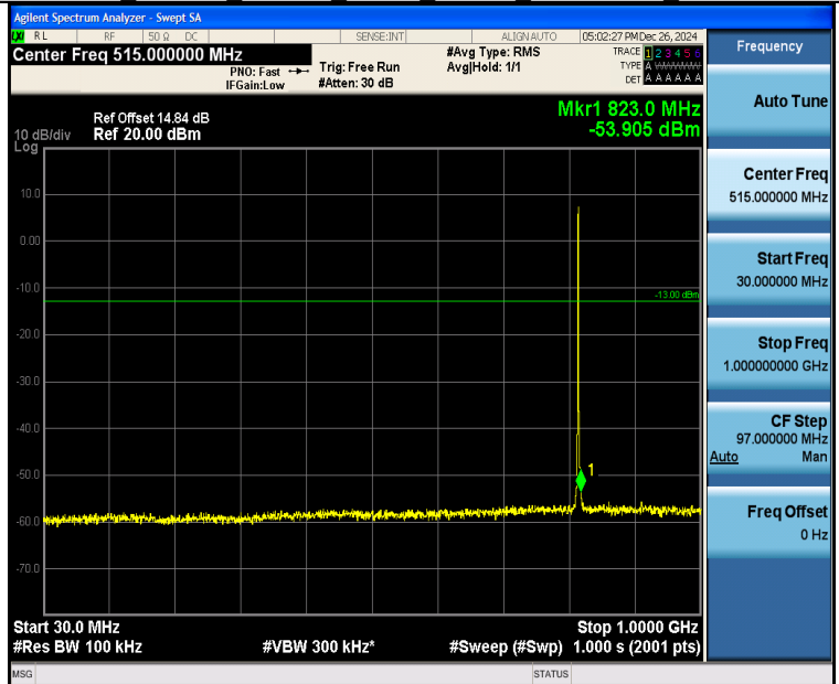
Band26 1.4MHz 16QAM 26740 6RB#0 30~1000 30~1000
